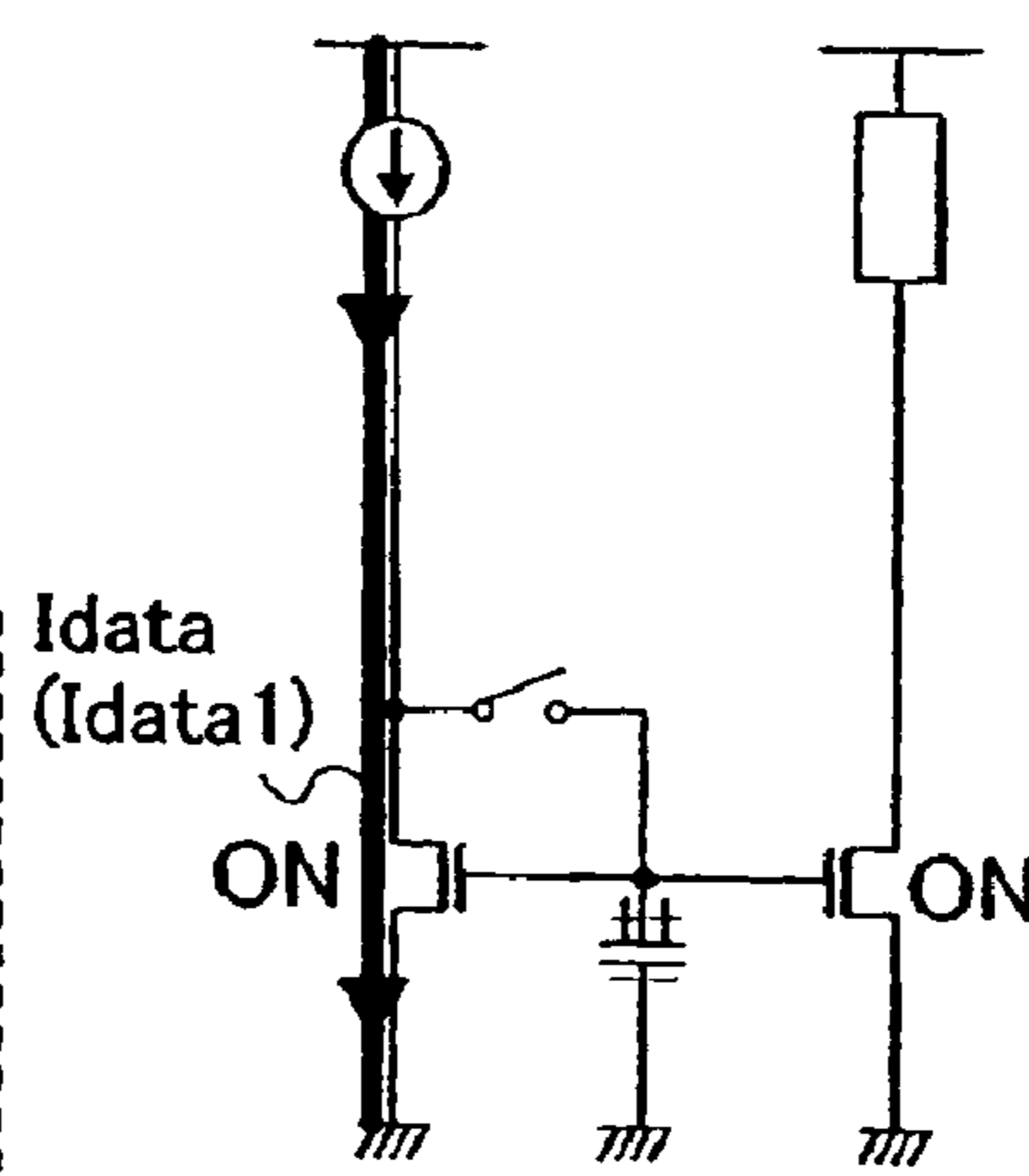
Fig. 20B signal input complete time
