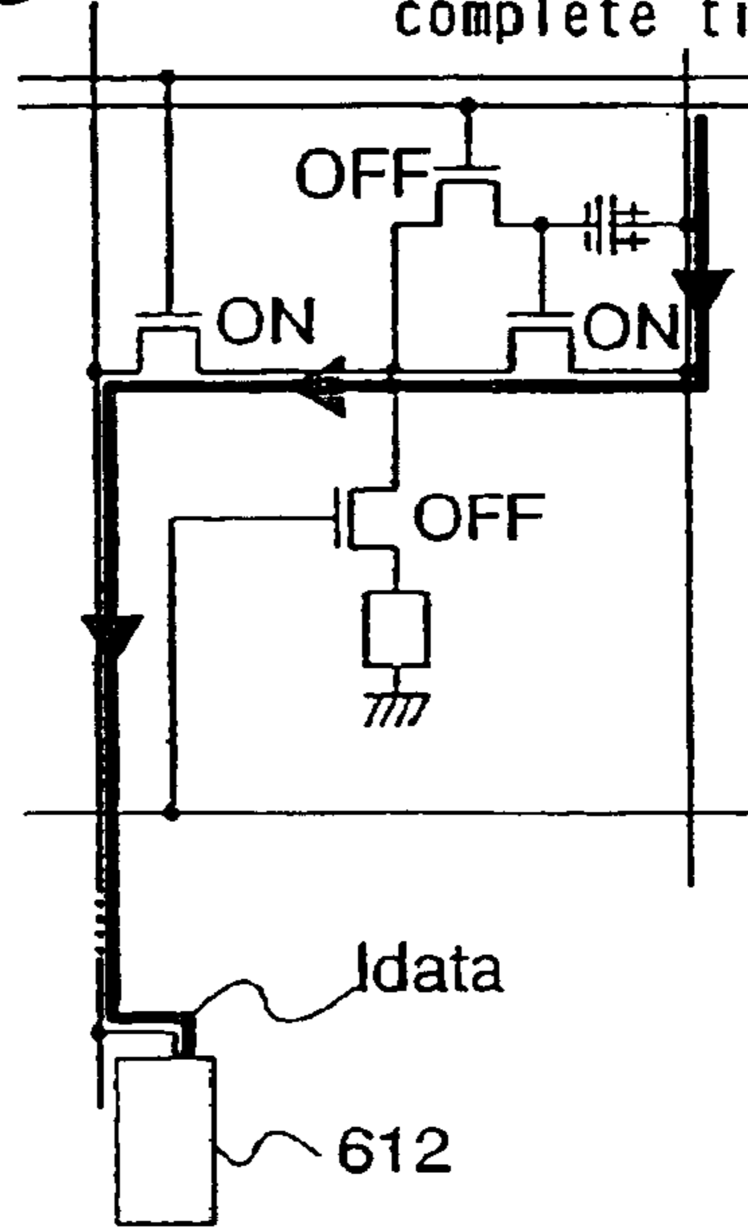
Fig. 17D PRIOR ART
