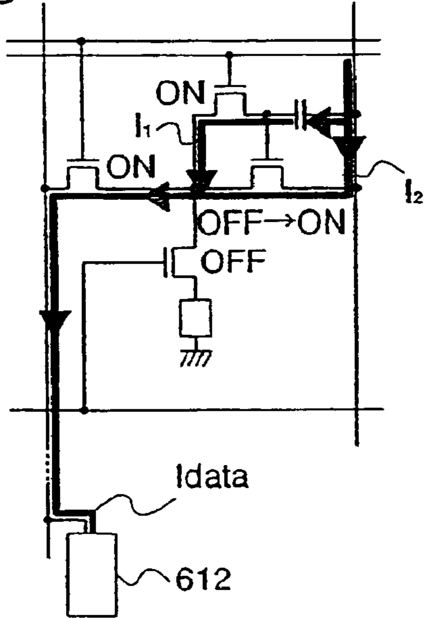
Fig. 17A signal input time
