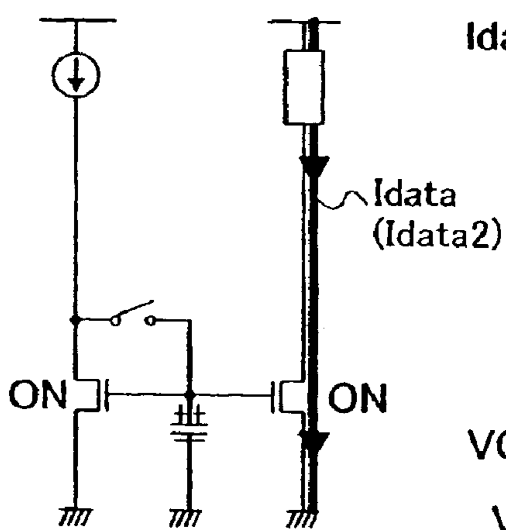
Fig. 20C signal input time to pixel
