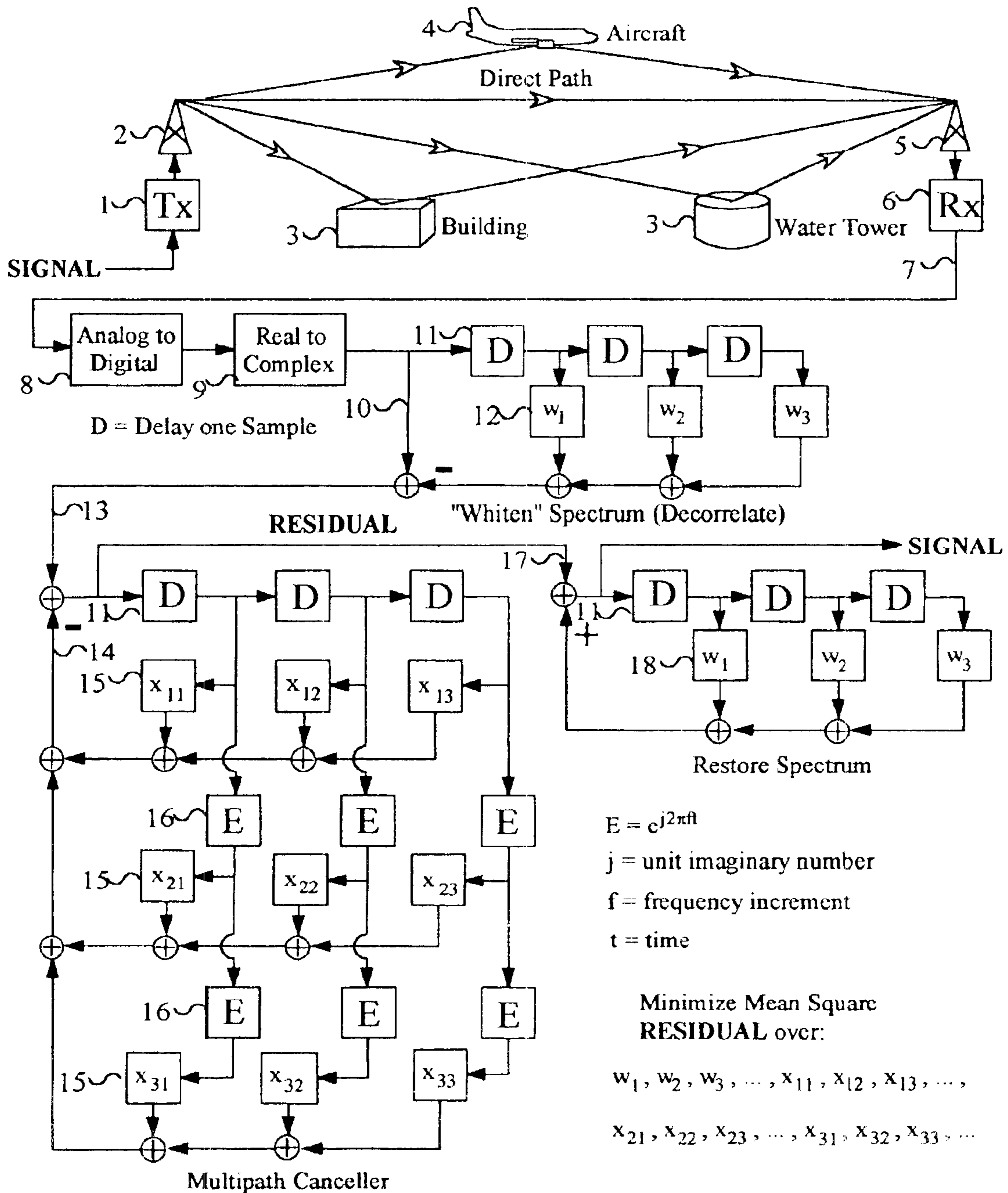
ADAPTIVE FILTER TO REDUCE MULTIPATH
