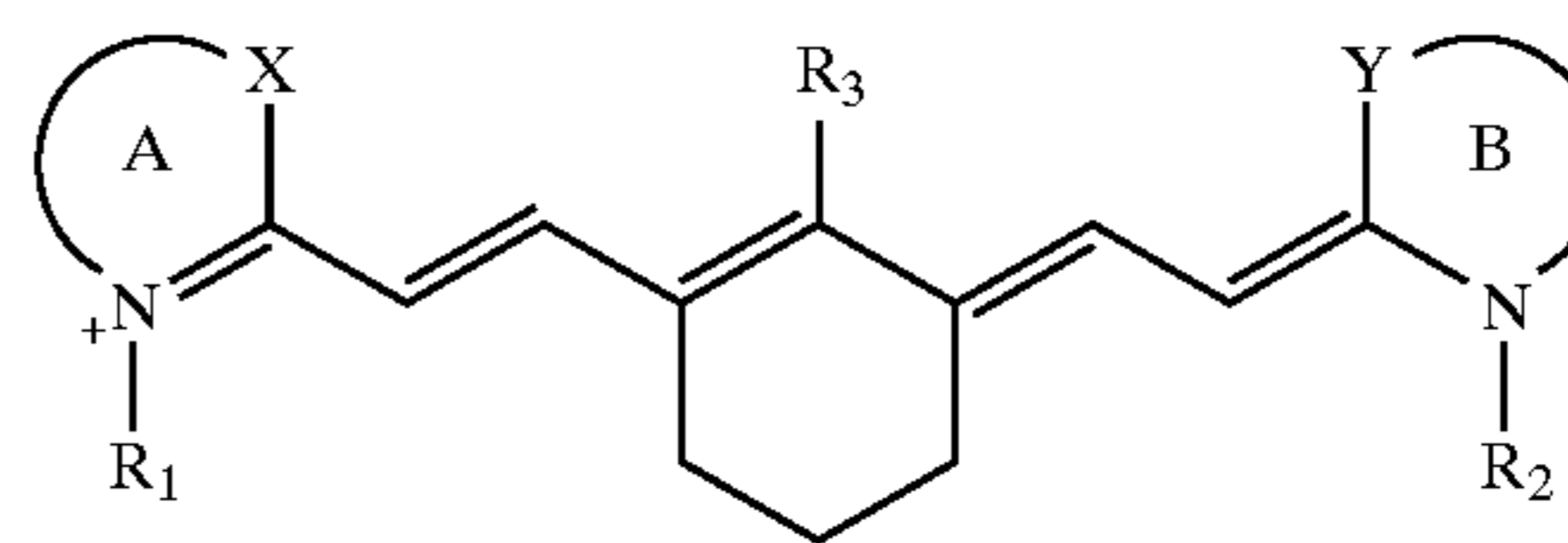
Structure B. A Ring-Locked Tricyanocyanine Chromophore.
