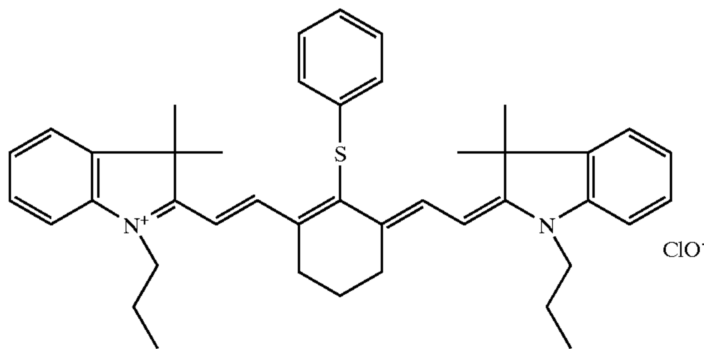
Structure D. IR 792 Perchlorate.
