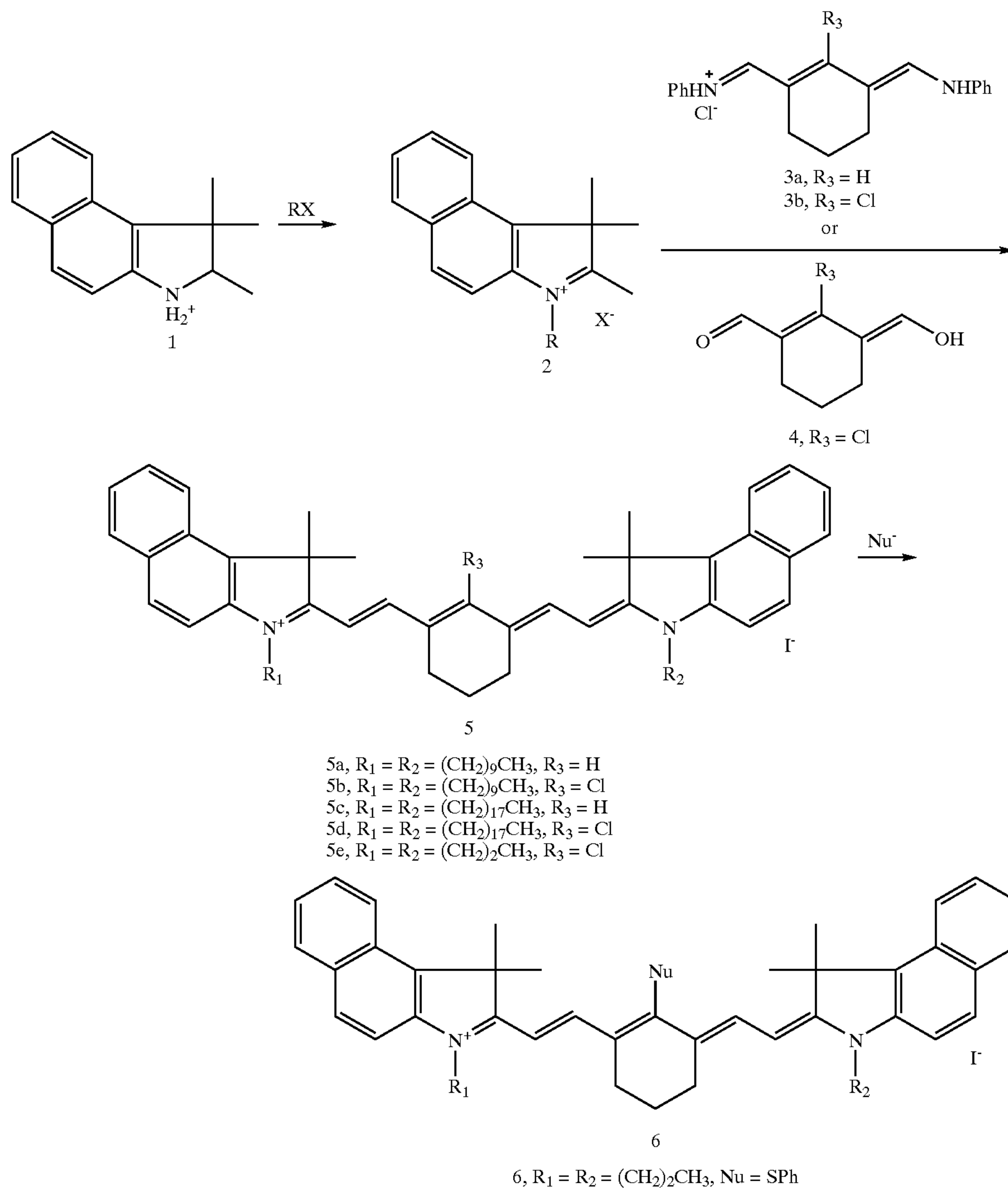
Scheme 1 Synthesis of Ring-locked Benzo-indotricarbocyanine Compounds.
