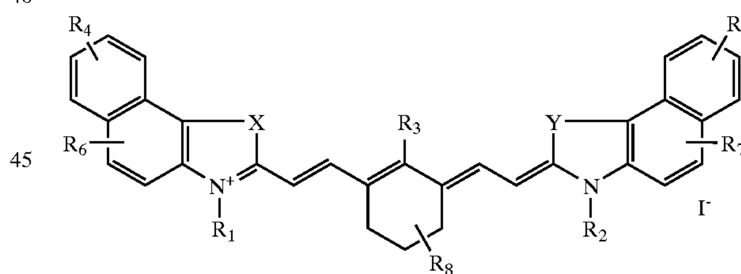
Structure C. Ring-Locked Benzo-indotricarbocyanine Compounds.
