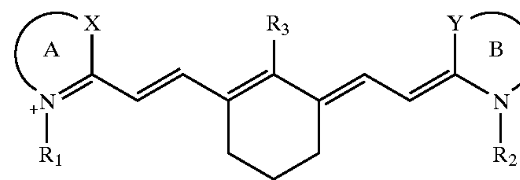
Structure B. A Ring-Locked Tricyanocyanine Chromophore.
