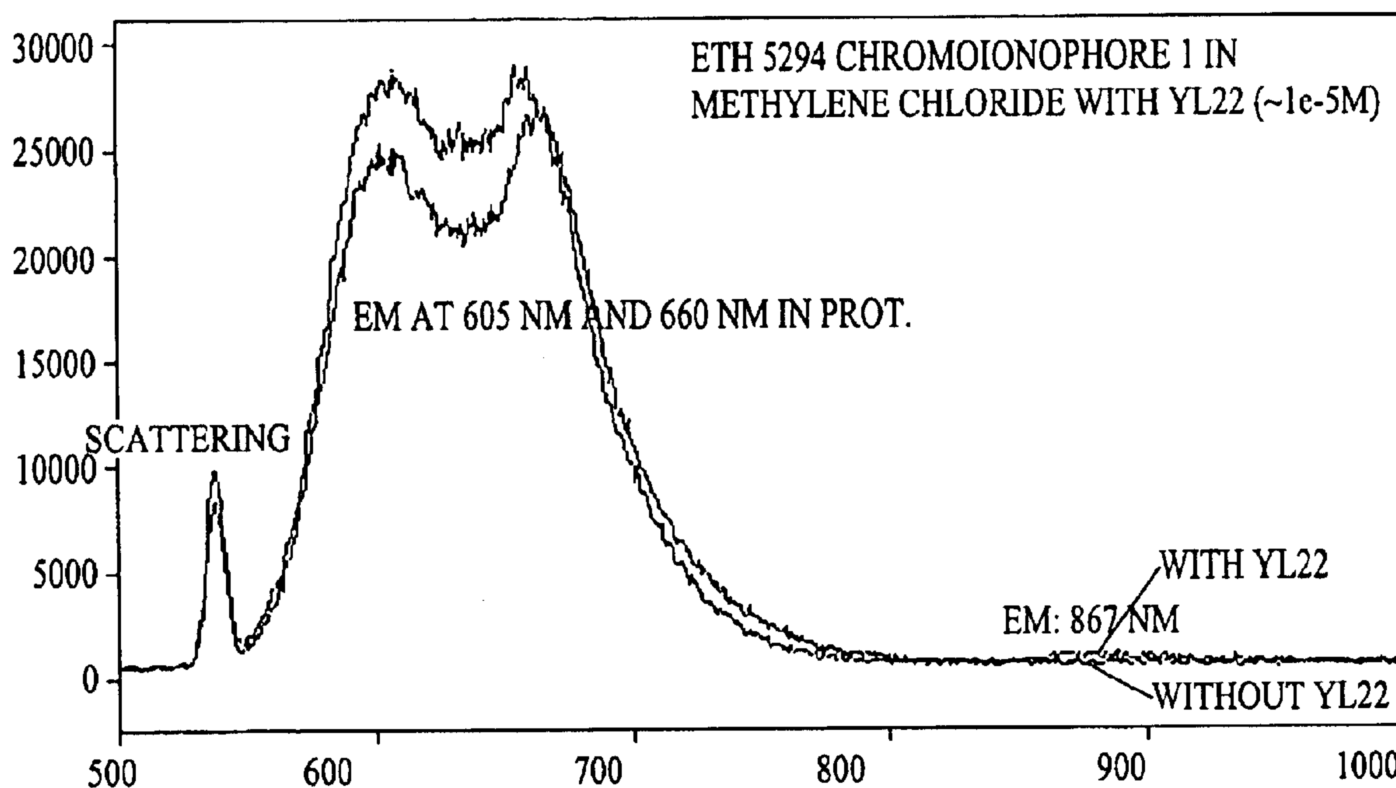
EMISSION SPECTRA OF ETH 5294 AND COMPOUND 6 MIXTURE IN METHYLENE CHLORIDE. EXCITATION WAVELENGTH IS AT 539 NM
