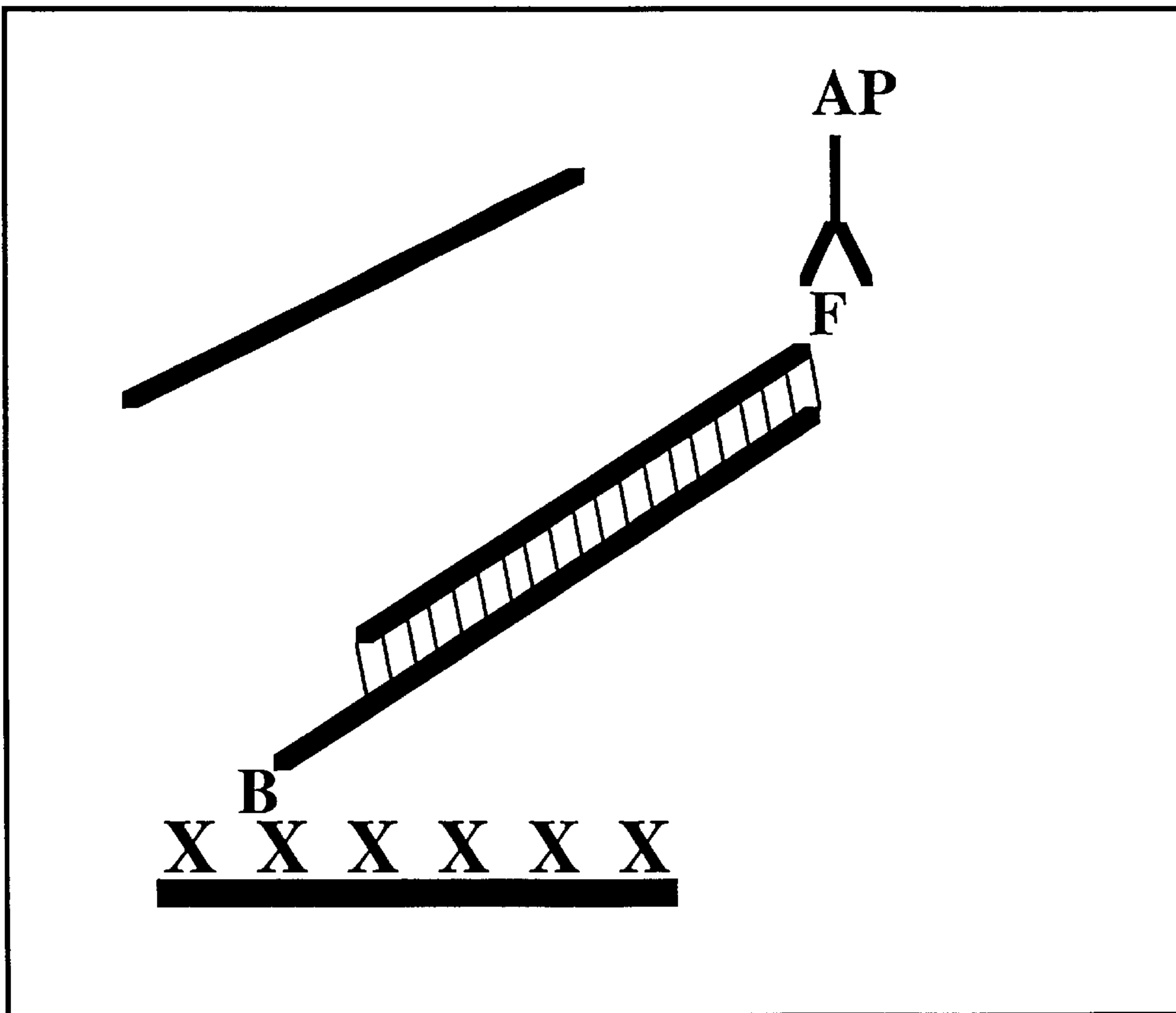
Figure 3 Molecular Diagram
