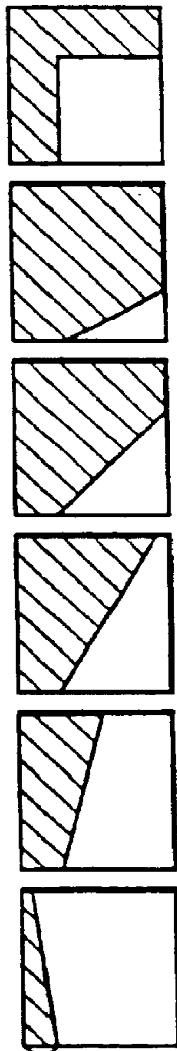
RL M=2
