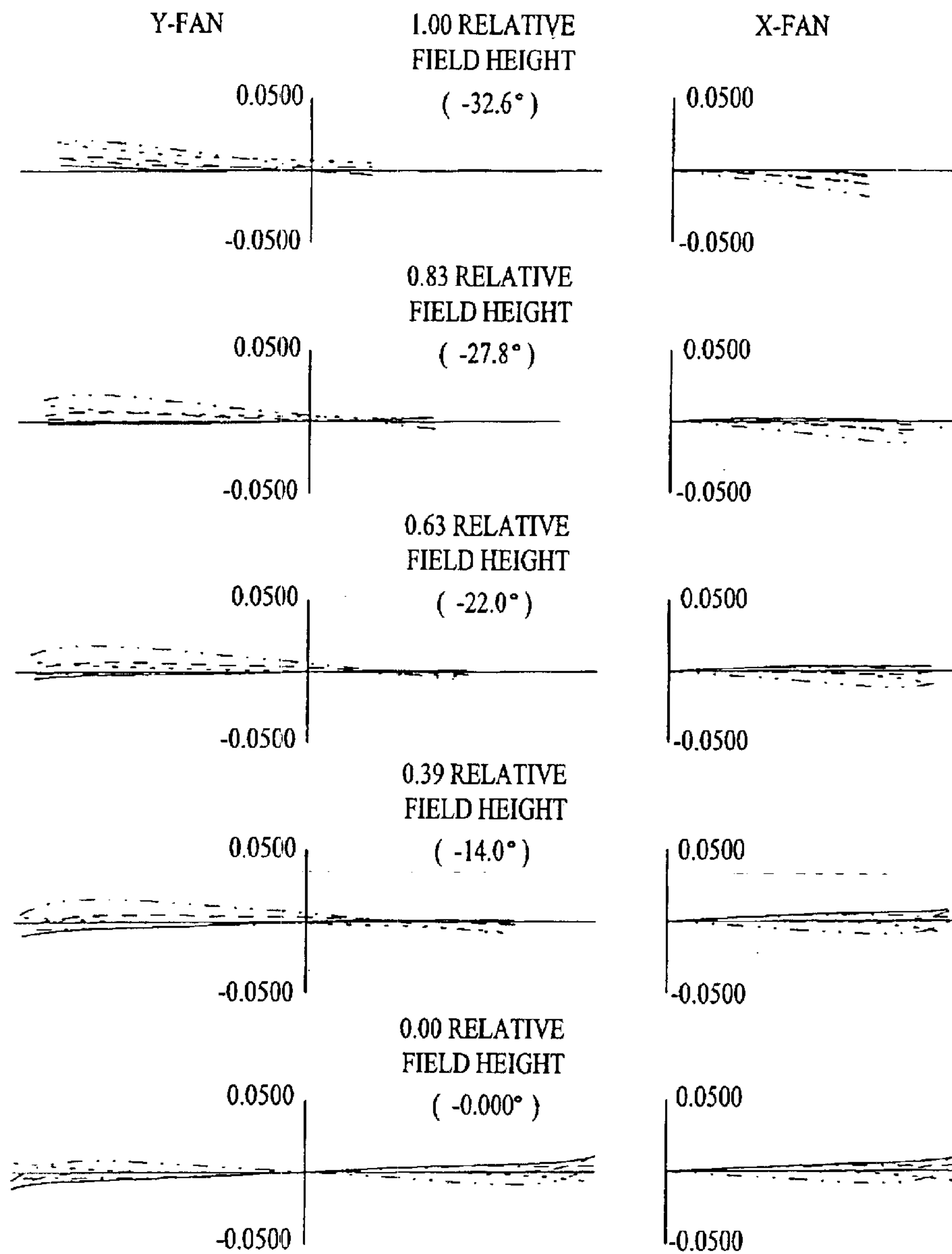
Fig. 40 RAY ABERRATIONS (MILLIMETERS) POSITION 2 ----- 643.8469 NM ----- 587.5600 NM ----- 546.0700 NM ----- 486.1300 NM ----- 460.0000 NM
