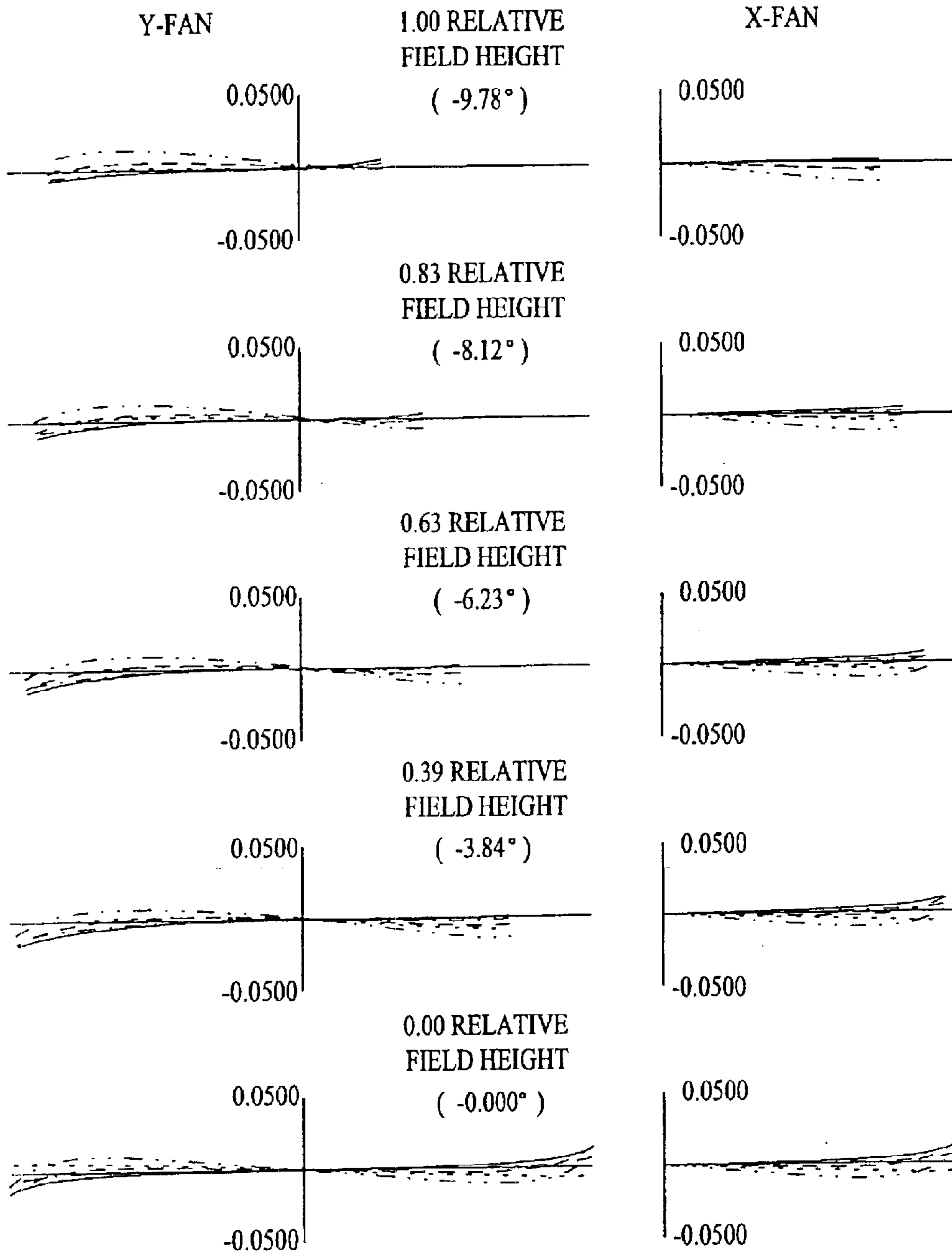
FIG. 43 RAY ABERRATIONS ( MILLIMETERS ) ----- 643.8469 NM ----- 587.5600 NM POSITION 5 ----- 546.0700 NM ----- 486.1300 NM ----- 460.0000 NM
