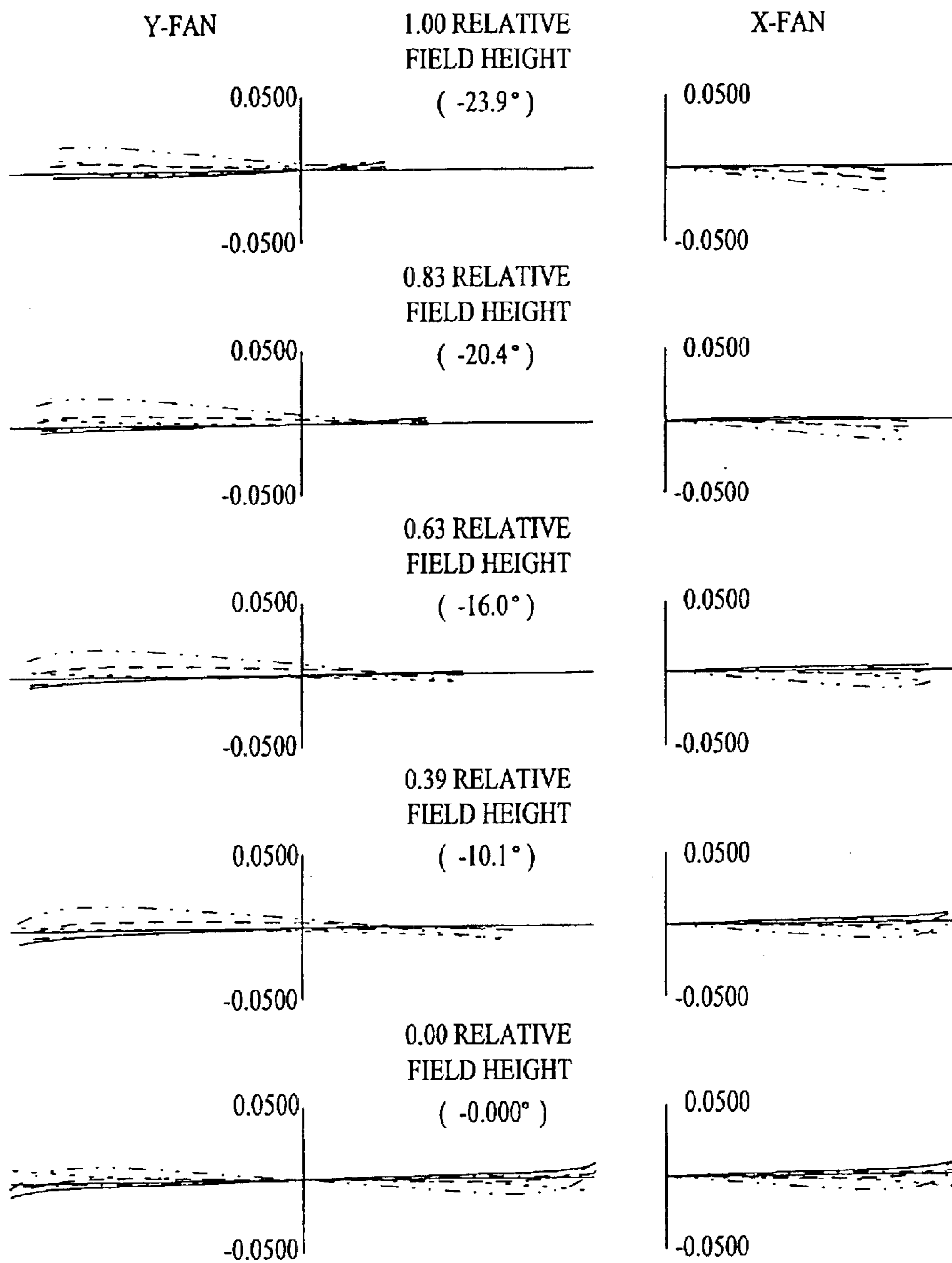
Fig. 41 RAY ABERRATIONS (MILLIMETERS) POSITION 3 ----- 643.8469 NM - - - - - 587.5600 NM _____ 546.0700 NM - - - - - 486.1300 NM ----- 460.0000 NM
