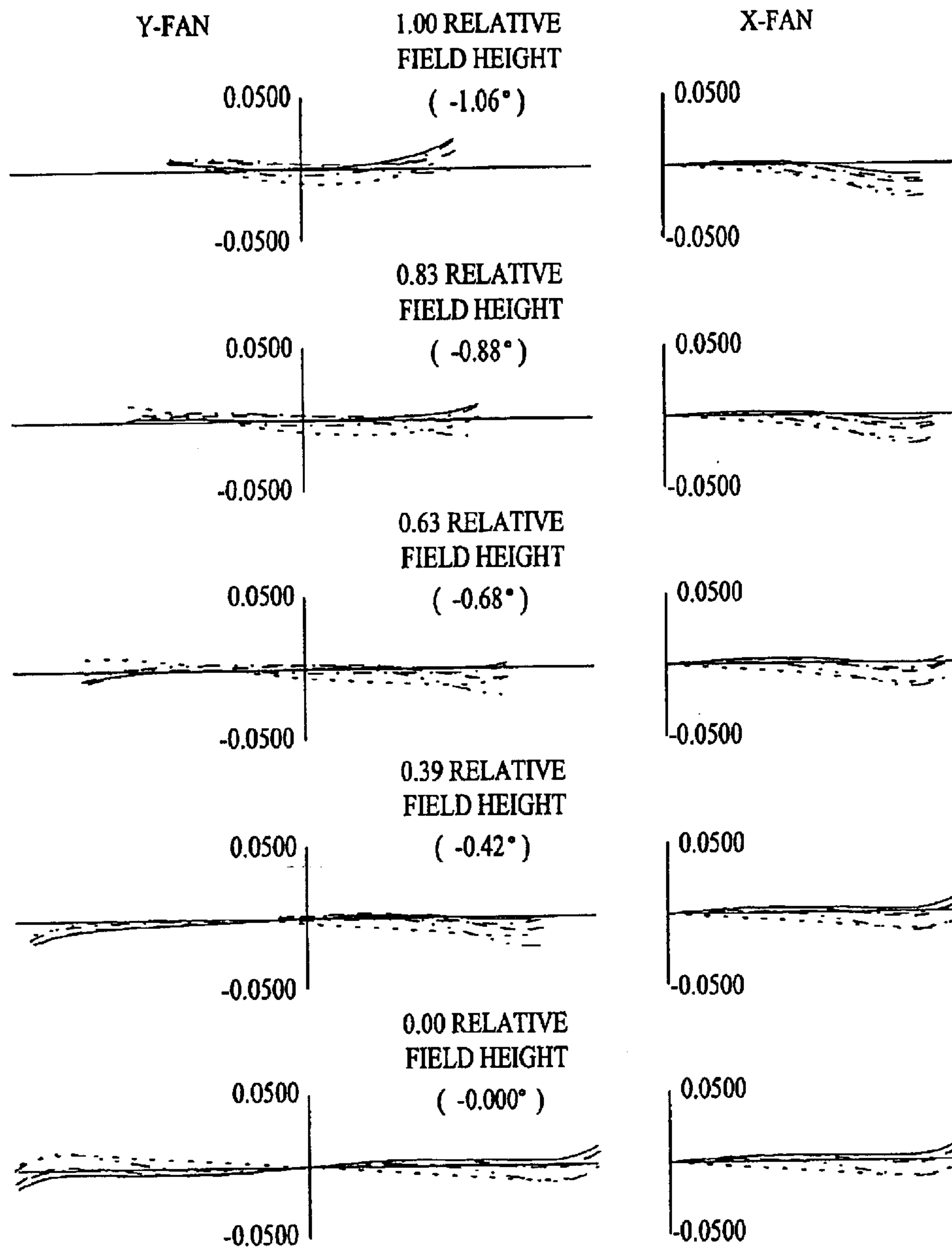
FIG. 58 RAY ABERRATIONS (MILLIMETERS) ----- 643.8469 NM ----- 587.5600 NM ----- 546.0700 NM ----- 486.1300 NM ----- 460.0000 NM POSITION 20
