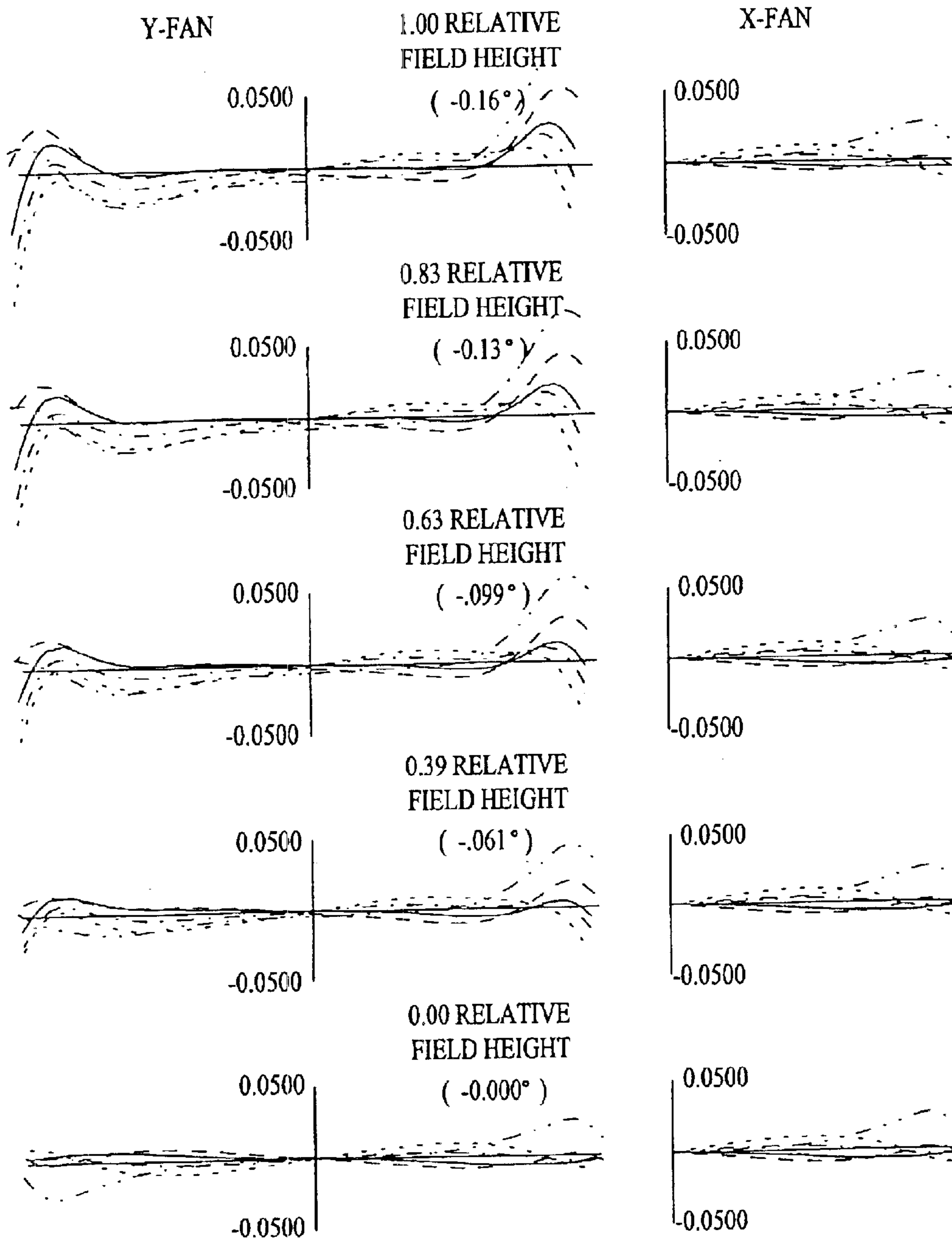
FIG. 50 RAY ABERRATIONS (MILLIMETERS) ----- 643.8469 NM ----- 587.5600 NM POSITION 12 ----- 546.0700 NM ----- 486.1300 NM ----- 460.0000 NM
