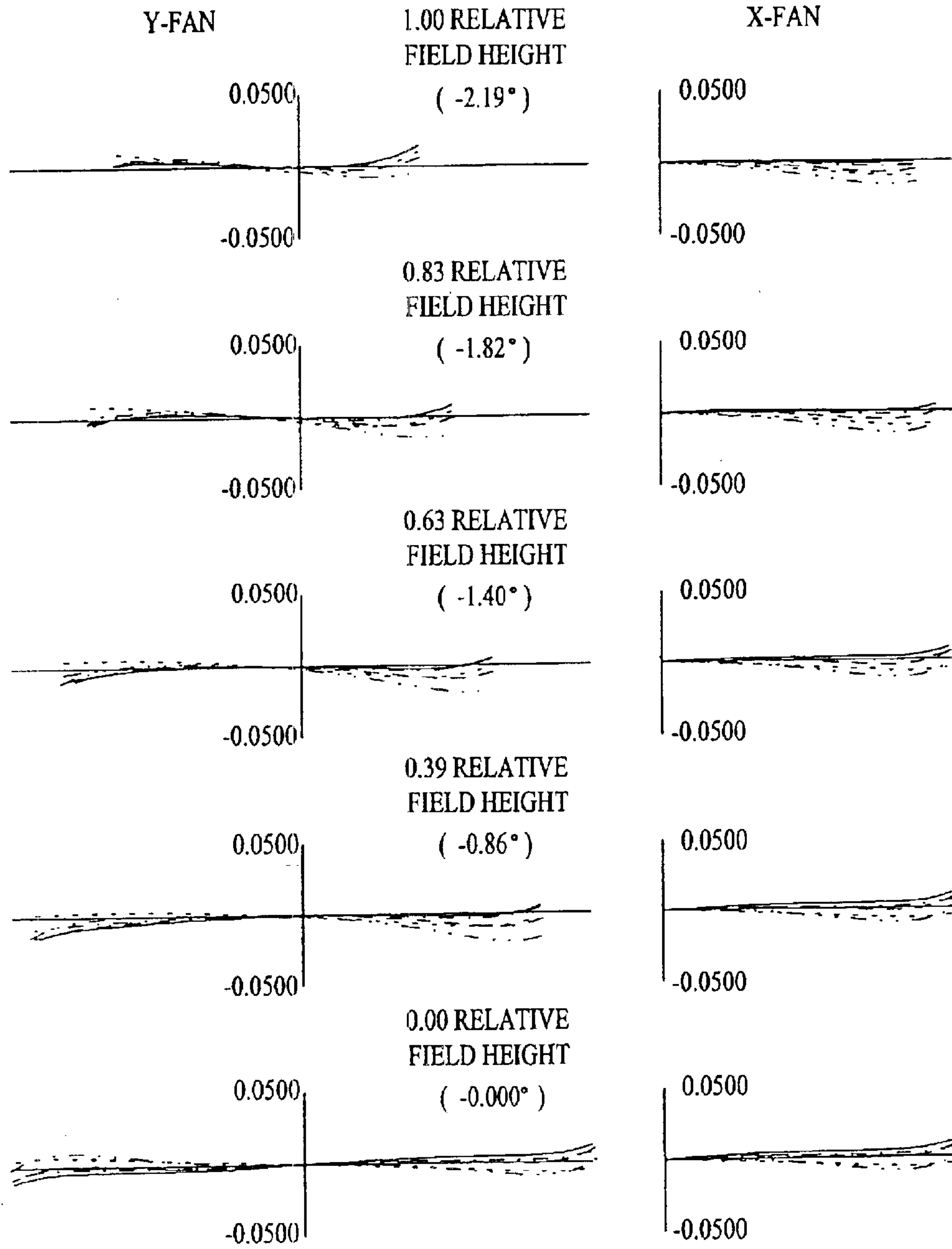
FIG. 40 RAY ABERRATIONS (MILLIMETERS) ----- 643.8469 NM ----- 587.5600 NM POSITION 8 ----- 546.0700 NM ----- 486.1300 NM ----- 460.0000 NM
