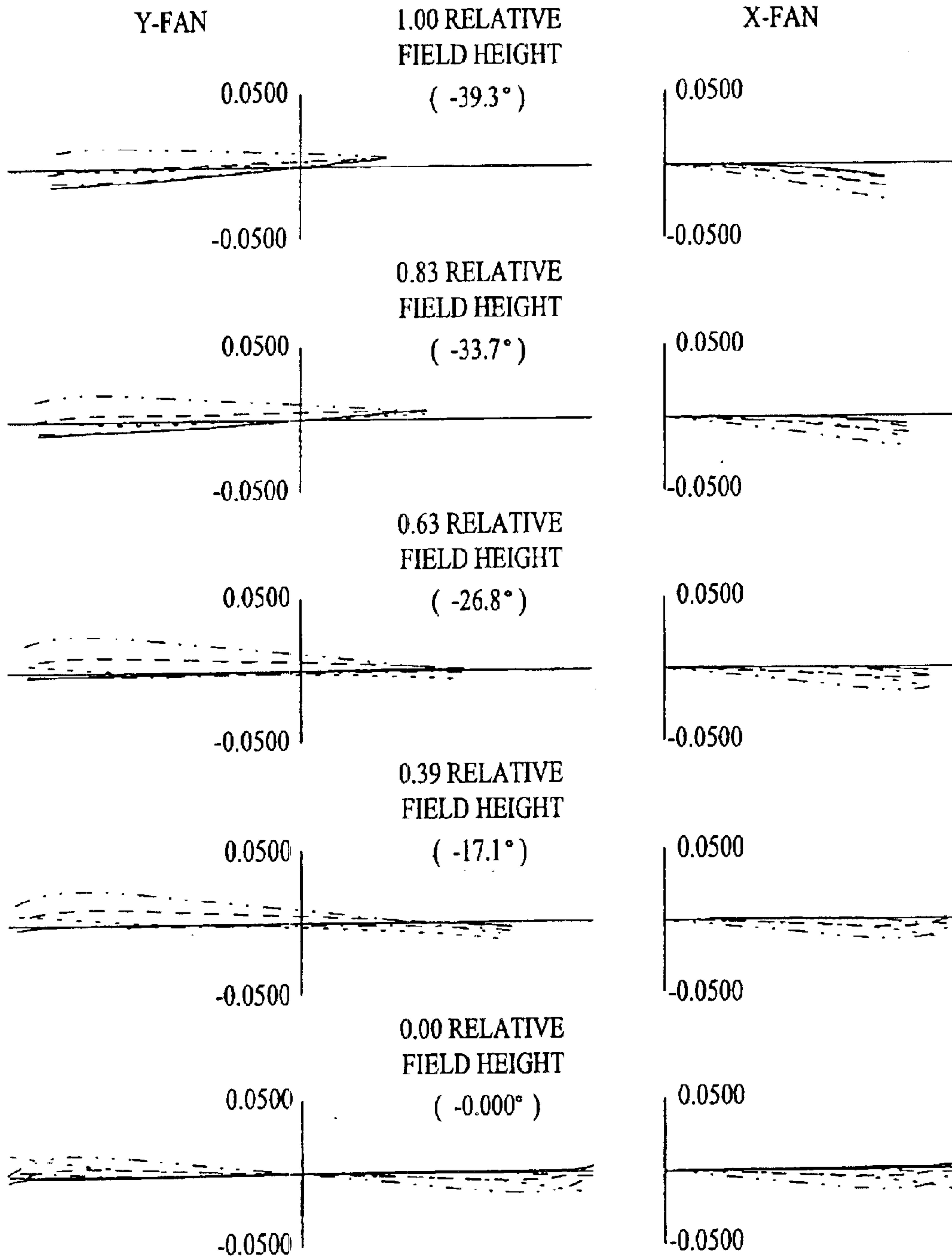
Fig. 50 RAY ABERRATIONS (MILLIMETERS) POSITION 18 ----- 643.8469 NM ----- 587.5600 NM ----- 546.0700 NM ----- 486.1300 NM ----- 460.0000 NM
