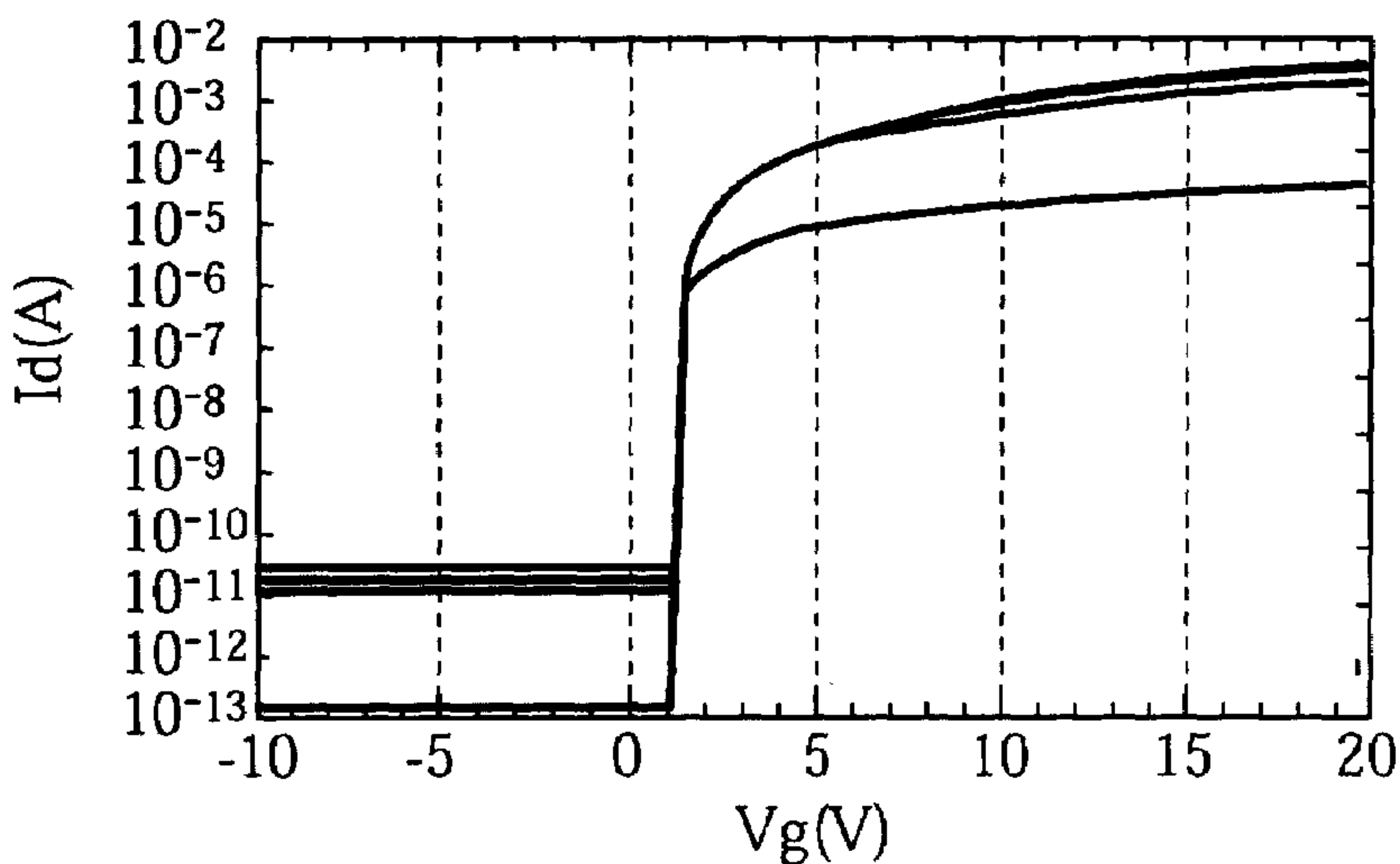
Characteristics of Mos-Tr ( Crystalline Silicon )
