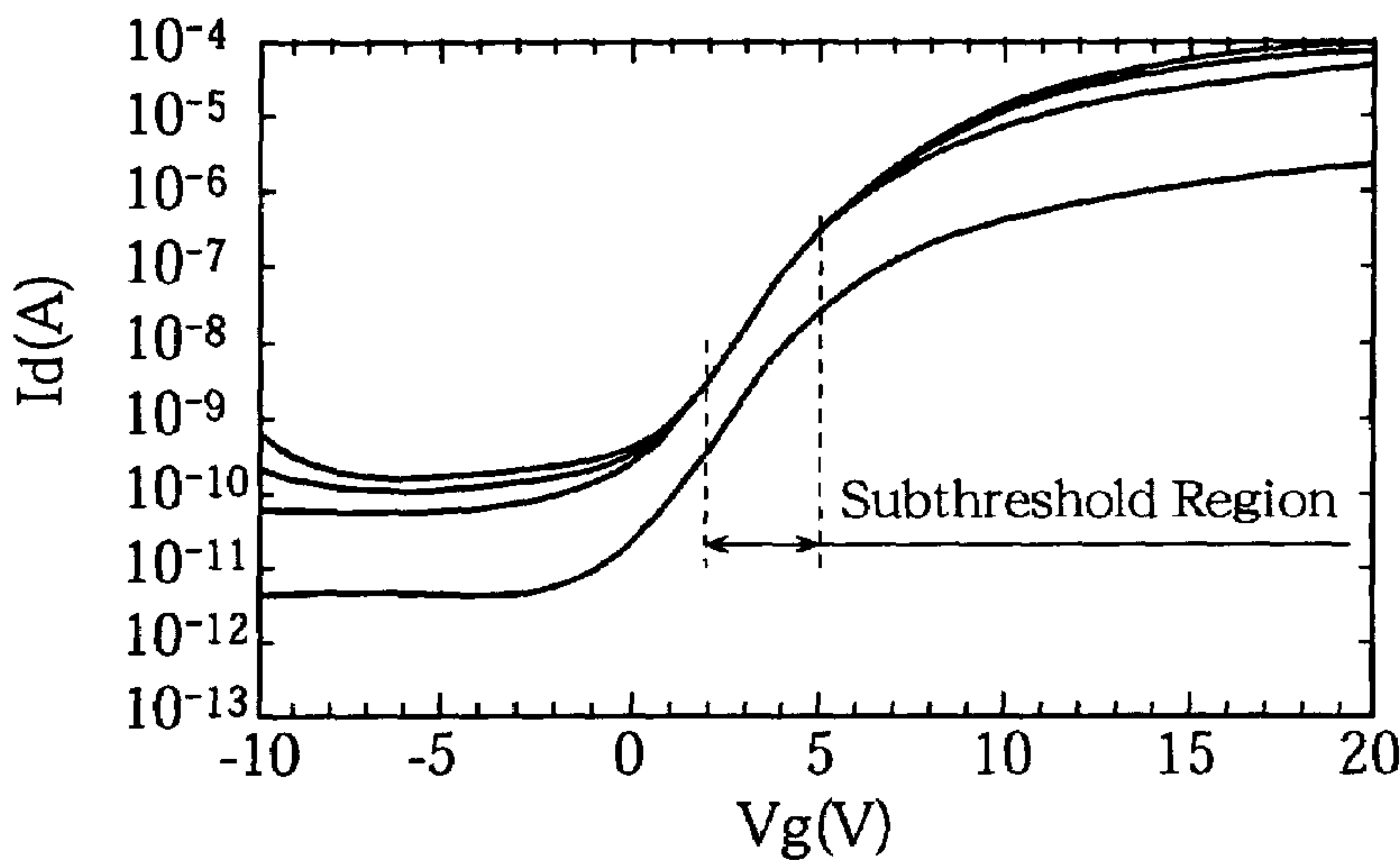
Characteristics of Polysilicon TFT
