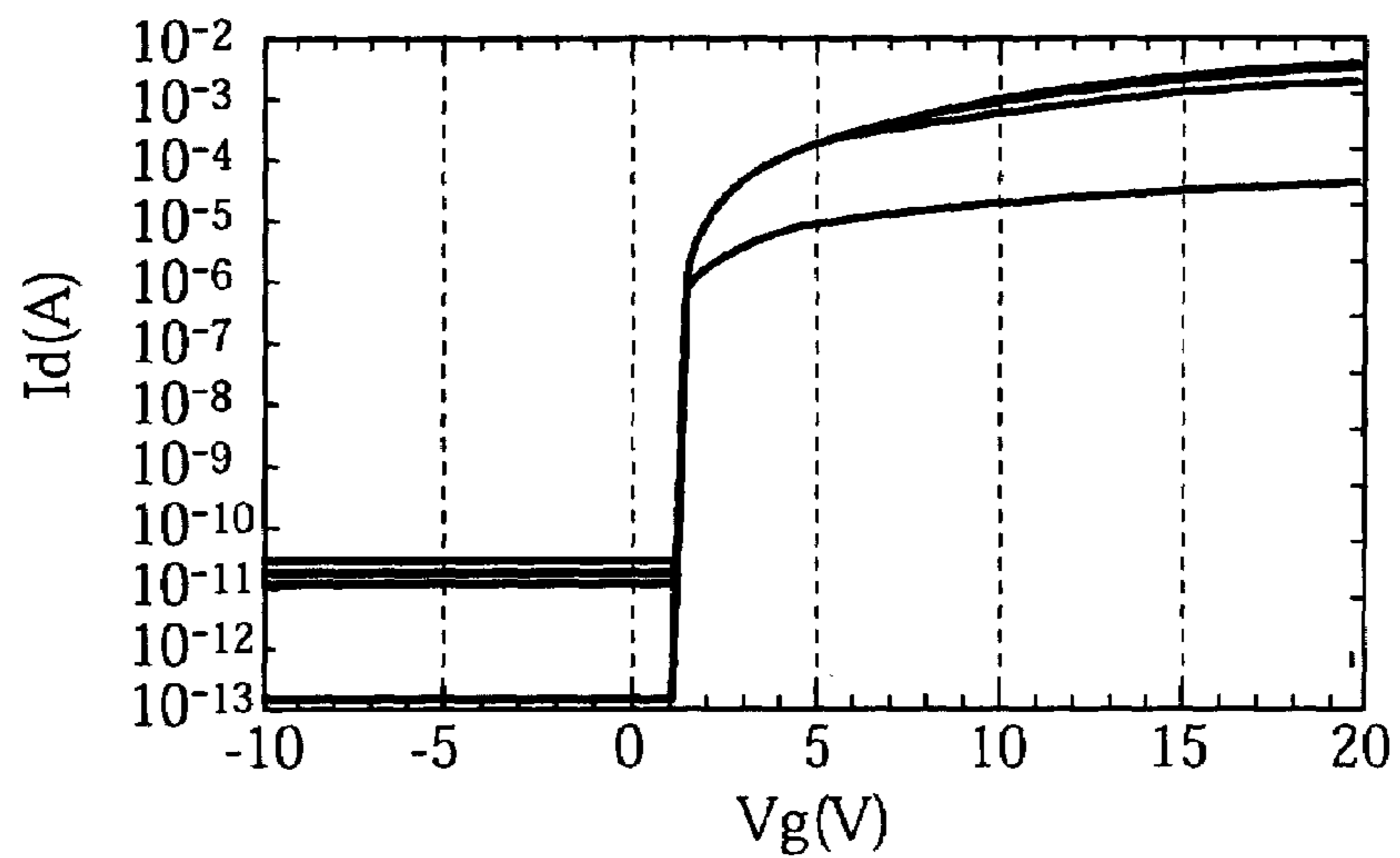
Characteristics of Mos-Tr ( Crystalline Silicon )
