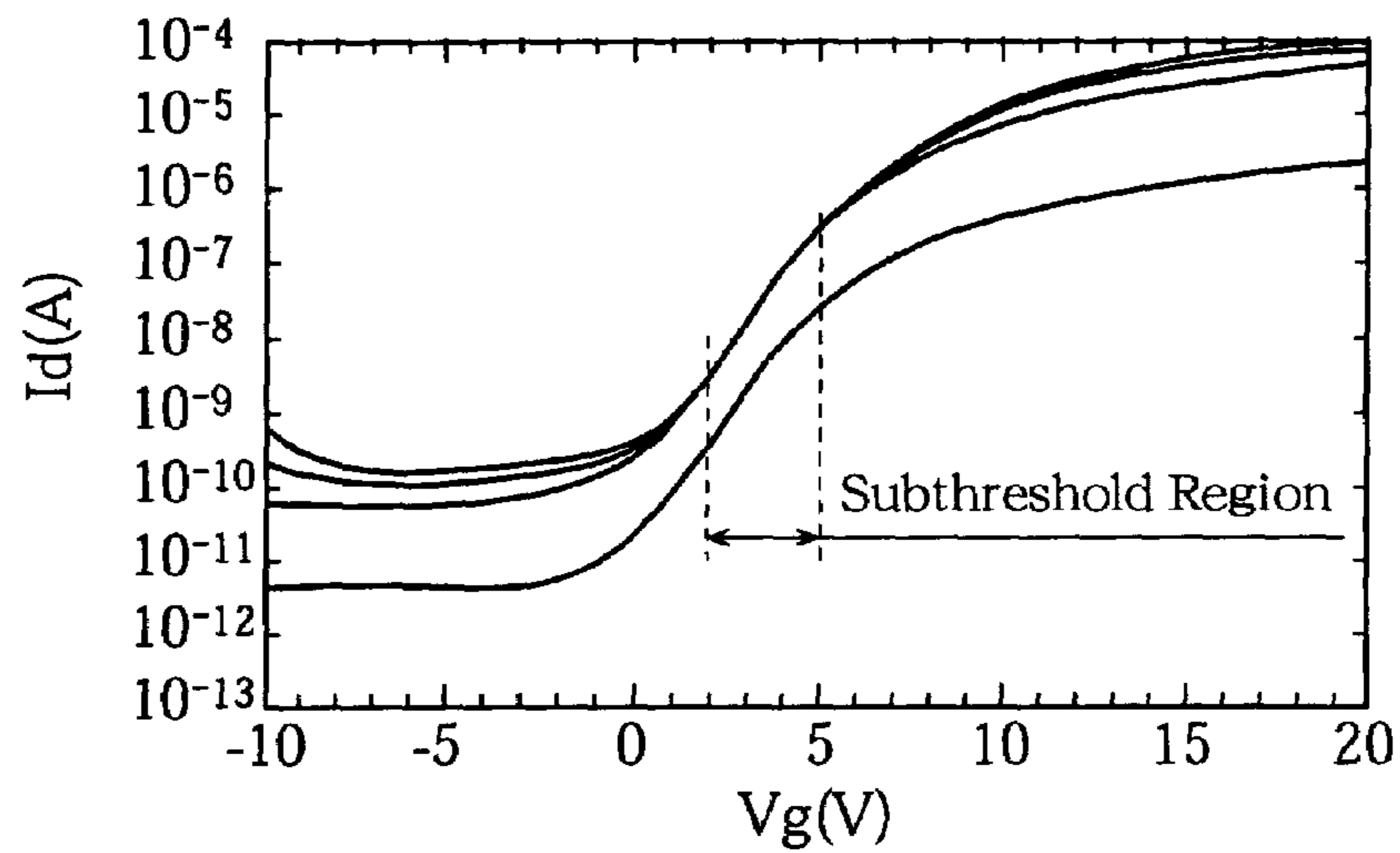
Characteristics of Polysilicon TFT
