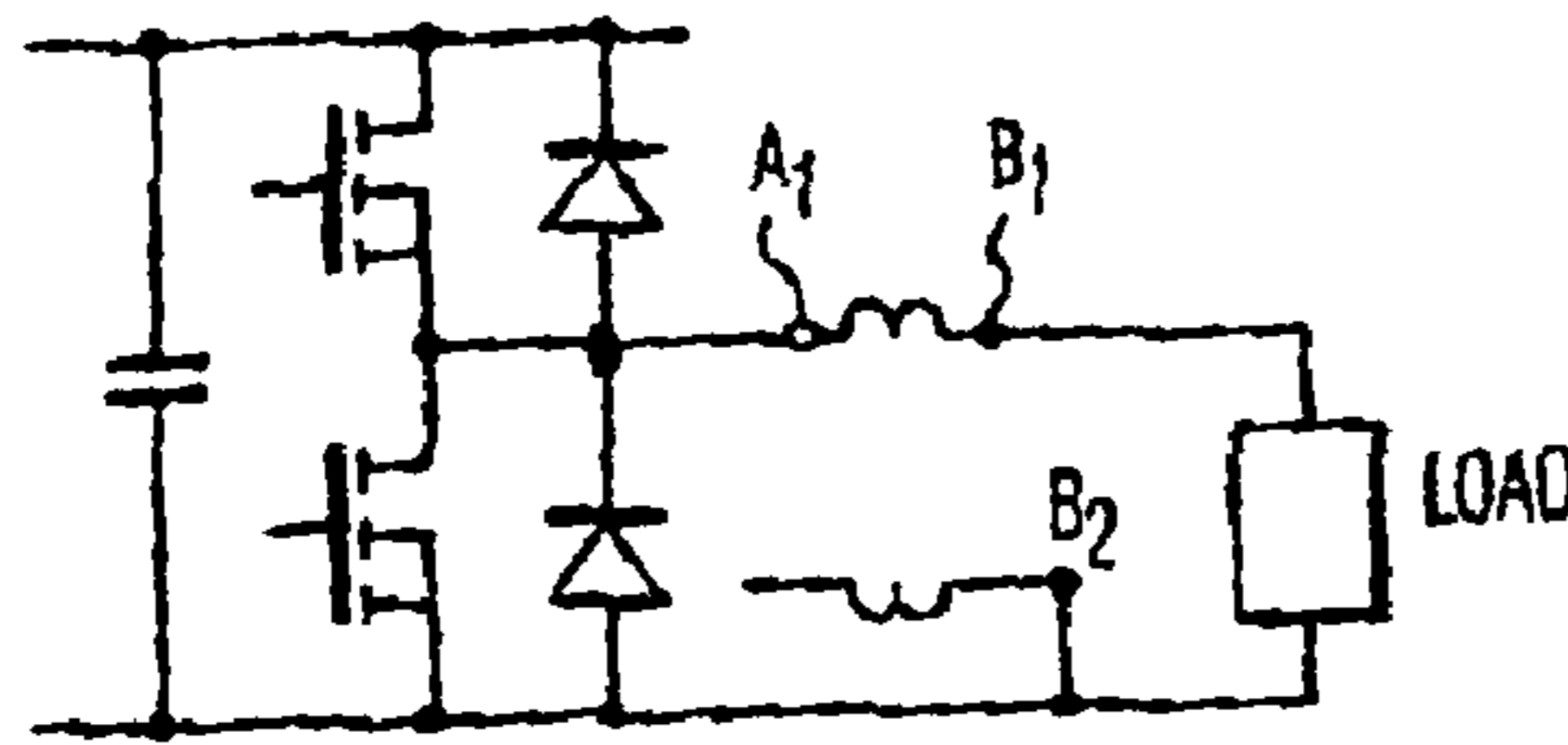
PARALLEL-LOADED RESONANT HALF BRIDGE
