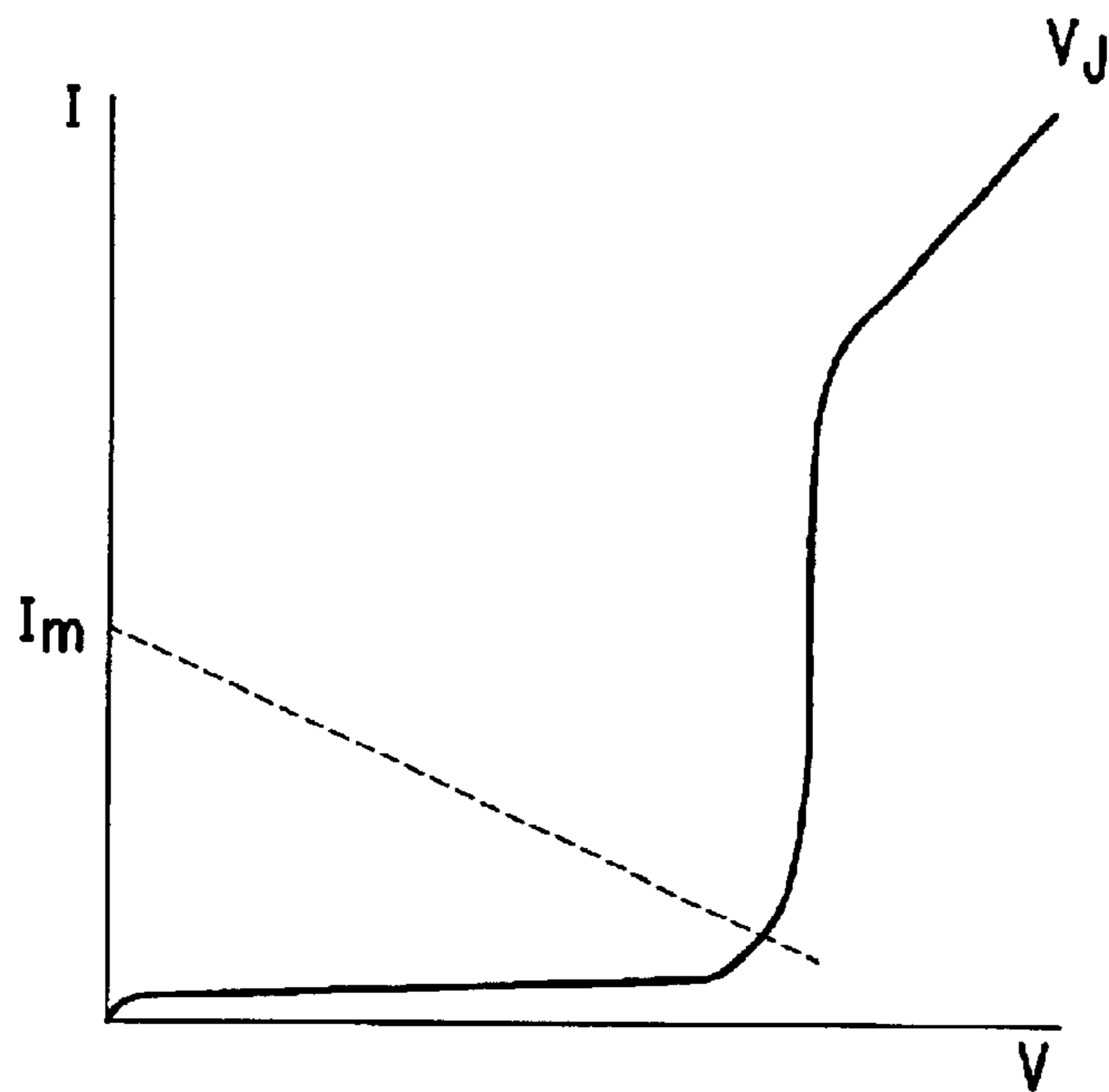
FIG. 2 PRIOR ART
