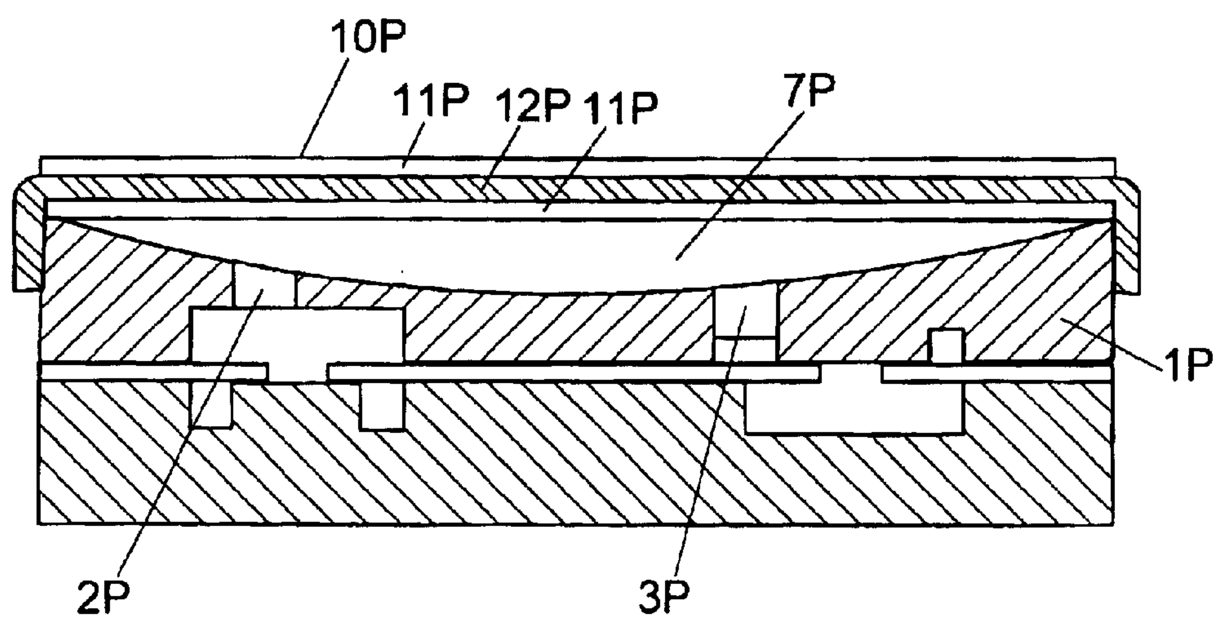
FIG. 12 (PRIOR ART)
