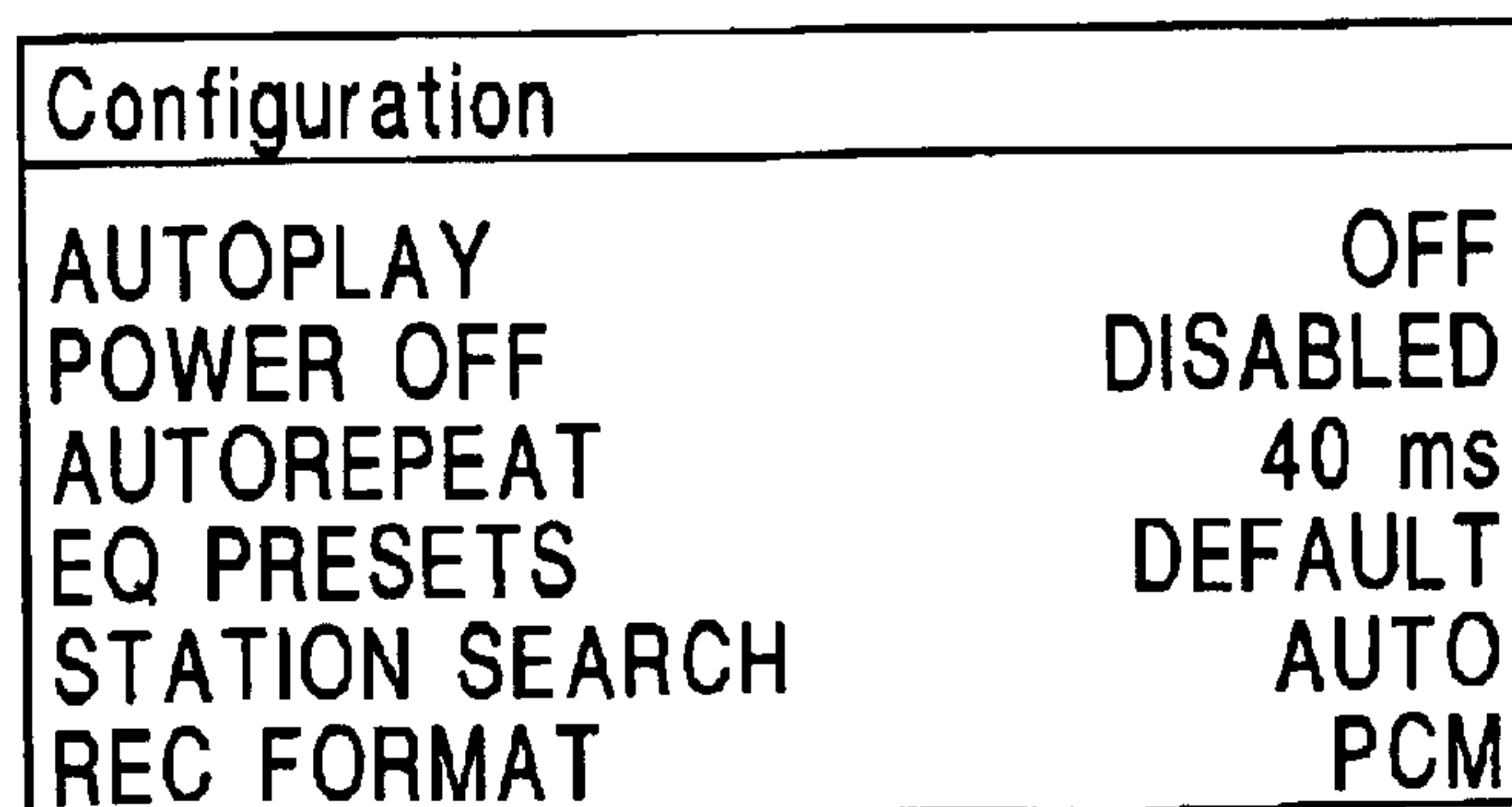
Configuration Screen
