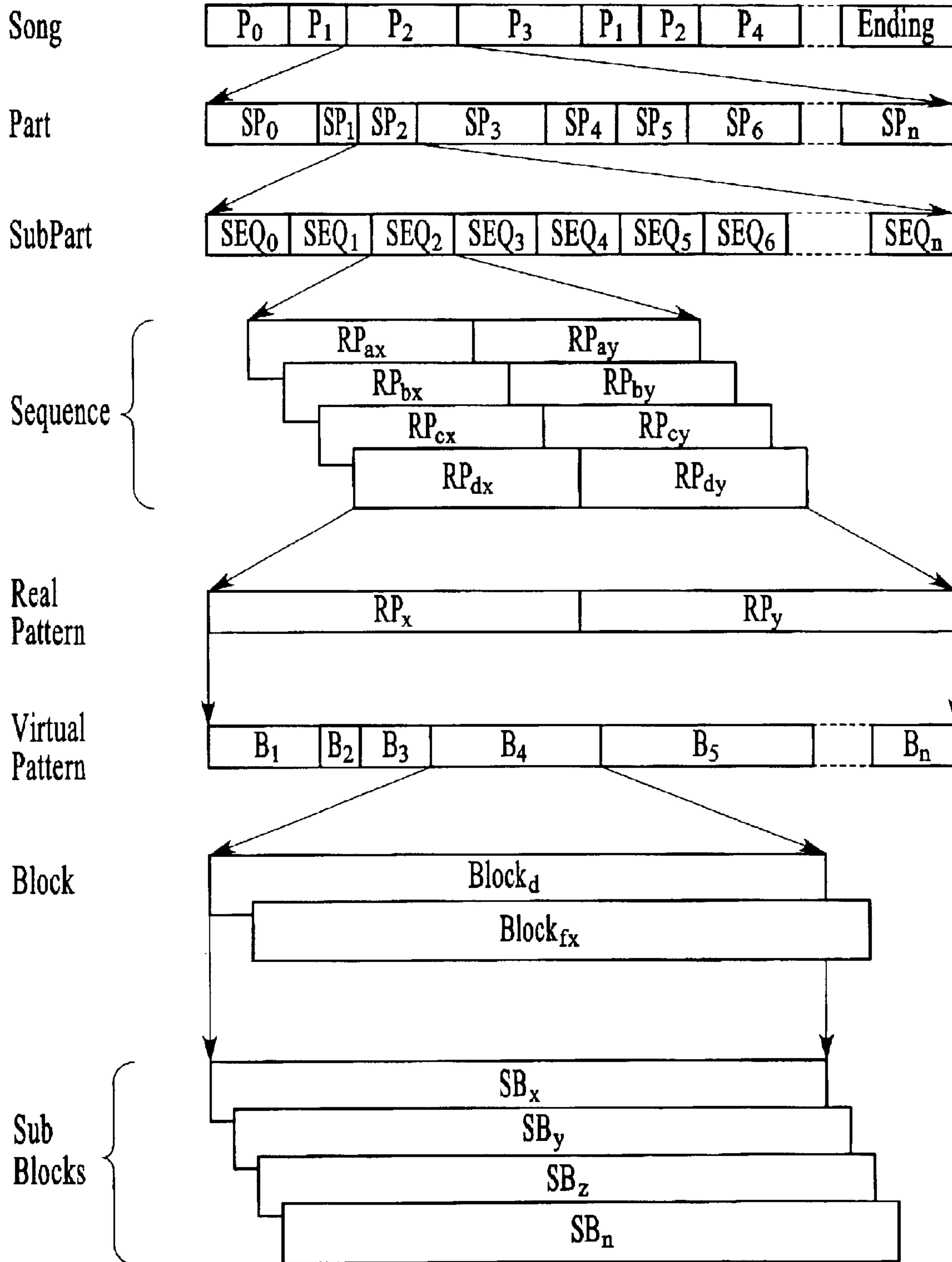
Song Structure
