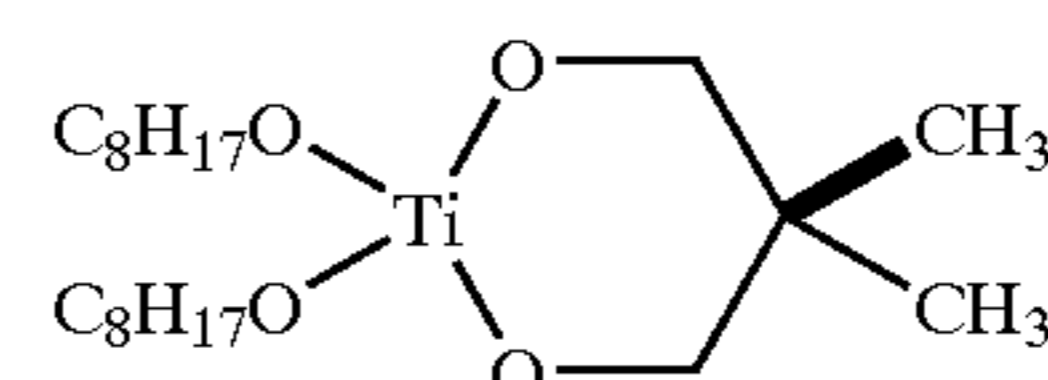
Di(2-ethyl-1-hexyl) 2,2-dimethylpropane-1,3-dioxytitanate
