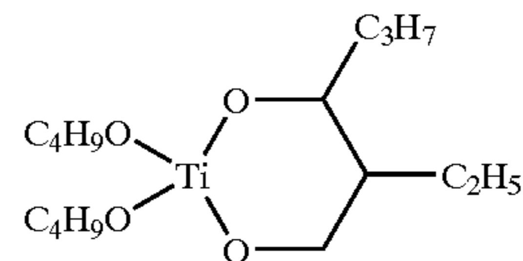
Di-1-butyl 2-ethylhexane-1,3-dioxytitanate
