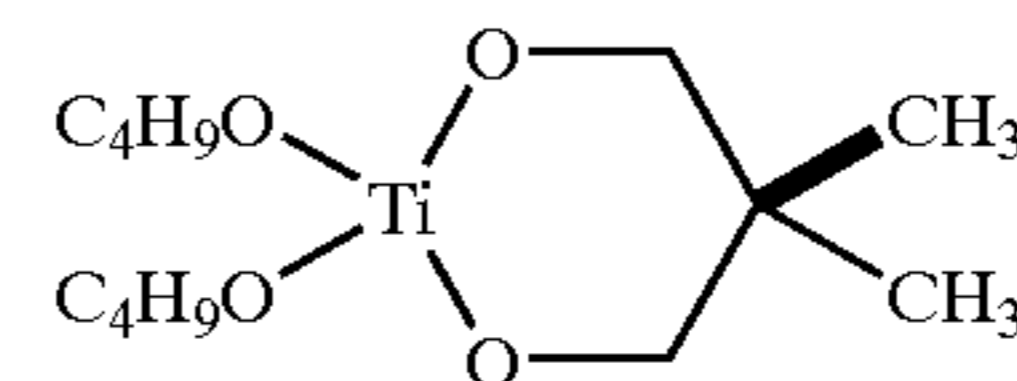
Di-1-butyl 2,2-dimethylpropane-1,3-dioxytitanate
