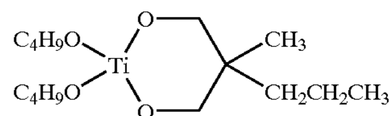
Di-1-butyl 2-(1-propyl)-2-methylpropane-1,3-dioxytitanate
