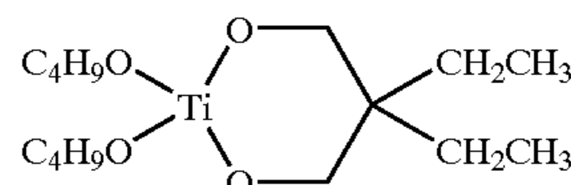
Di-1-butyl 2,2-diethylpropane-1,3-dioxytitanate
