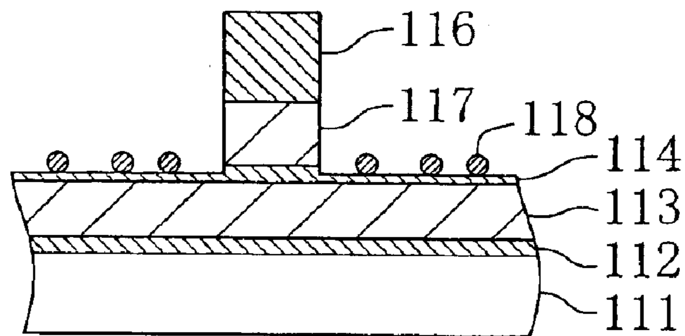
Fig. 23 (b) Prior Art
