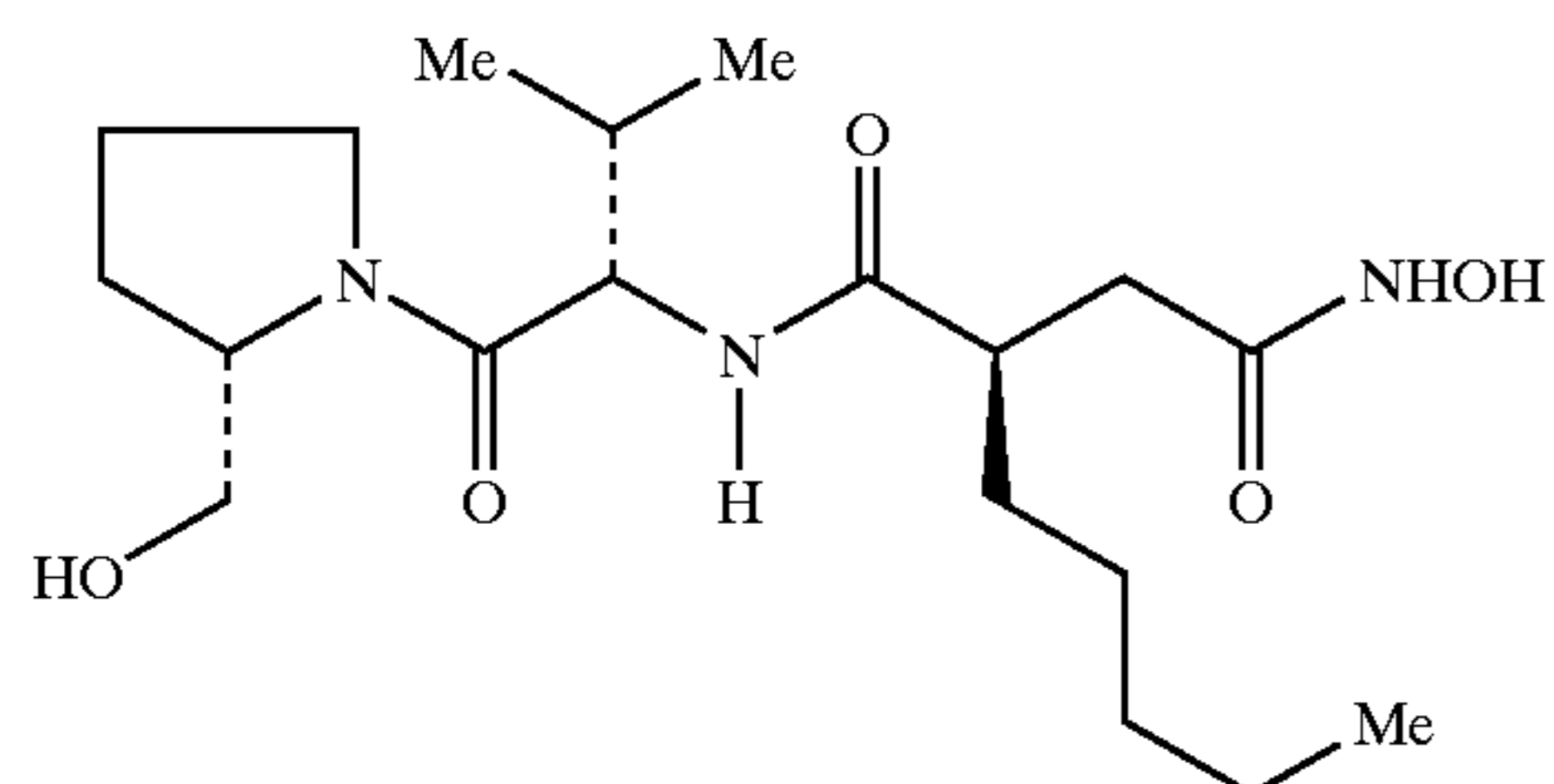
Actinonin
