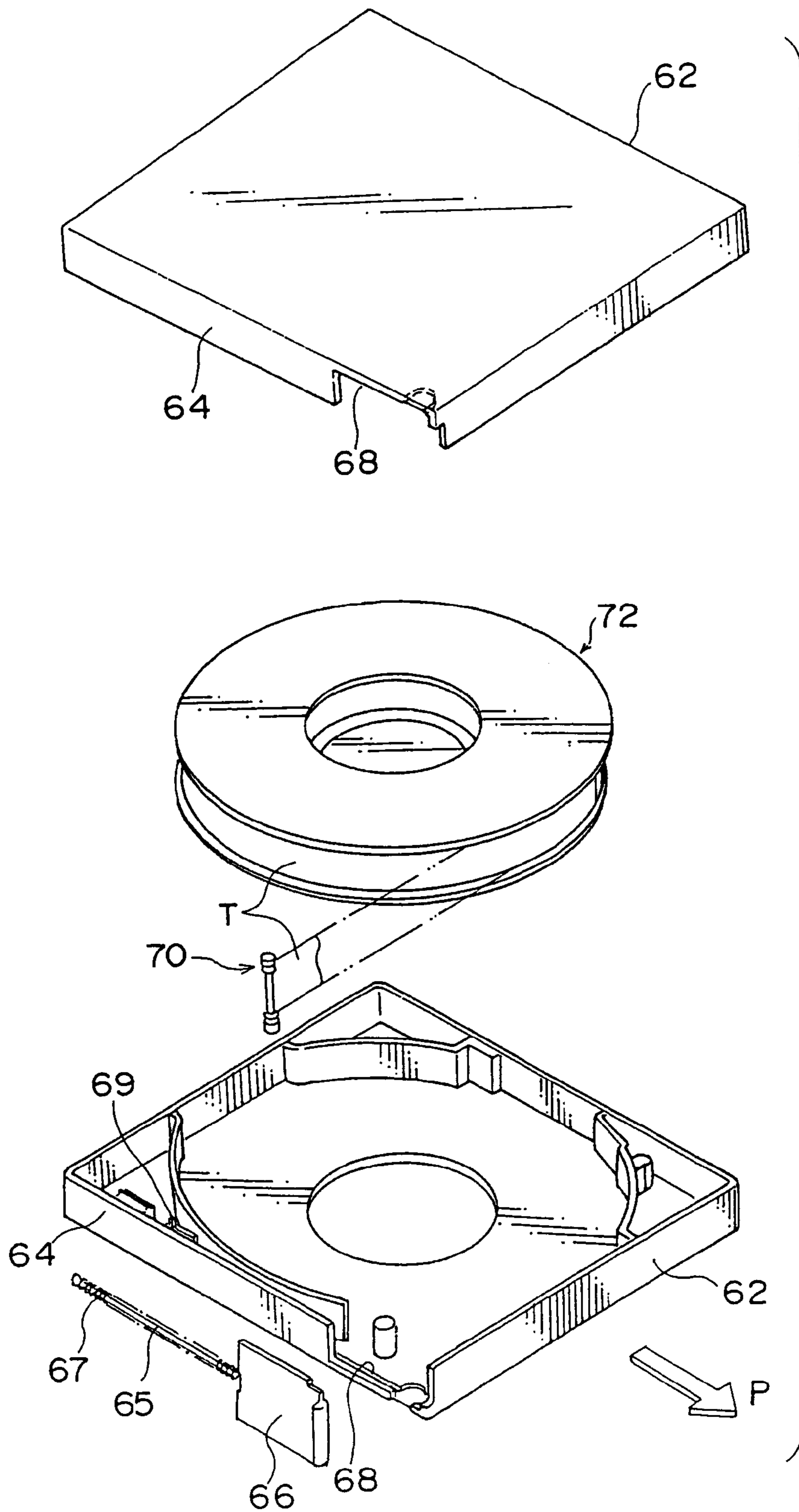
FIG. 8 PRIOR ART
