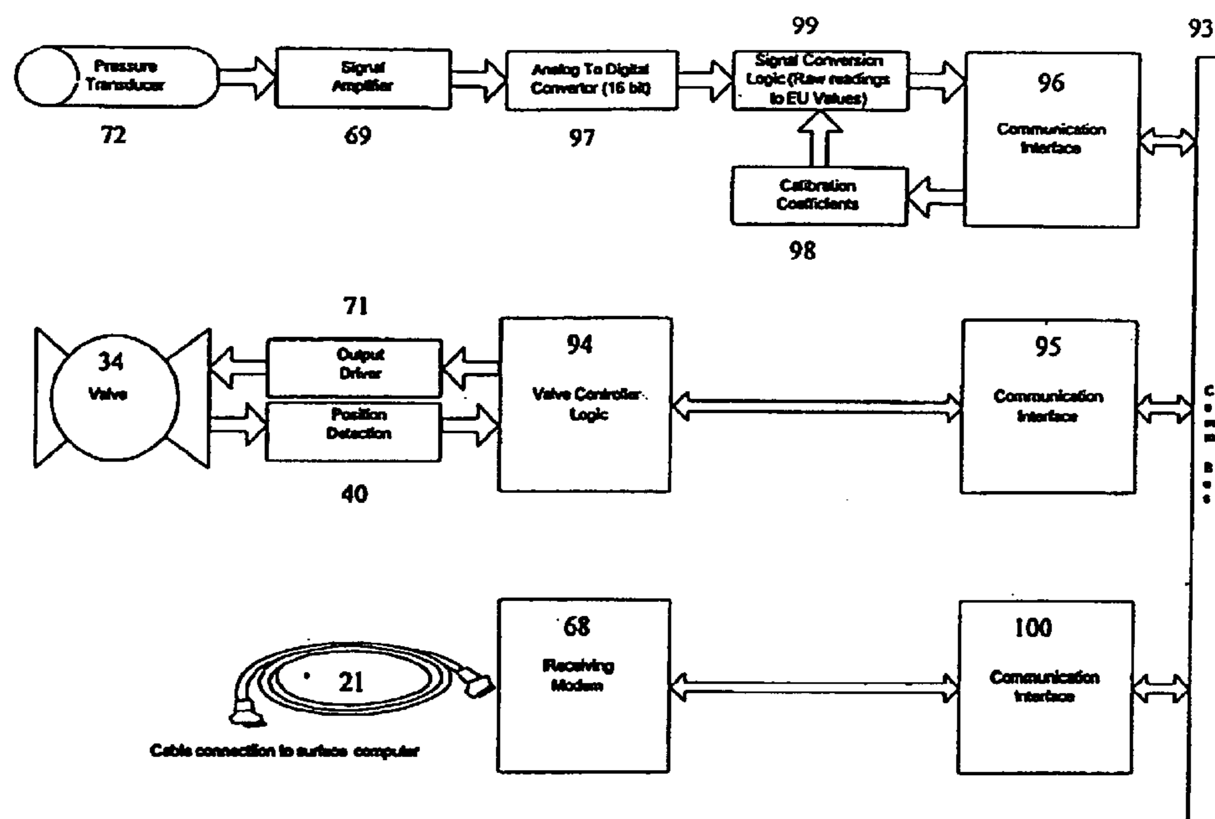
Figure 7 - Downhole Tool Software & Electronics
