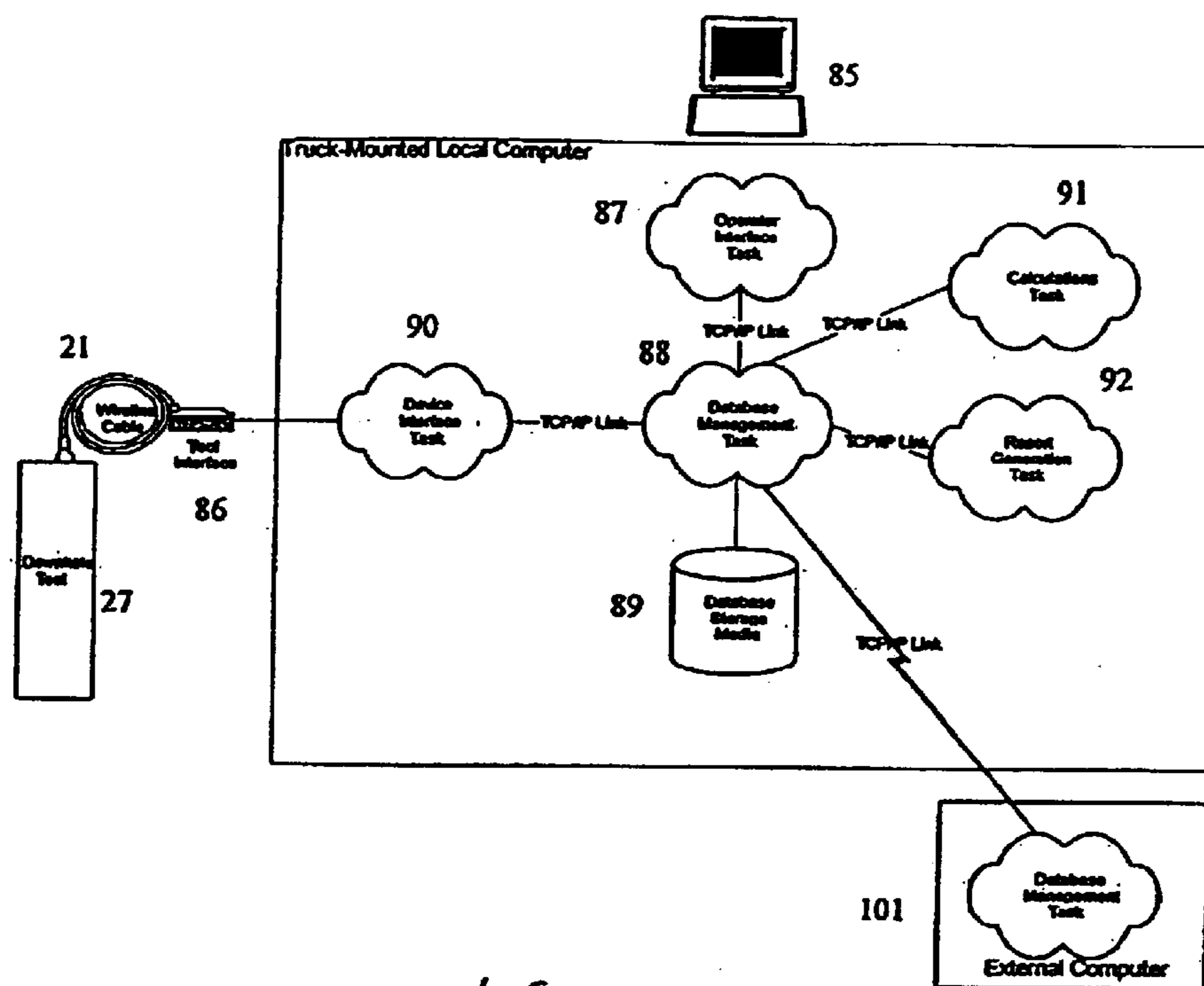
Figure 6 Software Architecture Overview
