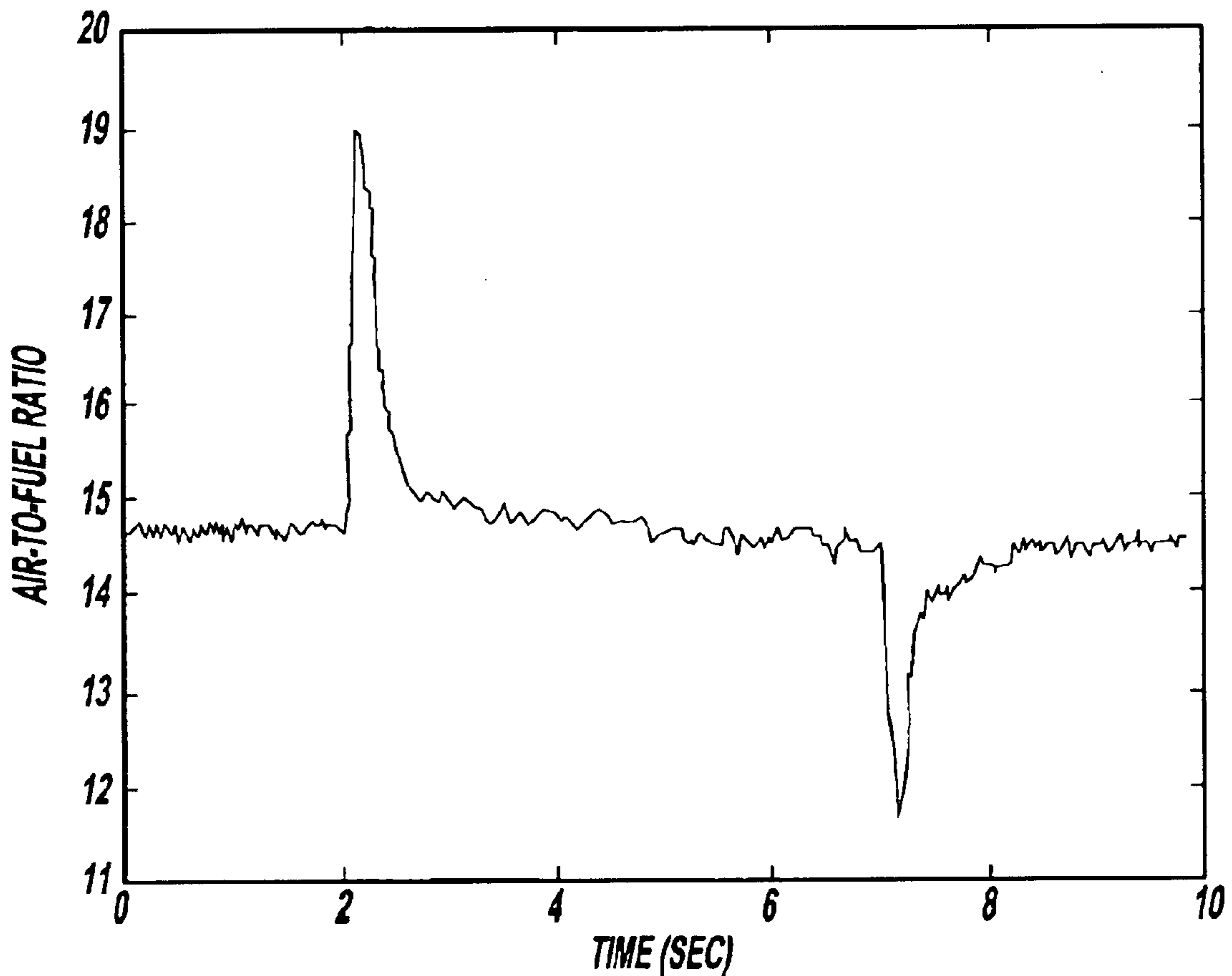
AIR-TO-FUEL RATIO DISTURBANCE IN EIVC/LIVC CHARGE DELIVERY MODE TRANSITIONS, CONDITIONS: CONSTANT INJECTOR PW, SAME STEADY-STATE AIRFLOW BEFORE AND AFTER TRANSITIONS.
