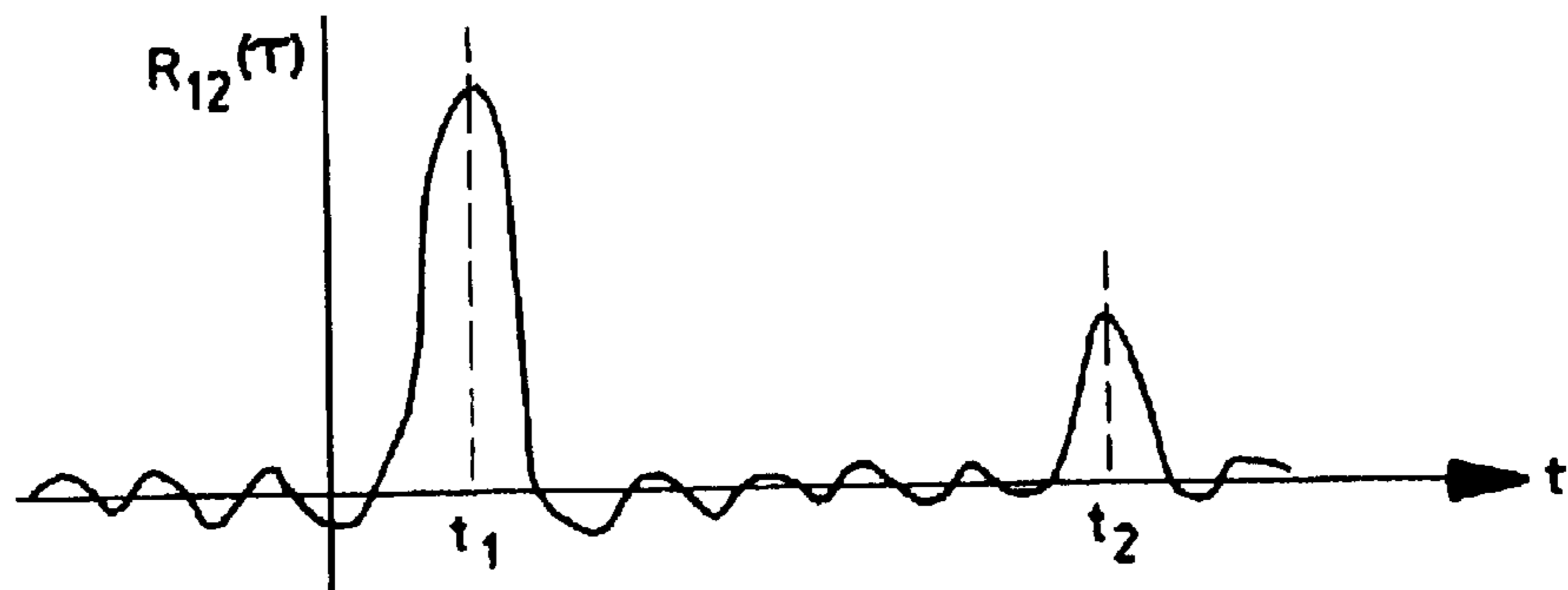
TYPICAL CROSS-CORRELATION FUNCTION
