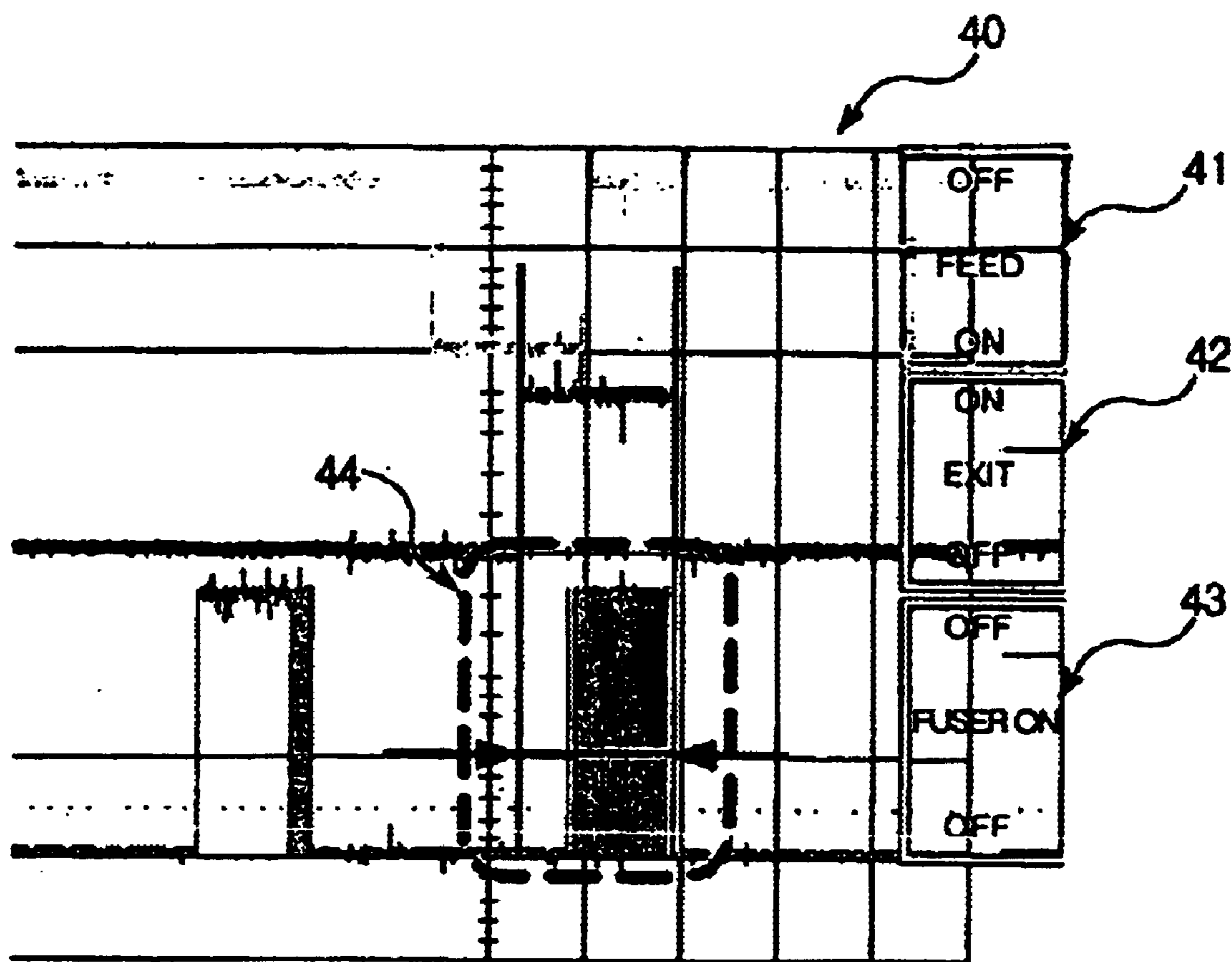
< FUSER ON WAVE FORM AT NORMAL PRINTING OPERATION >
