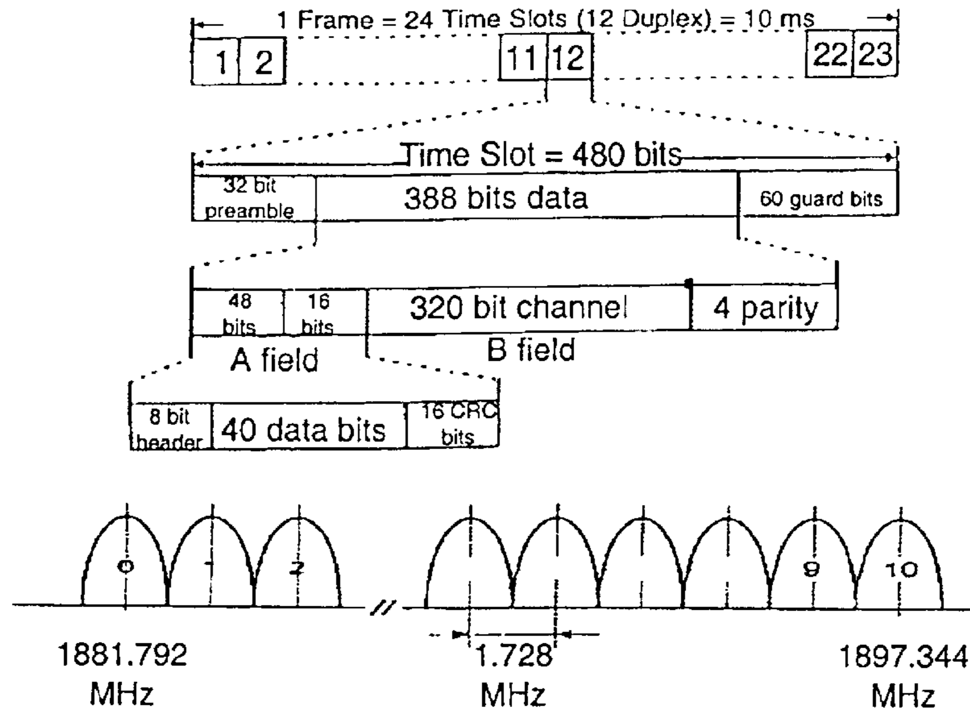
Fig. 1 (Prior Art)
