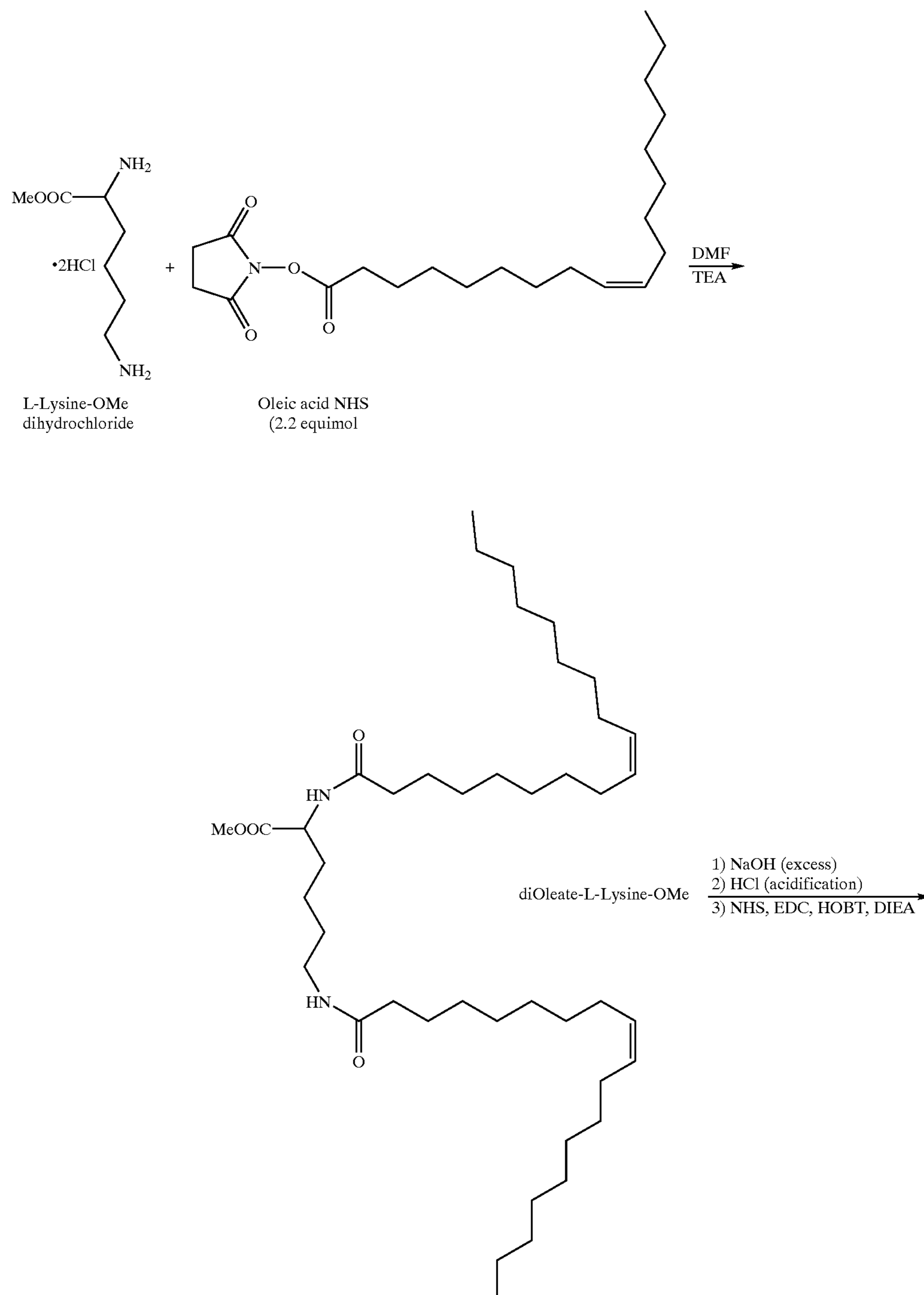
Scheme 6: Synthesis of diOleate-L-Lysine-NHS.
