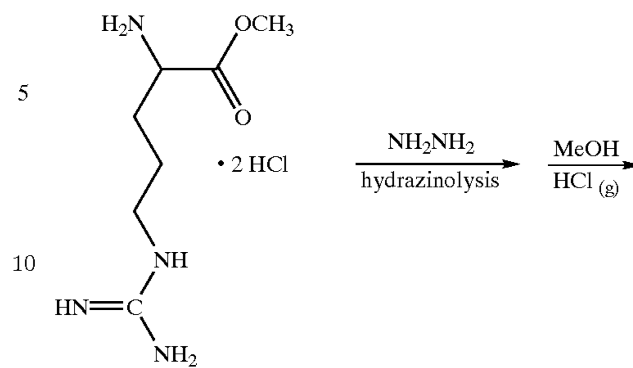
L-Arginine-O-methyl ester dihydrochloride
