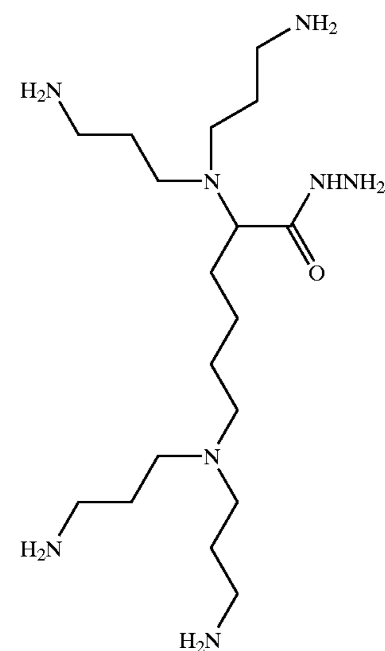
N^{\alpha}, N^{\epsilon} -tetra (3-amino propyl)-L-Lysine-hydrazide
