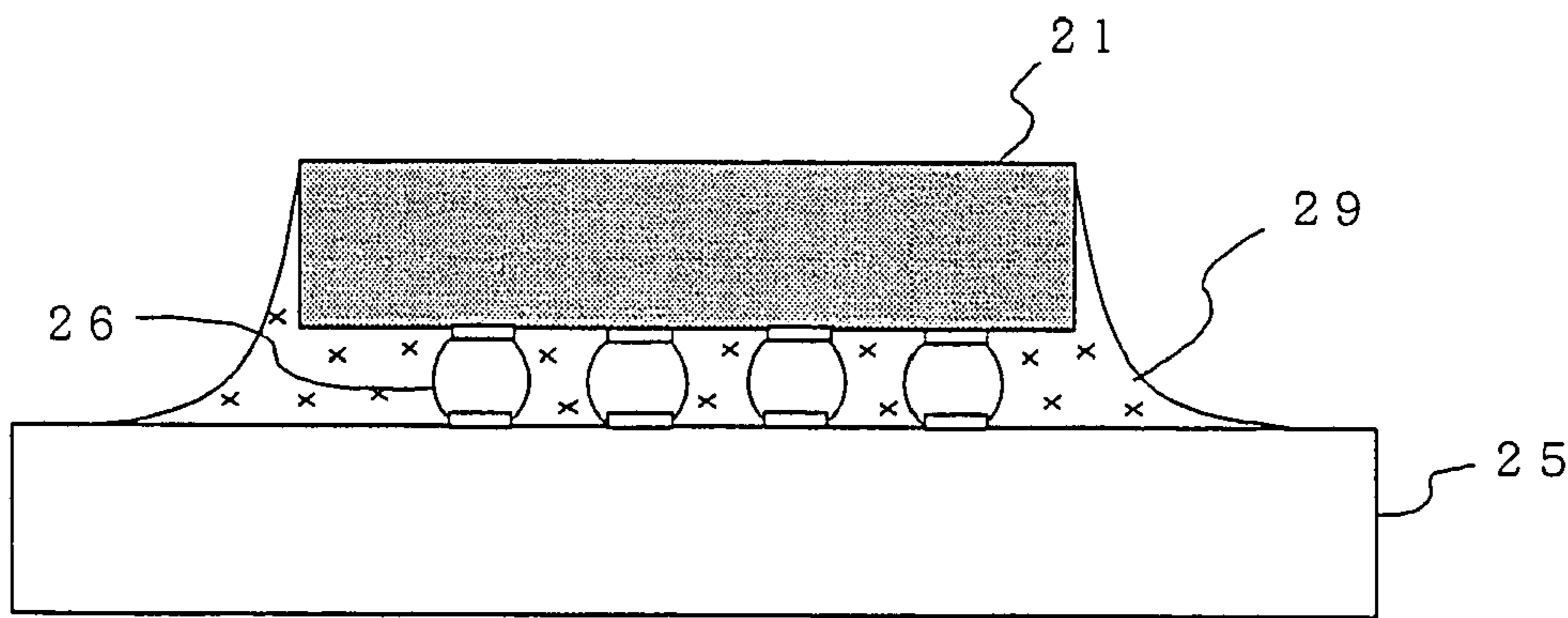
PRIOR ART Fig. 7
