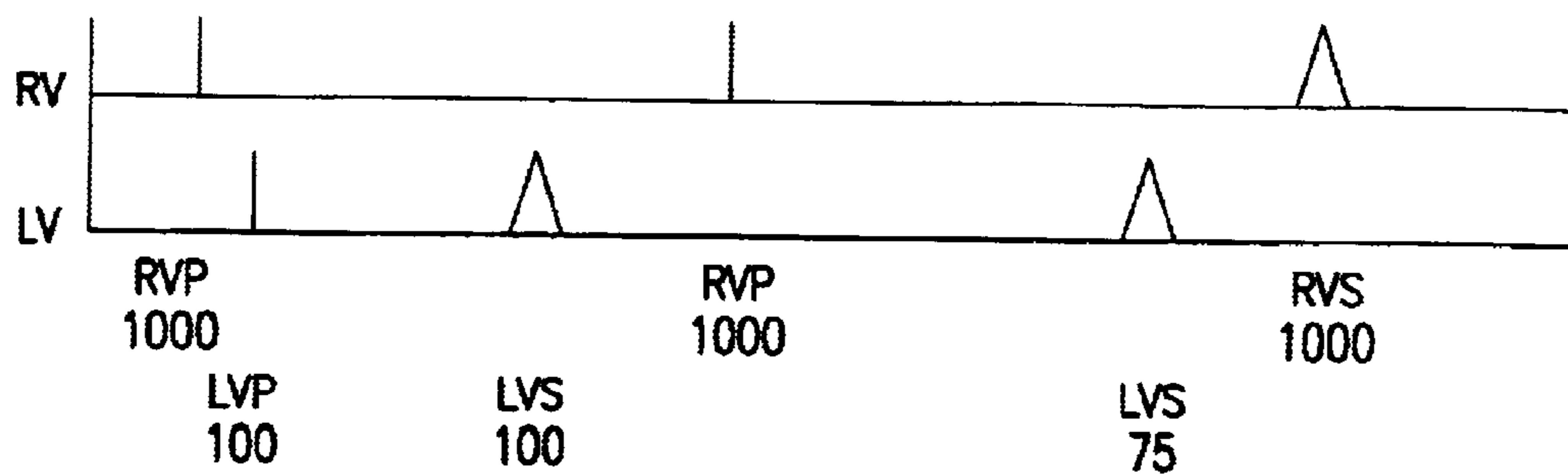
FIG. 2D
