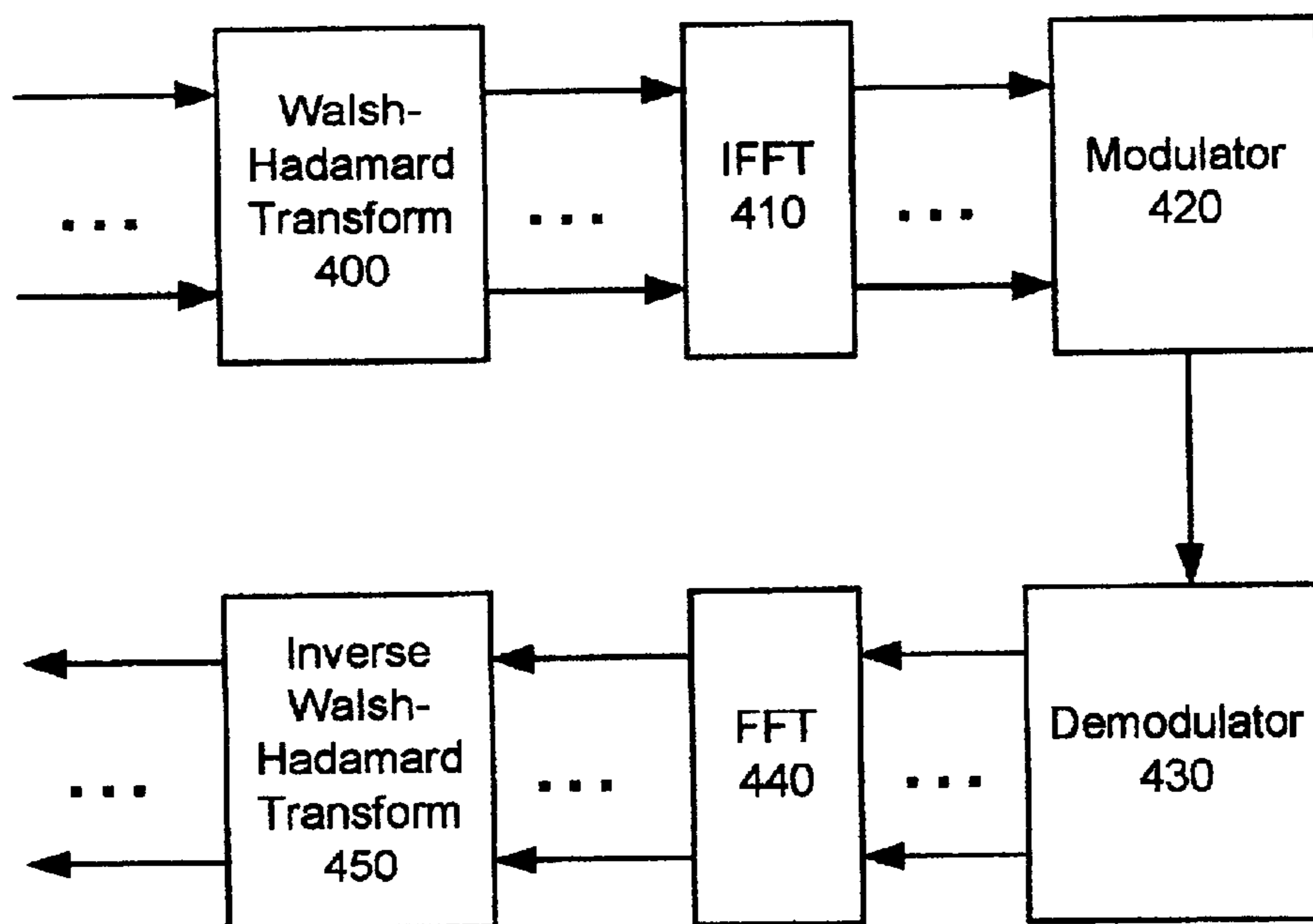
Fig. 2C Prior Art
