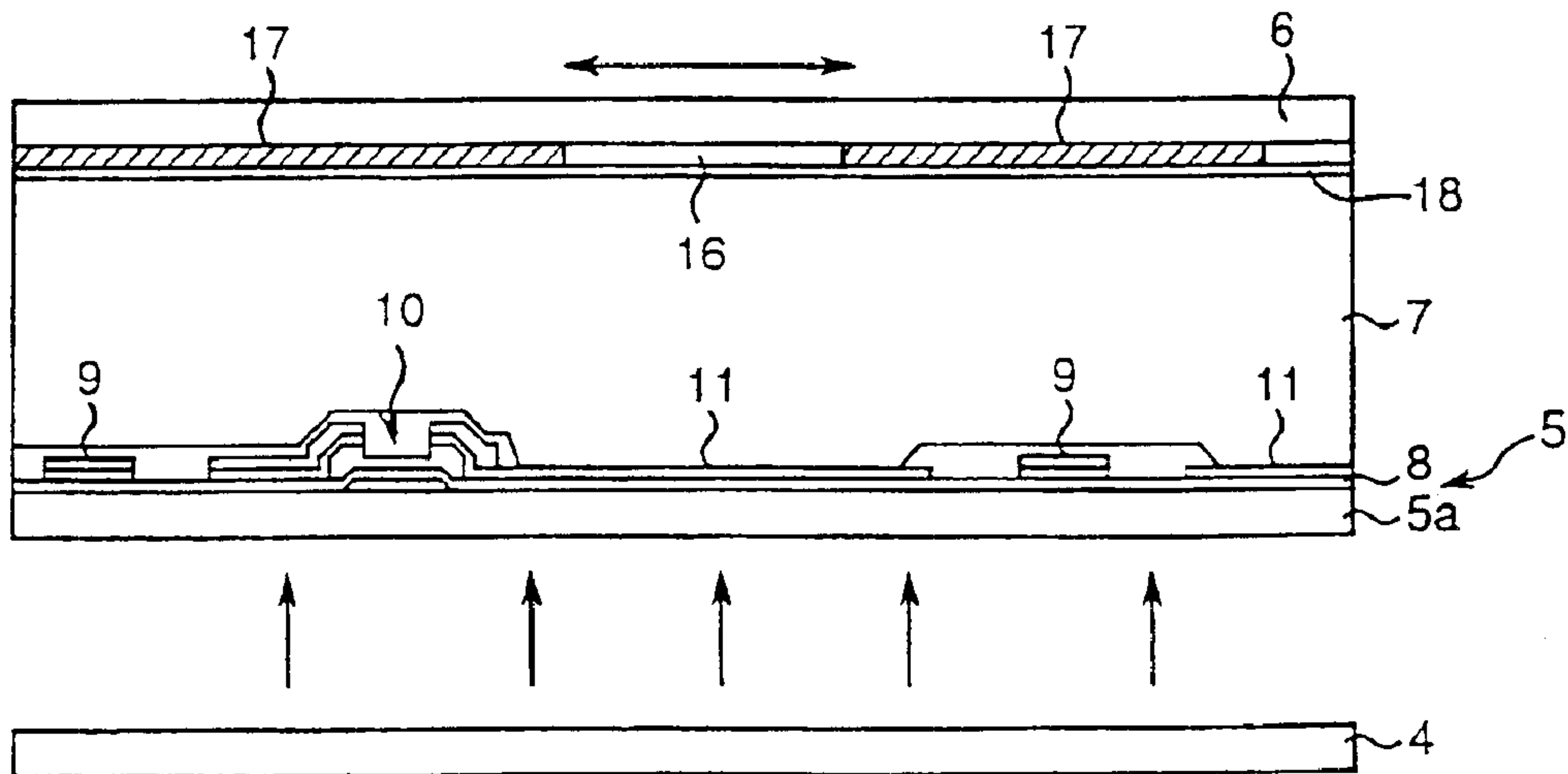
Fig.25 PRIOR ART
