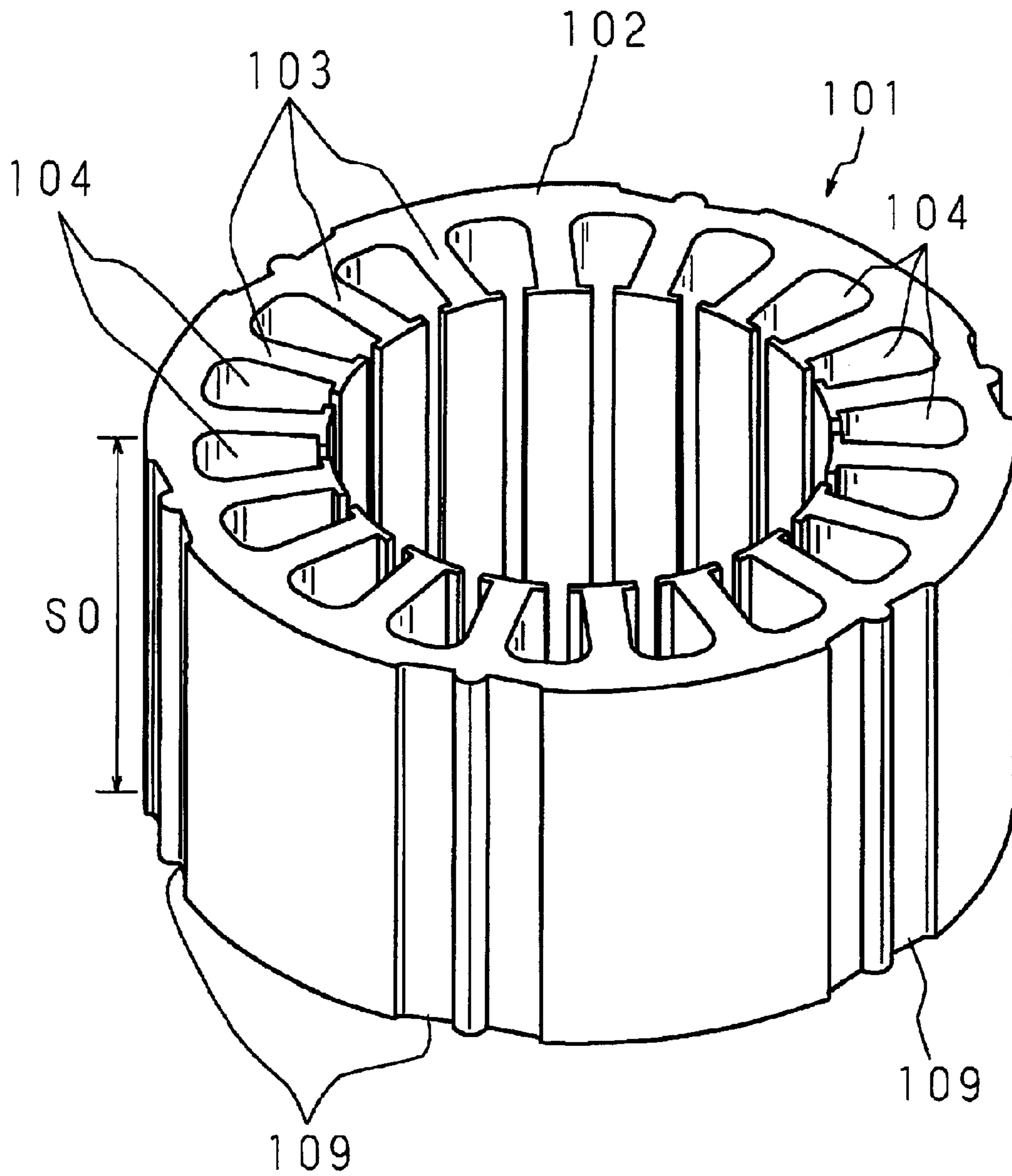
FIG. 7 PRIOR ART
