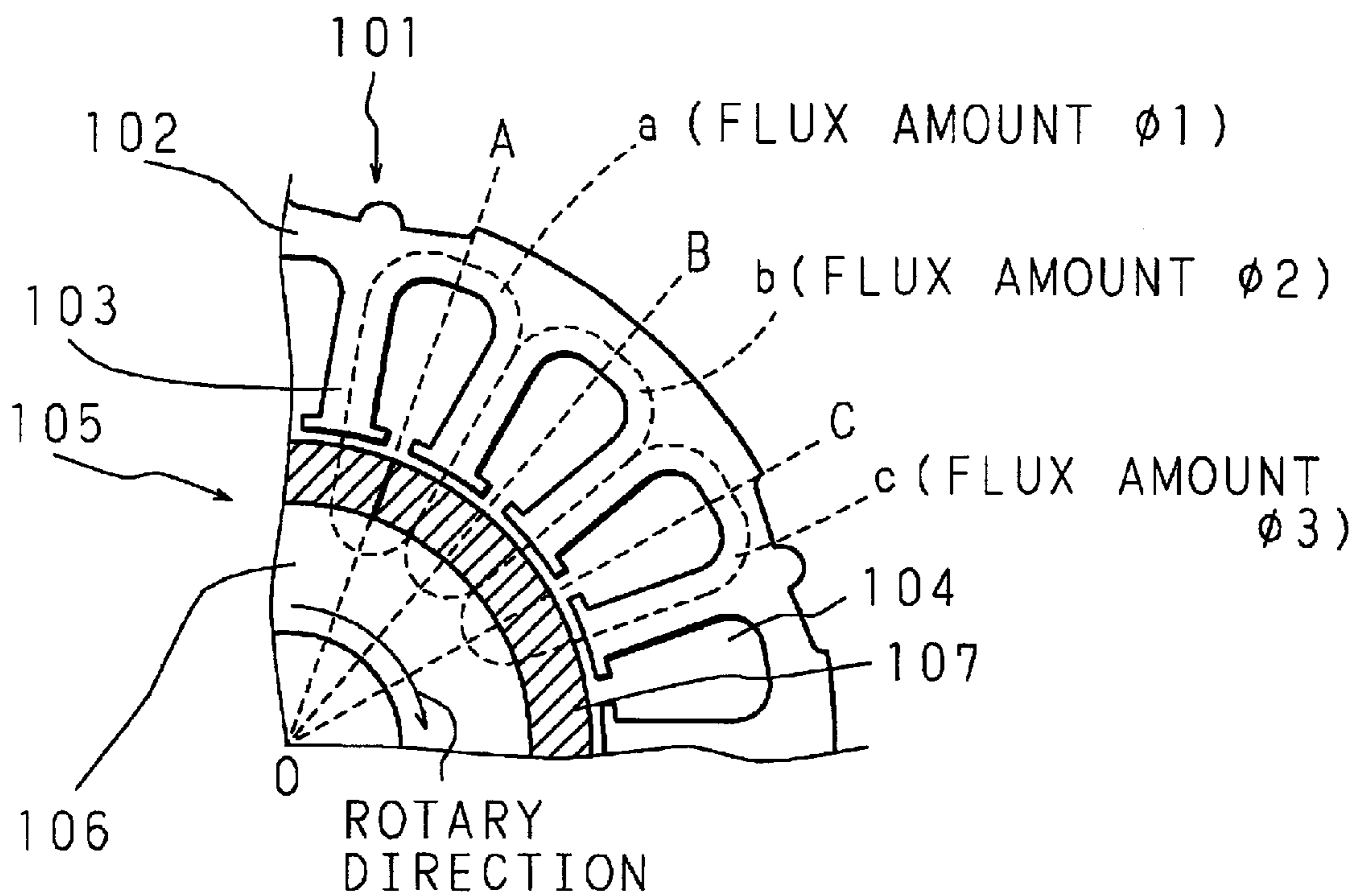
FIG. 8 PRIOR ART
