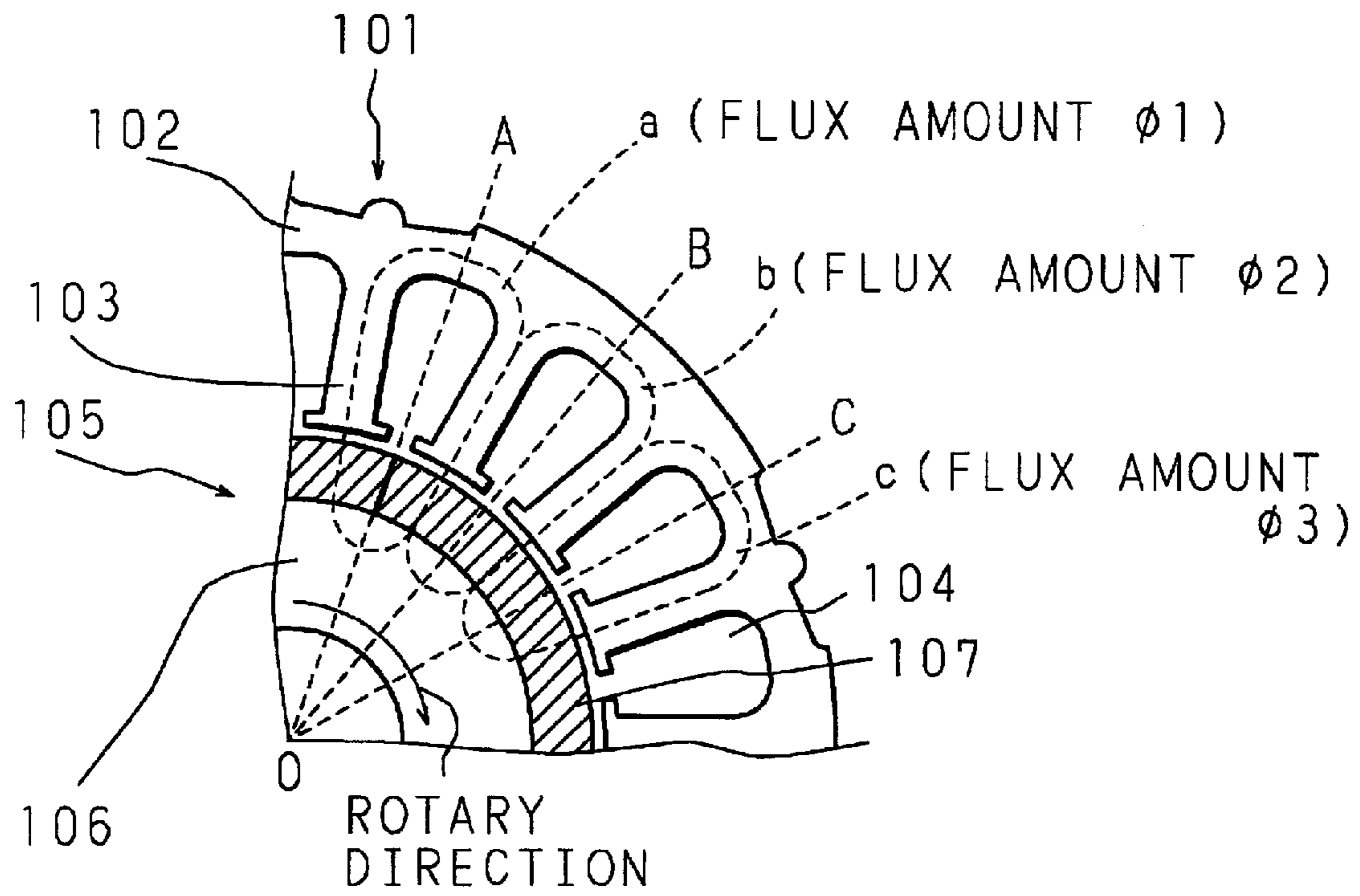
FIG. 8 PRIOR ART
