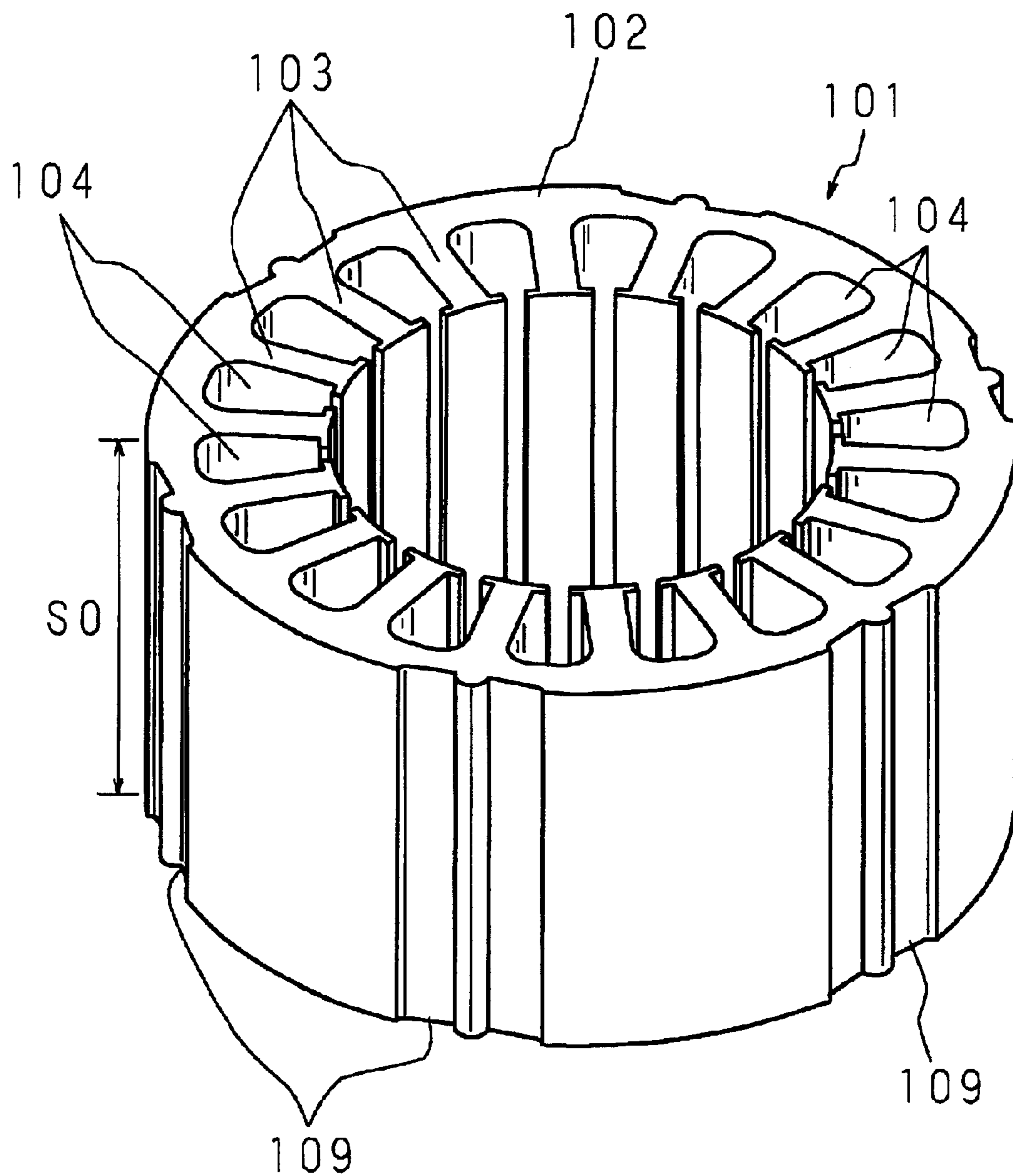
FIG. 7 PRIOR ART
