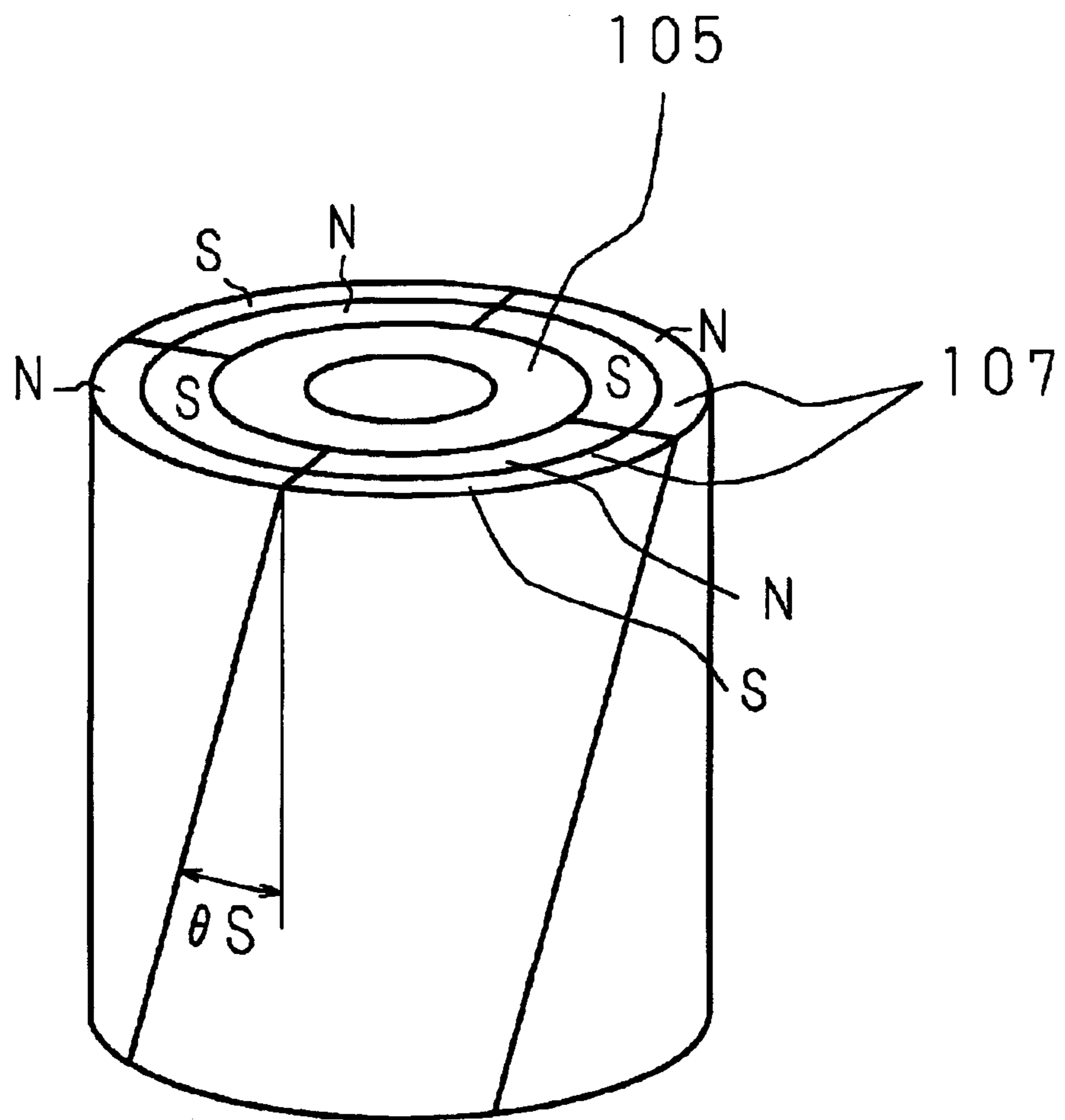
FIG. 6 PRIOR ART
