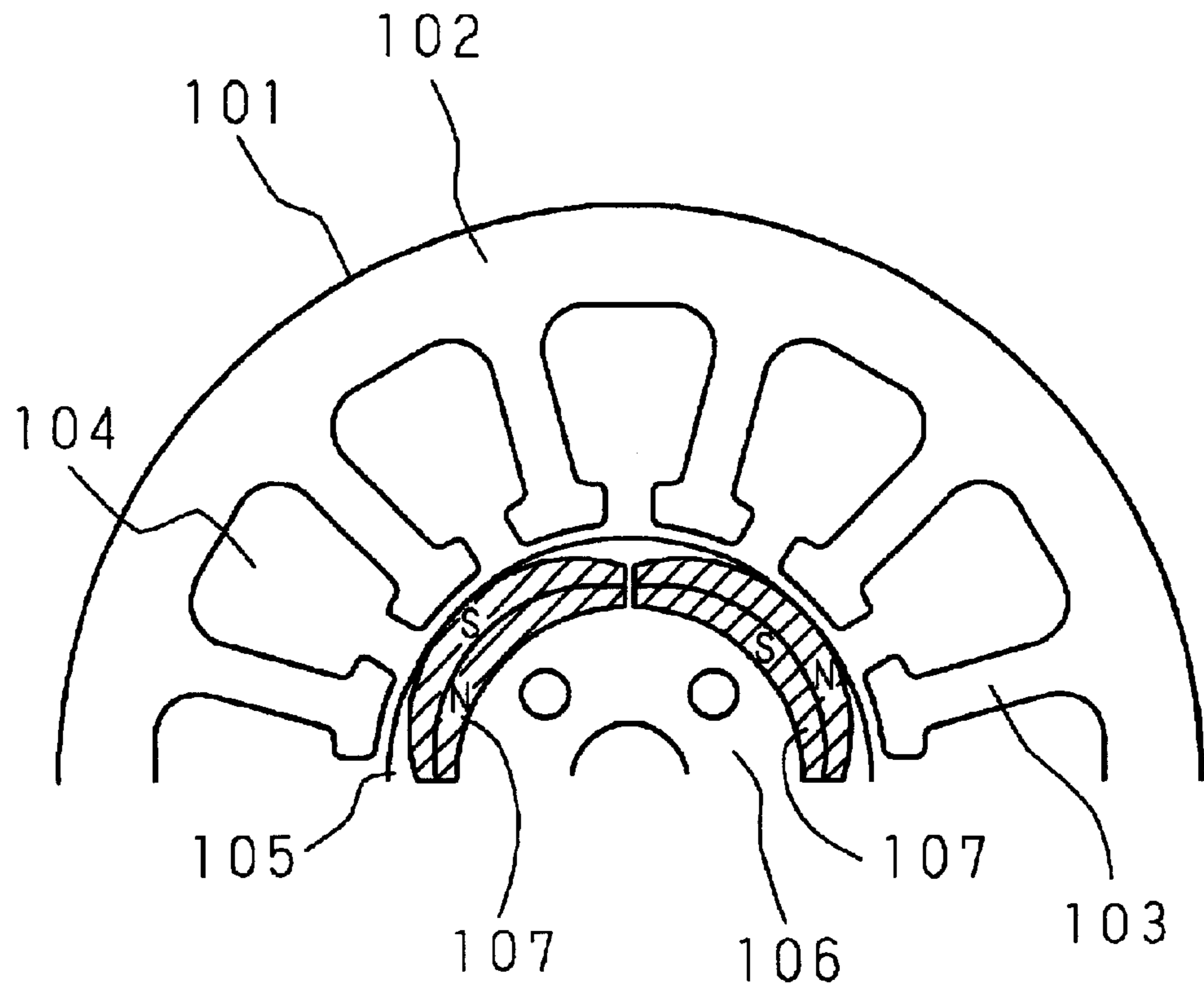
FIG. 5 PRIOR ART
