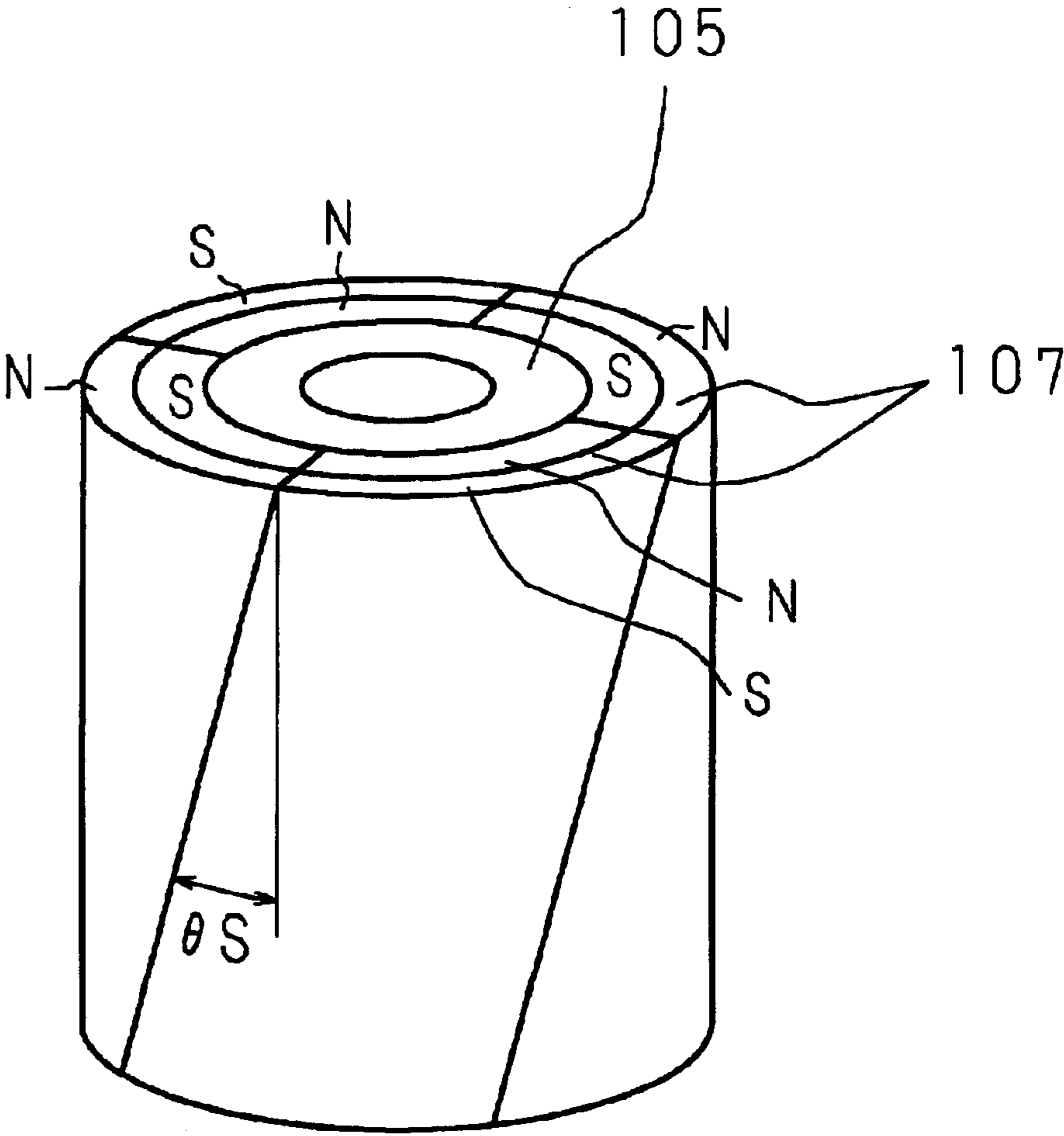
FIG. 6 PRIOR ART
