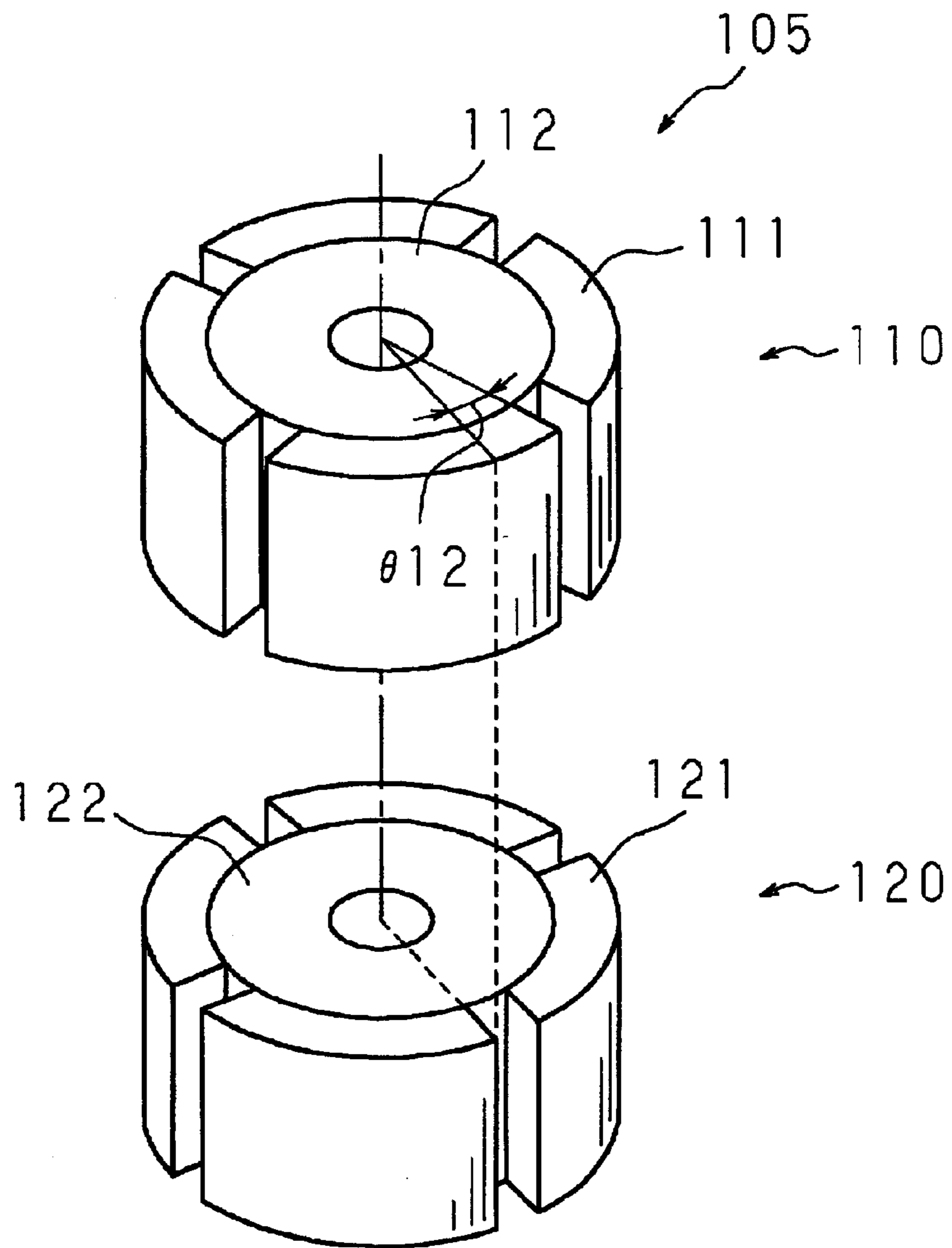
FIG. 1 PRIOR ART
