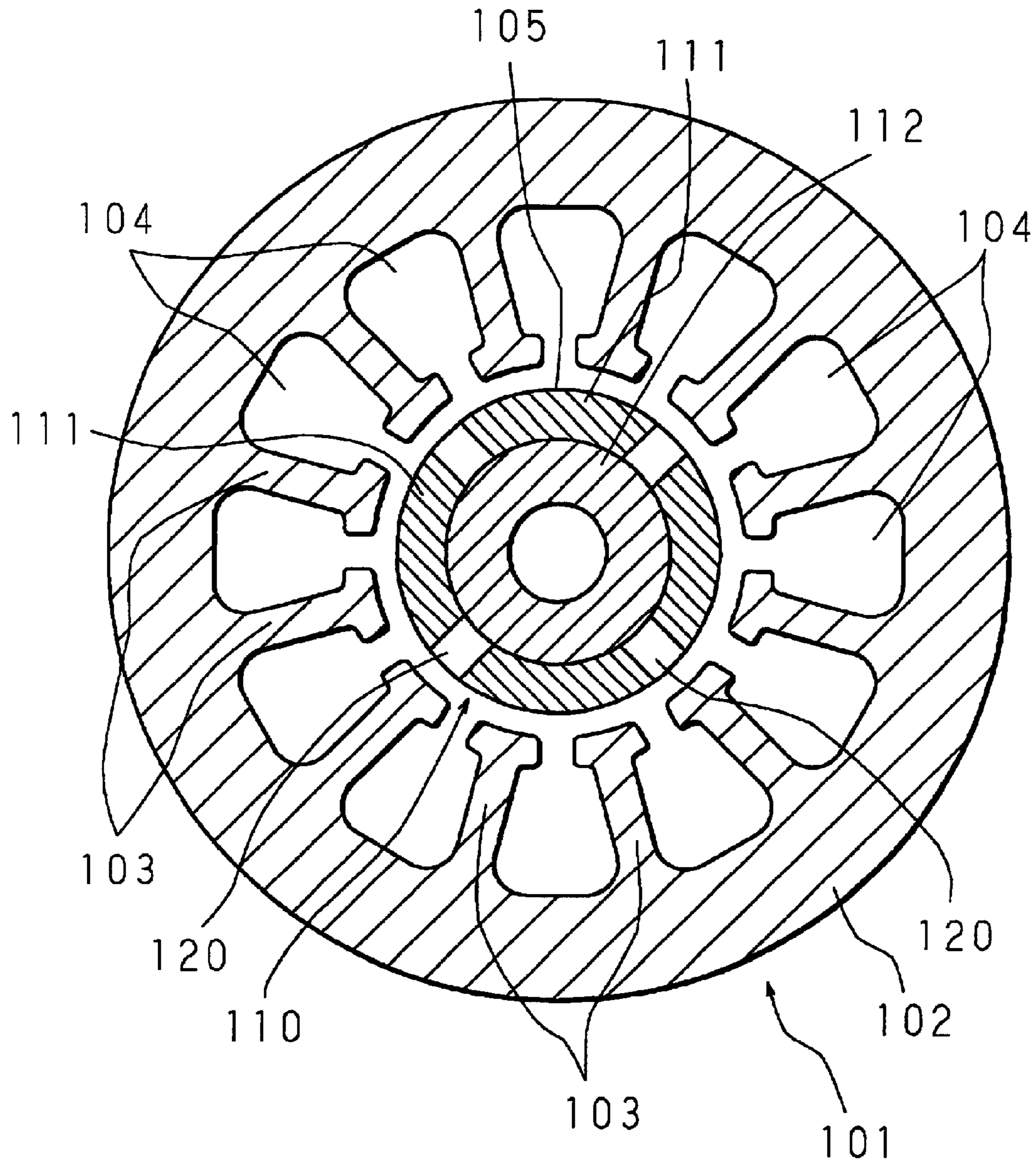
FIG. 2 PRIOR ART
