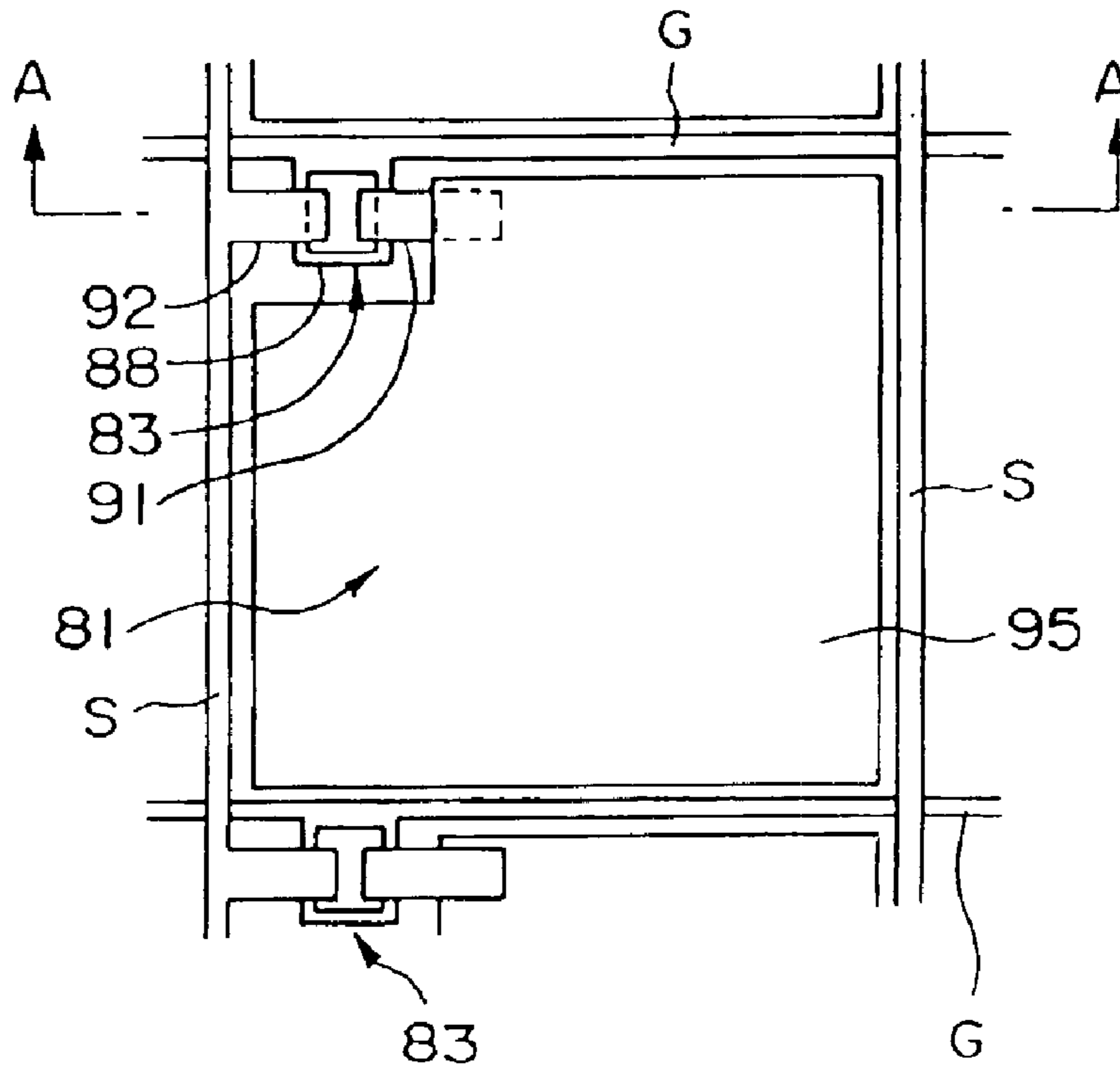
FIG. 33 PRIOR ART
