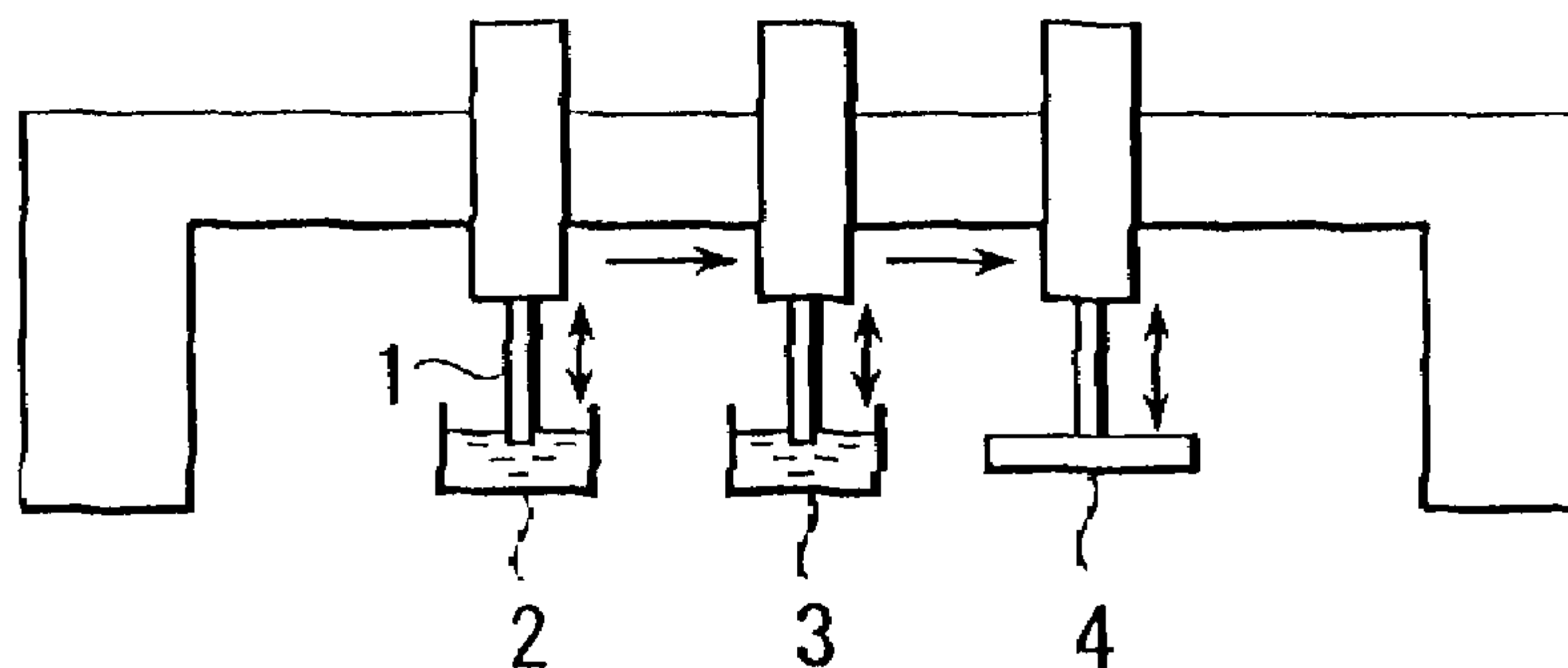
FIG. 1 PRIOR ART
