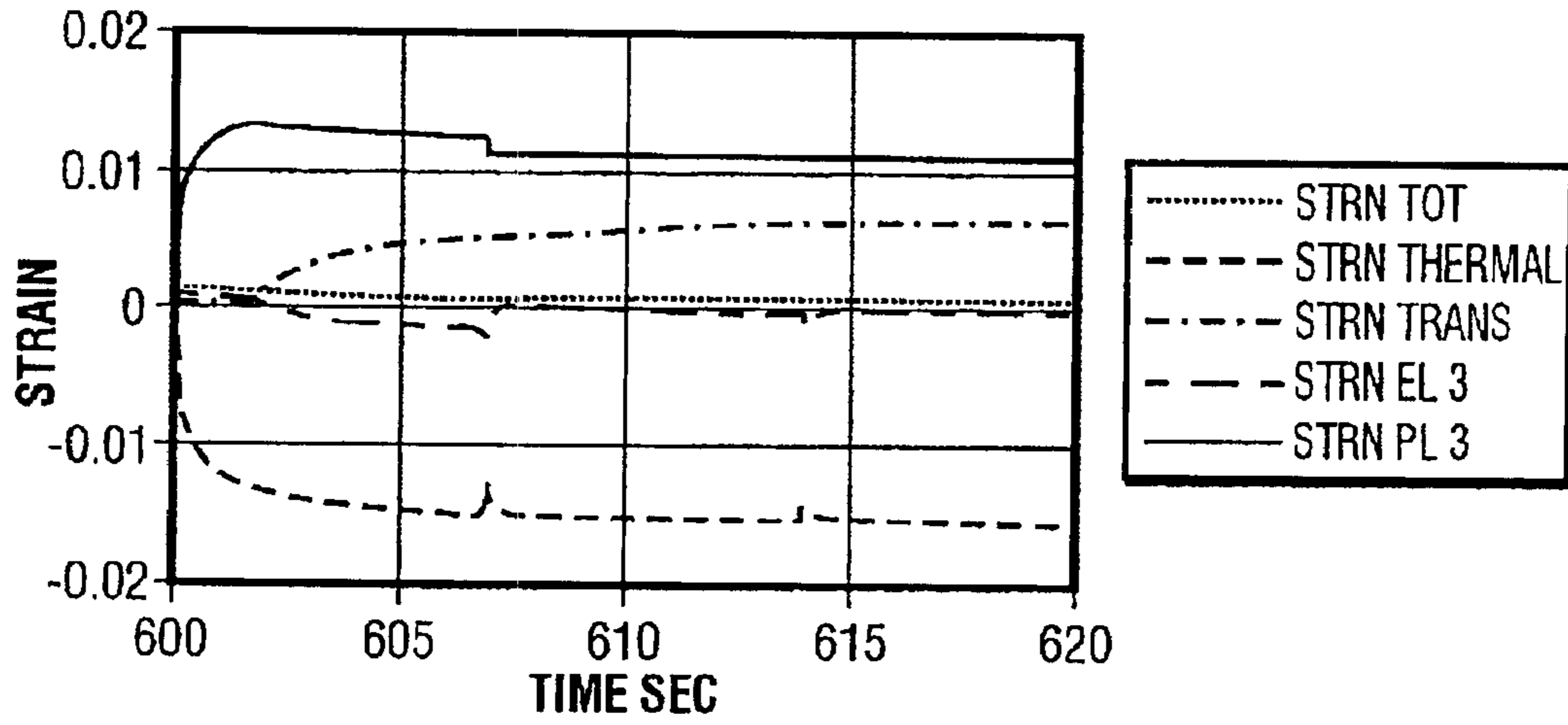
In-Plane Strains, Position #1 FIG. 15
