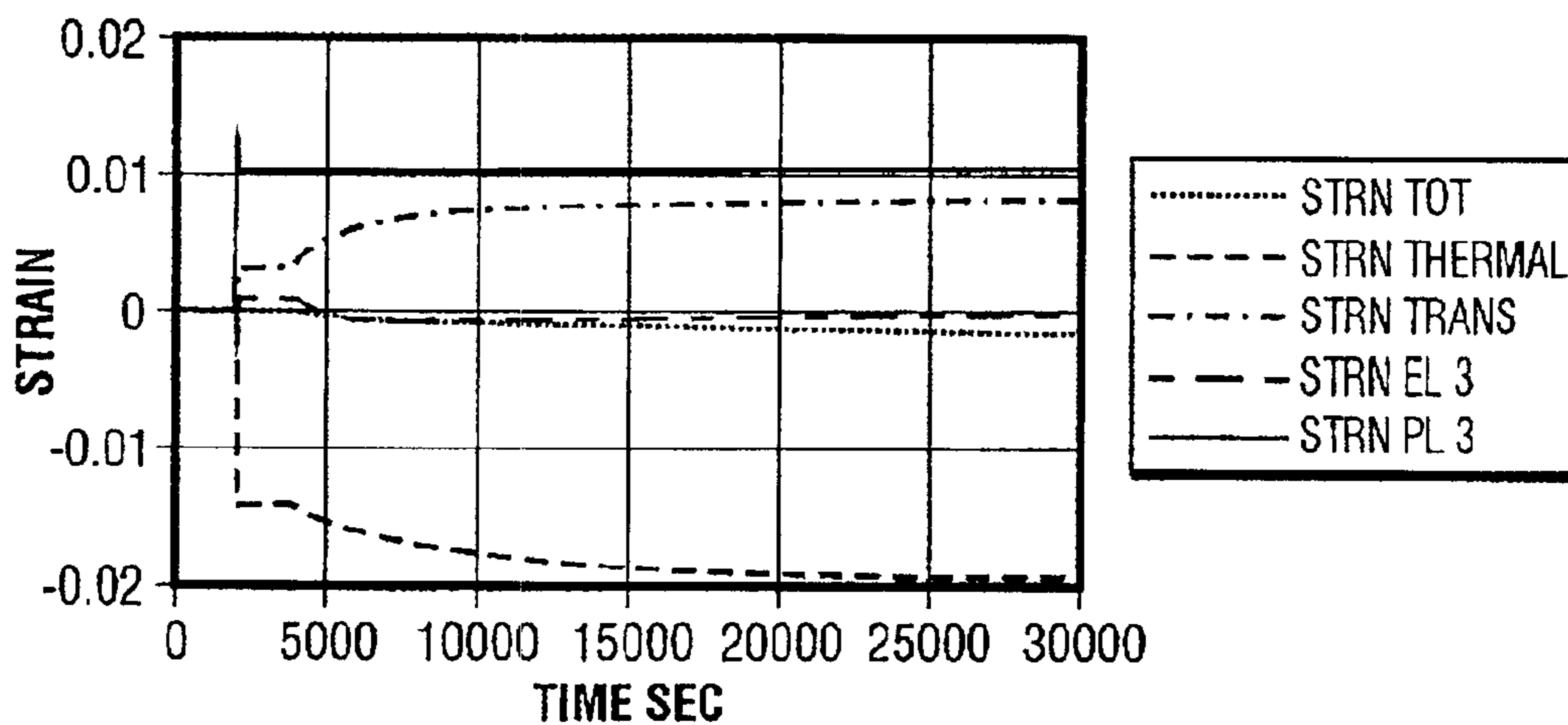
In-Plane Strains, Position #10 FIG. 5
