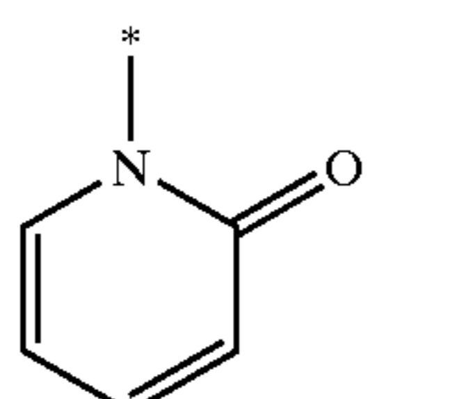
pyrid-2-on-1-yl
