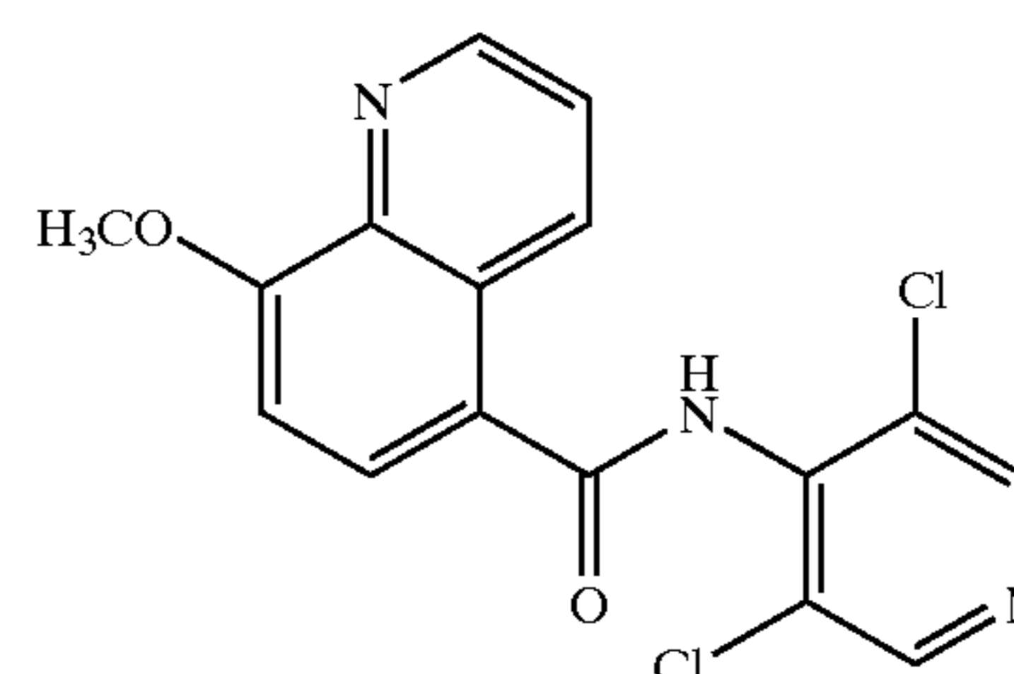
D4418
