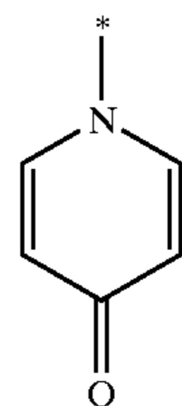
pyrid-4-on-1-yl
