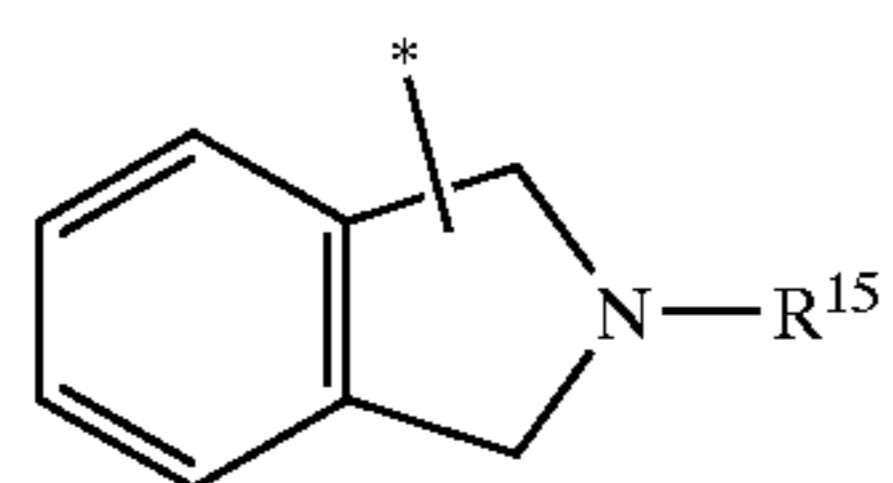
isoindolinyl
