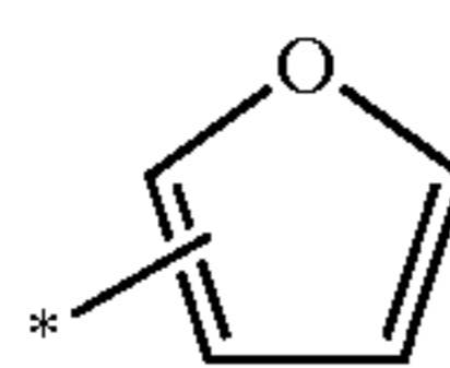
furanyl
