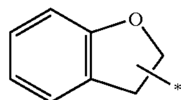
2,3-dihydrobenzofuranlyl
