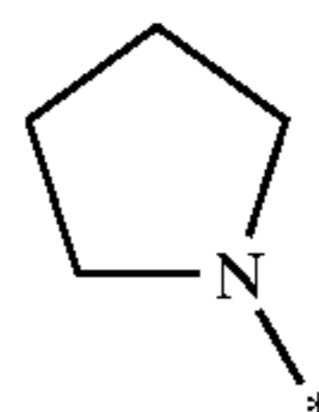
pyrrolidin-1-yl
