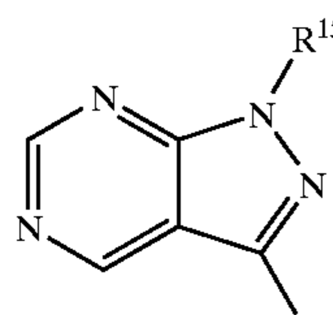
1H-pyrazolo[3,4-d]- pyrimidinyl
