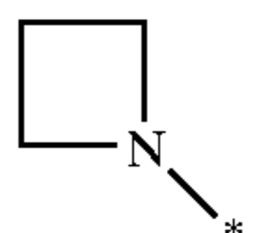
azetidin-1-yl
