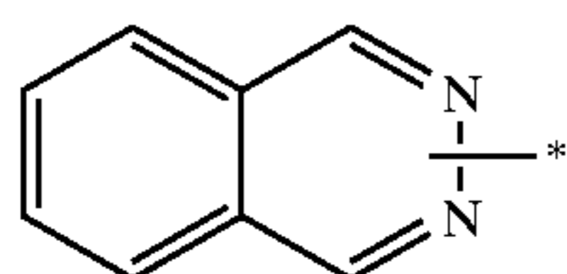
phthalazinyl
