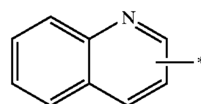
quinolinyl
