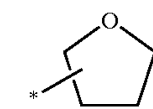
tetrahydrofuranyl
