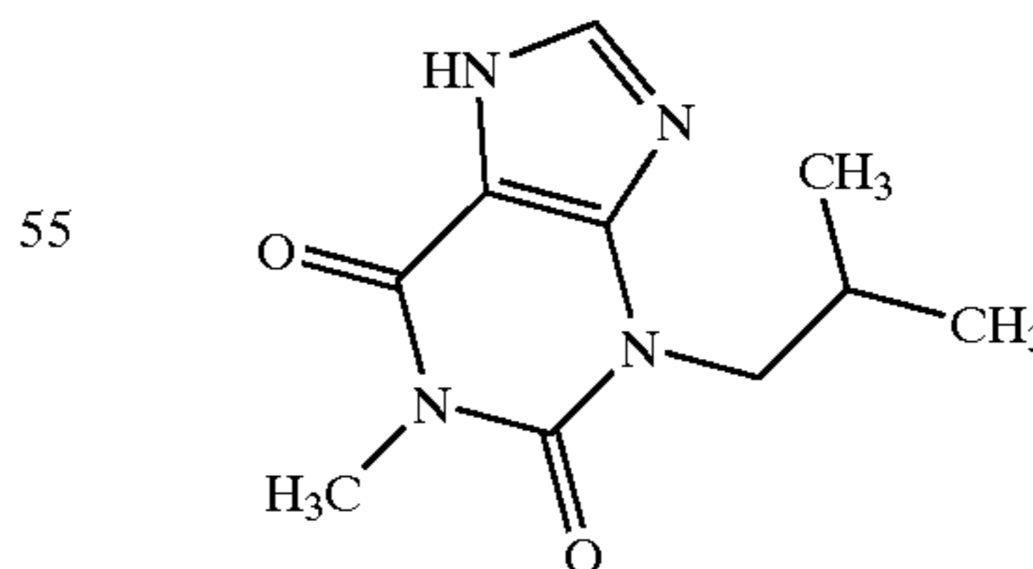
IBMX
