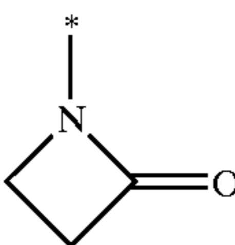
azetid-2-on-1-yl
