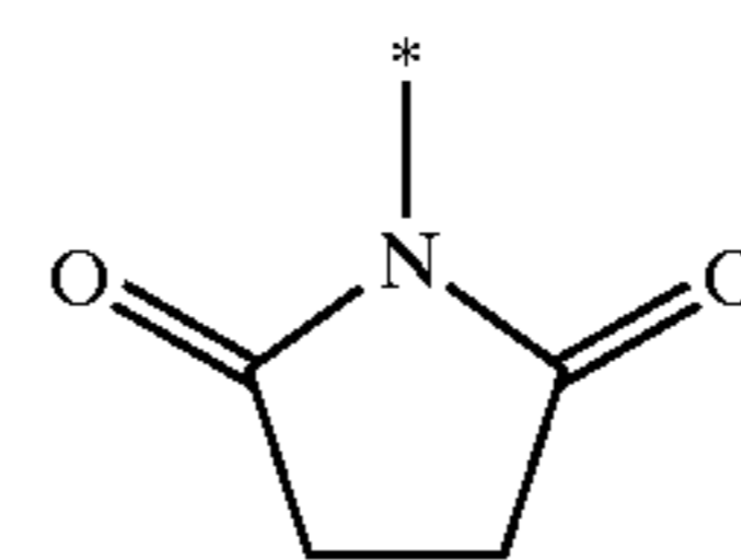
succinimid-1-yl
