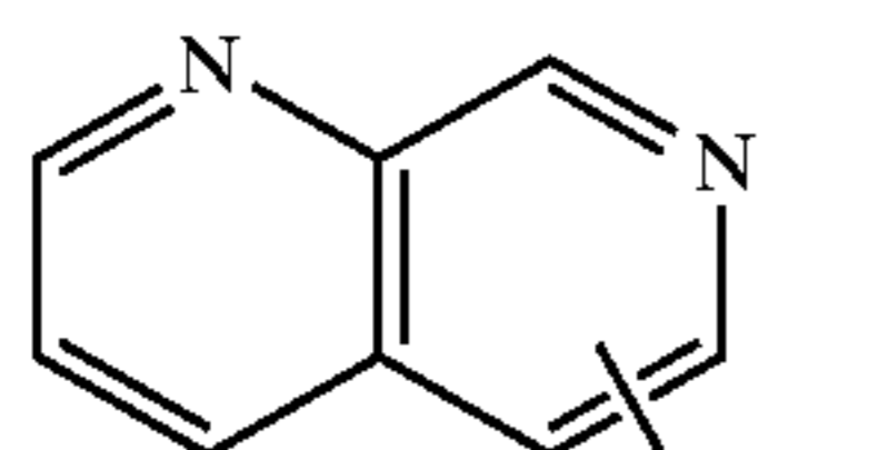
pyridopyridinyl
