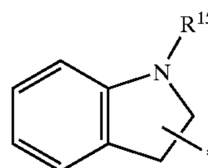
indolinyl
