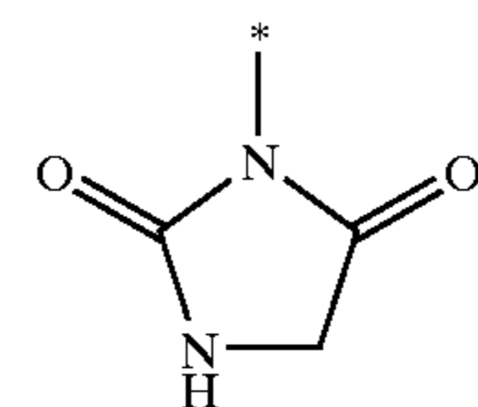
imidazolidin-2,4-dion-1-yl
