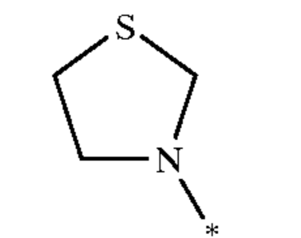
thiazolidin-3-yl
