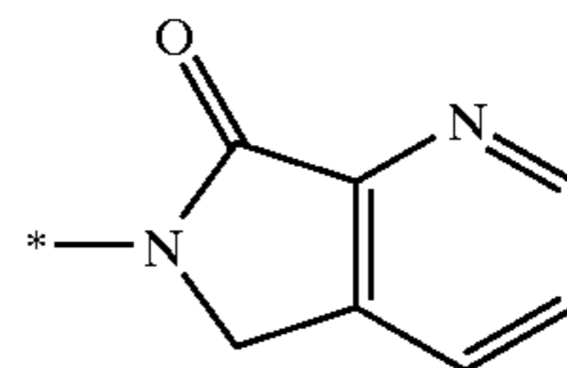
pyrrolo[3,4-b]pyridin- 7-on-6-yl
