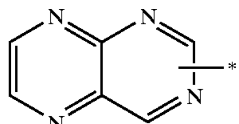
pteridinyl
