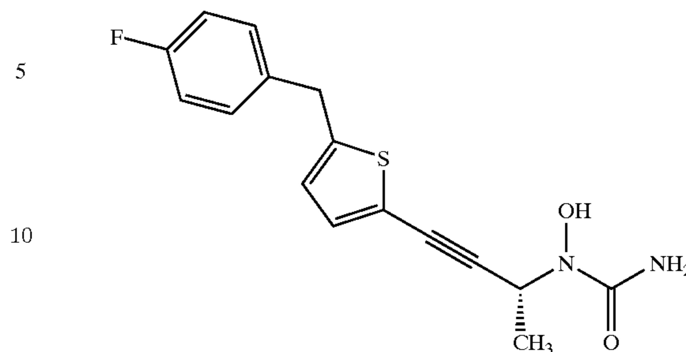
ABT-761
