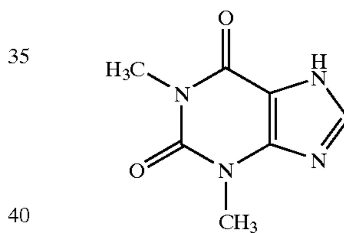
Theophylline
