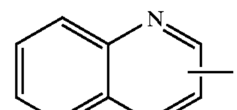
quinolinyl
