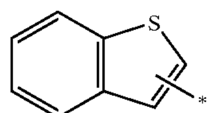
benzothieryl
