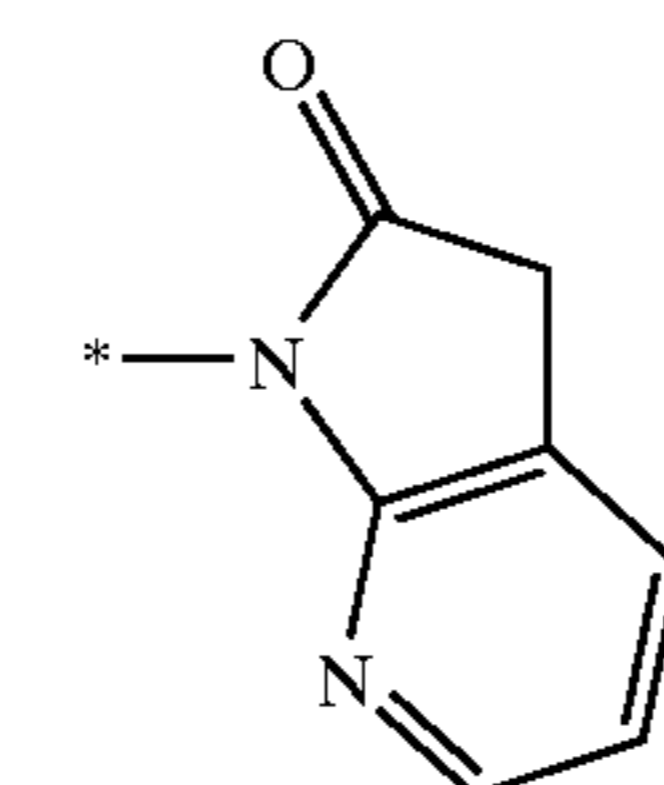
pyrrolo[4,5-b]pyridin- 3-on-2-yl
