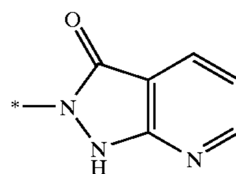
1H-pyrazolo[4,5- e]pyridin-4-on-2-yl
