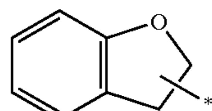
2,3-dihydrobenzofuranyl
