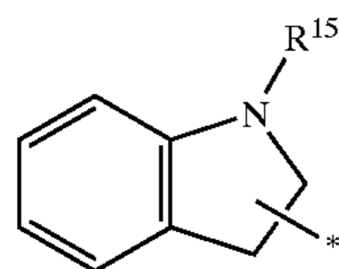
indolinyl
