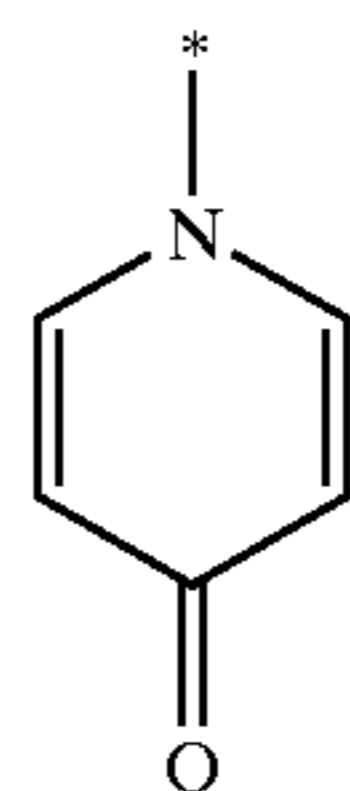
pyrid-4-on-1-yl
