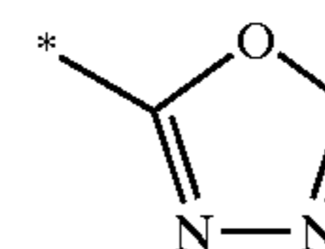
1,3,4-oxadiazolyl
