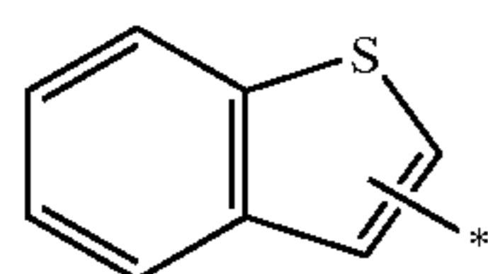
benzothieryl
