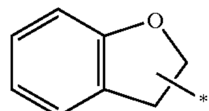
2,3-dihydrobenzo- furanyl
