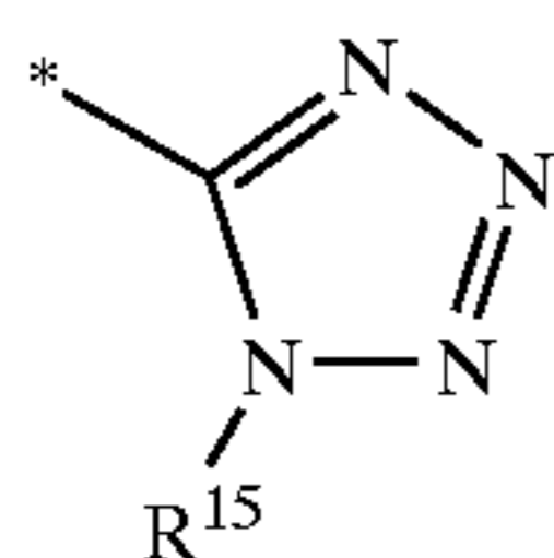
tetrazol-5-yl
