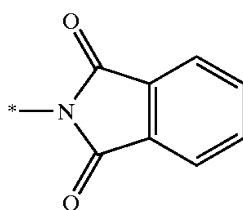
pyrrolo[3,4-b]pyridin- 5,7-dion-6-yl
