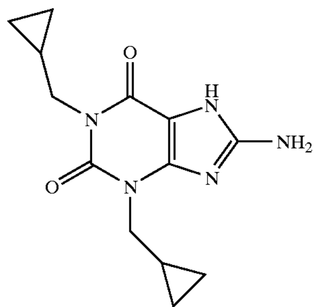
Cipamfylline
