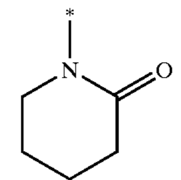
piperid-2-on-1-yl
