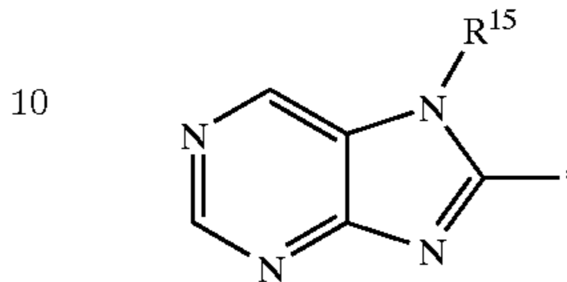
1H-puriny
