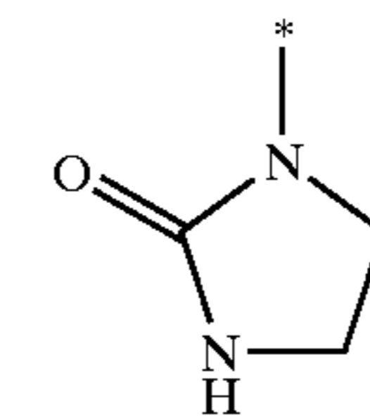
imidazolidin-2-on-1-yl
