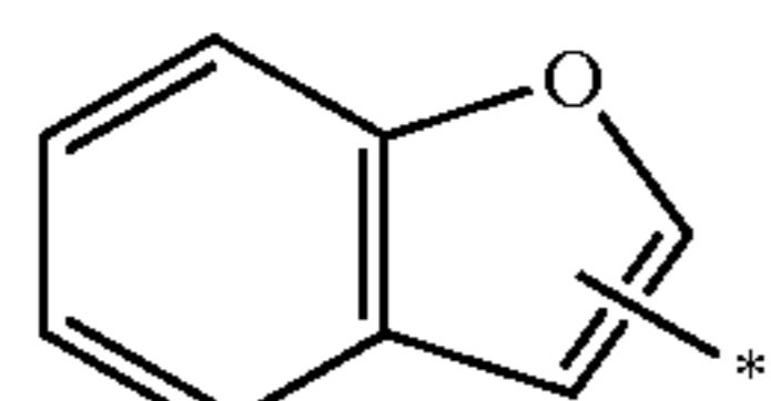
benzo[b]furanlyl
