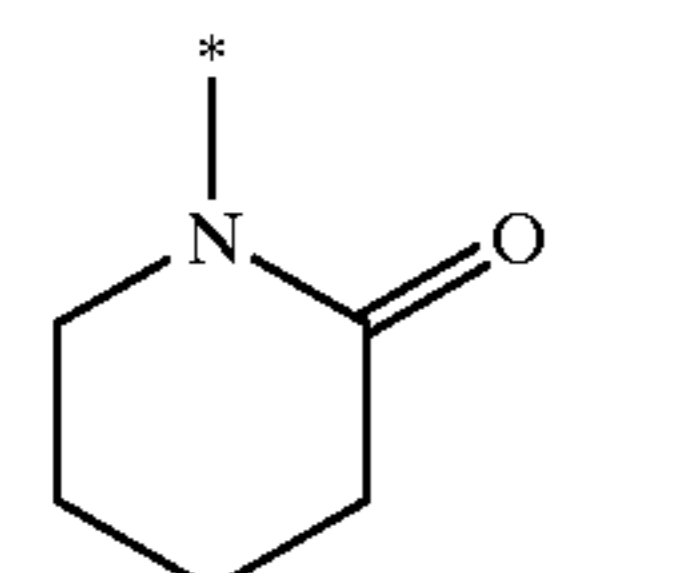
piperid-2-on-1-yl
