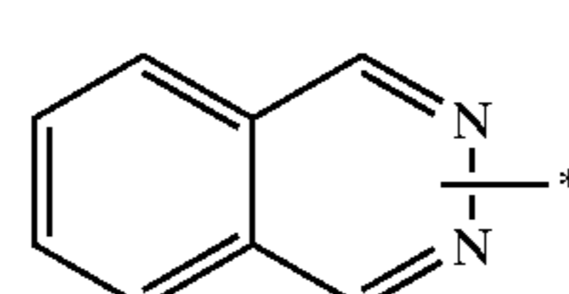
phthalazinyl
