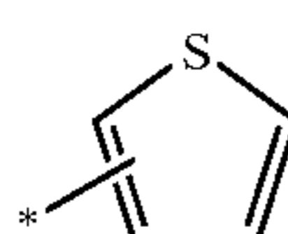
thienyl
