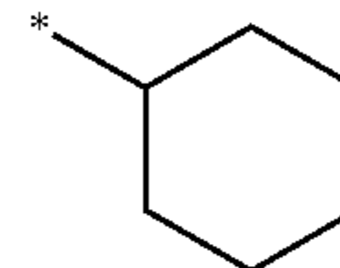
cyclohexyl
