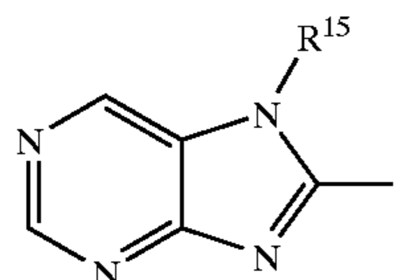
1H-puriny
