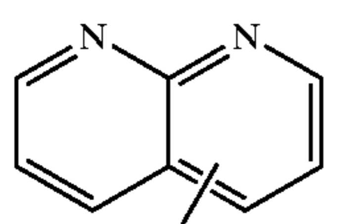
1,8-naphthyridinyl
