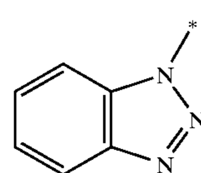
benzothiazolyl
