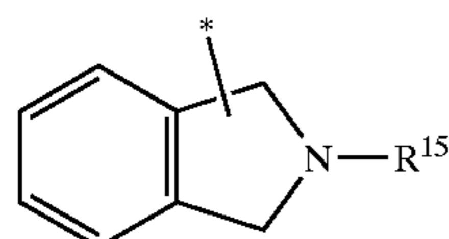
isoindolinyl
