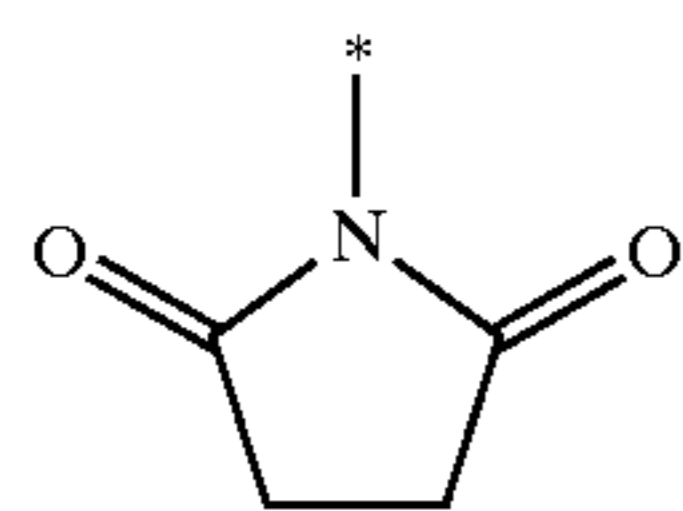
succinimid-1-yl
