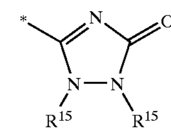
1,2,4-triazol-3-on-5-yl
