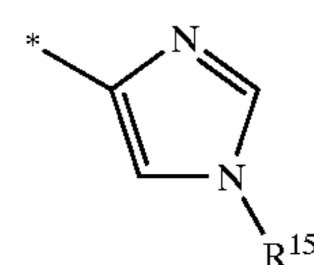
imidazol-4-yl
