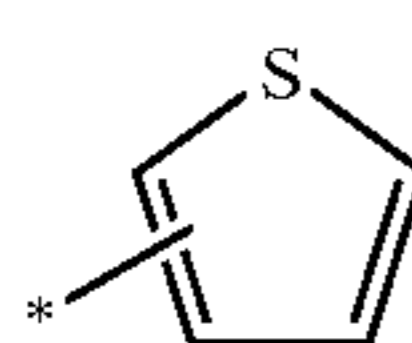
thienyl
