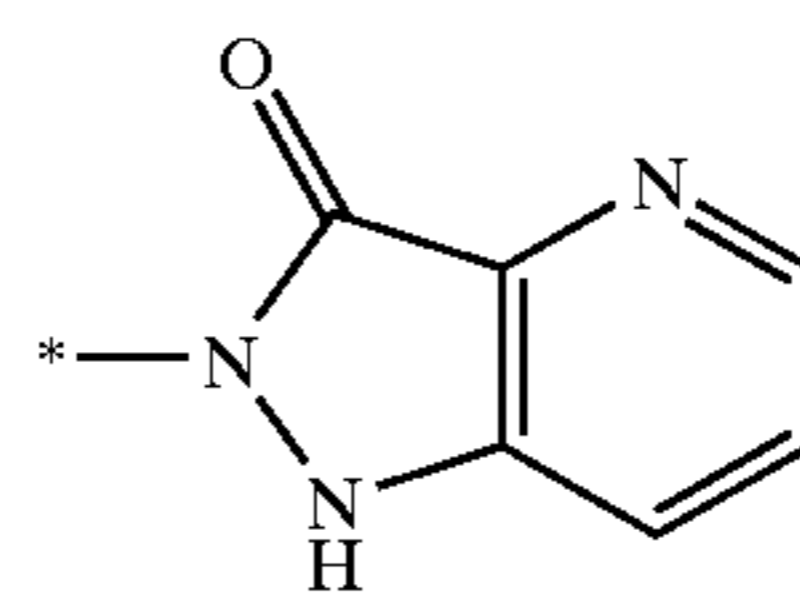
1H-pyrazolo[4,5- e]pyridin-7-on-2-yl
