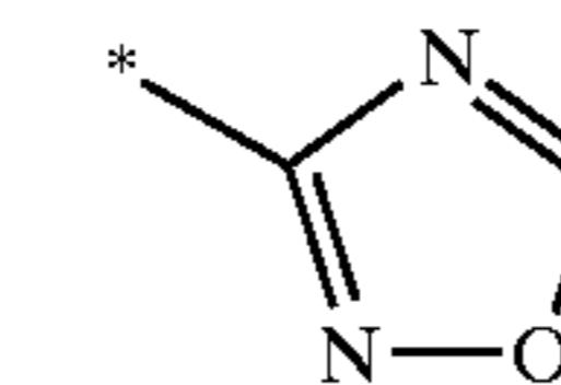
1,2,4-oxadiazol-3-yl
