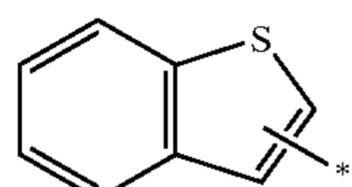
benzothieryl
