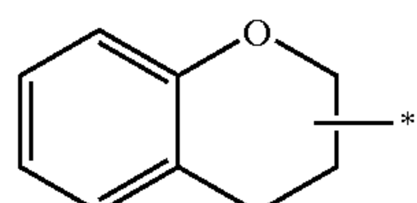
chromanyl
