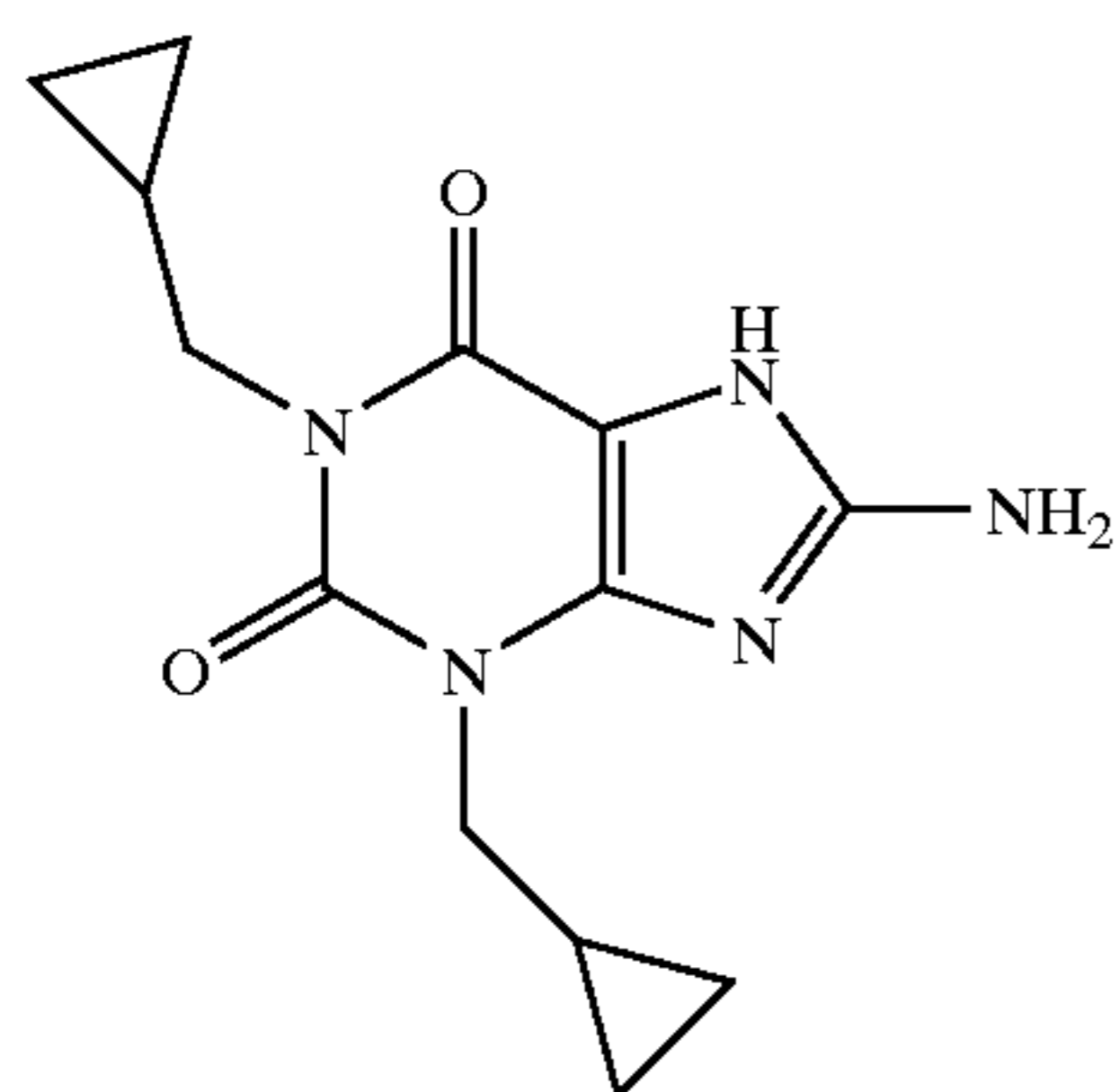
Cipamfylline (BRL-61,063)
