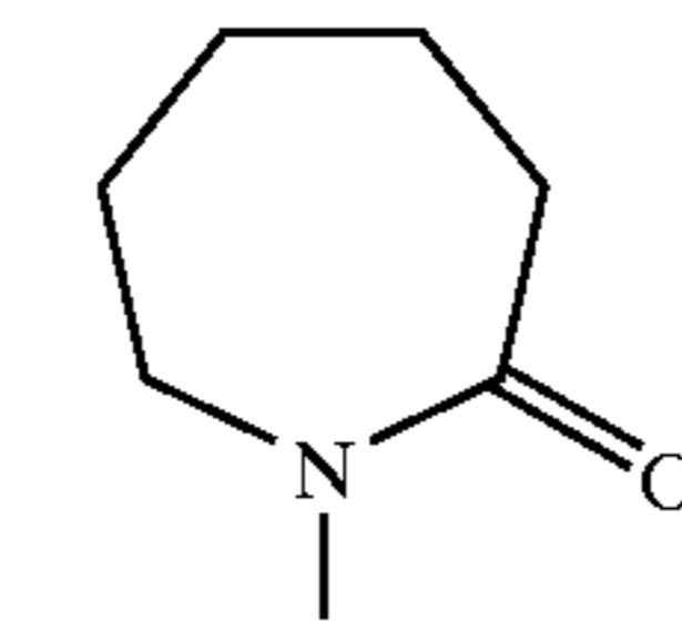
2H-azepin-2-on-1-yl
