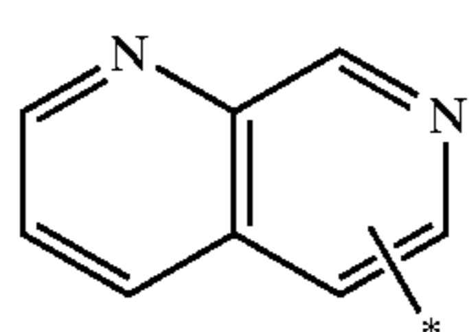
1,7-naphthyridinyl
