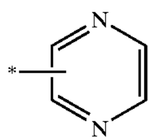
pyrazinyl
