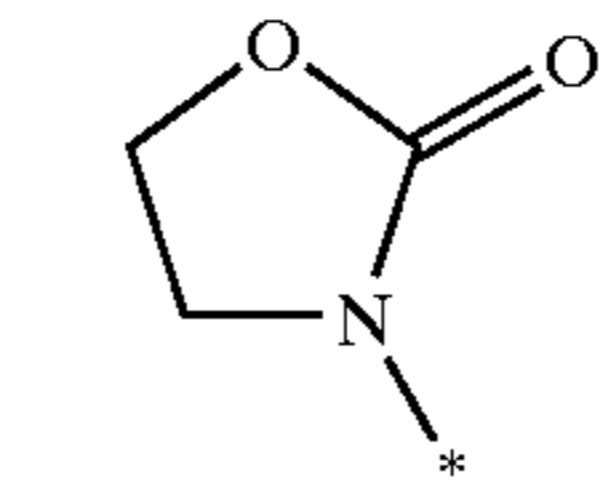
oxazolidin-2-on-1-yl
