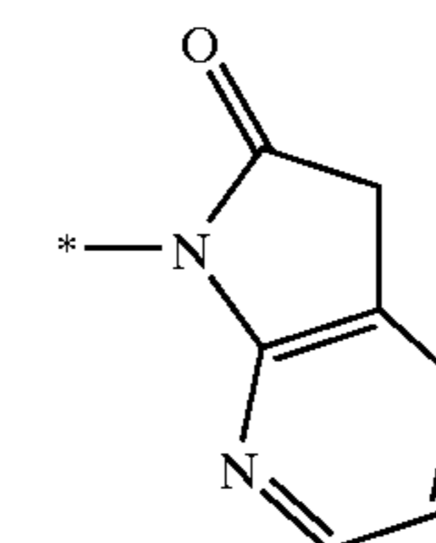
pyrrolo[4,5-b]pyridin- 3-on-2-yl
