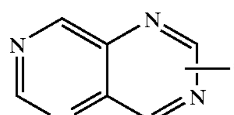
pyrimido[5,4-d]- pyrimidinyl
