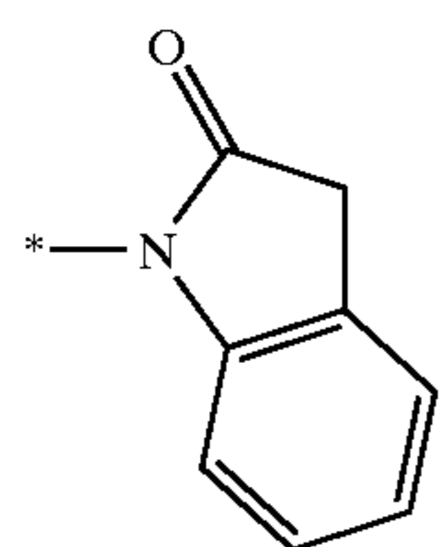
1,3-dihydro-indol-2-on-1-yl
