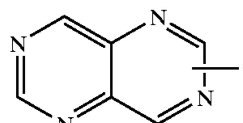
pyrimido[5,4-d]- pyrimidinyl
