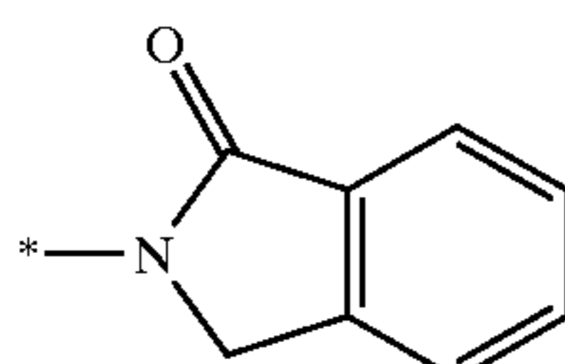
2,3-dihydro-iso-indol- 1-on-2-yl
