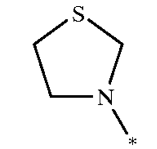
thiazolidin-3-yl
