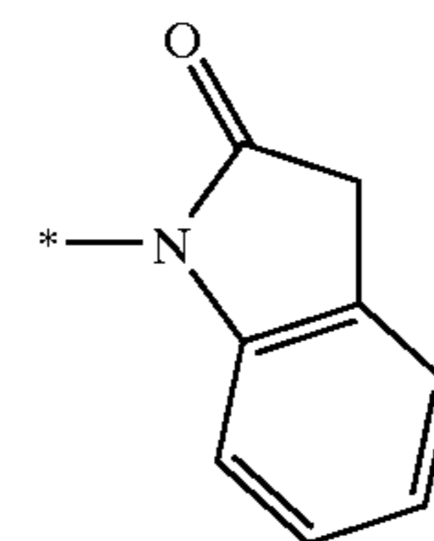
1,3-dihydro-indol-2- on-1-yl
