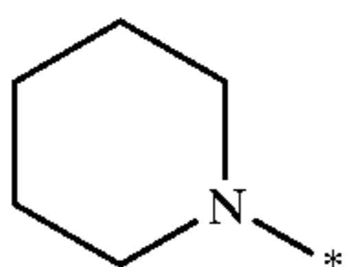
piperidin-1-yl
