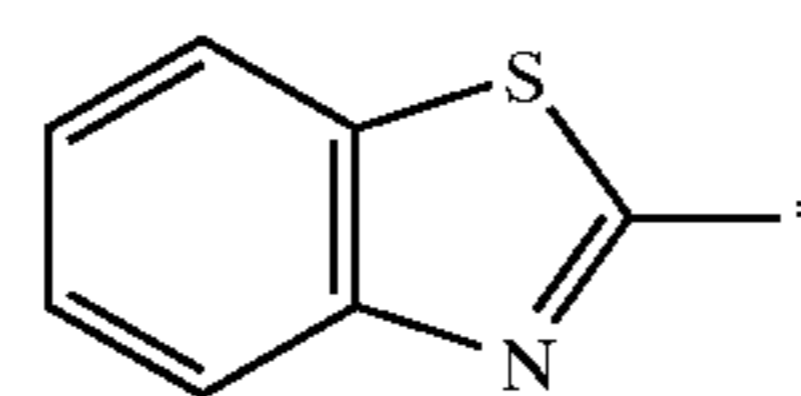
benzothiazolyl
