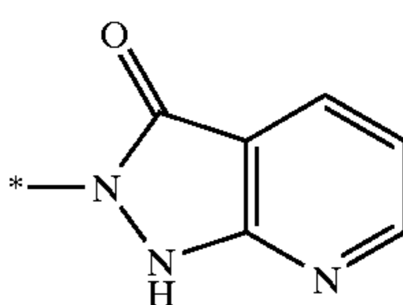
1H-pyrazolo[4,5-e]pyridin-4-on-2-yl
