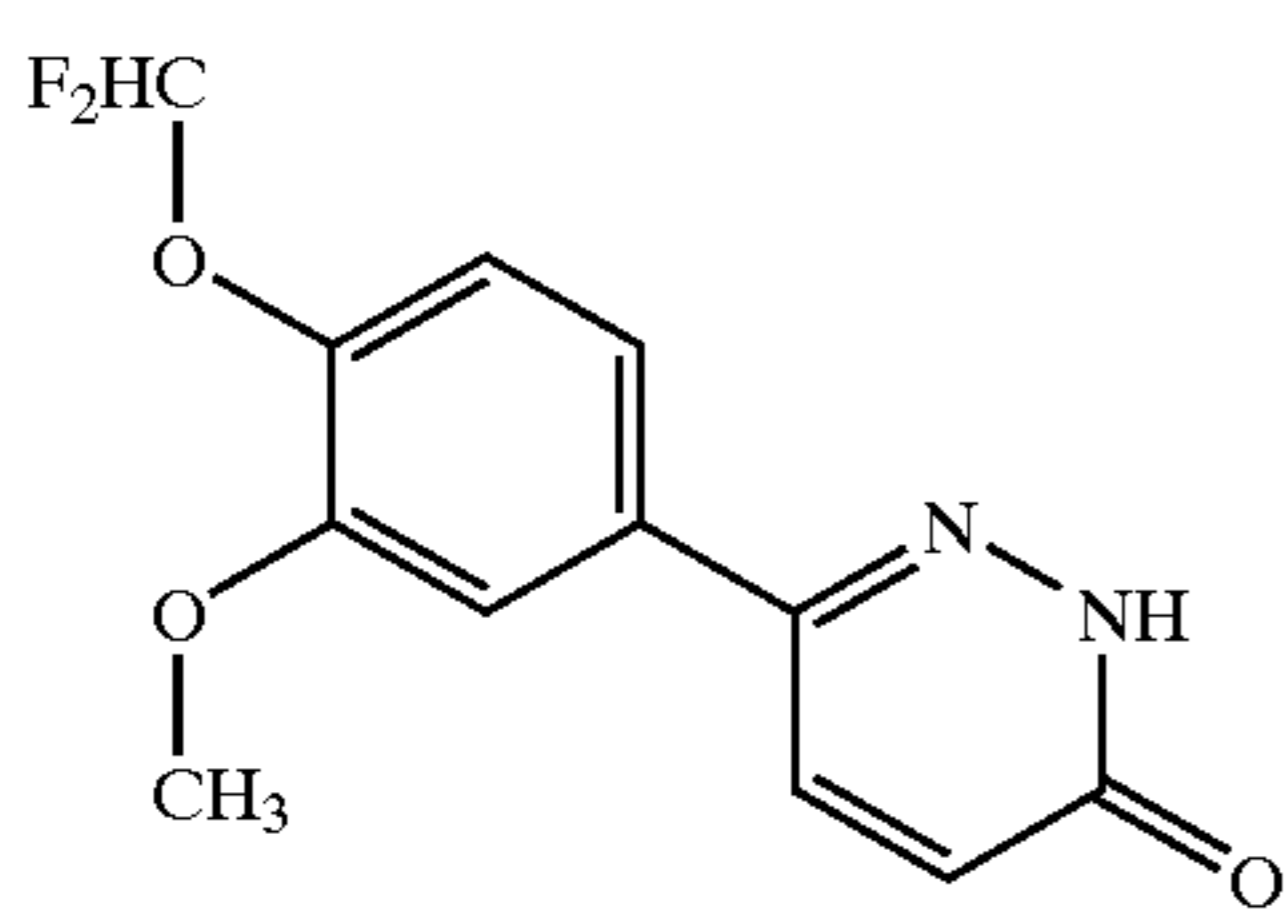
Zardaverine
