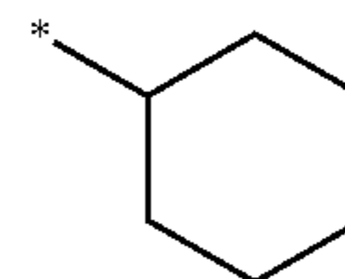
cyclohexyl
