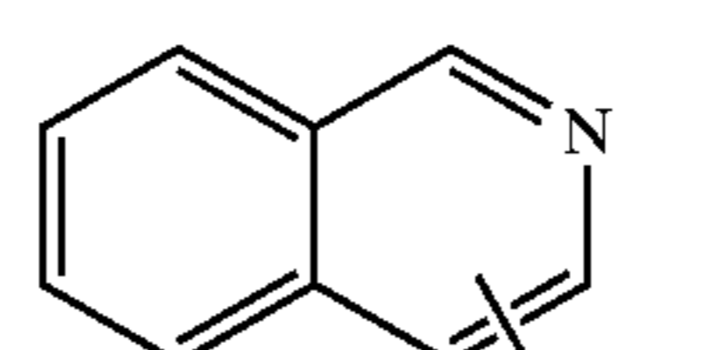
isoquinolinyl
