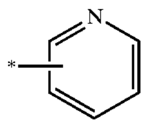
pyridyl
