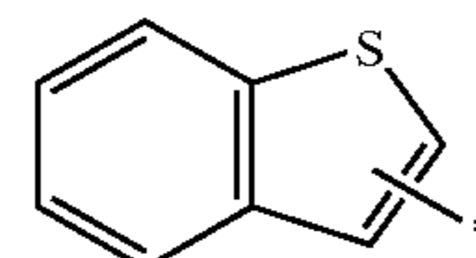
benzothiophenyl
