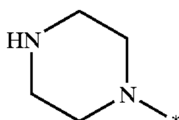
piperazin-1-yl
