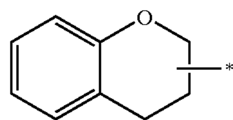
chromanyl
