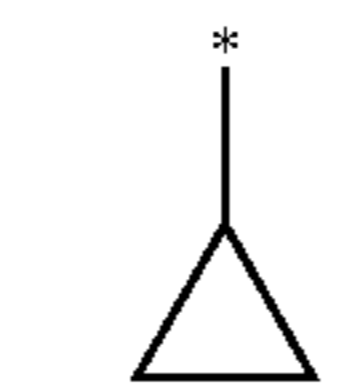
cyclopropyl
