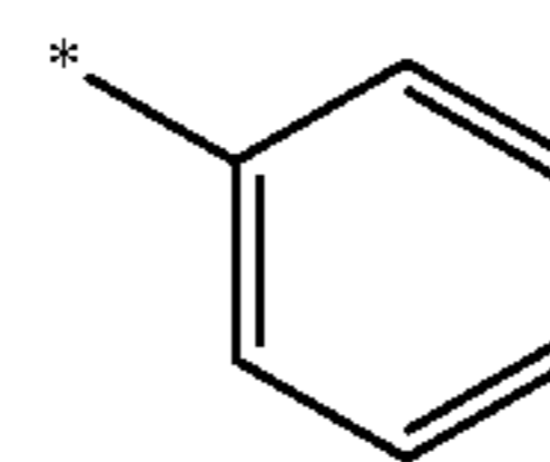
phenyl
