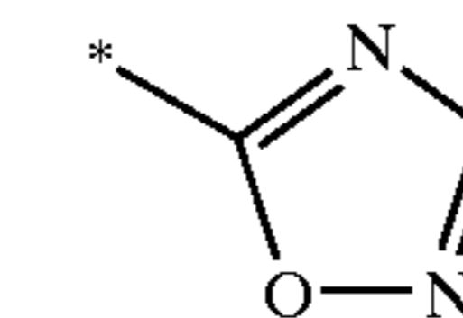
1,2,4-oxadiazol-5-yl
