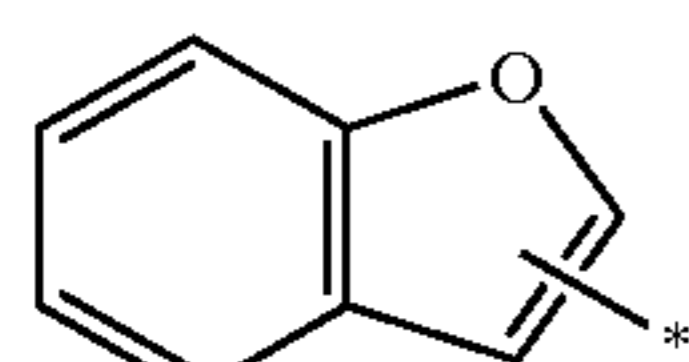
benzo[b]furanyl
