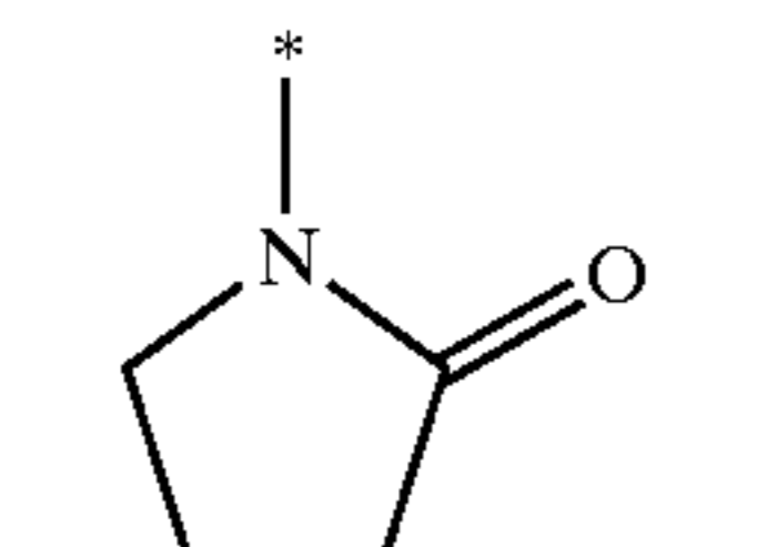
pyrrolidin-2-on-1-yl
