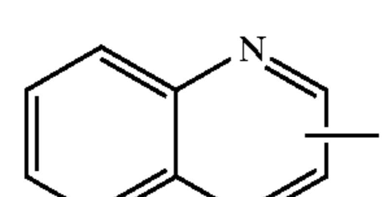
quinolinyl
