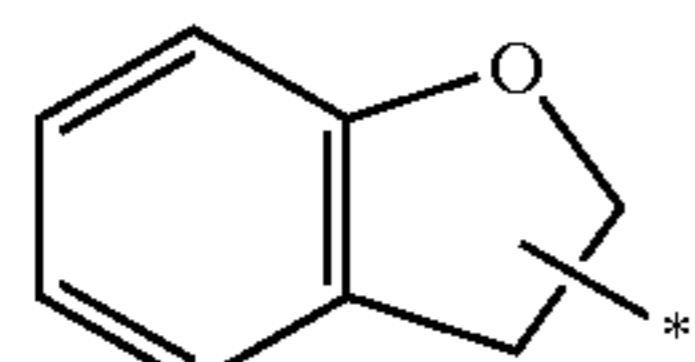
2,3-dihydrobenzofuranlyl
