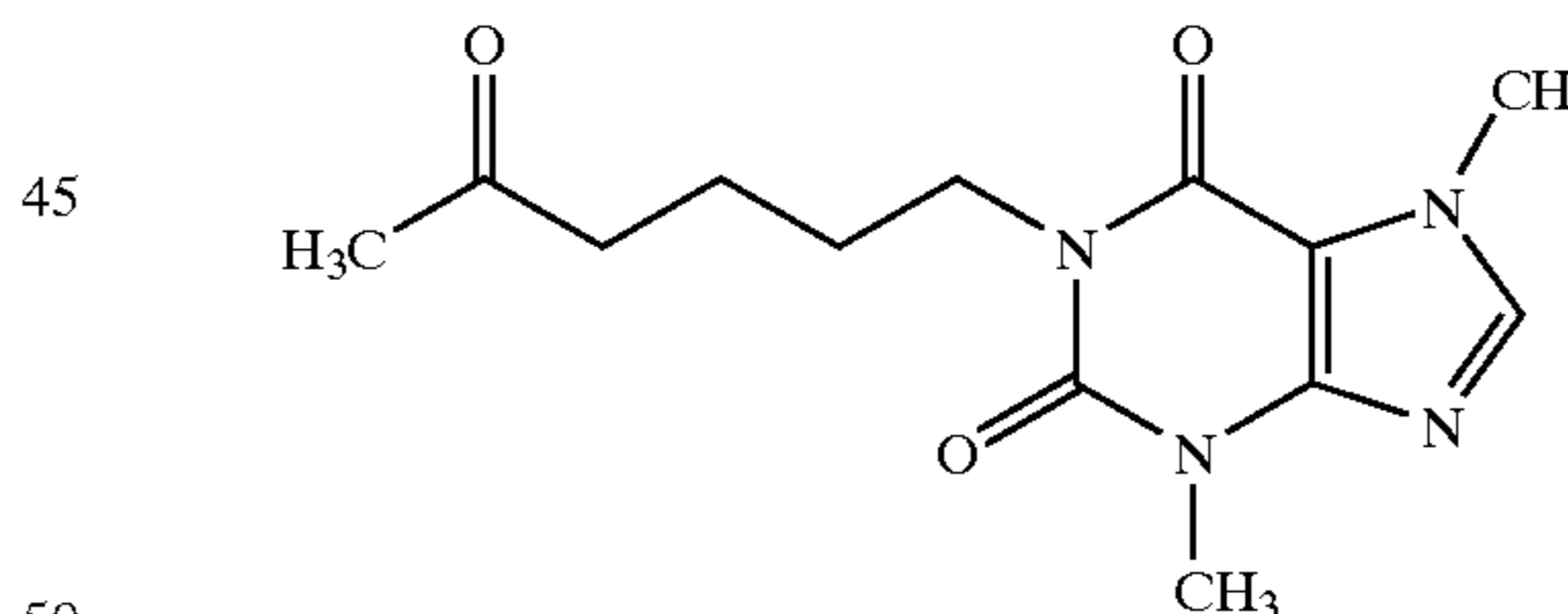
Pentoxifylline
