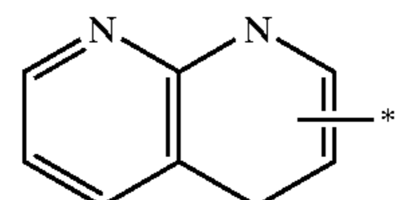
1,8-naphthyridinyl
