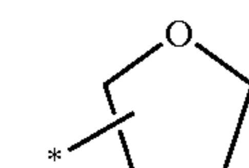
tetrahydrofuranyl
