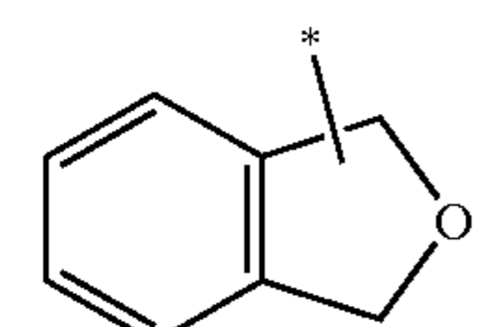
1,3-dihydroisobenzofuranyl; phthalanyl
