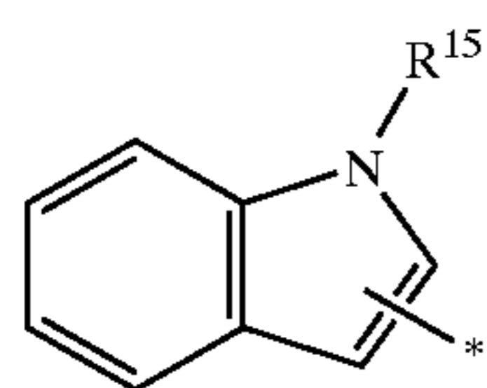
indoyl
