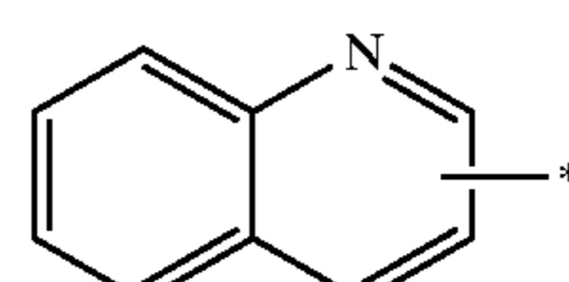
quinolinyl
