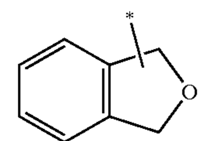
1,3-dihydroisobenzofuranlyl; phthalanyl
