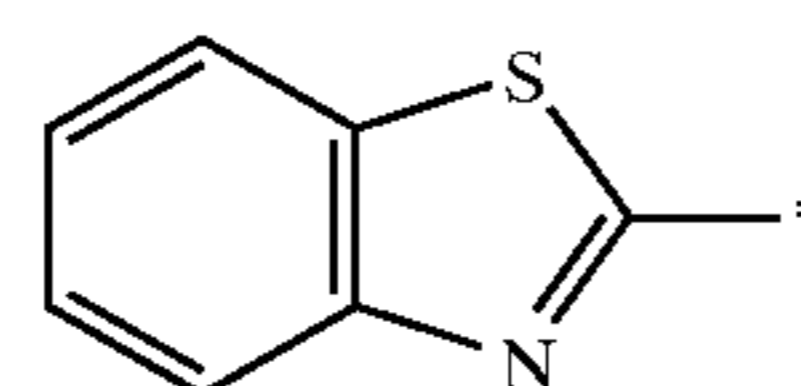
benzothiazolyl
