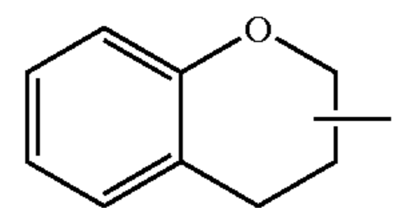
chromanyl
