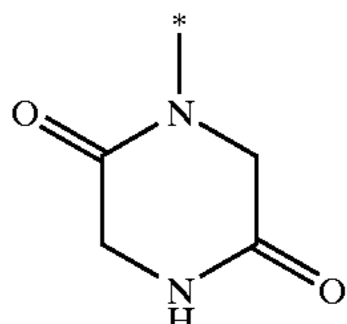
piperazin-2,5-dion-1-yl
