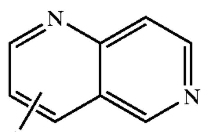
1,6-naphthyridinyl
