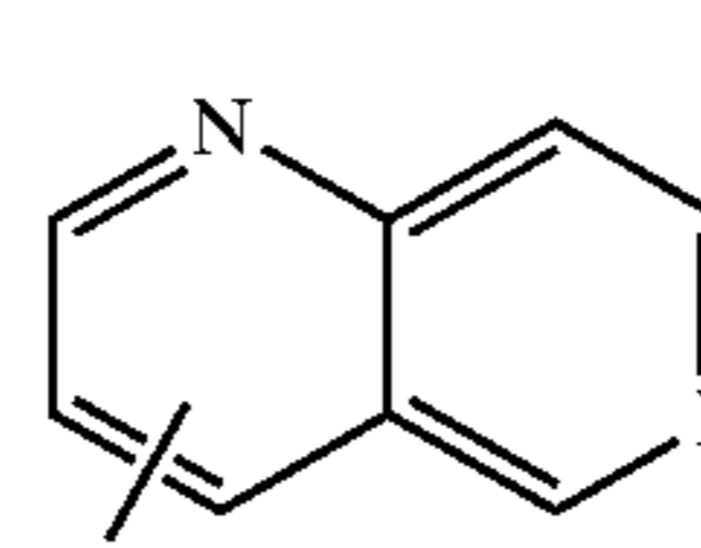
1,6-naphthyridinyl
