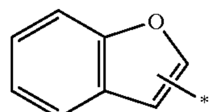
benzo[b]furanyl
