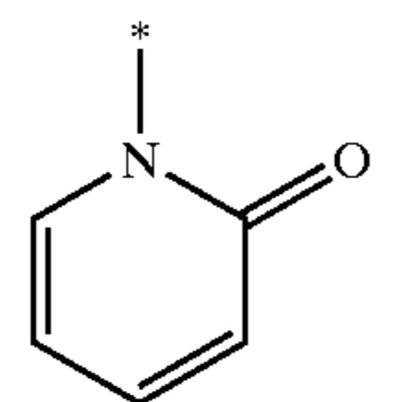
pyrid-2-on-1-yl
