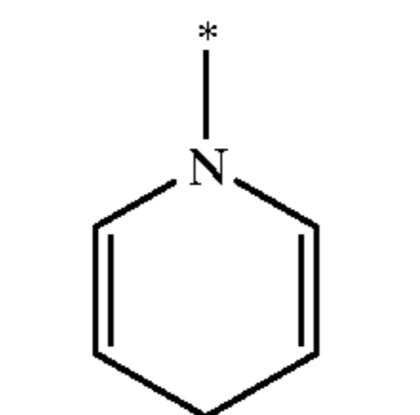
pyrid-4-on-1-yl
