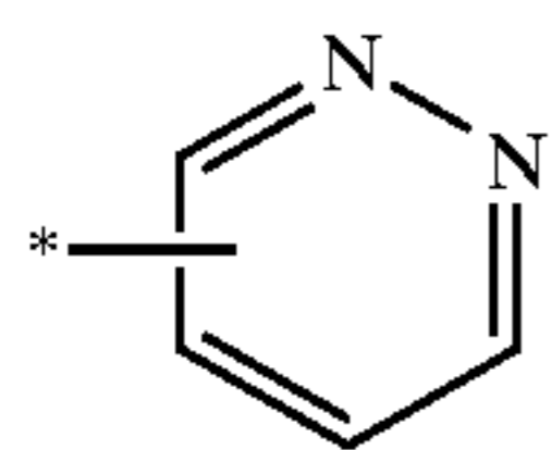
pyridazinyl
