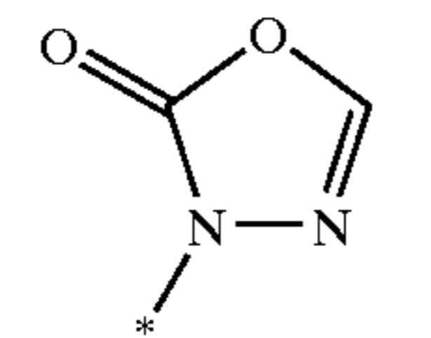
1,3,4-oxadiazol-2(3H)-on-3-yl
