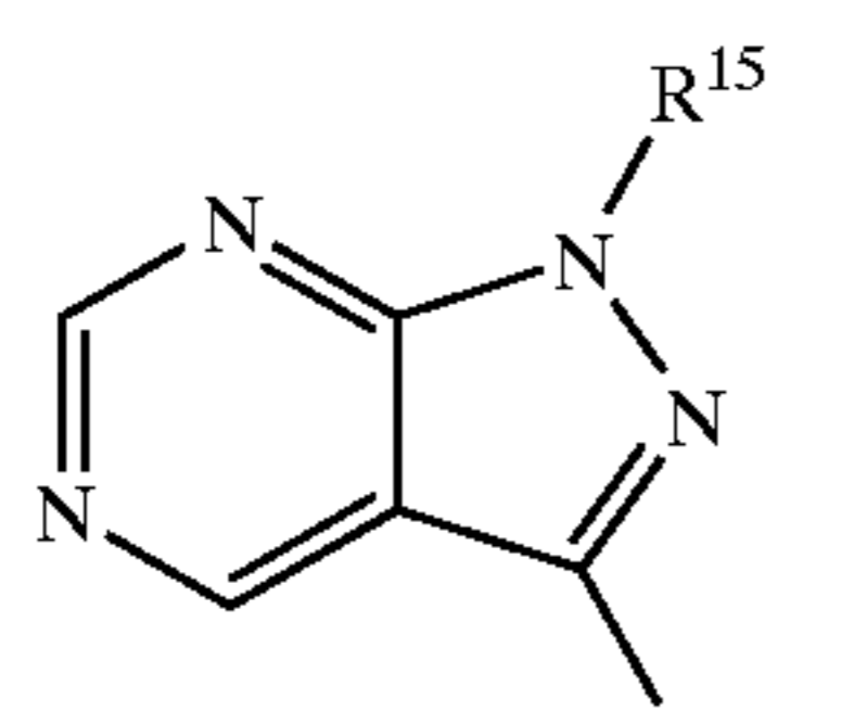
1H-pyrazolo[3,4-d]- pyrimidinyl
