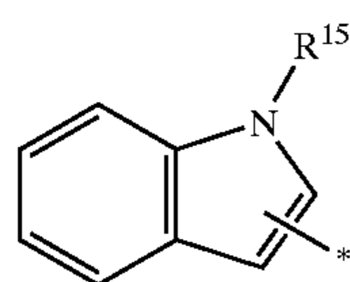
indoyl
