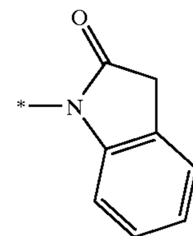
1,3-dihydro-indol-2- on-1-yl
