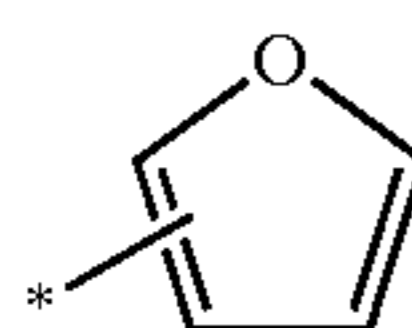
furanyl
