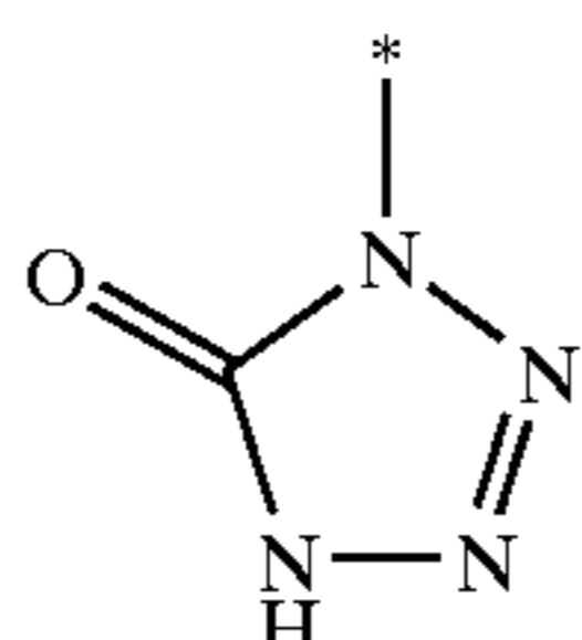
4,5-dihydro-5-oxo-1H-tetrazol-1-yl
