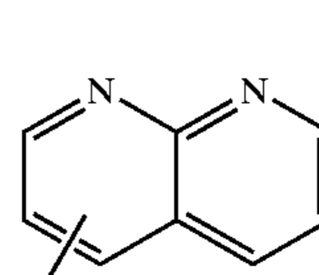
1,8-naphthyridinyl
