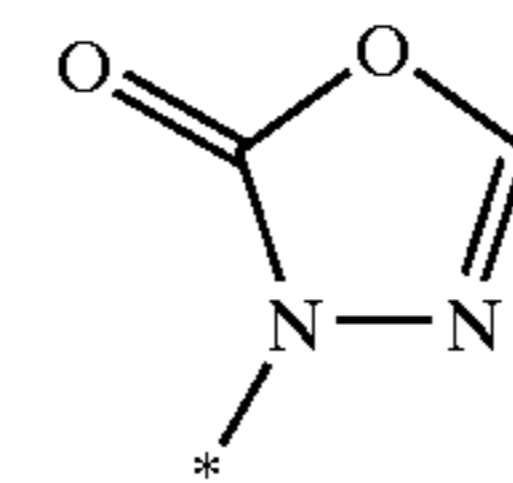
1,3,4-oxadiazol-2(3H)-on-3-yl
