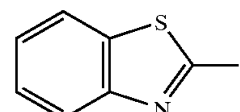
benzothiazolyl
