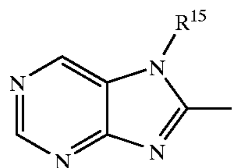
1H-puriny
