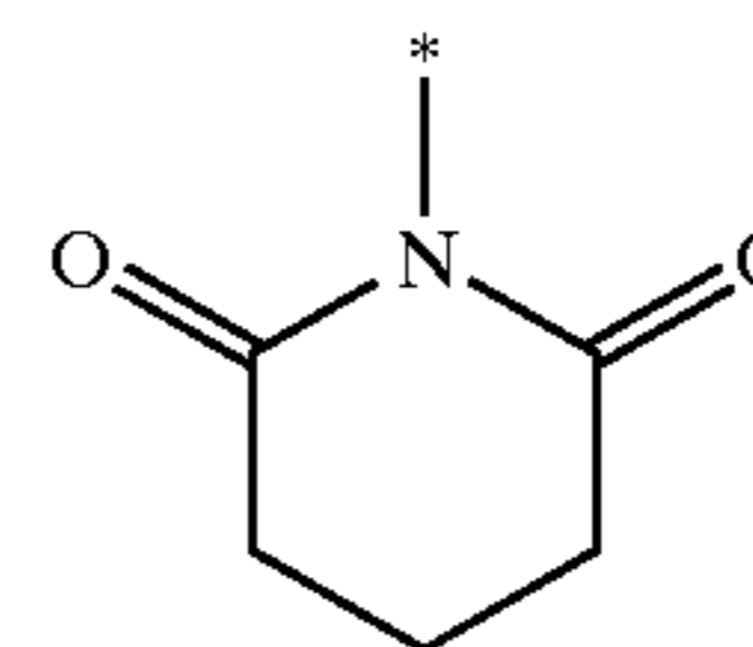
glutarimid-1-yl
