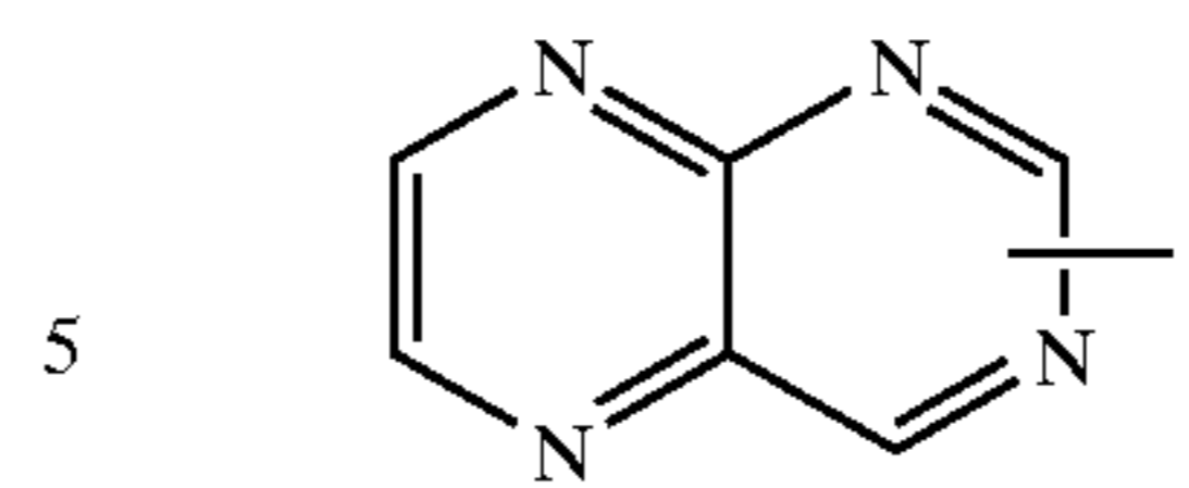
pteridinyl
