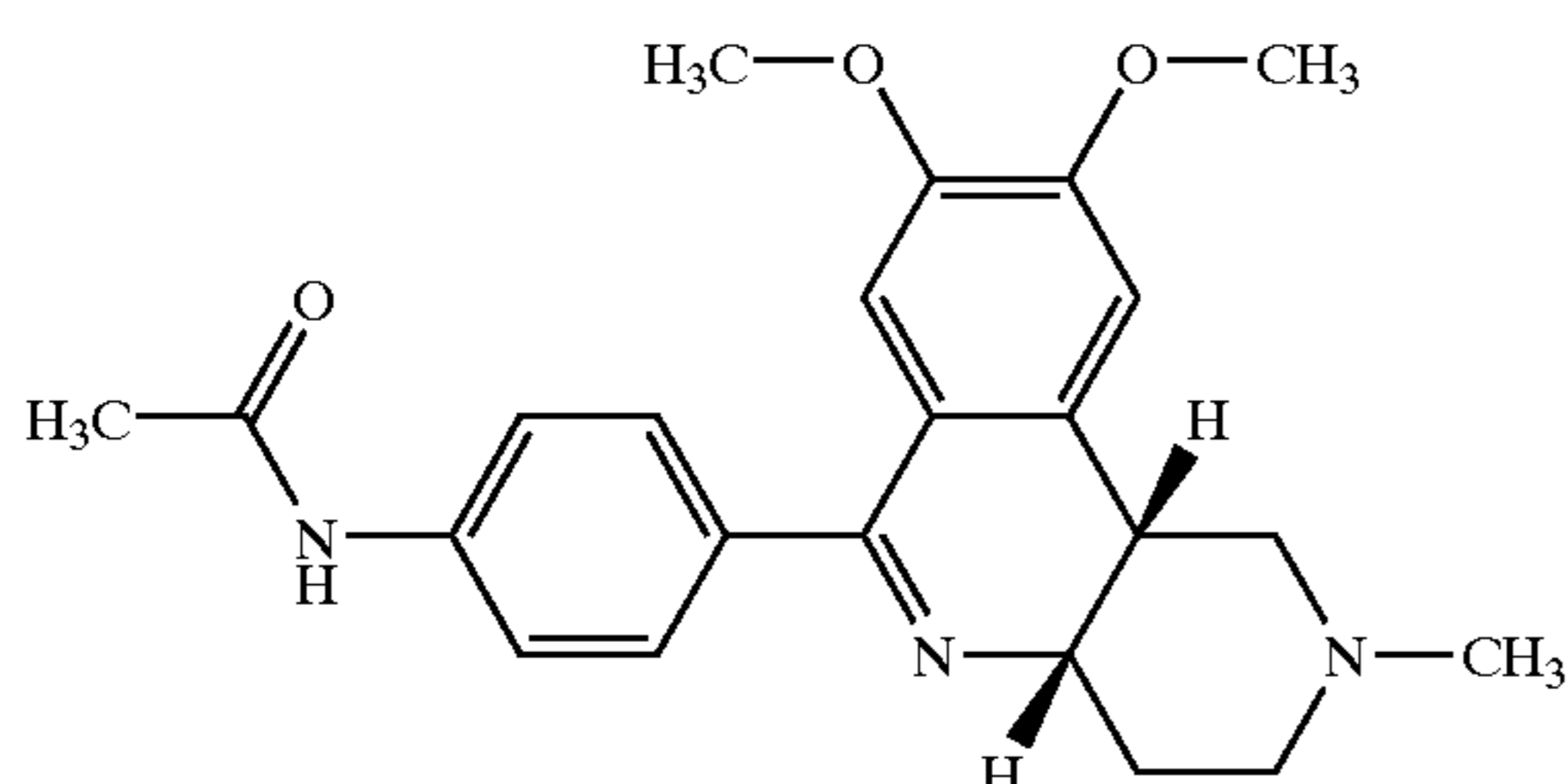
Benafentrine
