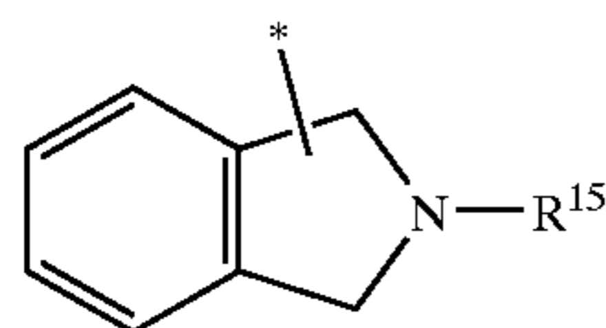
isoindolinyl
