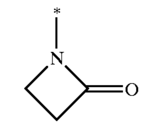
azetidin-2-on-1-yl
