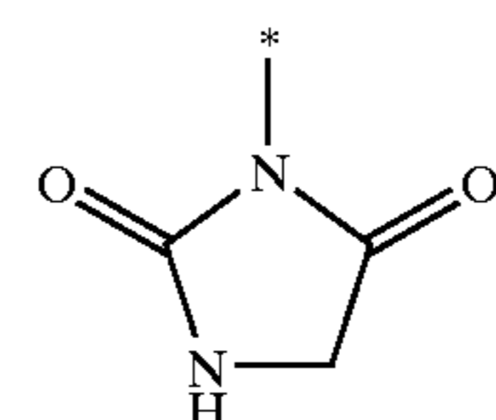
imidazolidin-2,4-dion-1-yl
