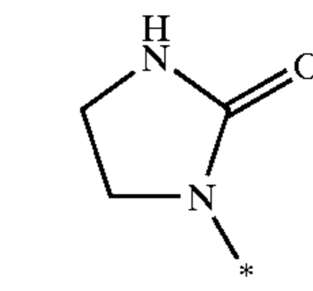
imidazolidin-2-on-1-yl
