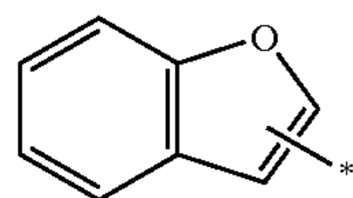
benzo[b]furanlyl
