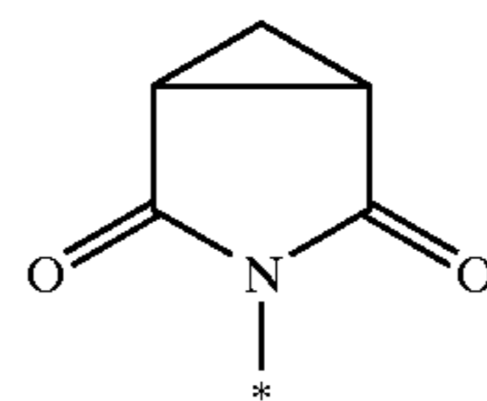
3-azabicyclo[3.1.0]hexane-2,4-dion-3-yl
