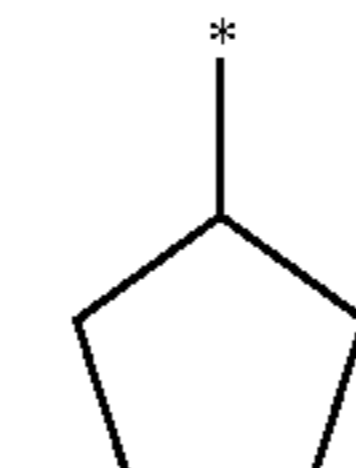
cyclopentyl
