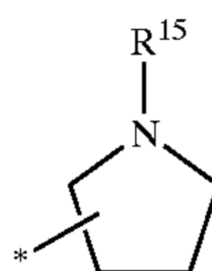
pyrrolidinyl
