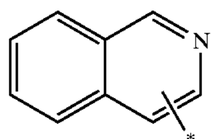
isoquinolinyl
