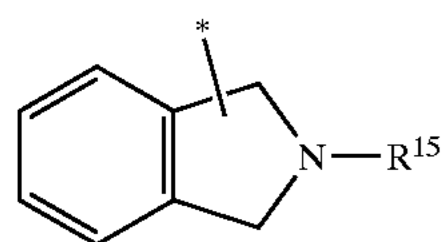
isoindolinyl
