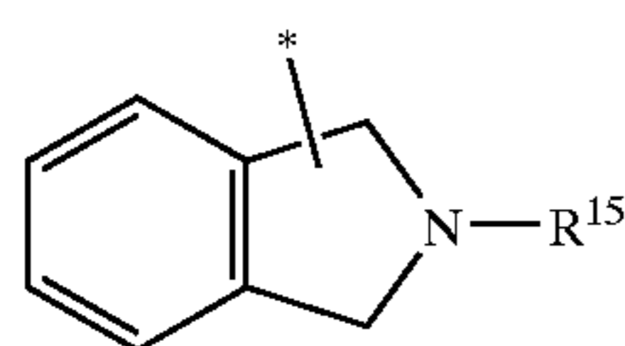
isoindolinyl
