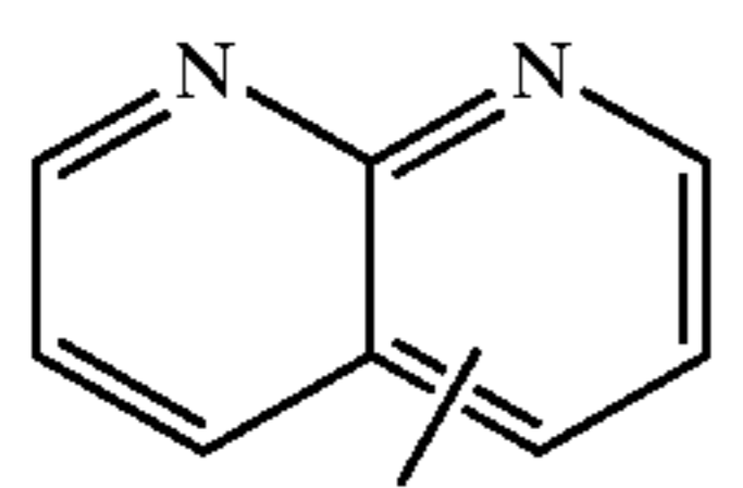
1,8-naphthyridinyl
