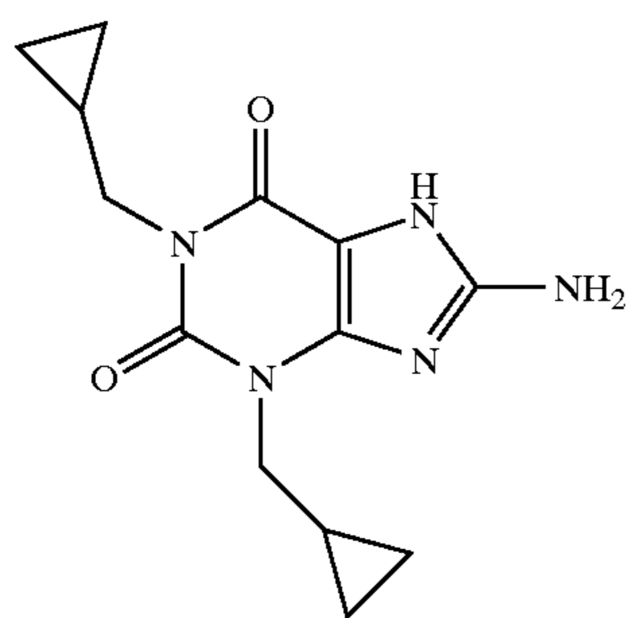
Cipamfylline
