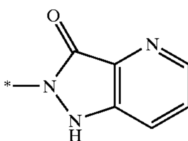
1H-pyrazolo[4,5-e]pyridin-7-on-2-yl
