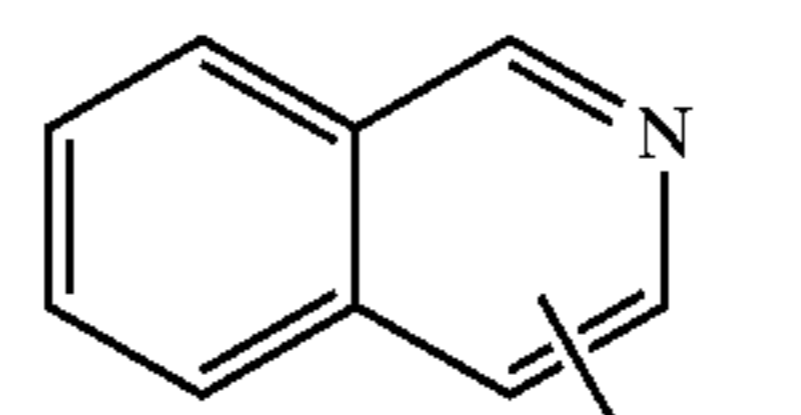
isoquinolinyl
