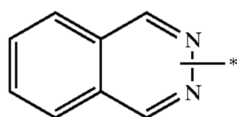
phthalazinyl
