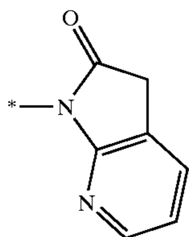
pyrrolo[4,5-b]pyridin-3-on-2-yl
