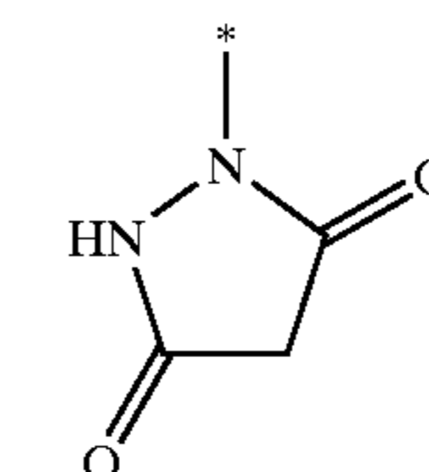
pyrazolidin-3,5-dion-1-yl
