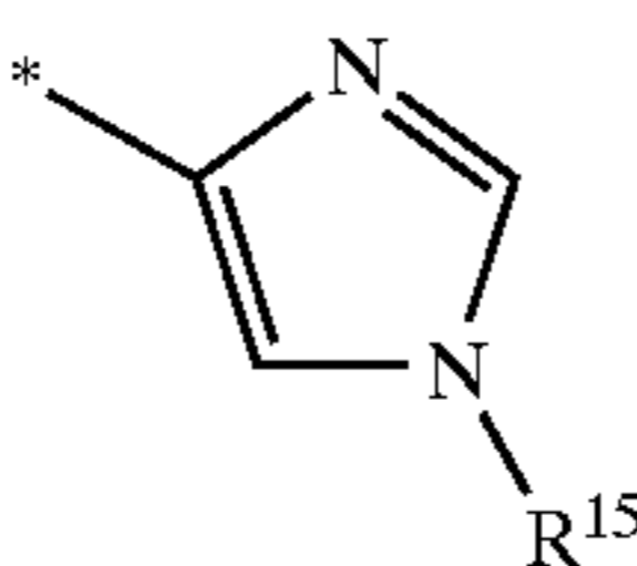
imidazol-4-yl
