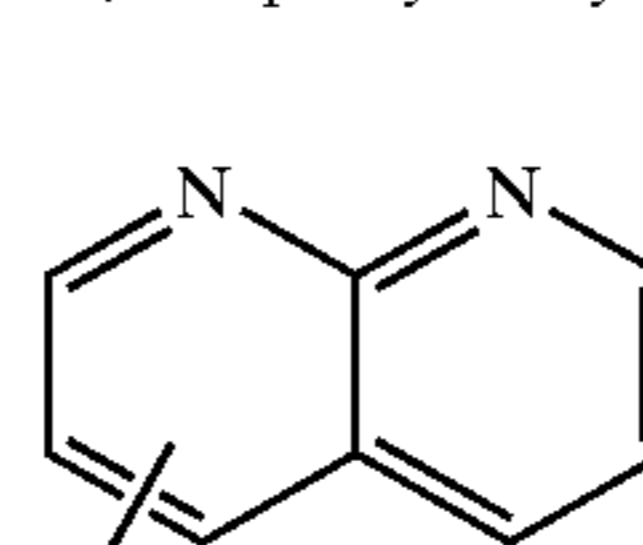
1,8-naphthyridinyl
