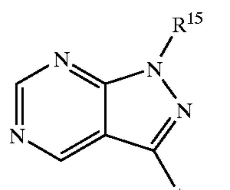
1H-pyrazolo[3,4-d]- pyrimidinyl
