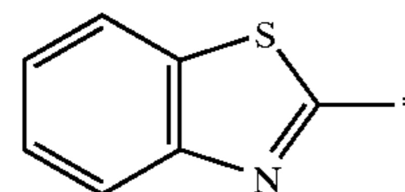
benzothiazolyl
