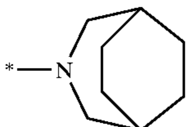
3-azabicyclo[3.2.2]- non-3-yl
