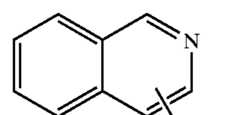
isoquinolinyl
