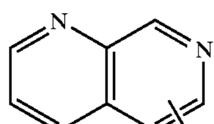
1,7-naphthyridinyl
