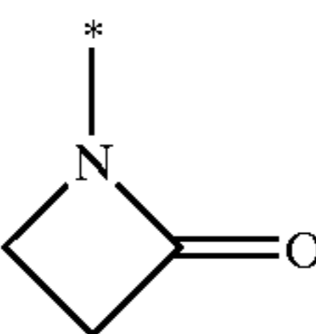
azetid-2-on-1-yl
