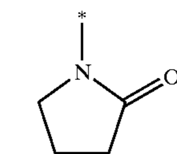
pyrrolidin-2-on-1-yl
