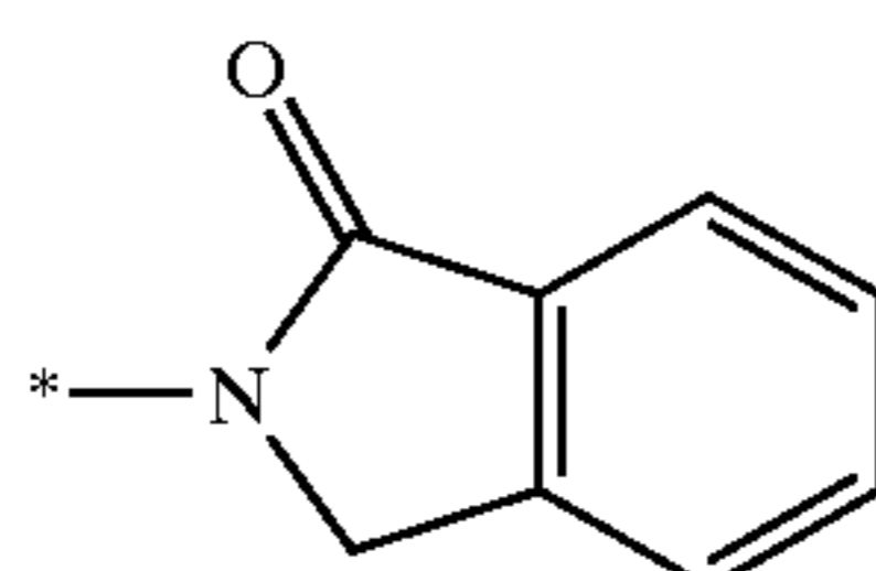
2,3-dihydro-iso-indol- 1-on-2-yl
