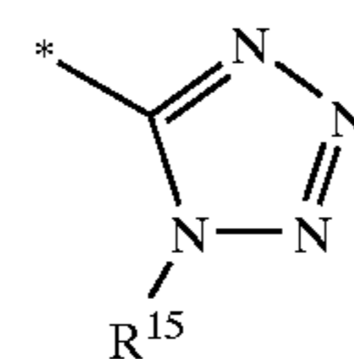
tetrazol-5-yl
