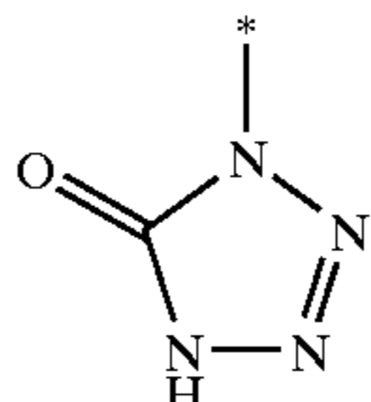
4,5-dihydro-5-oxo-1H-tetrazol-1-yl
