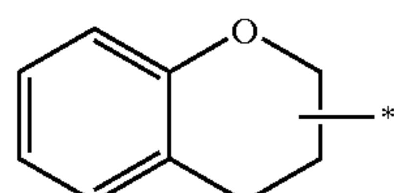
chromanyl
