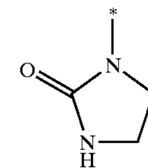
imidazolidin-2-on-1-yl
