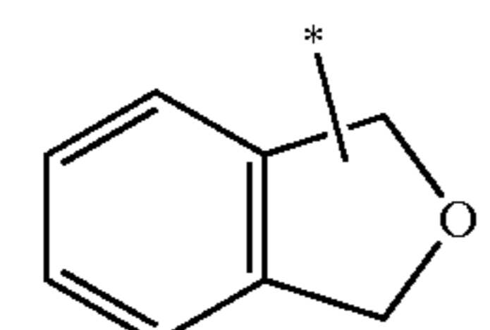
1,3-dihydroisobenzofuranyl; phthalanyl
