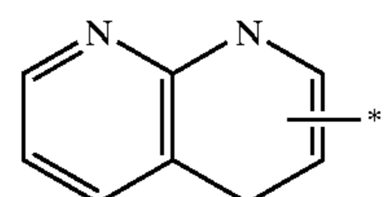
1,8-naphthyridinyl
