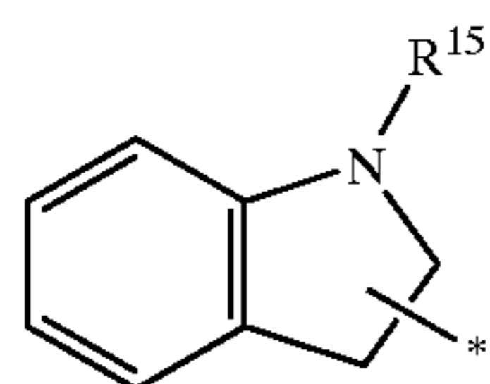
indolinyl
