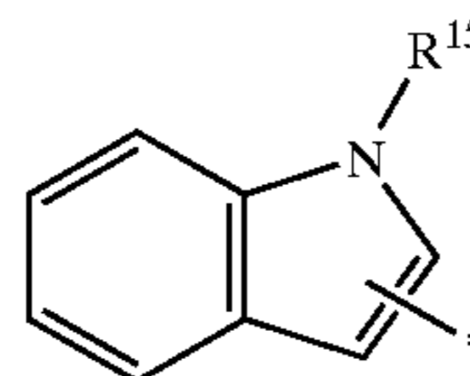
indoyl
