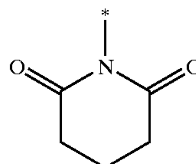
glutarimid-1-yl
