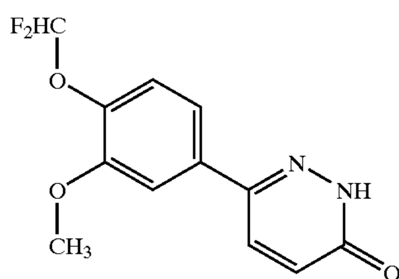
Zardaverine
