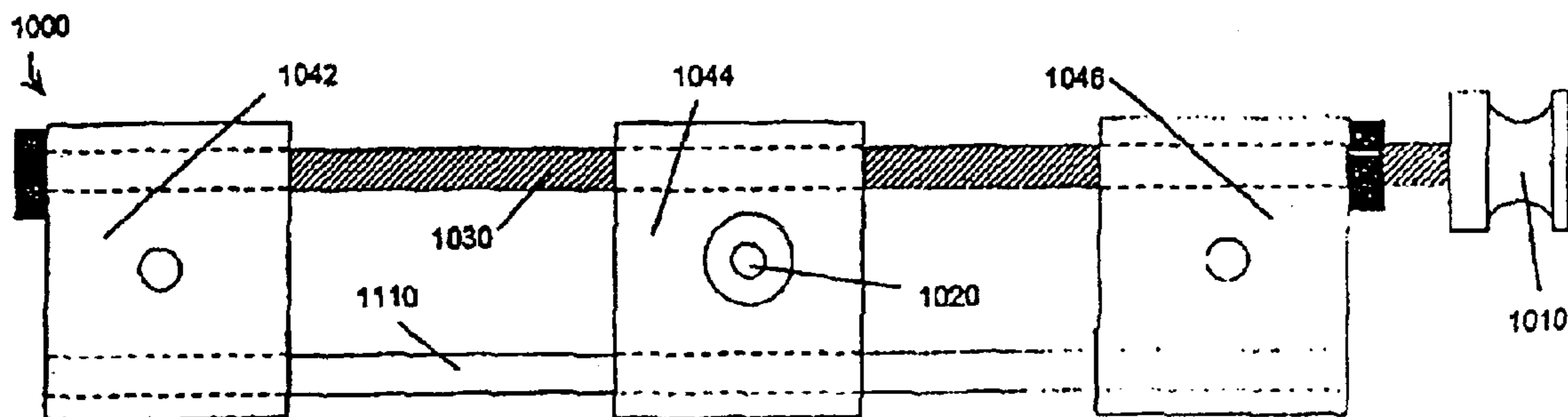
HOPPER ADJUSTMENT ASSEMBLY TOP VIEW
