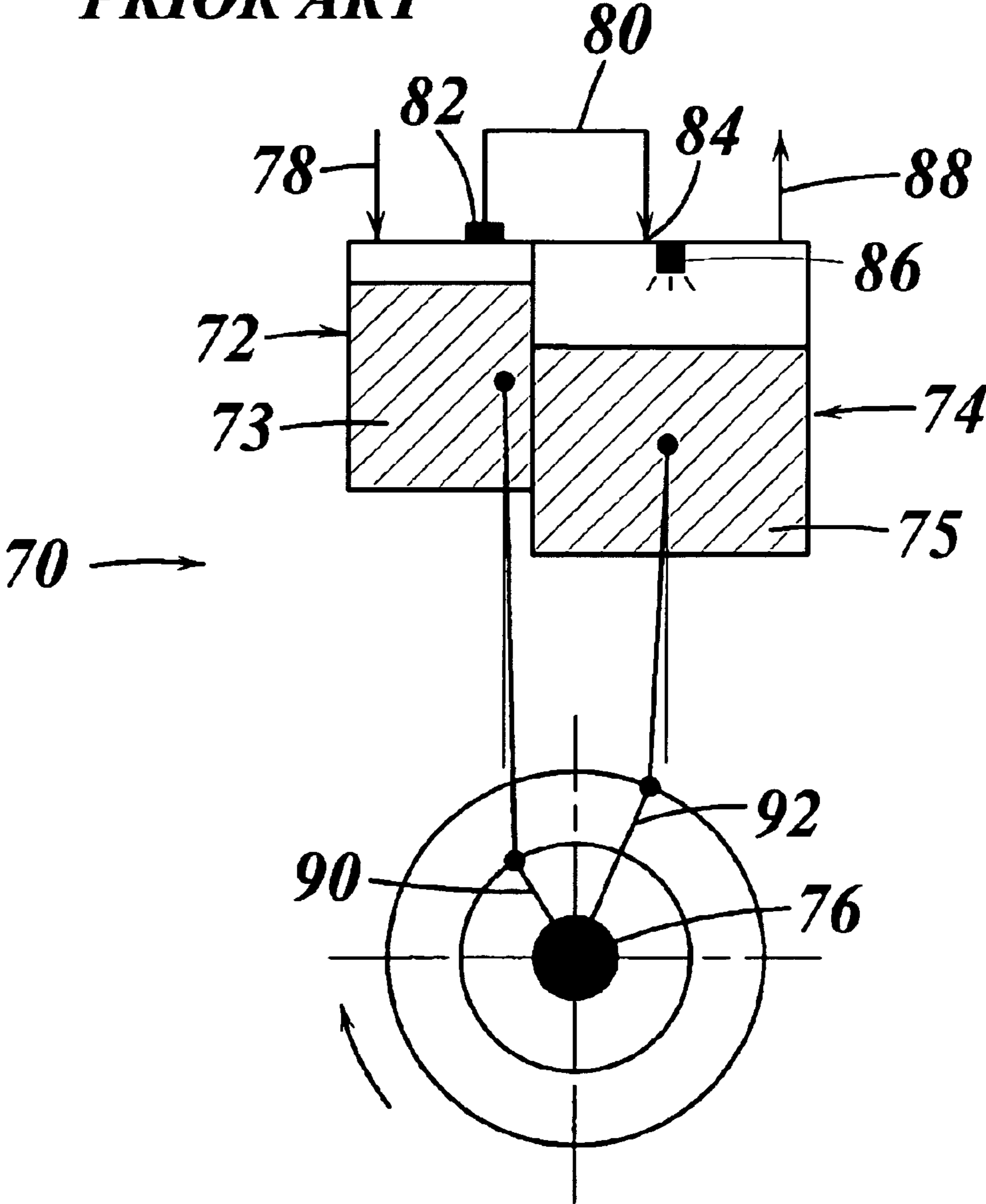
FIG. 5 PRIOR ART
