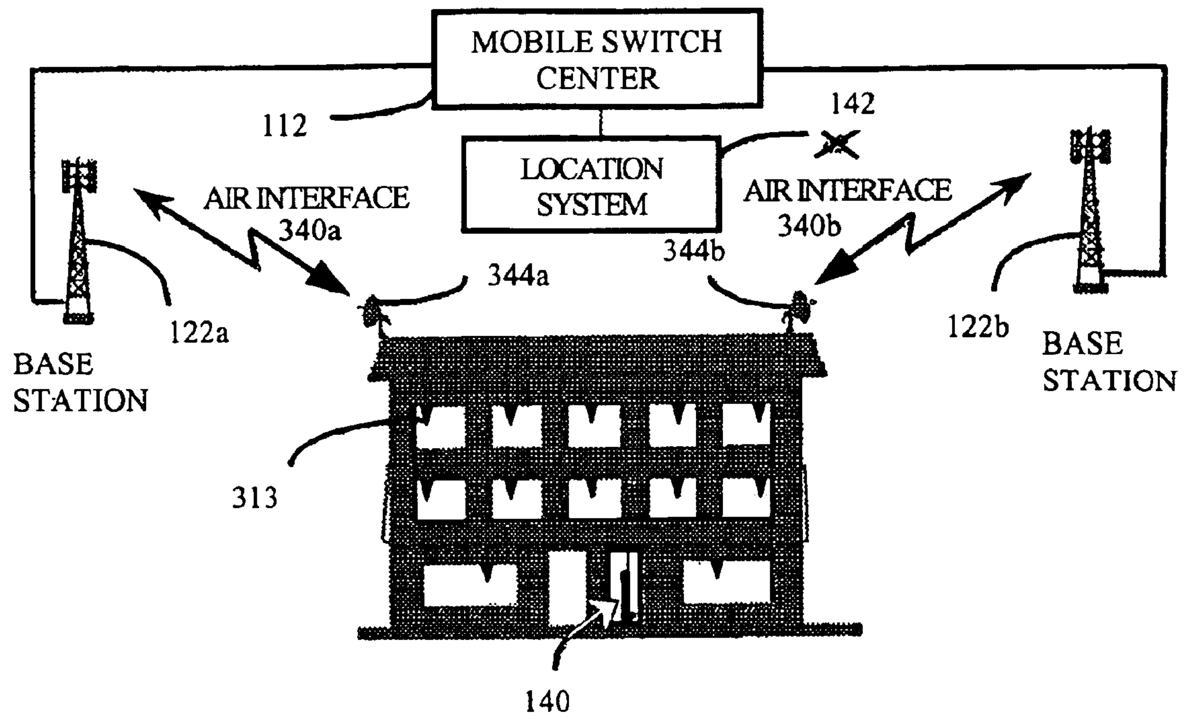
FIG. 11: Dual-Microwave Access Distributed Antenna Example
