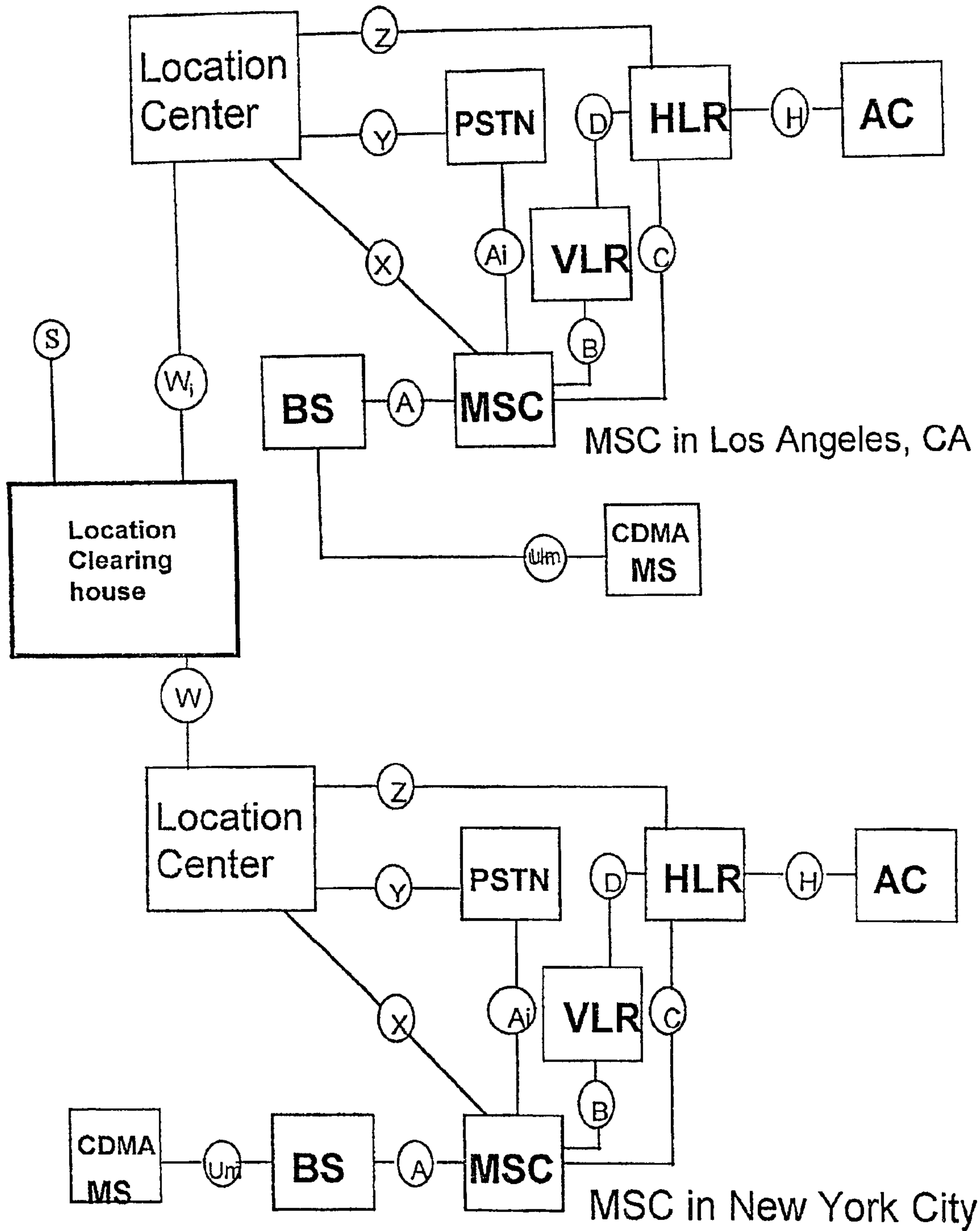
Figure 25: National Location Clearinghouse Structure
