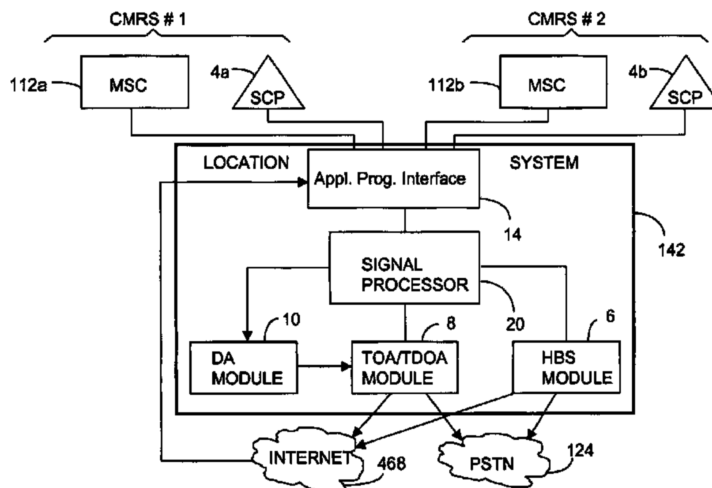
WIRELESS LOCATION USING MULTIPLE CMRSs
