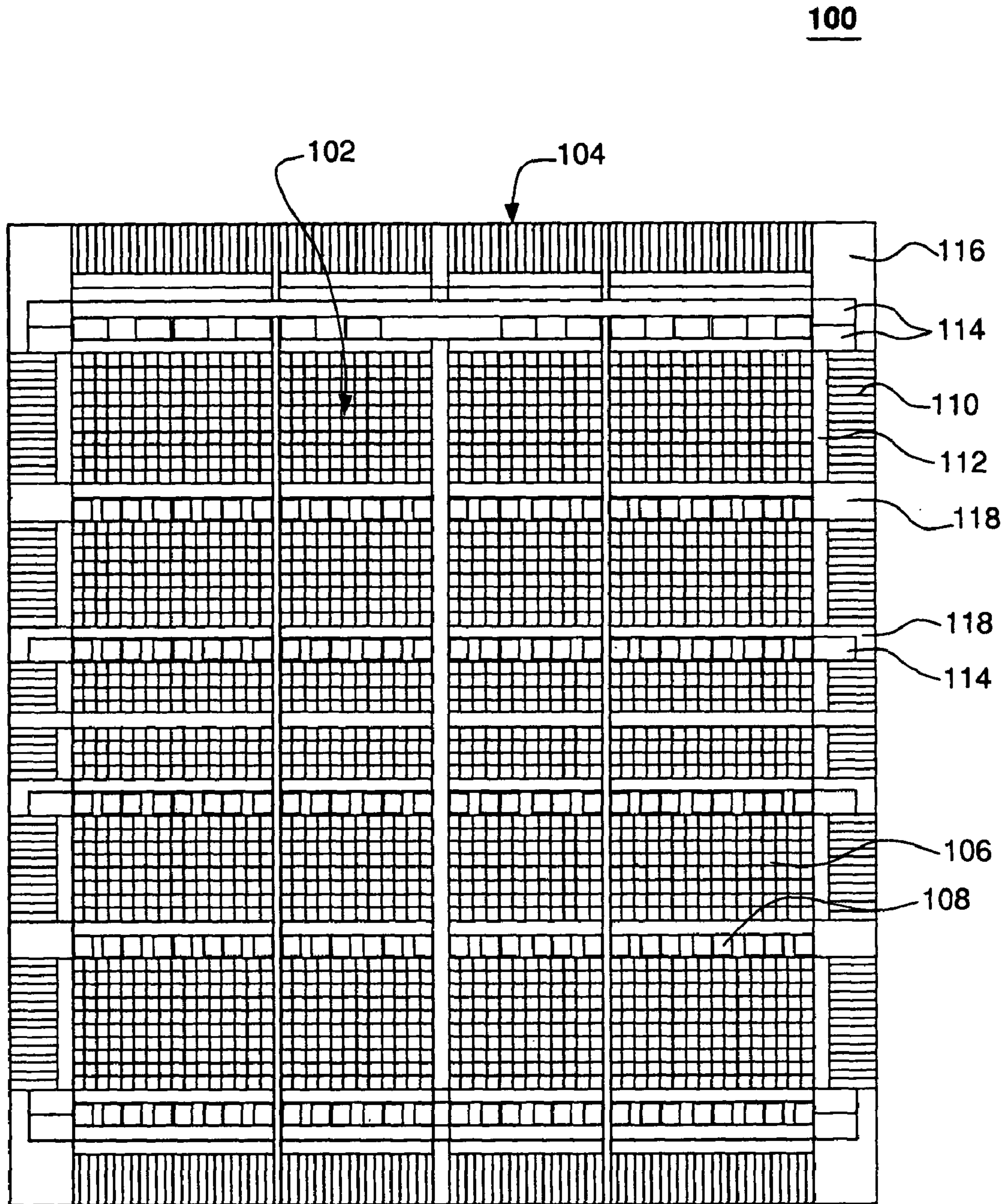
FIG. 1 (PRIOR ART)
