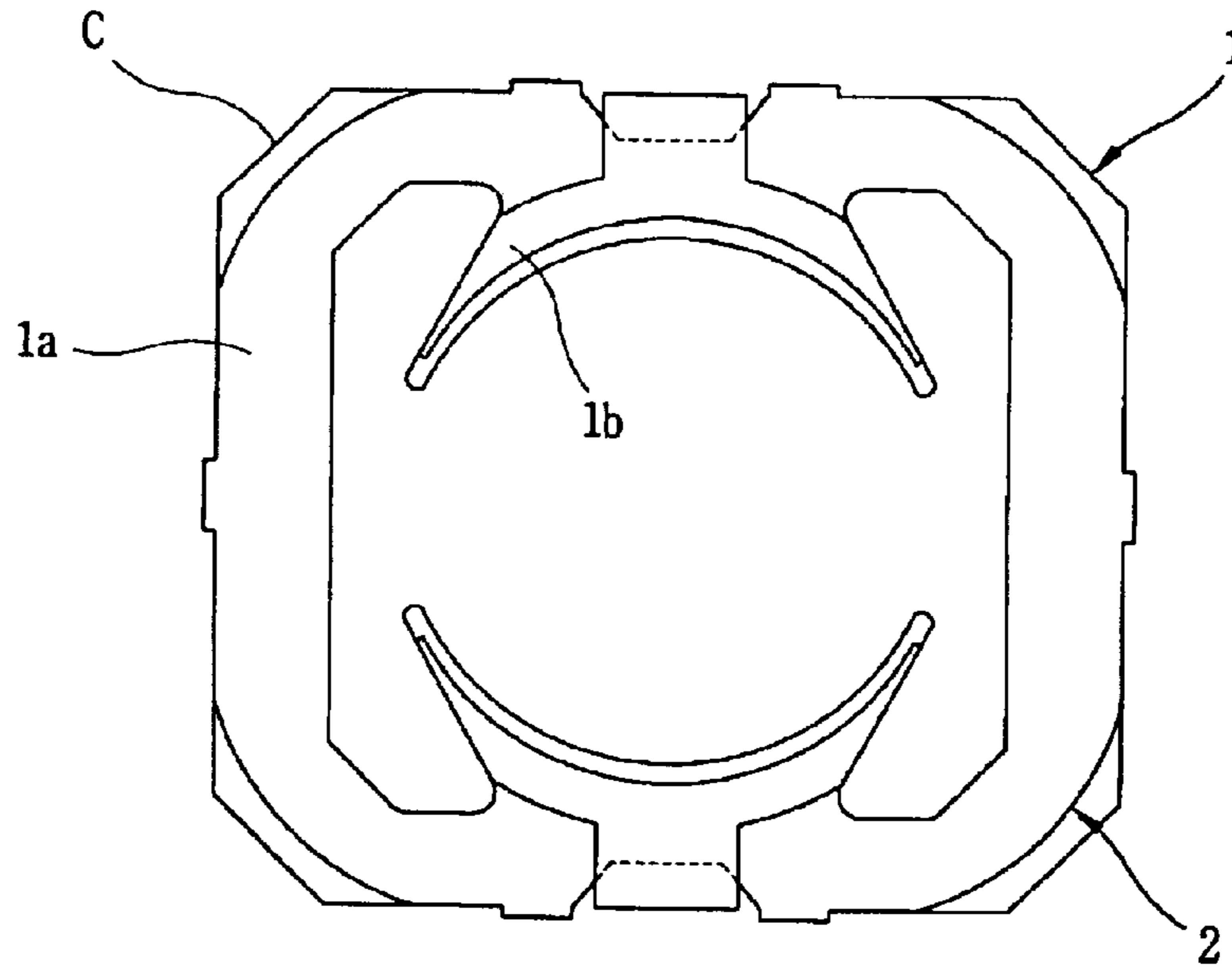
FIG. 2 CONVENTIONAL ART
