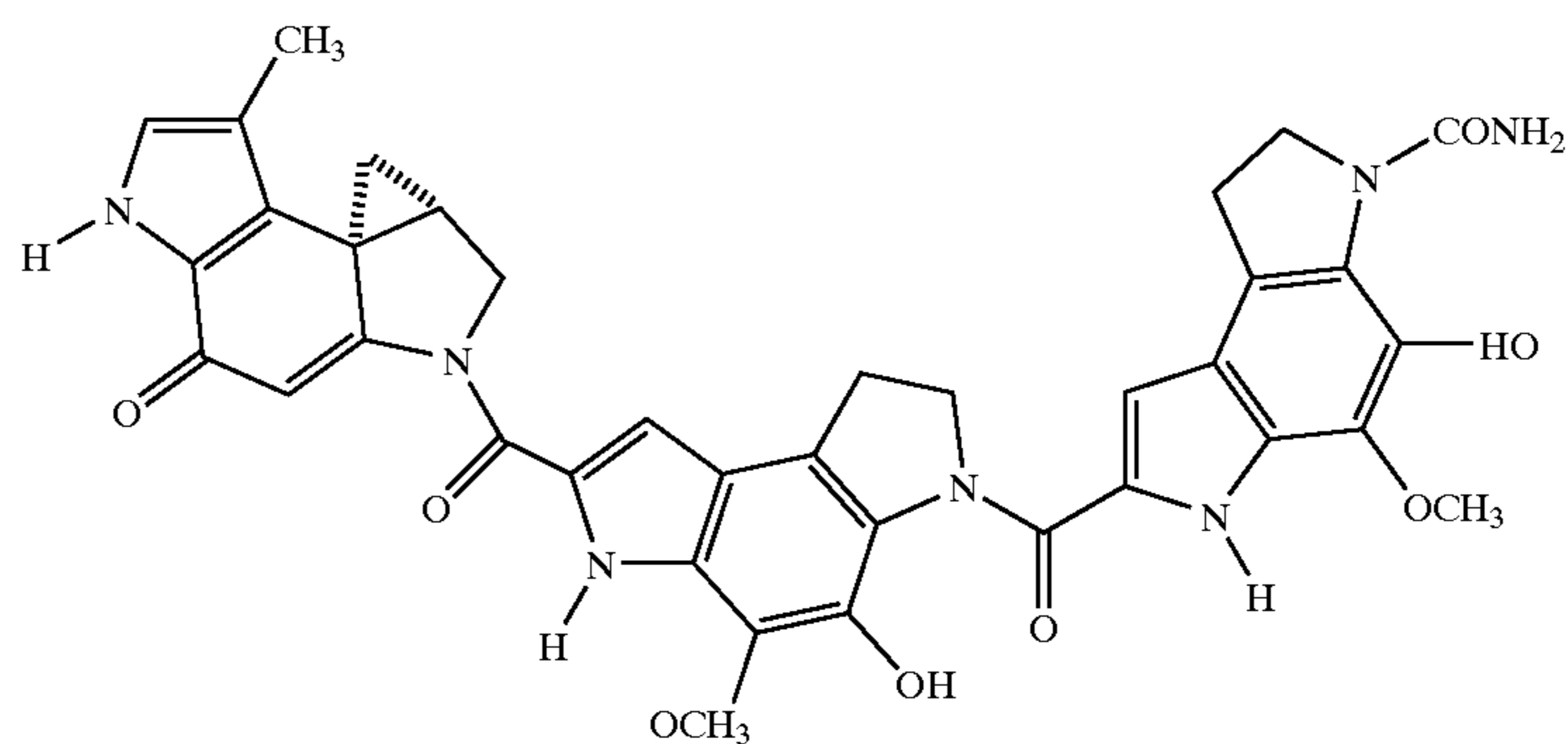
CC-1065
