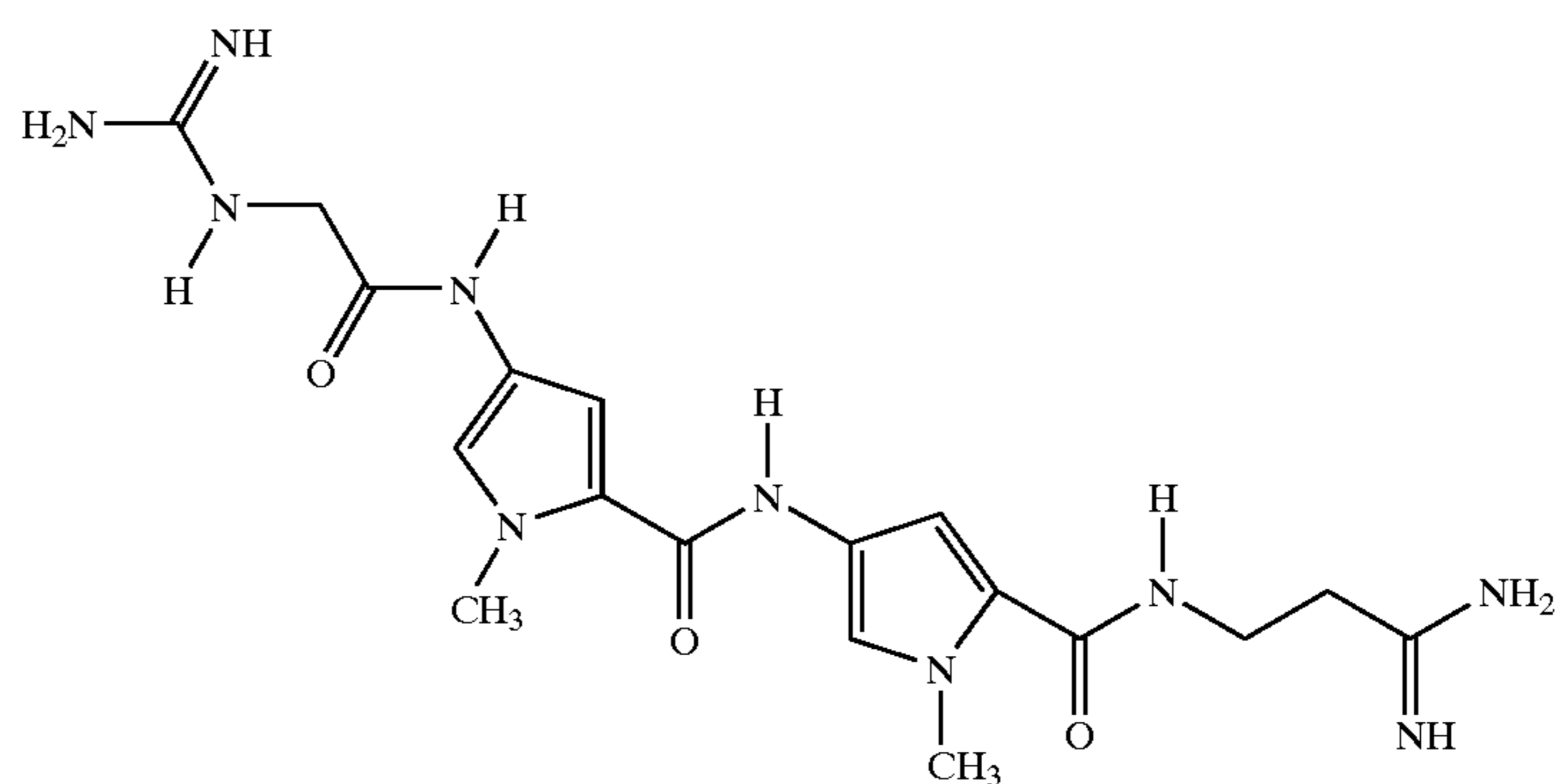
Netropsin
