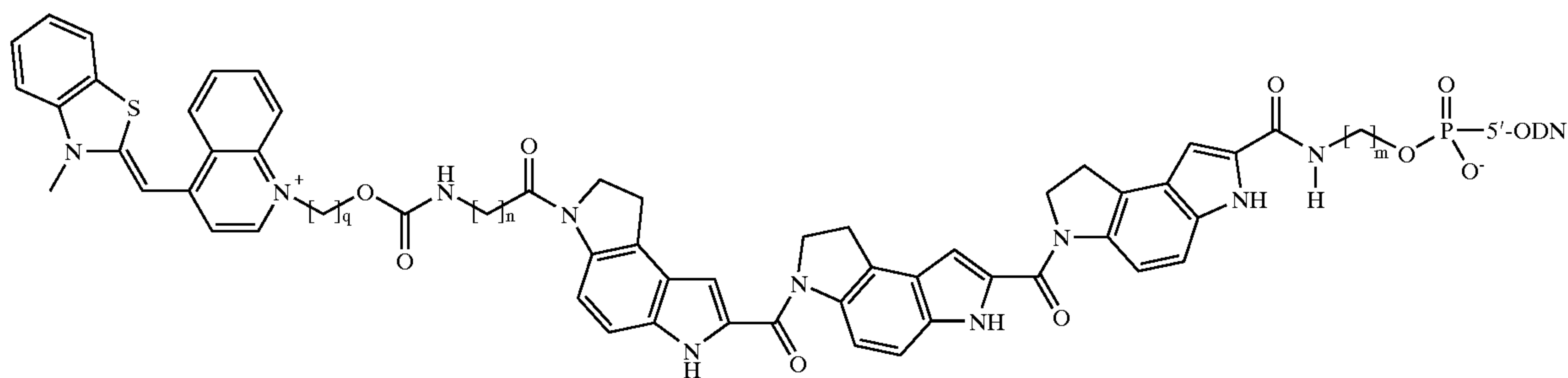
Formula 12
