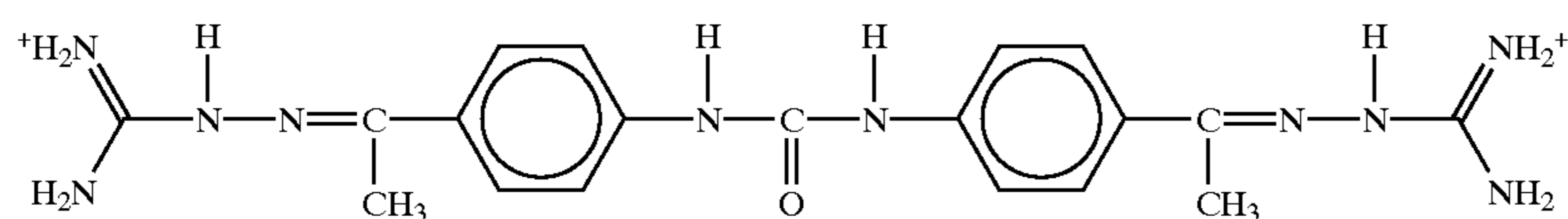
DDUG
