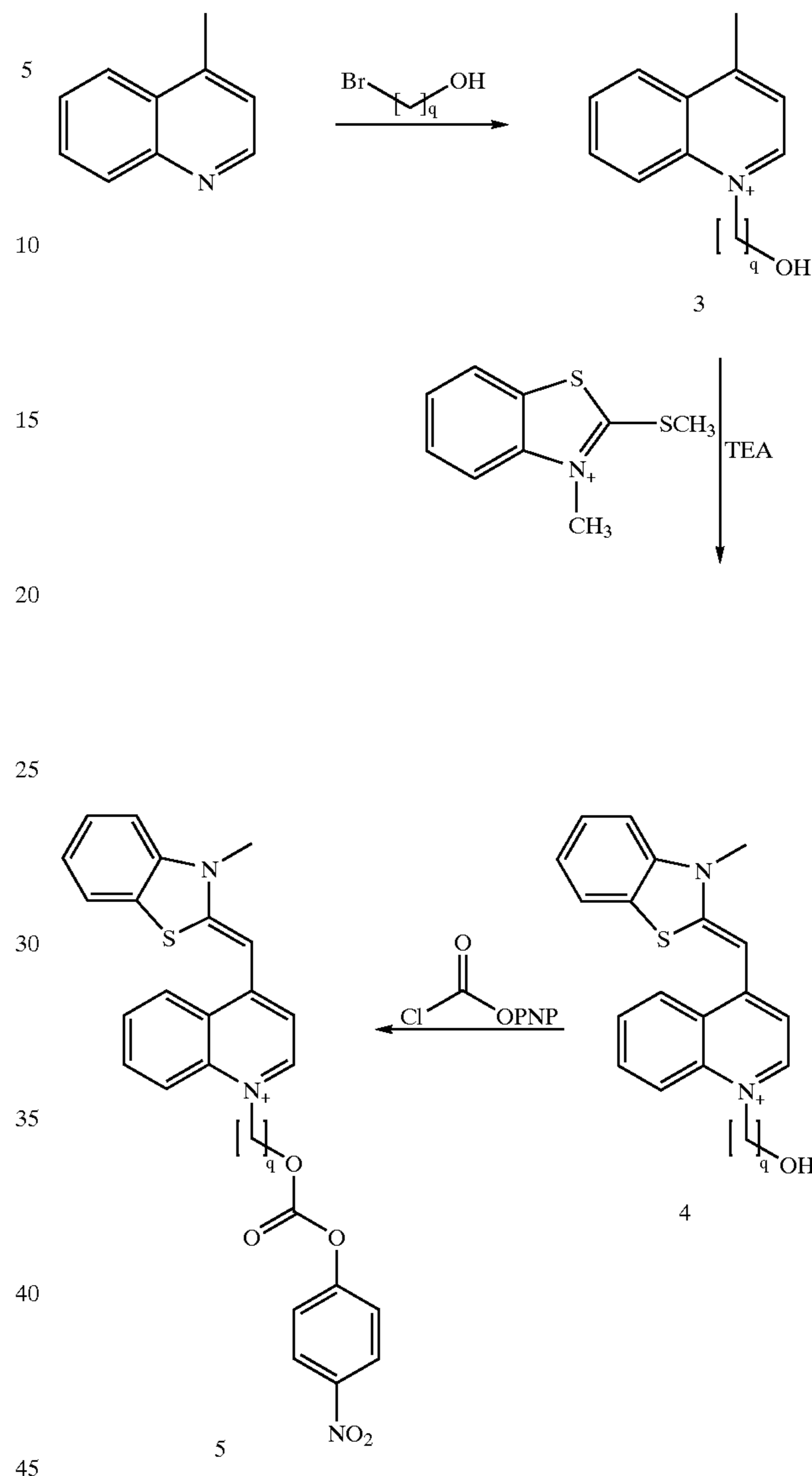
Reaction Scheme 3
