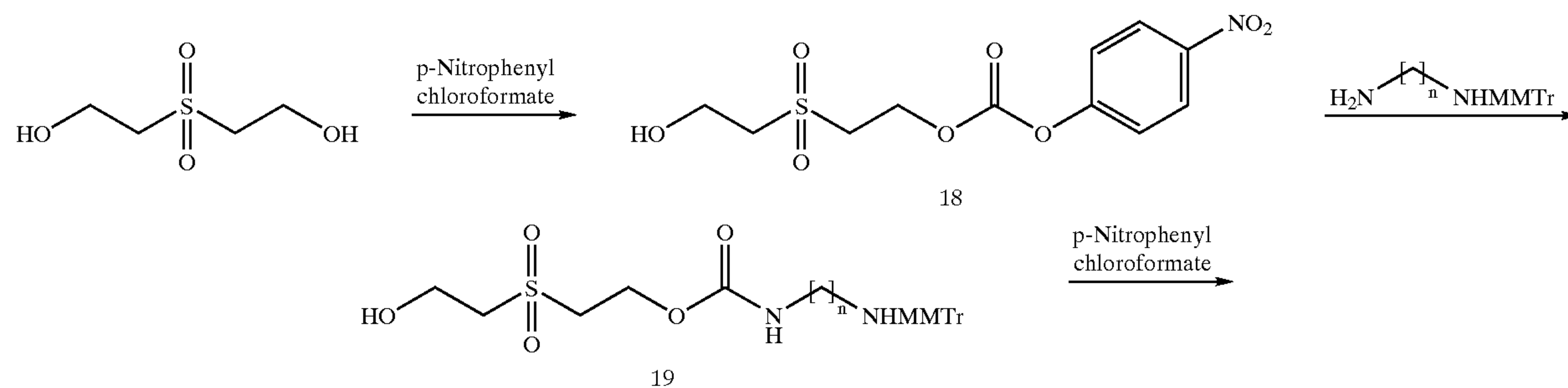
Reaction Scheme 7
