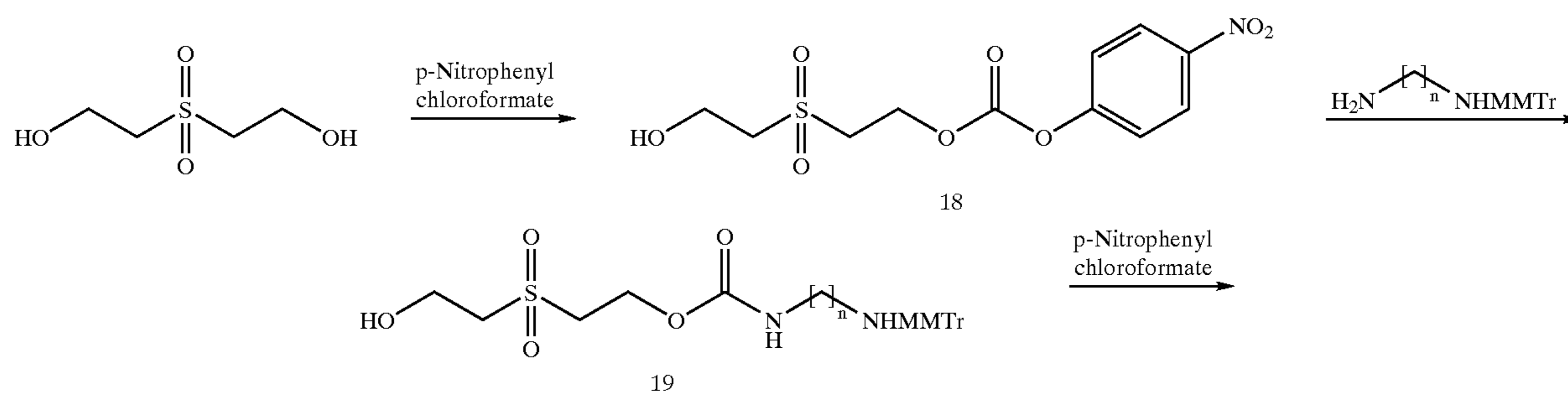
Reaction Scheme 7
