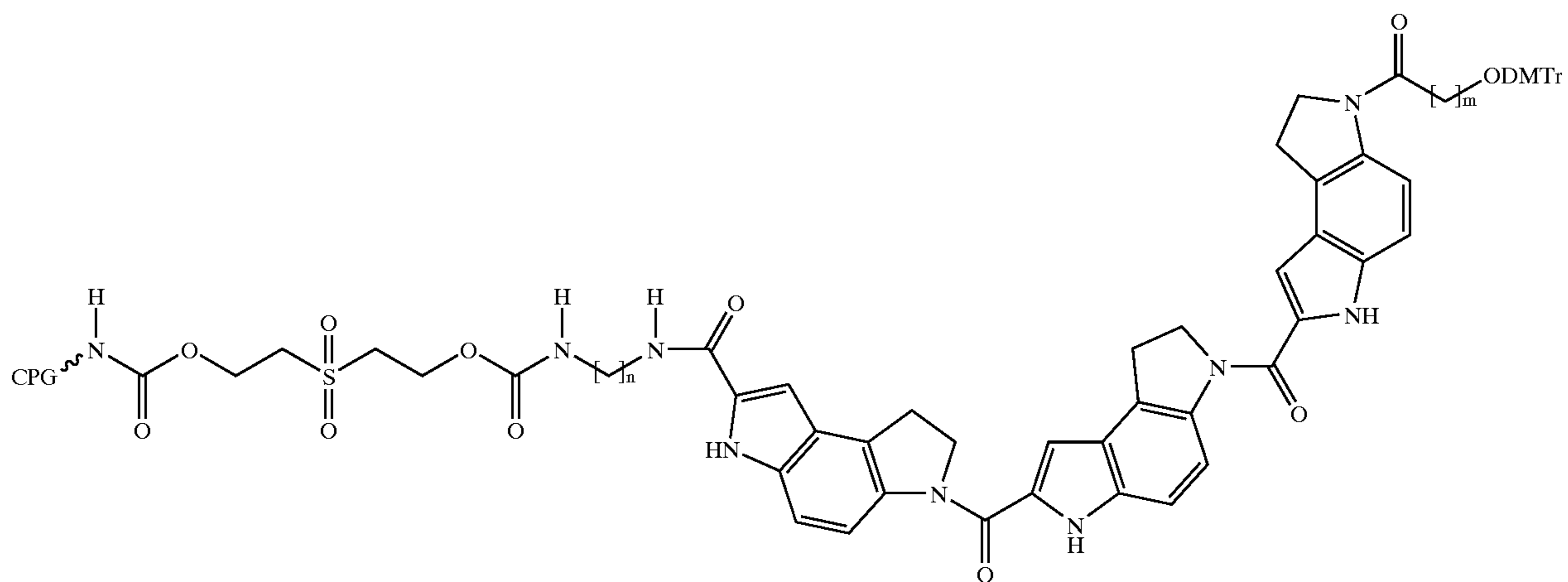
Reaction Scheme 6
