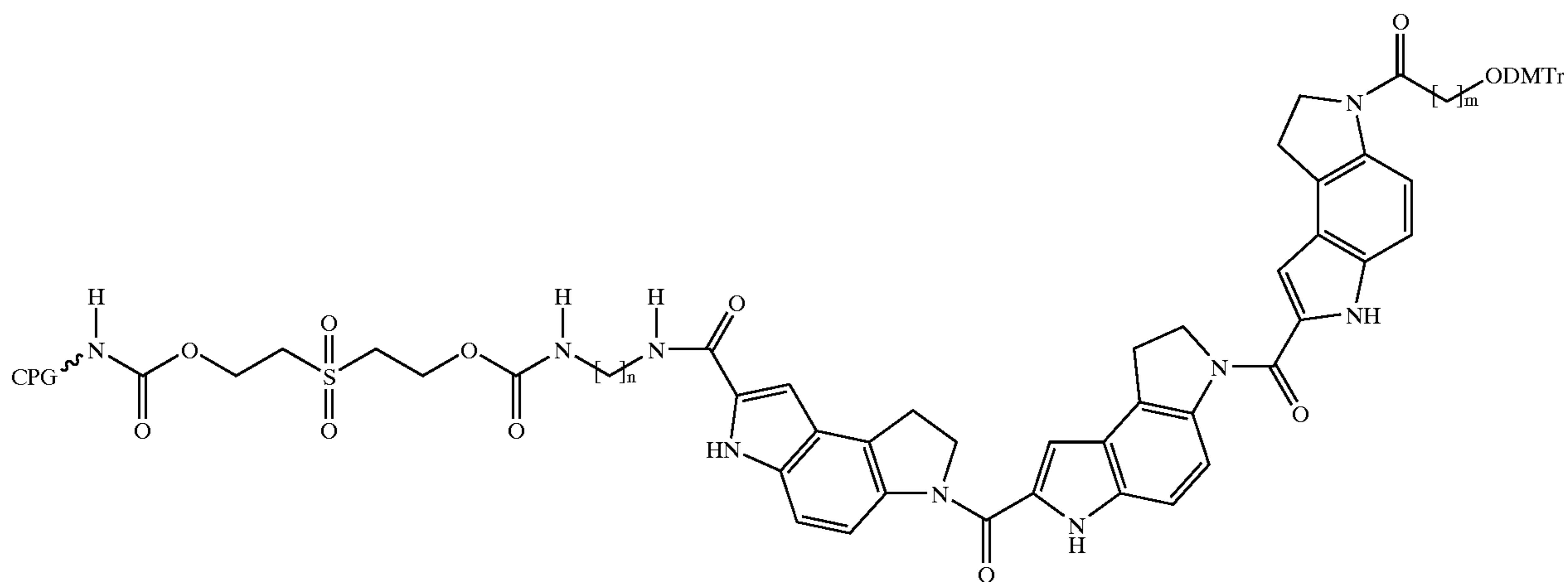
Reaction Scheme 6
