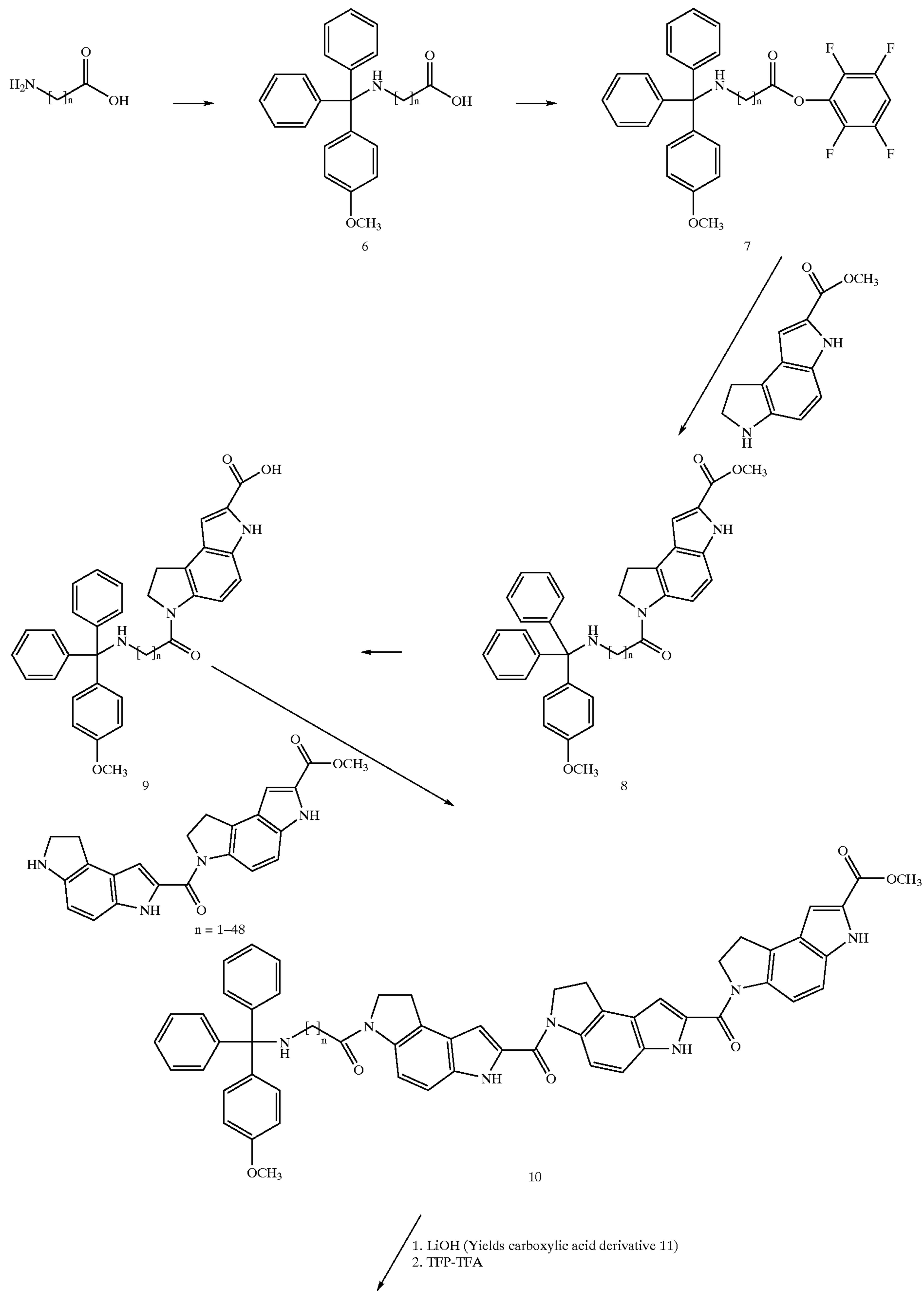
Reaction Scheme 4
