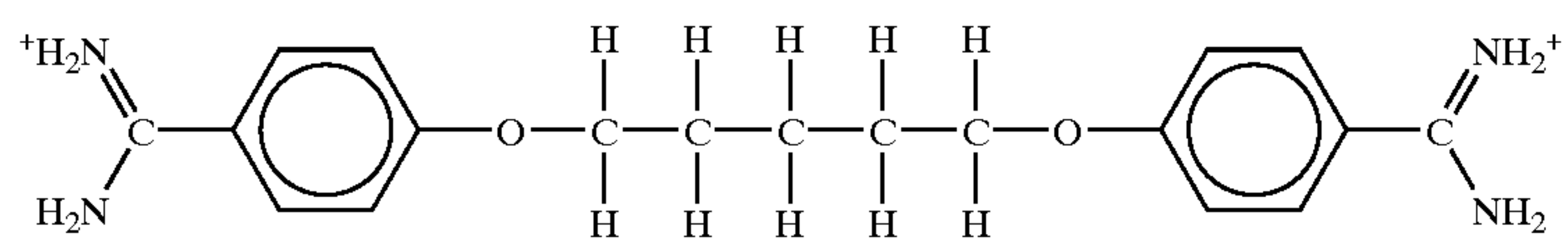
Pentamidine
