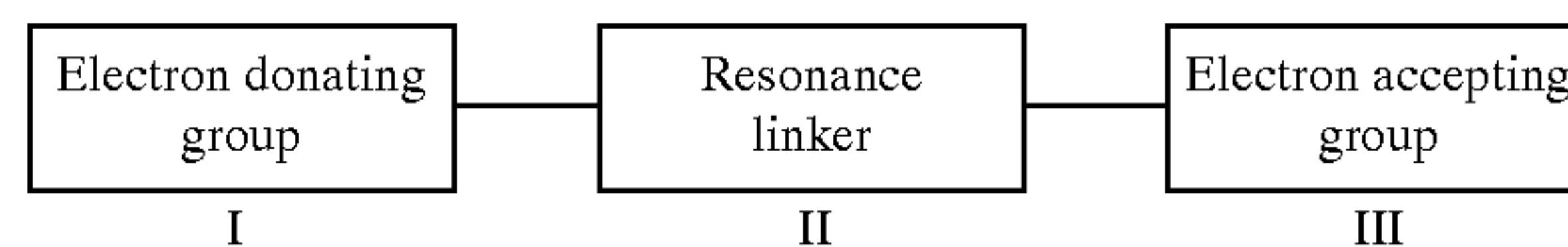
Formula 10
