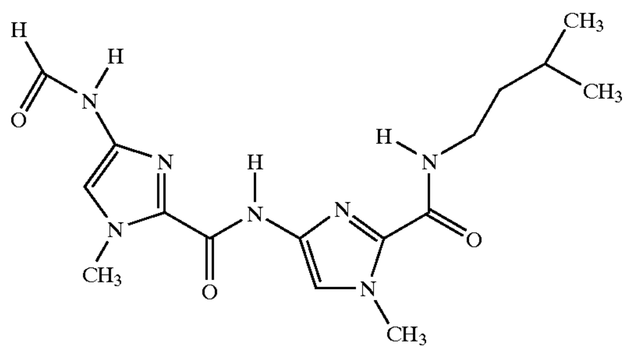
Lexitropsin
