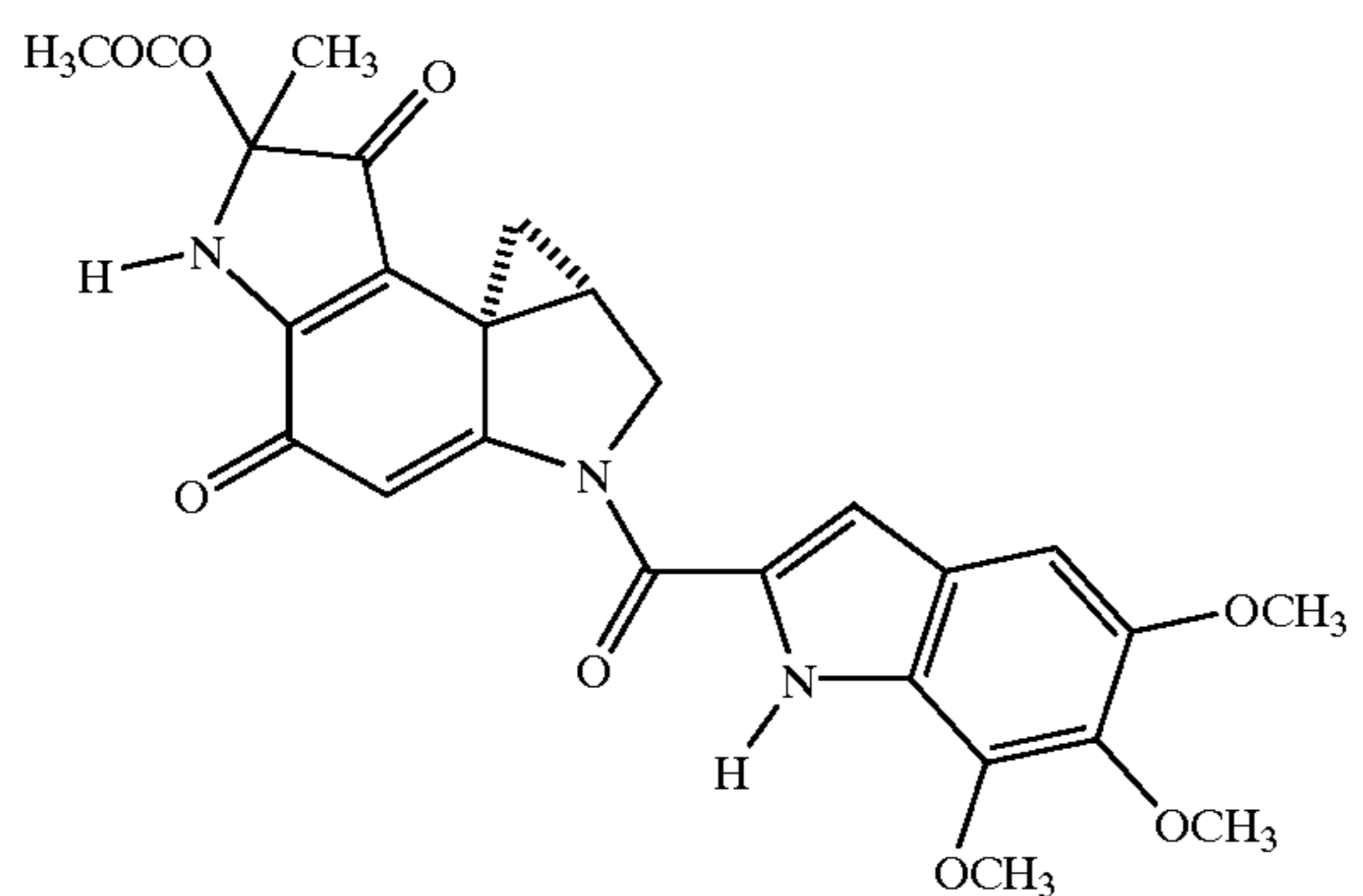
Duocarmycin A
