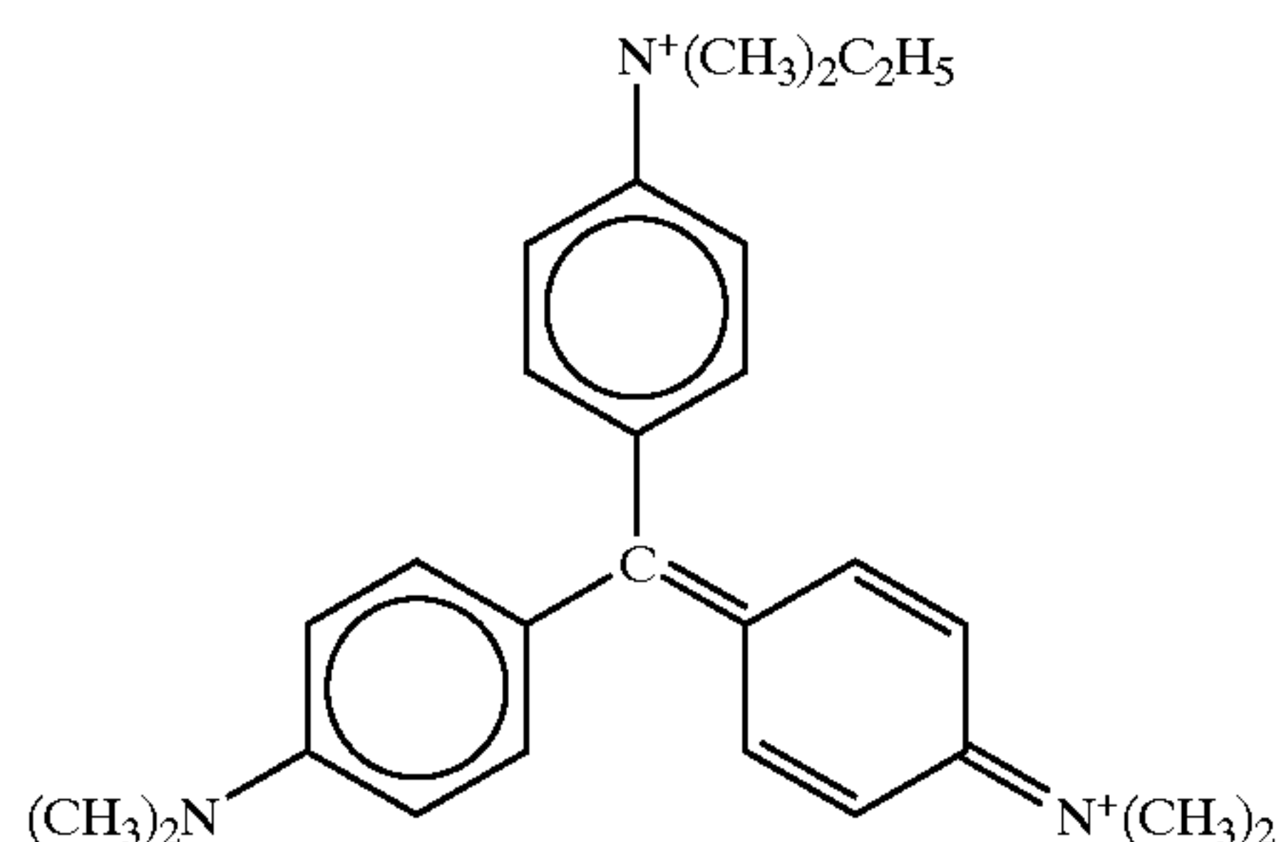
Methyl Green
