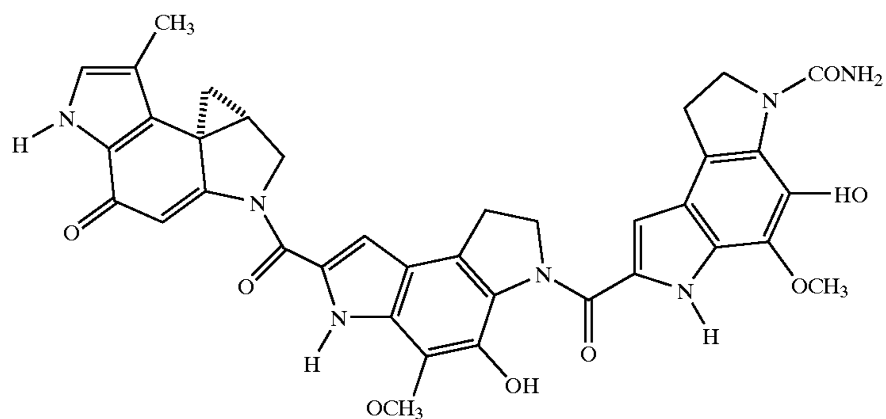
CC-1065
