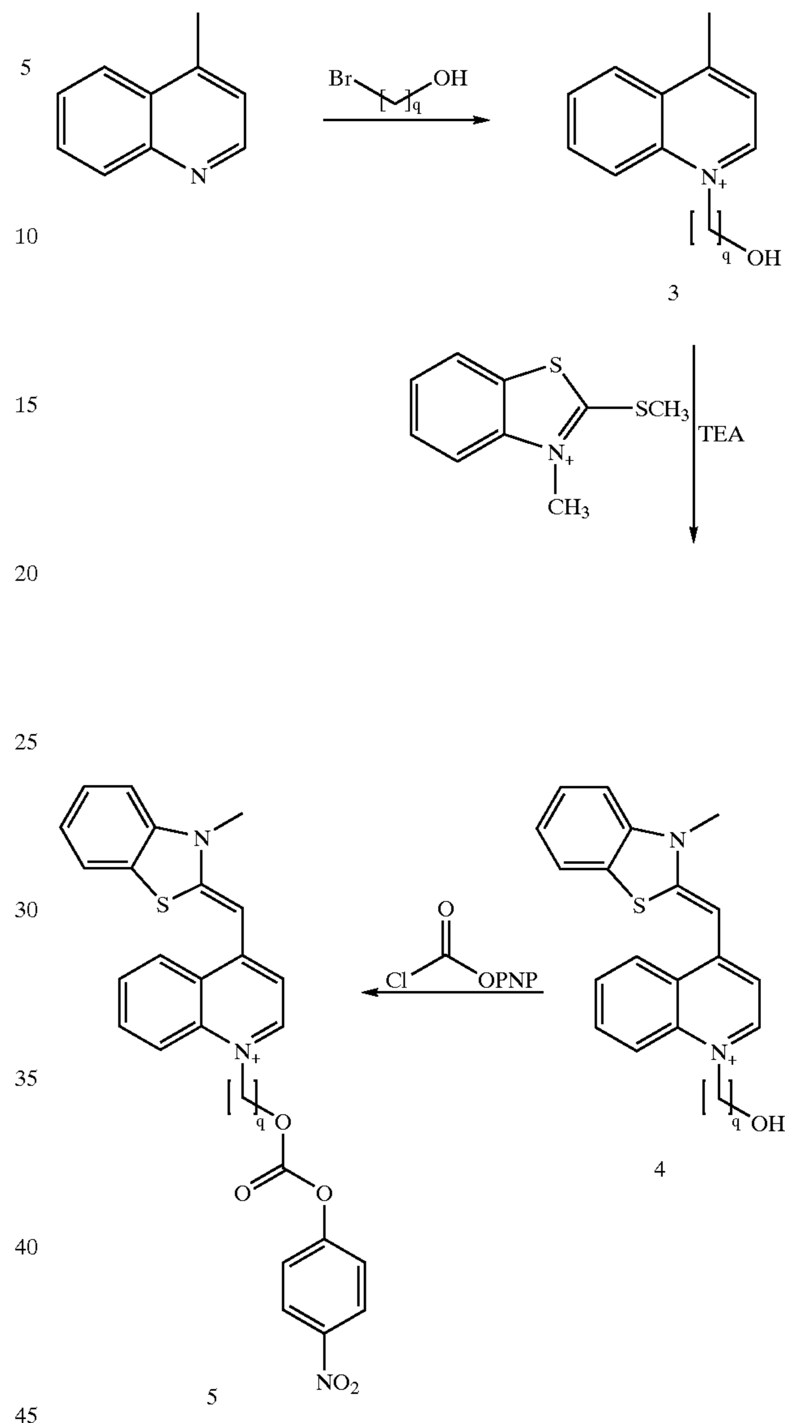
Reaction Scheme 3
