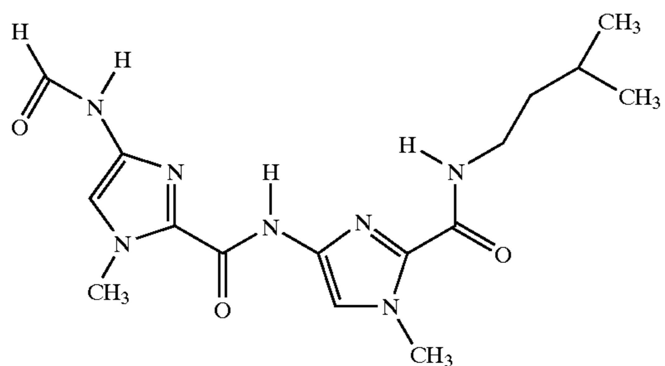
Lexitropsin
