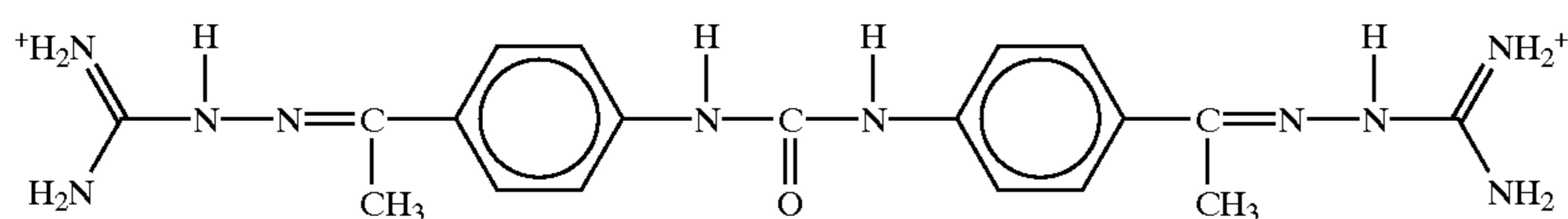
DDUG
