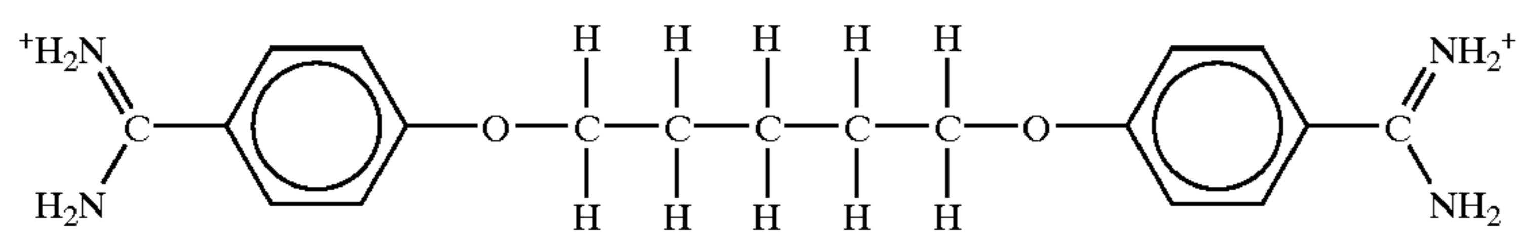
Pentamidine
