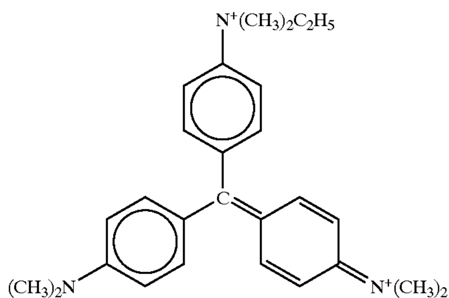
Methyl Green
