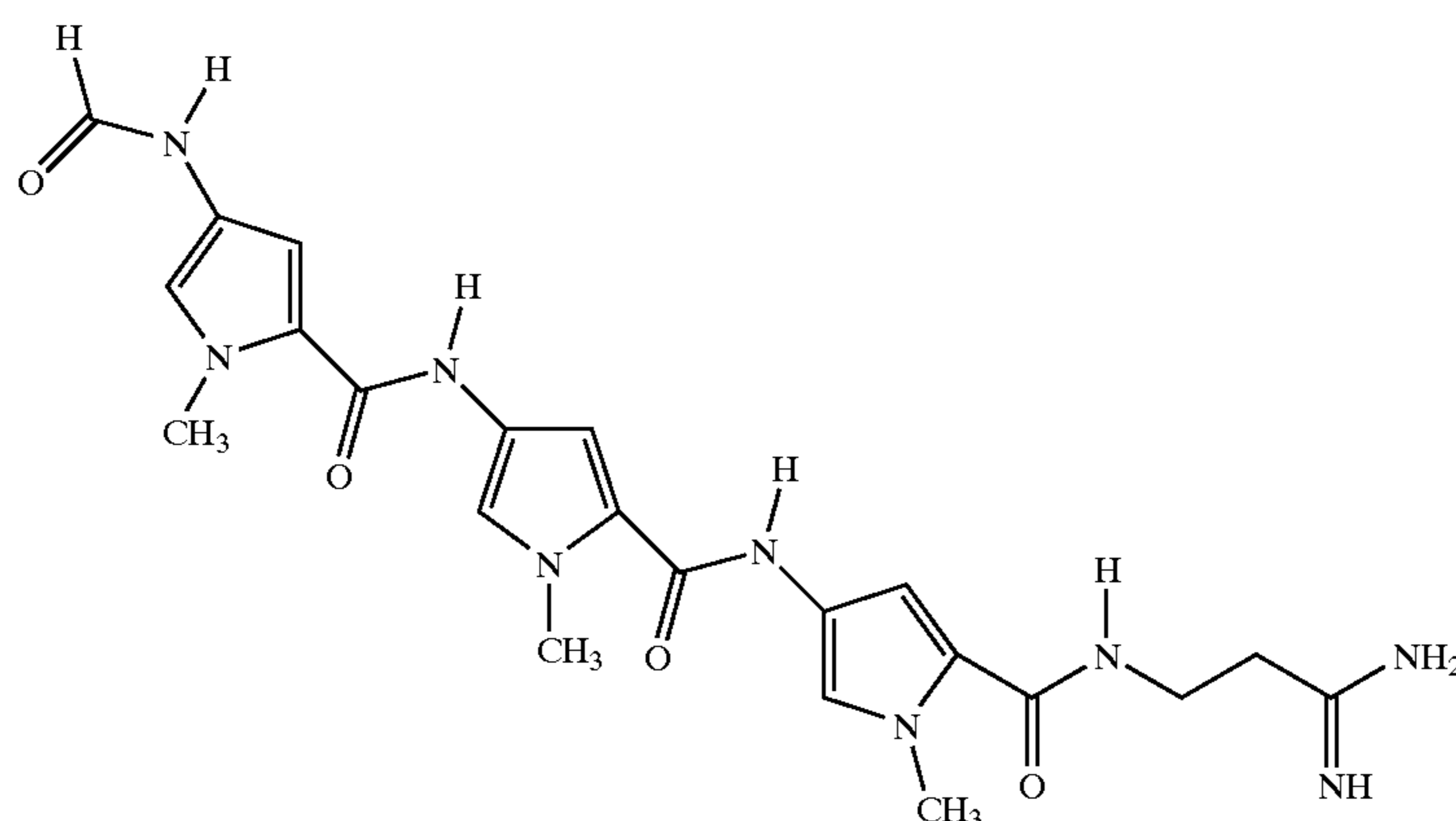
Distamycin
