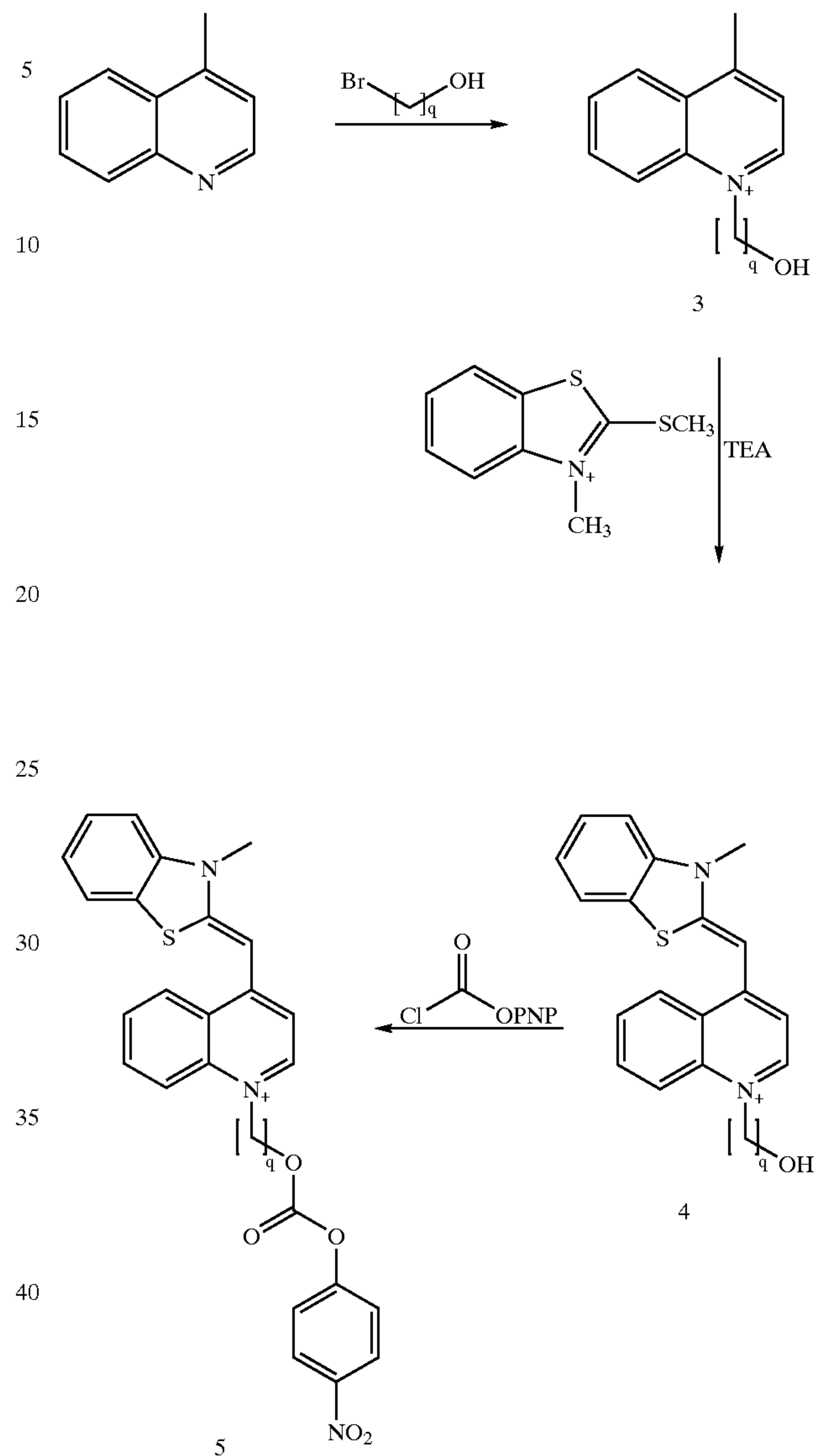
Reaction Scheme 3
