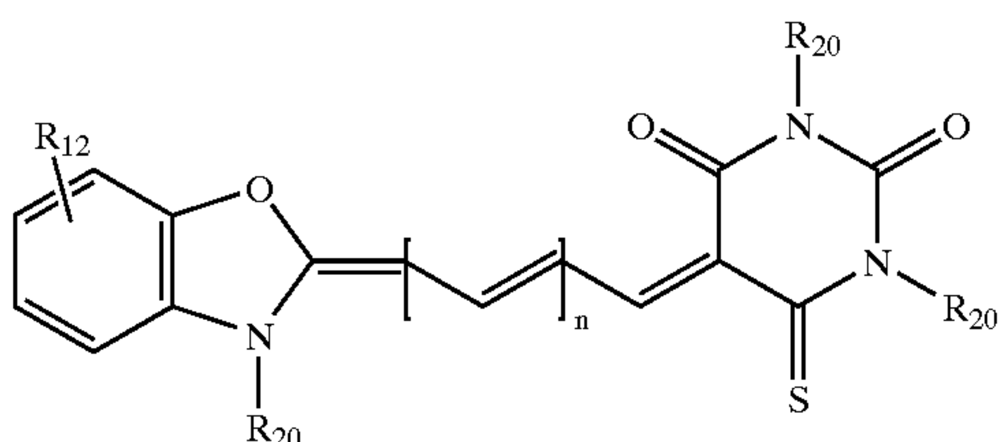
Formula 10
