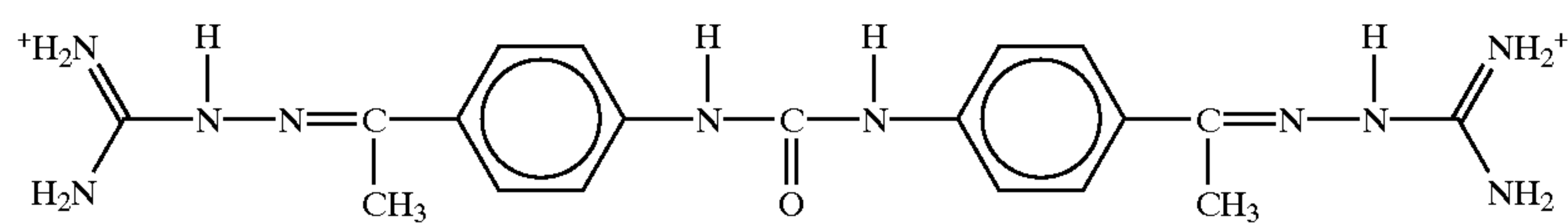
DDUG
