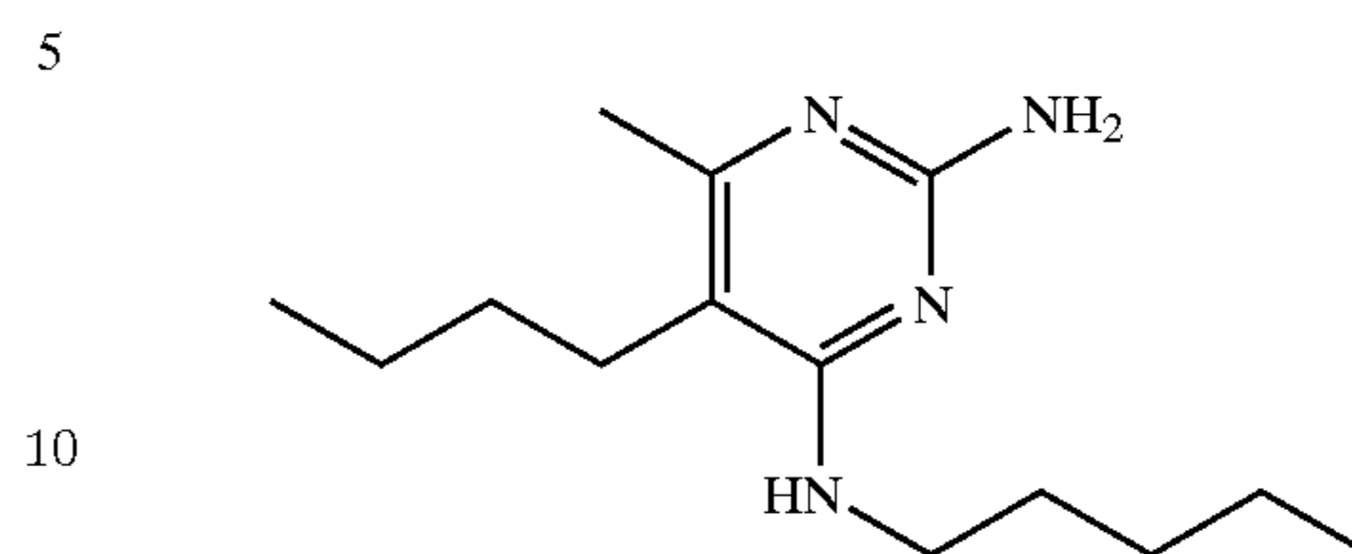
N-(2-Amino-5-butyl-6-methylpyrimidine-4-yl)-N-pentylamine
