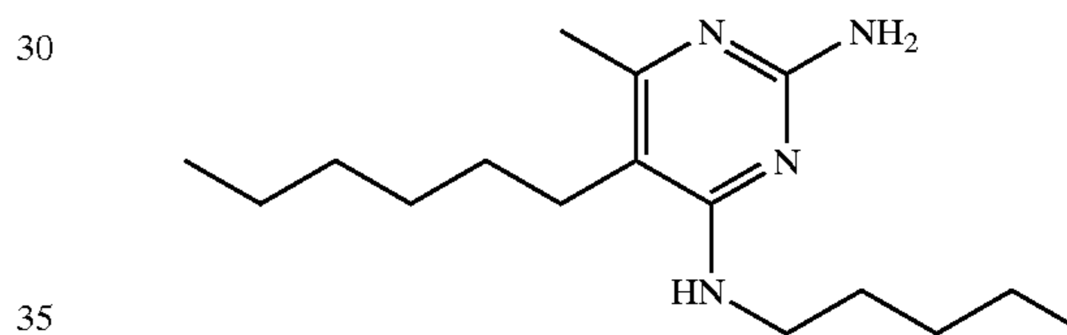
N-(2-Amino-5-hexyl-6-methylpyrimidine-4-yl)-N-pentylamine
