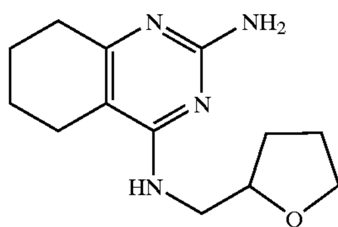
N-(2-Amino-5,6,7,8-tetrahydroquinazoline-4-yl)-N-(tetrahydrofuran-2-yl methyl)amine
