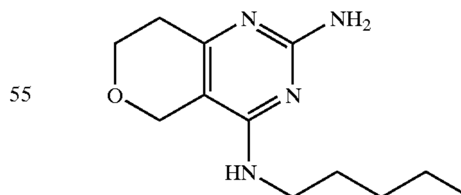
N-(2-Amino-7,8-dihydro-5H-pyrano[4,3-d]pyrimidine-4-yl)-N-pentylamine
