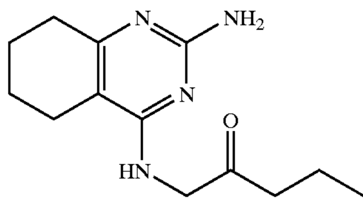
1-[(2-Amino-5,6,7,8-tetrahydroquinazoline-4-yl)amino]pentane-2-one
