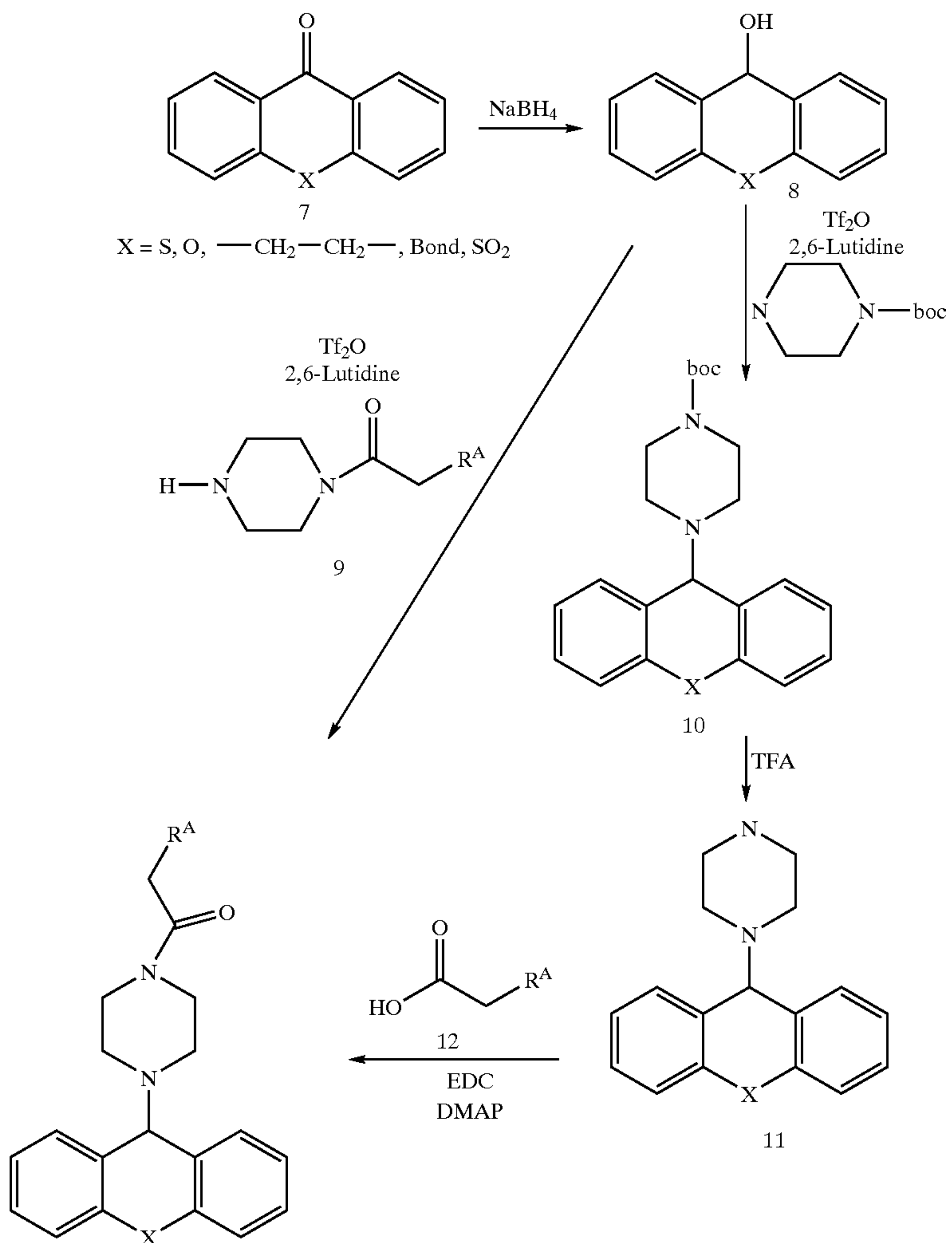
Reaction Scheme 2
