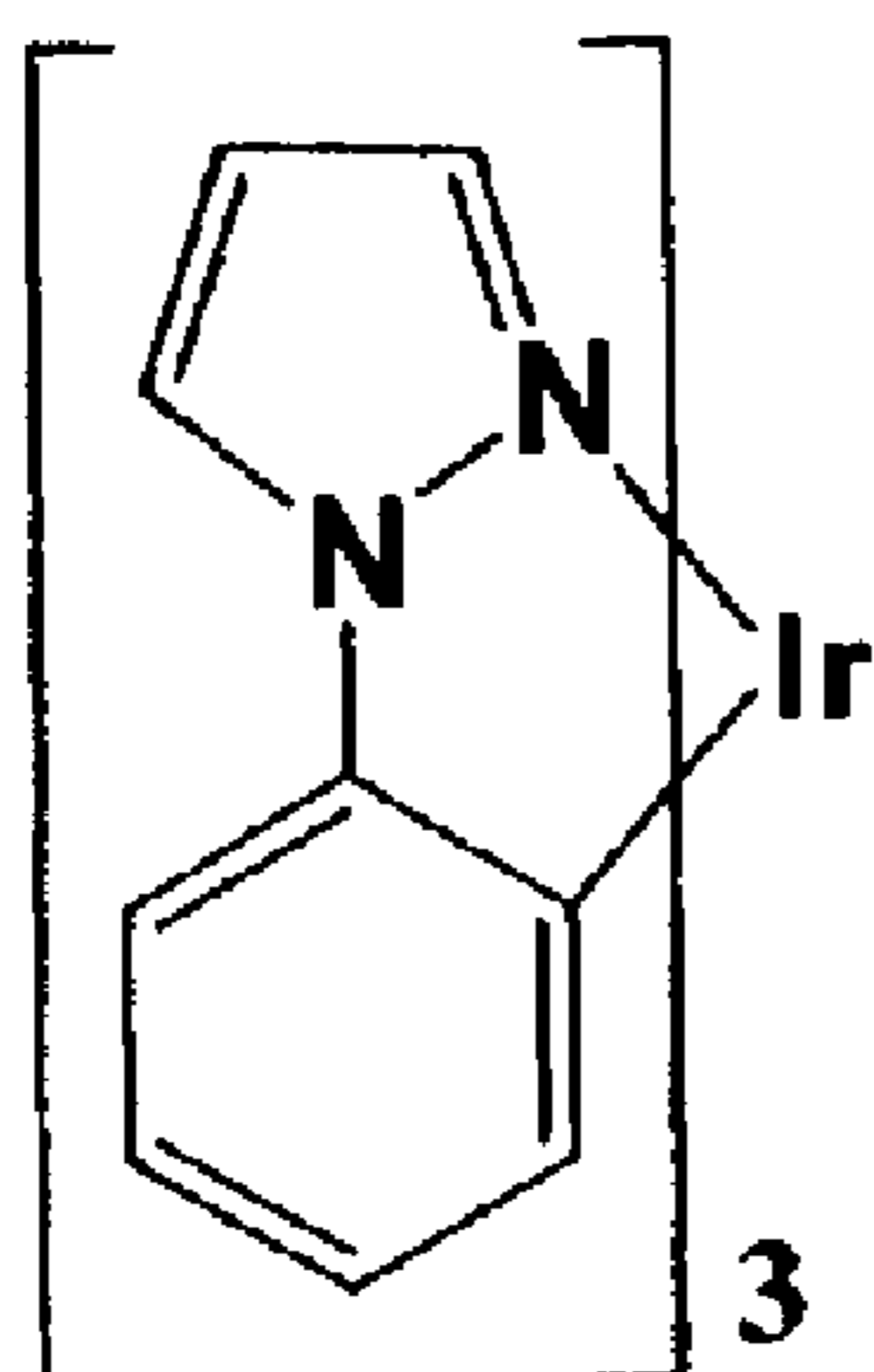
tris(phenylpyrazole) Iridium (Irppz)
