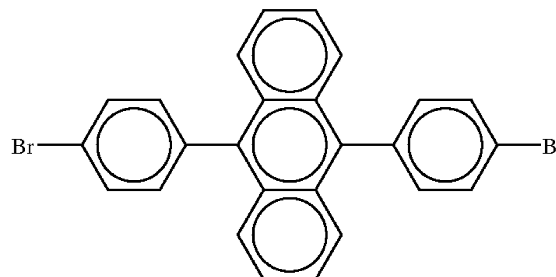
(Intermediate Compound B)
