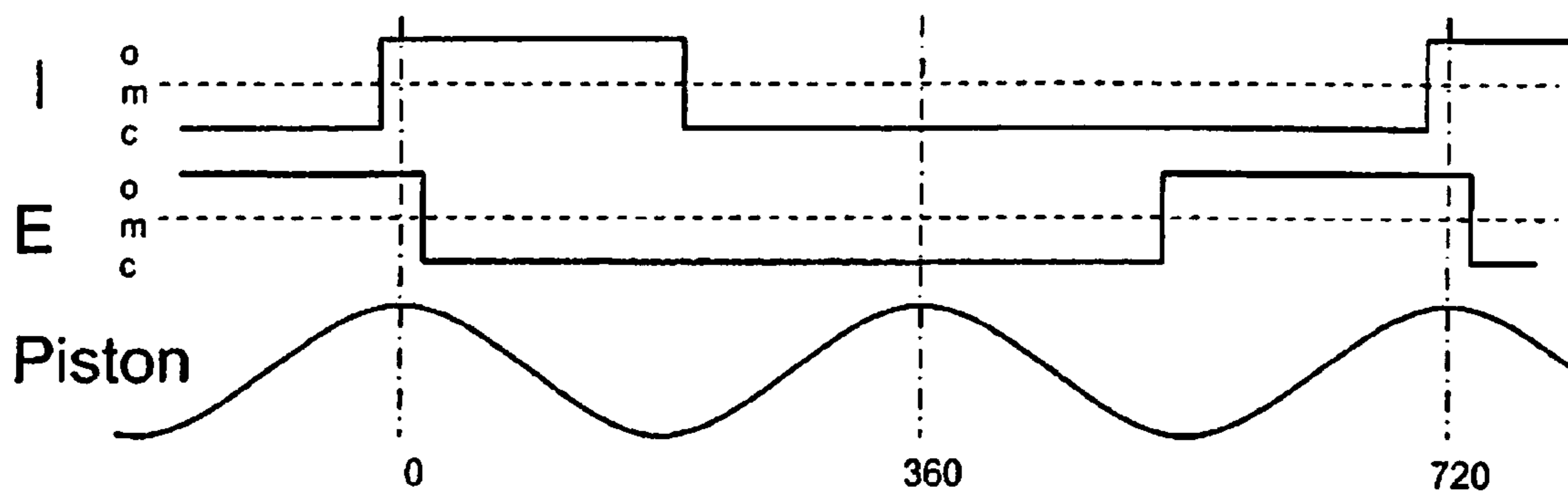
Fig. 19 Prior Art
