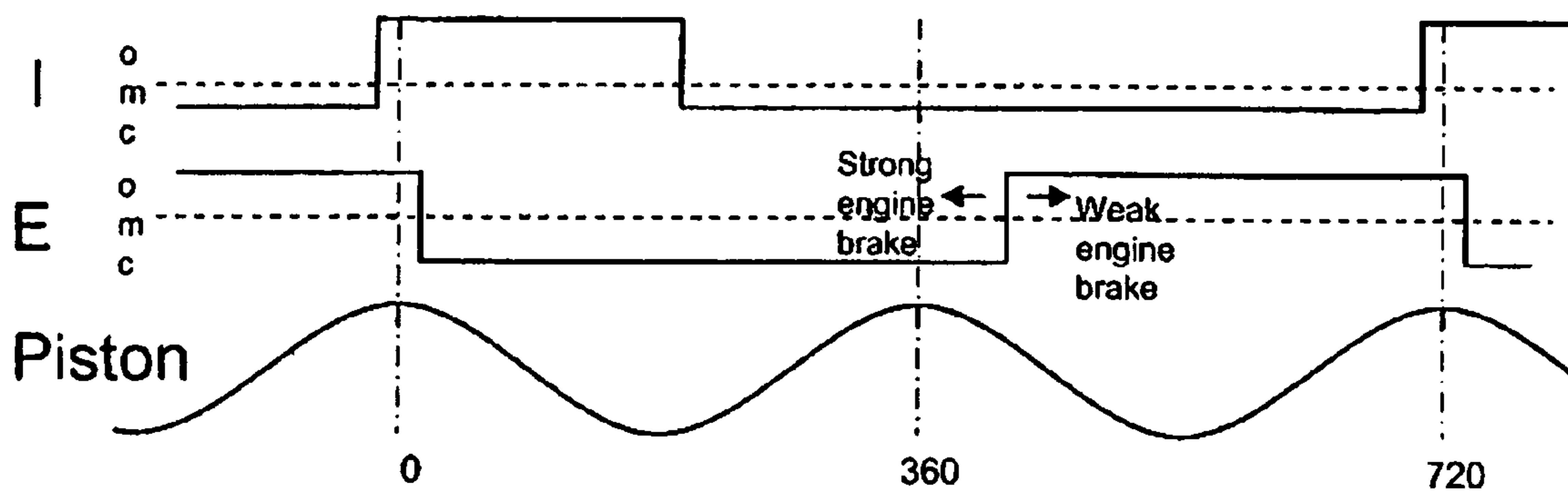
Fig. 20 Prior Art
