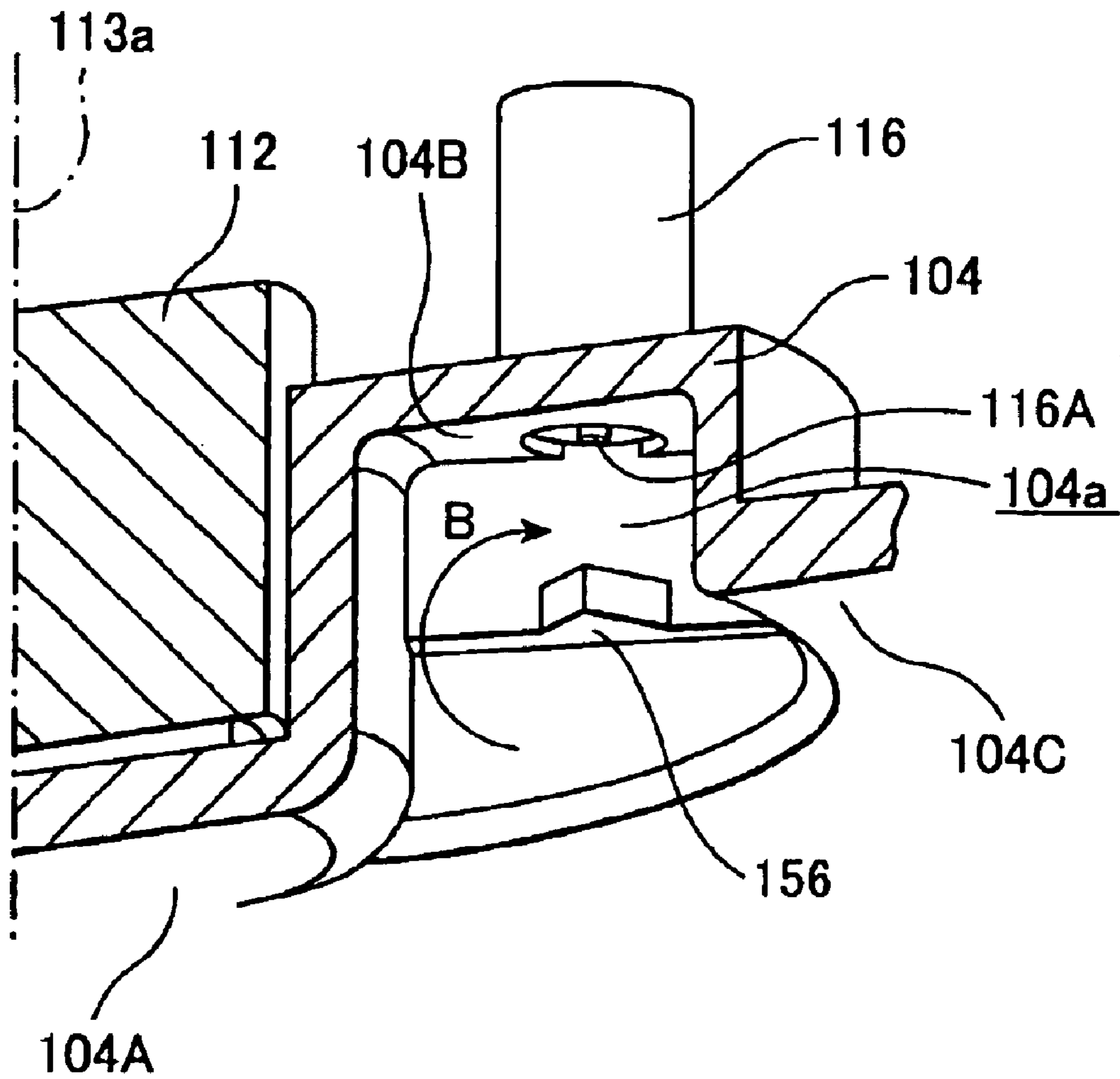
FIG. 4 PRIOR ART
