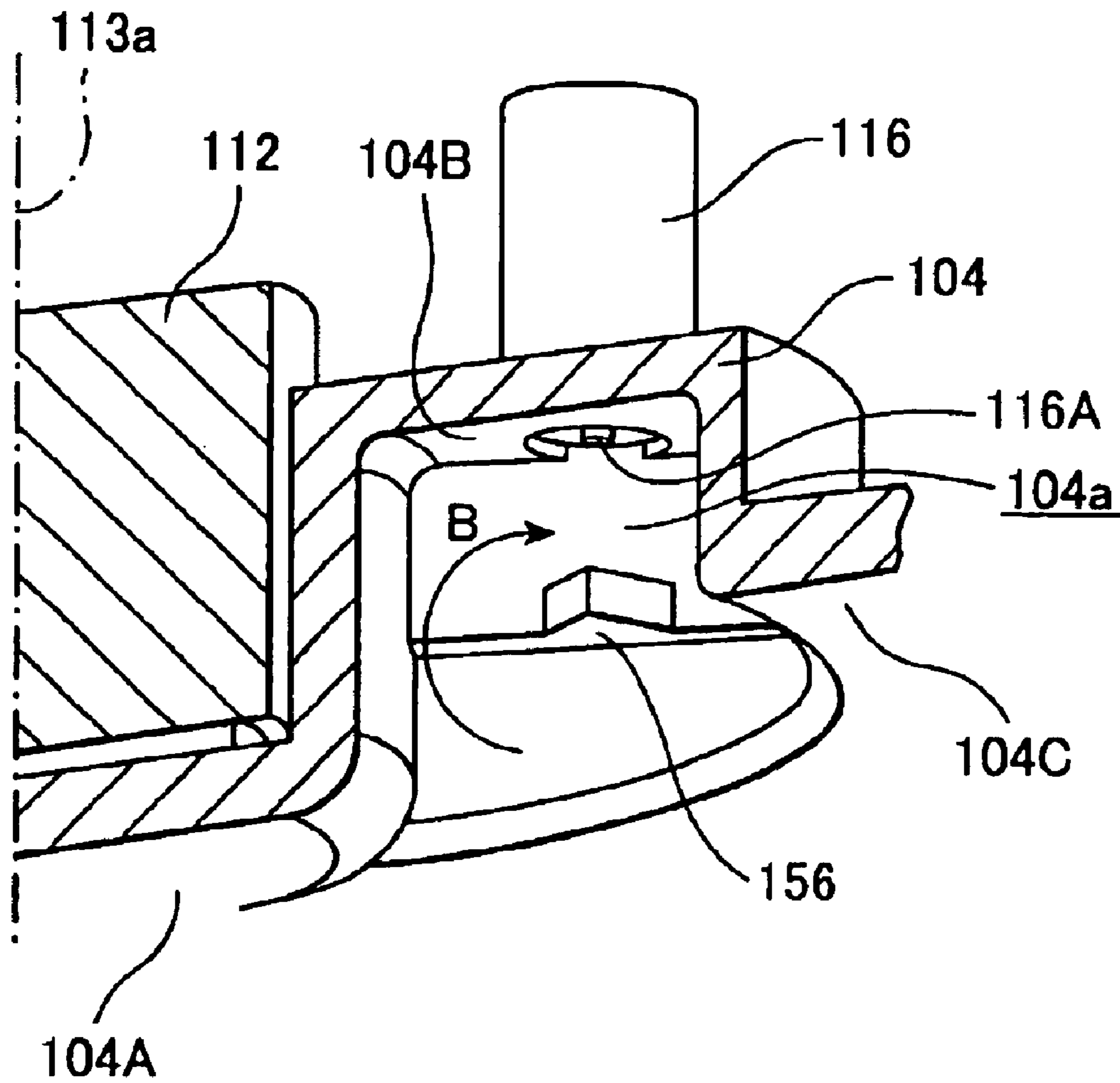
FIG. 4 PRIOR ART
