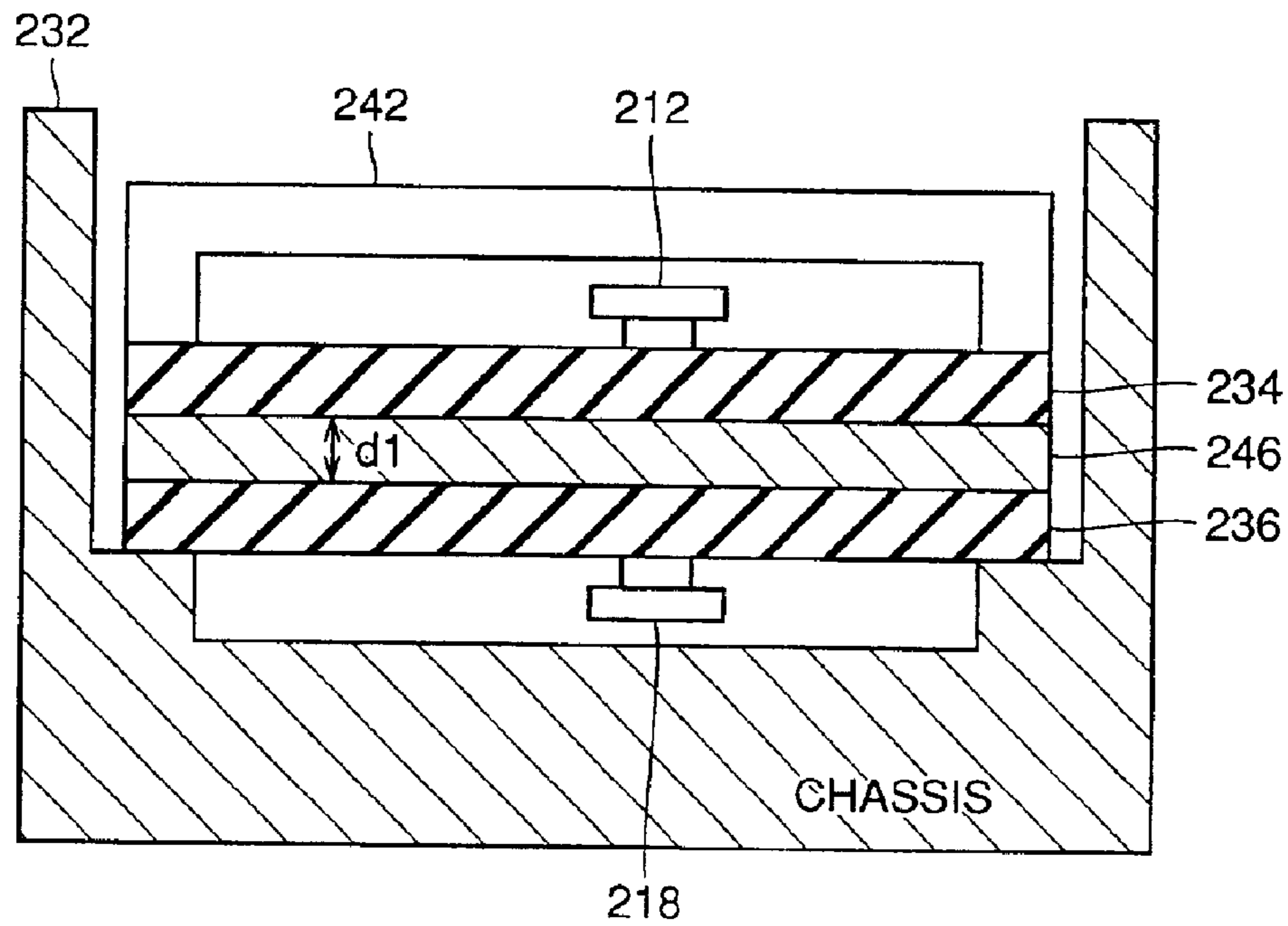
FIG. 10 PRIOR ART
