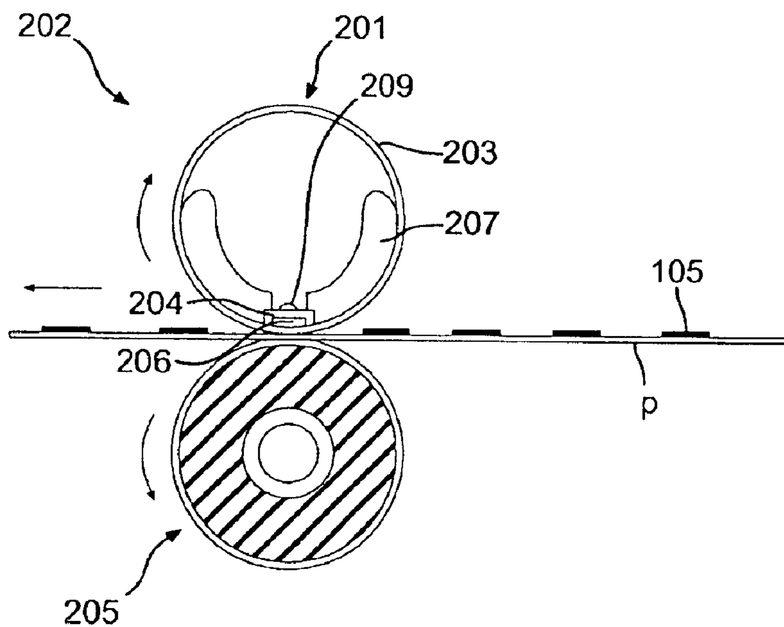
FIG. 5 PRIOR ART
