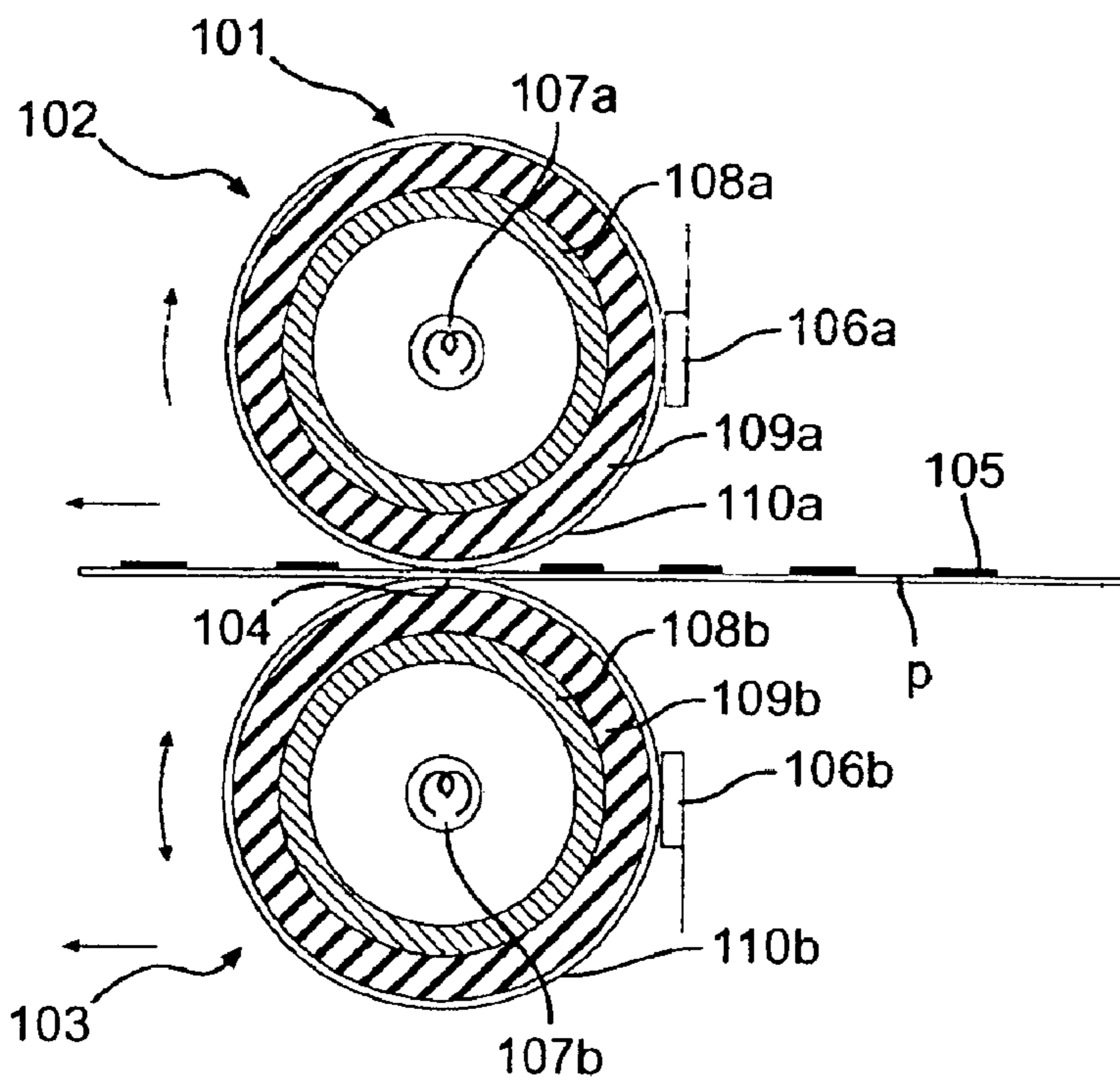
FIG. 4 PRIOR ART
