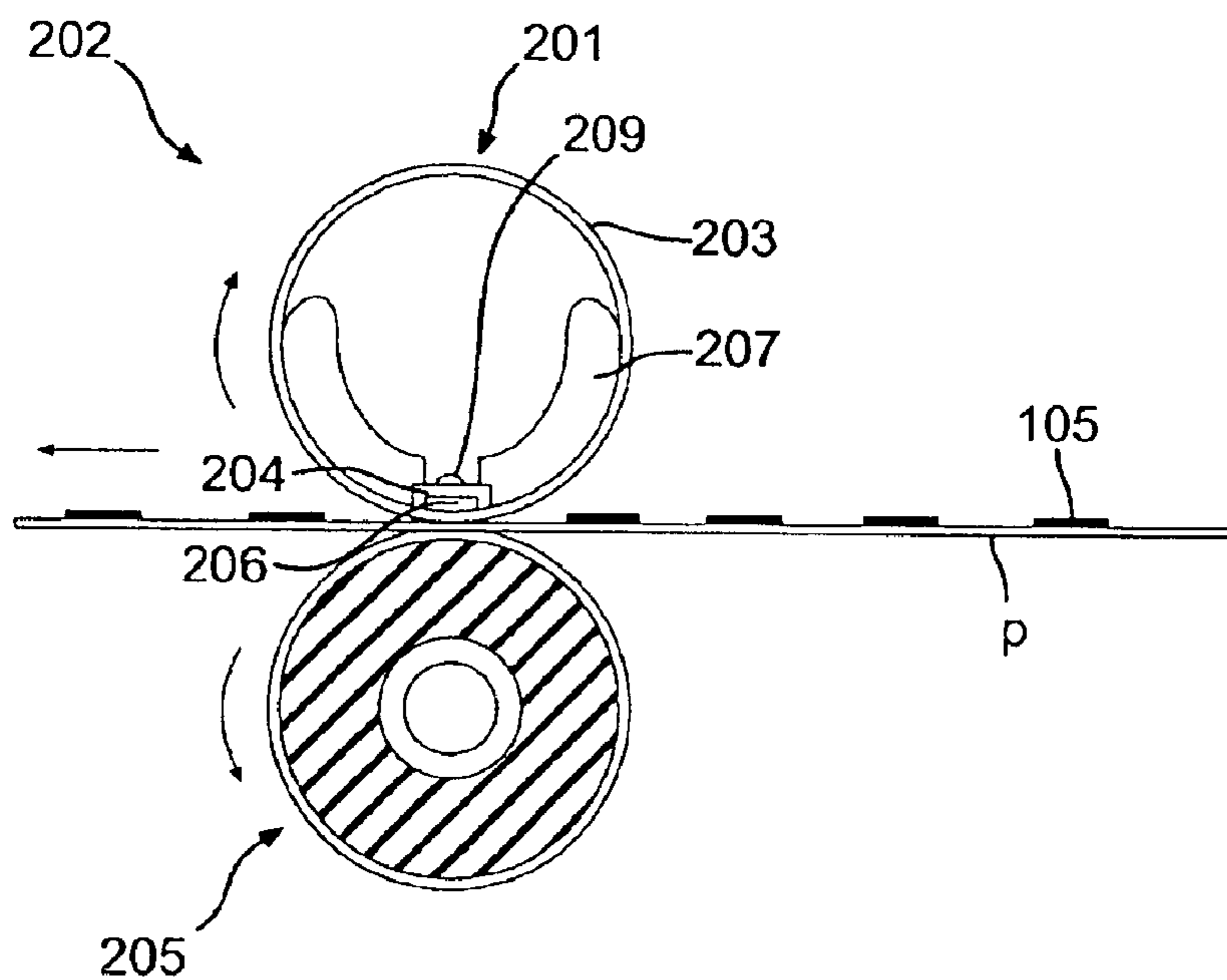
FIG. 5 PRIOR ART
