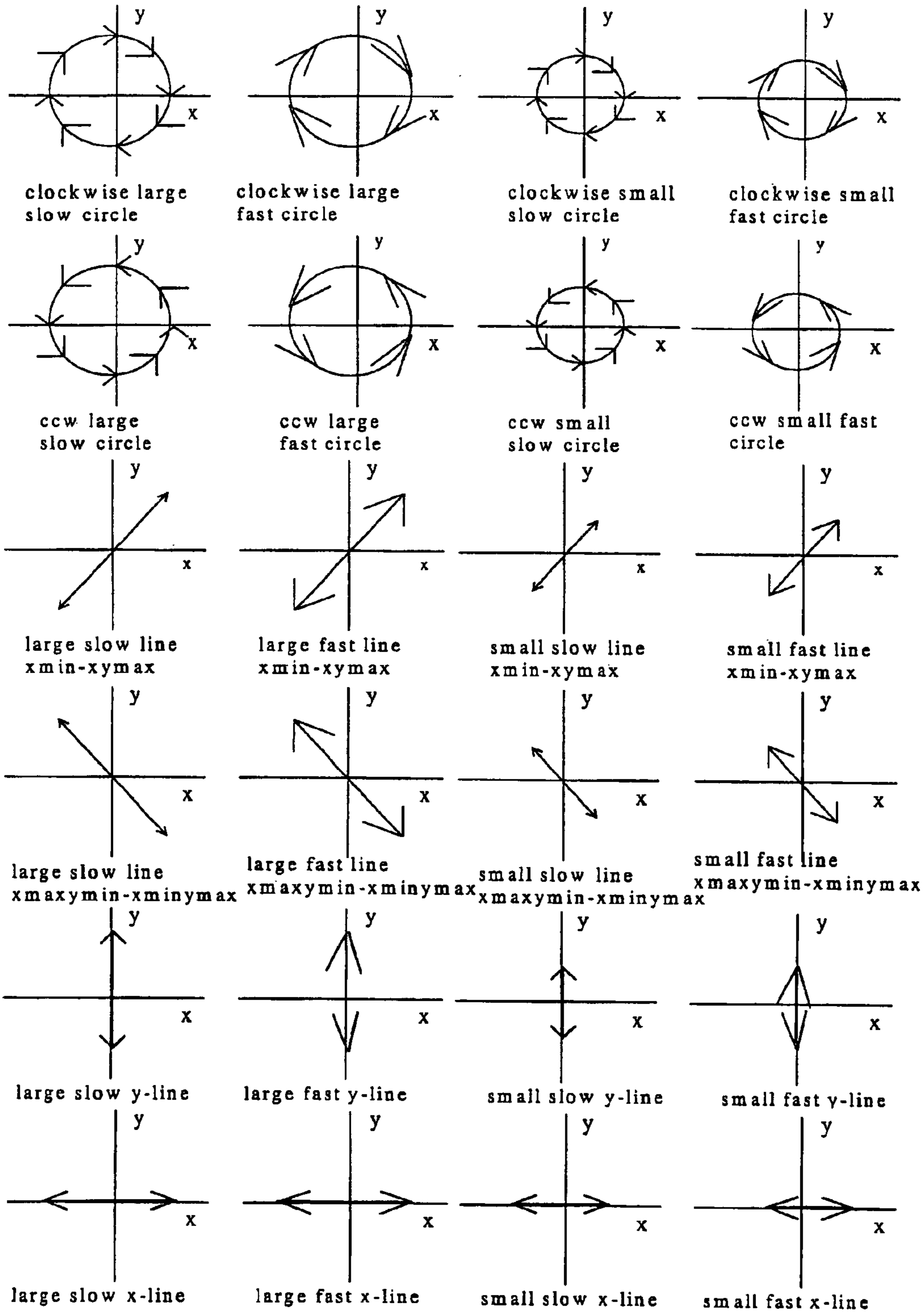
Figure 6: An Example 24 Gesture Lexicon.
