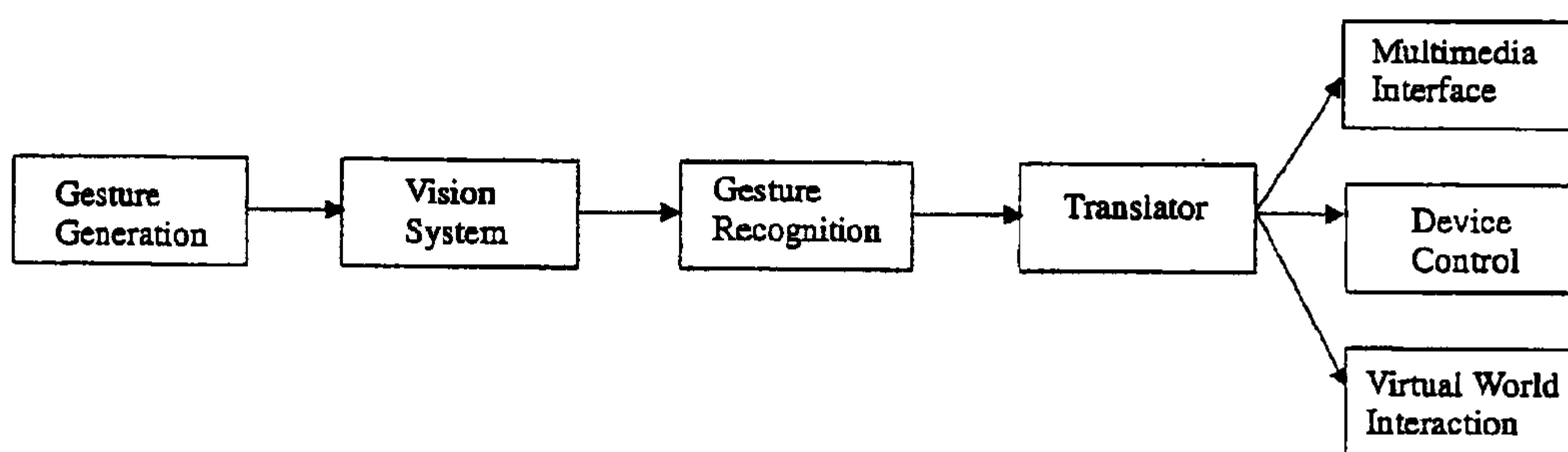
Figure 2: Gesture Recognition System Flow Chart.
