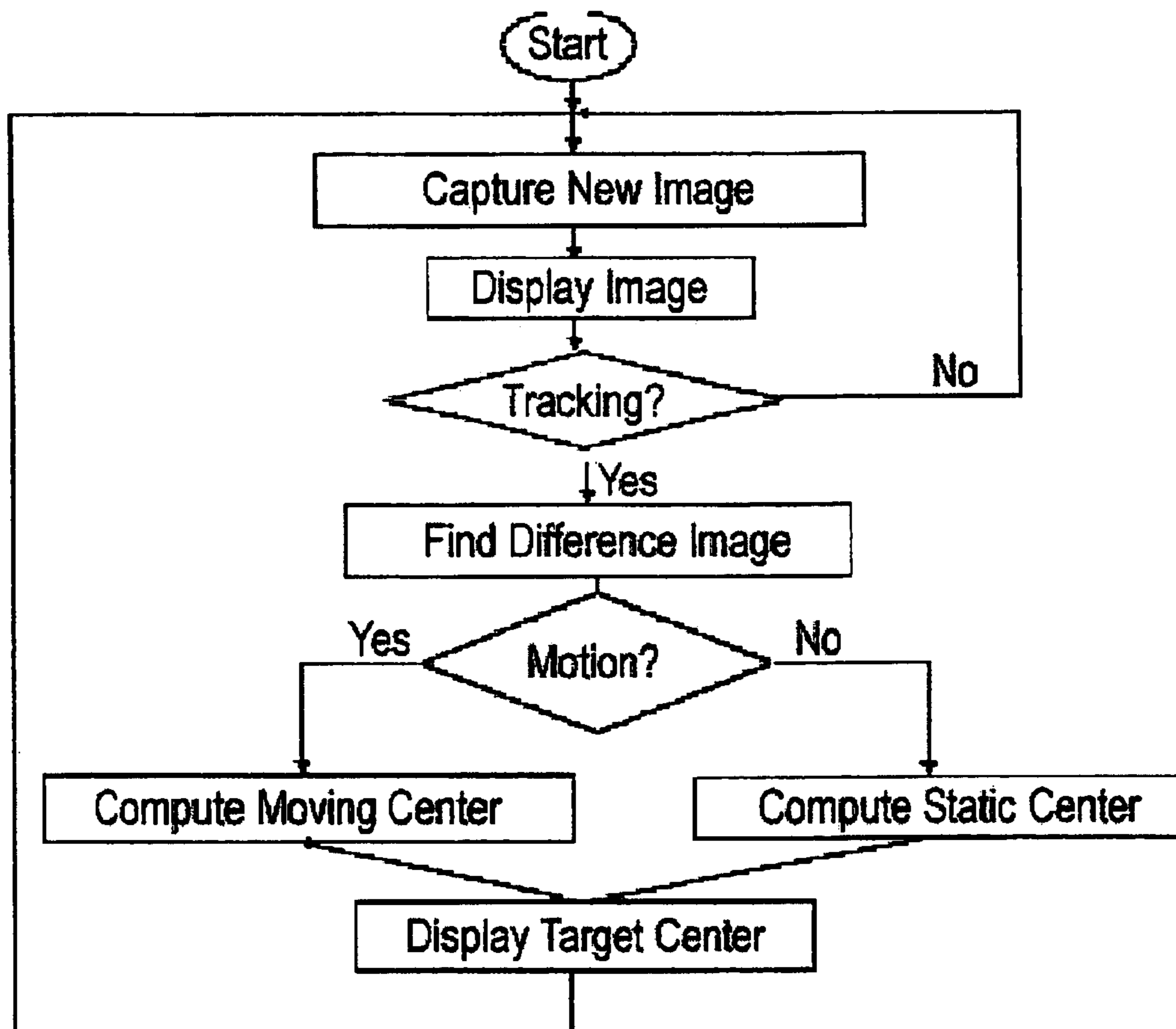
Figure 27: Flowchart of the CTS.
