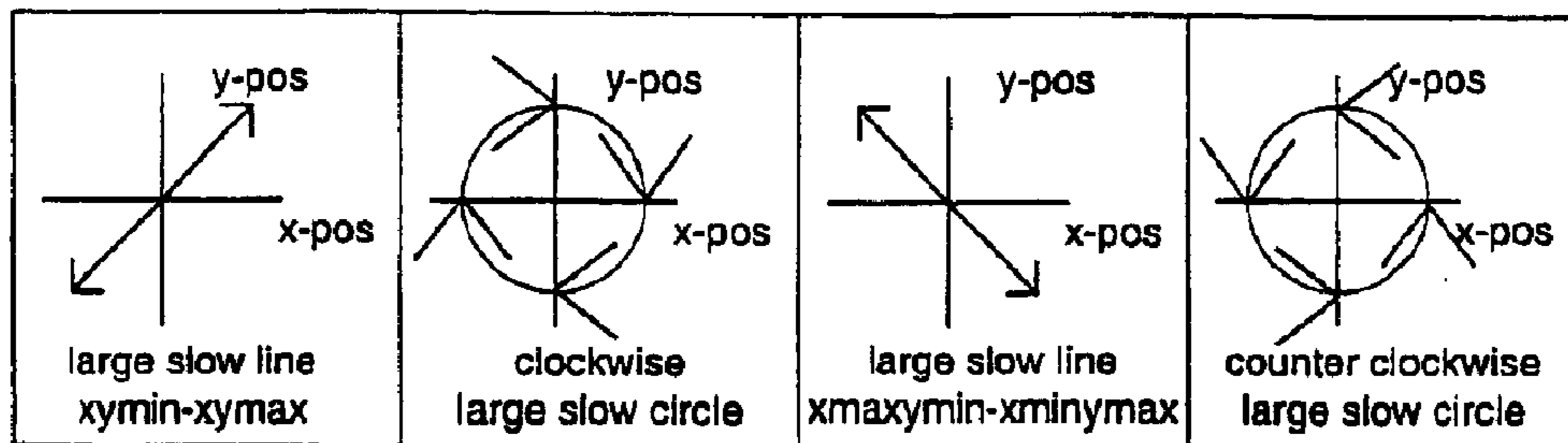
Figure 4: Example gestures, showed in two dimensions.
