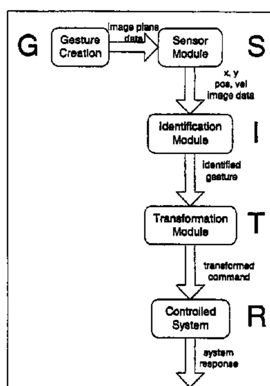
Signal Flow Diagram of the Gesture Recognition System.
