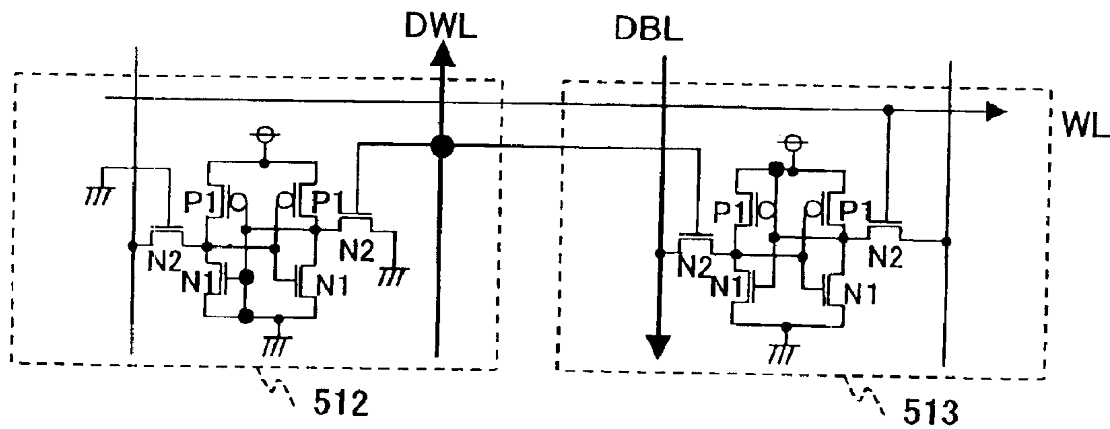
FIG.28 PRIOR ART
