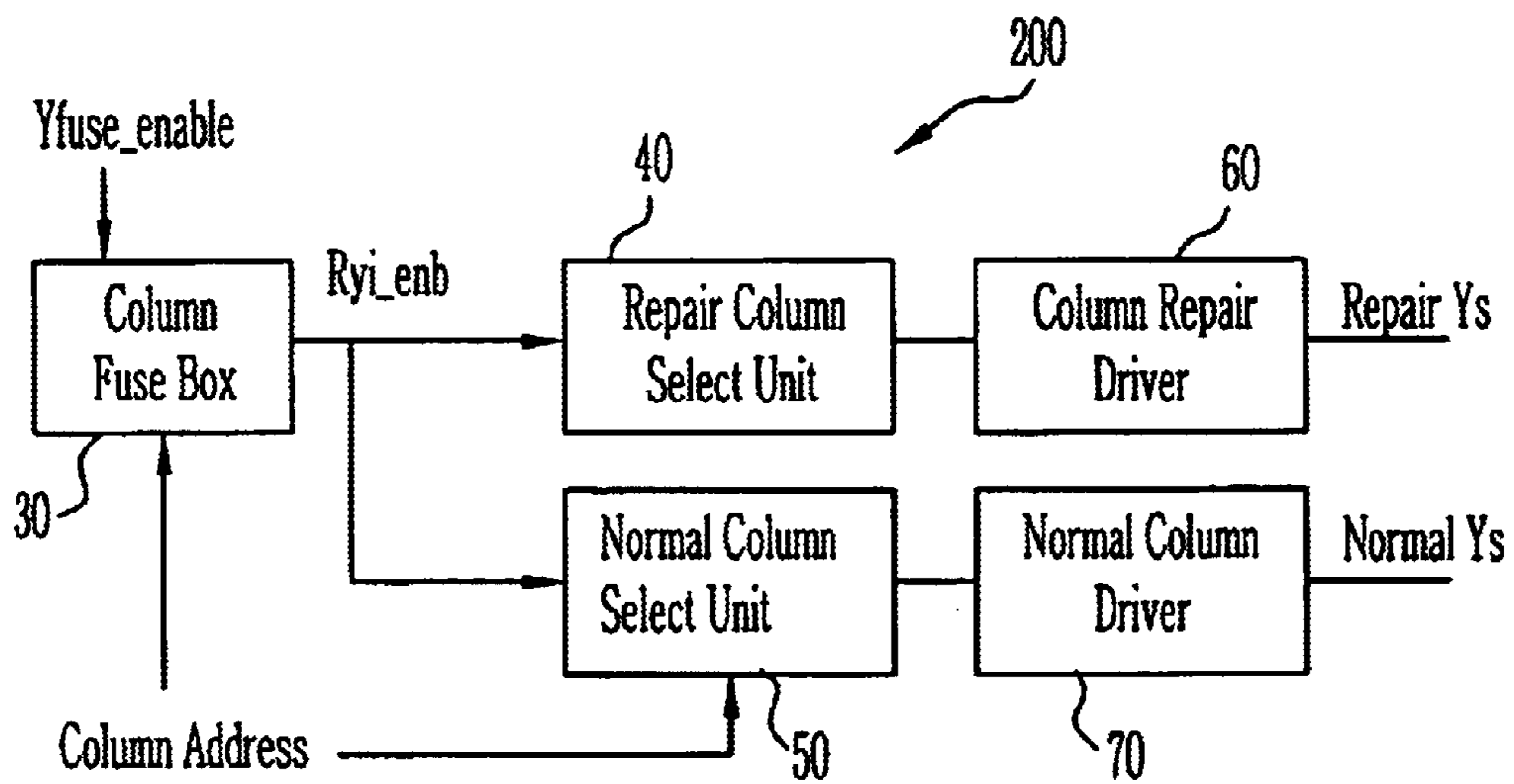
FIG. 4 (PRIOR ART)
