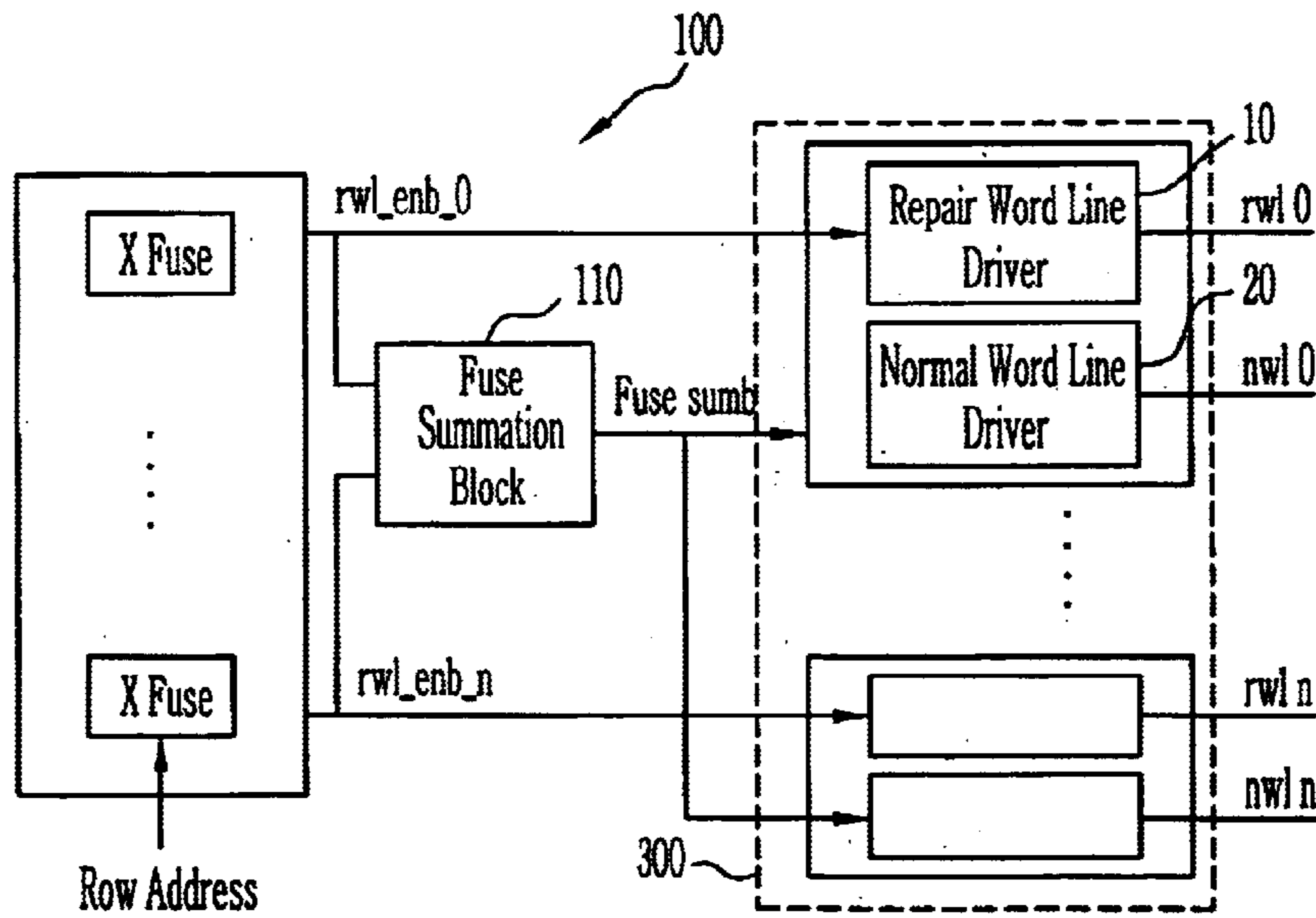
FIG. 2 (PRIOR ART)
