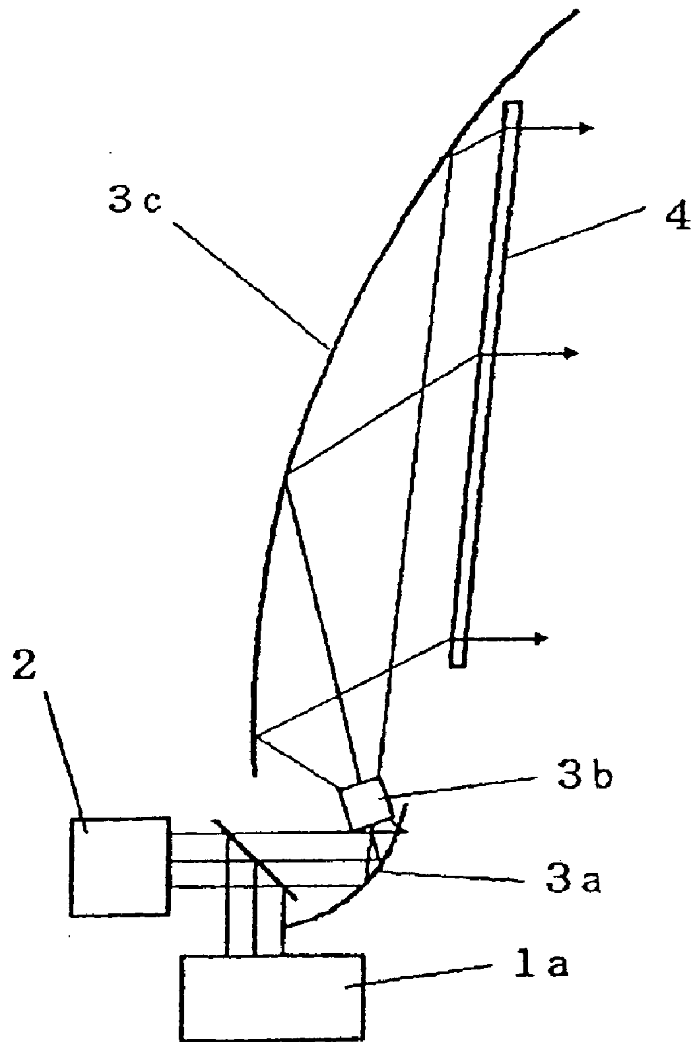
FIG. 37 (PRIOR ART)
