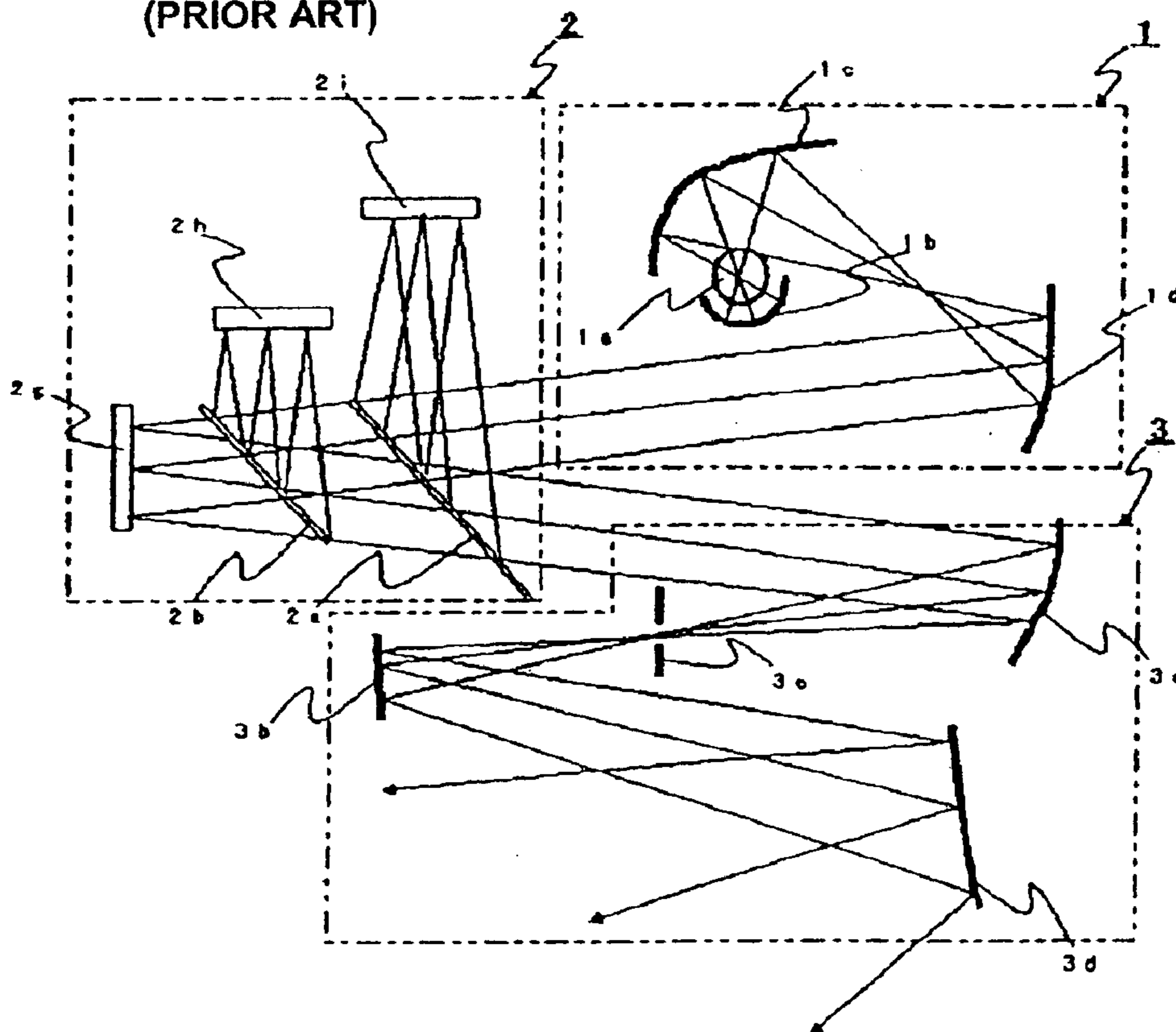
FIG. 28 (PRIOR ART)
