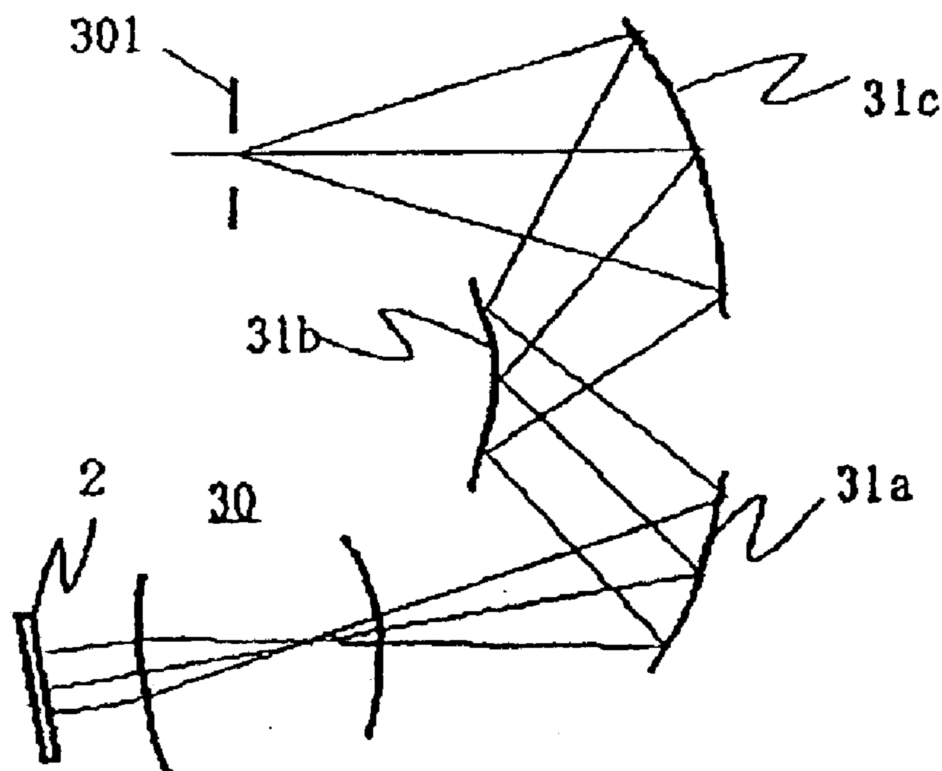
FIG. 44 (PRIOR ART)
