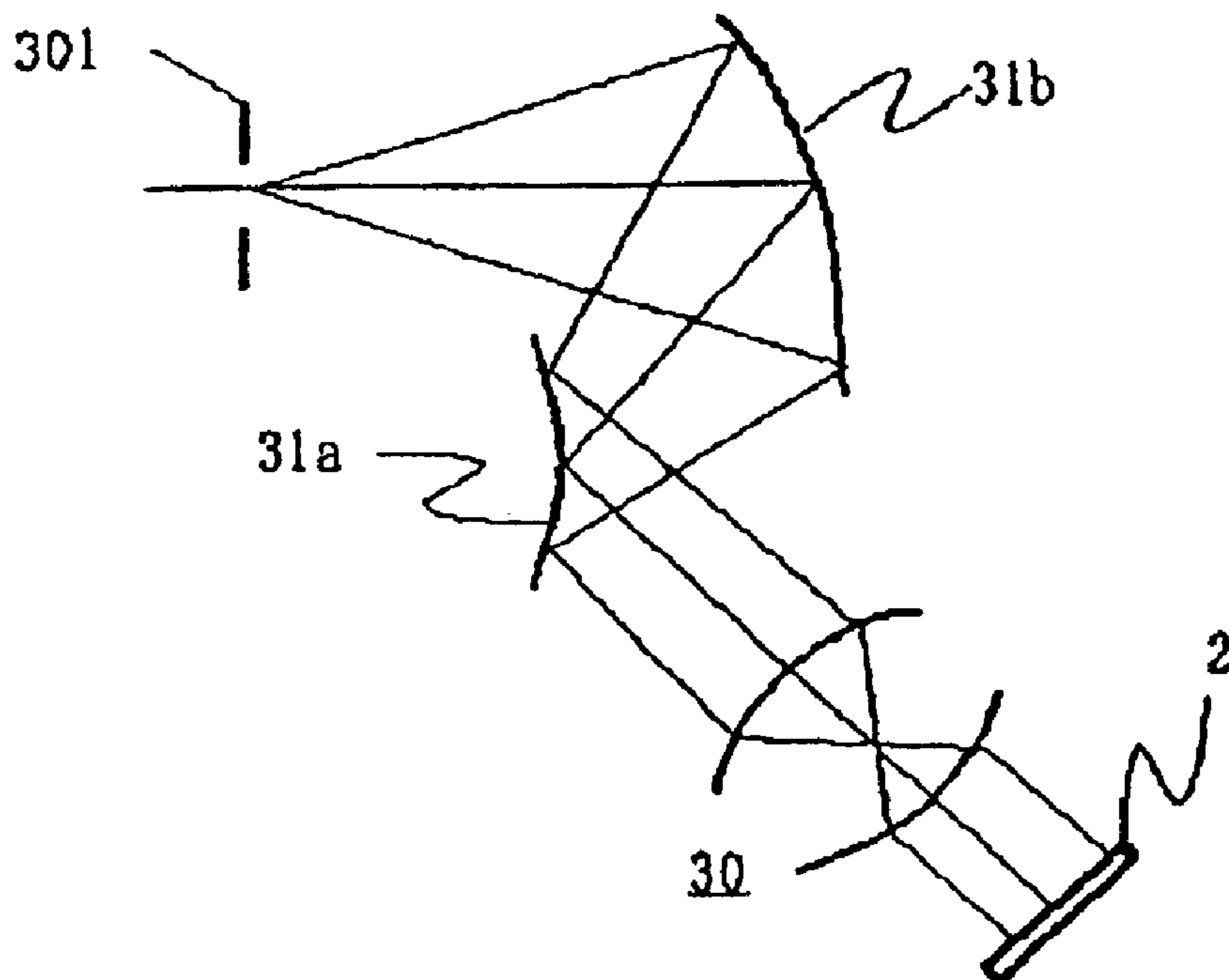
FIG. 43 (PRIOR ART)
