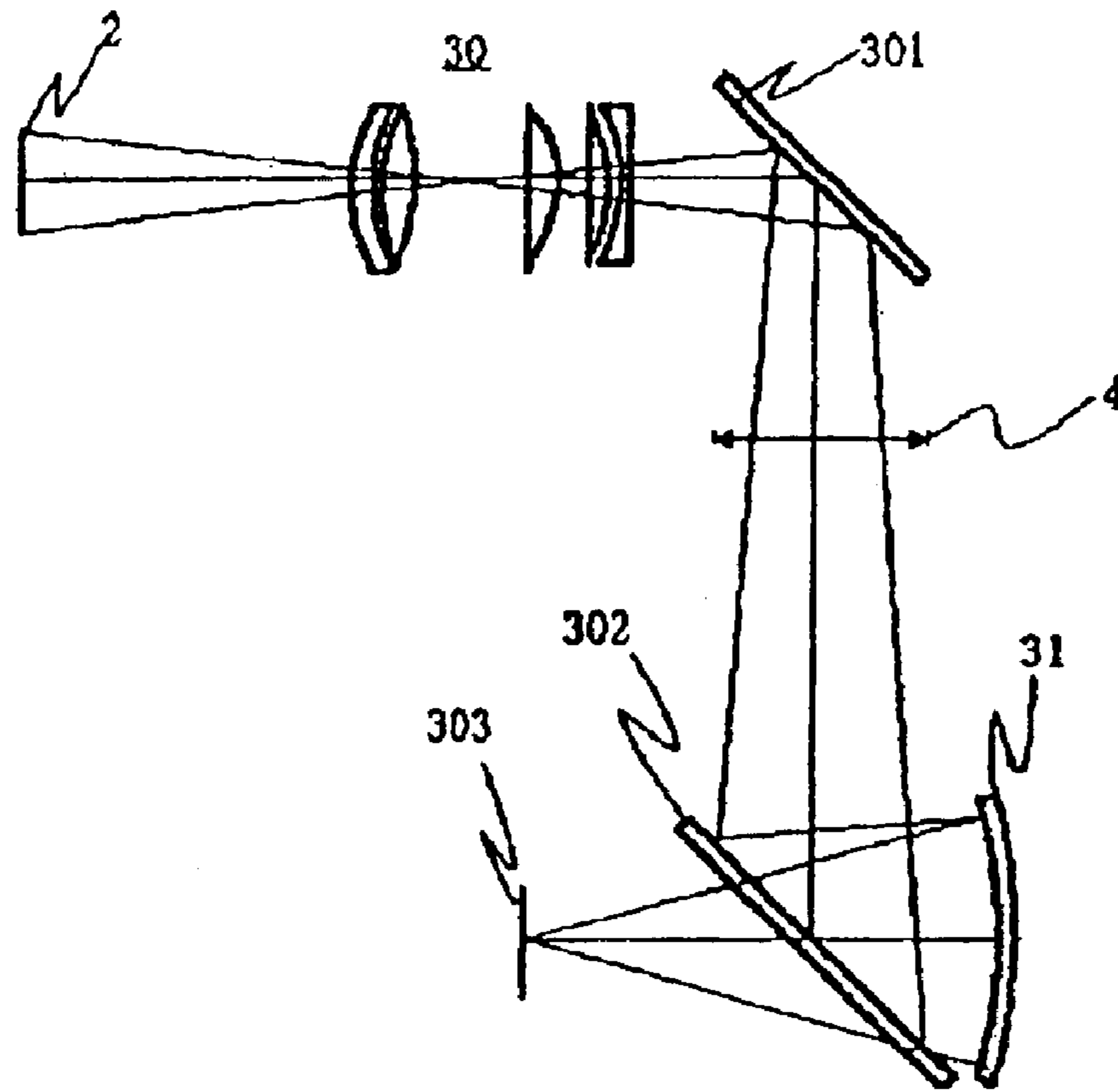
FIG. 41 (PRIOR ART)
