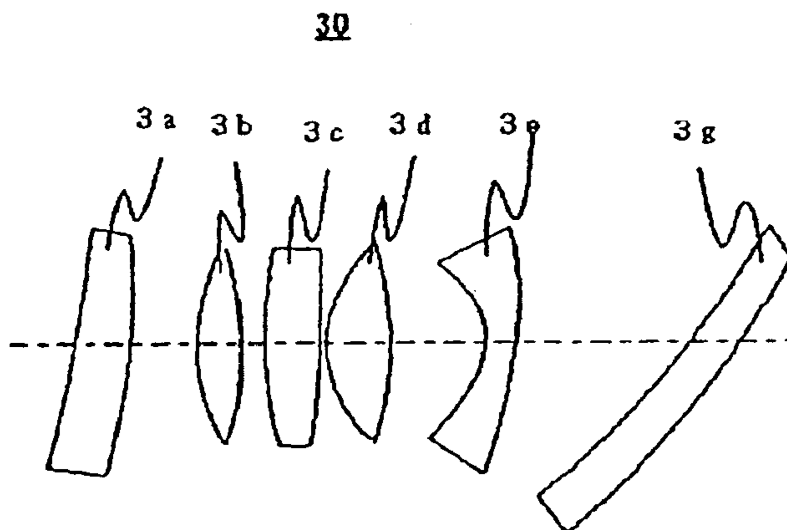
FIG. 39 (PRIOR ART)
