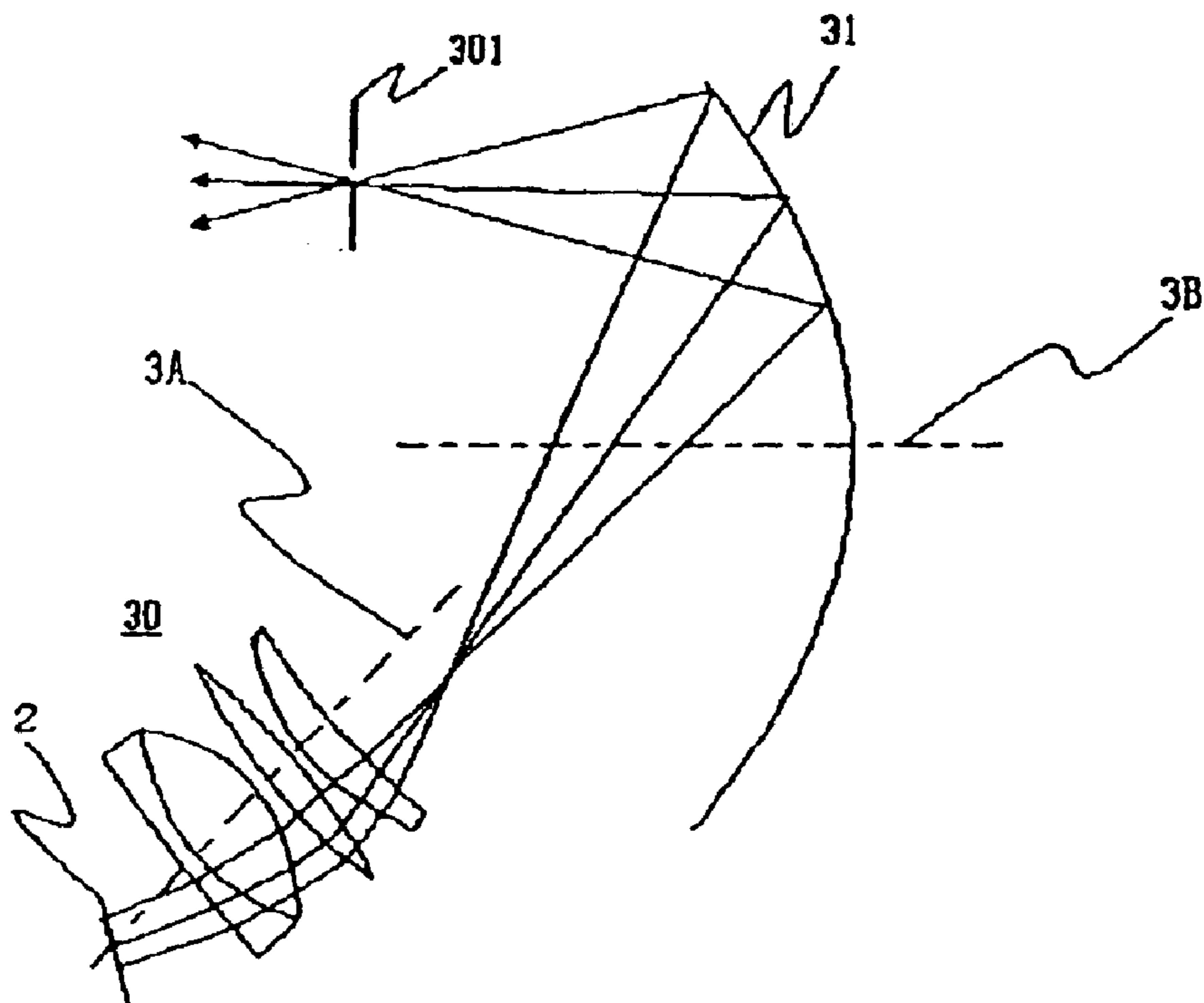
FIG. 41 (PRIOR ART)
