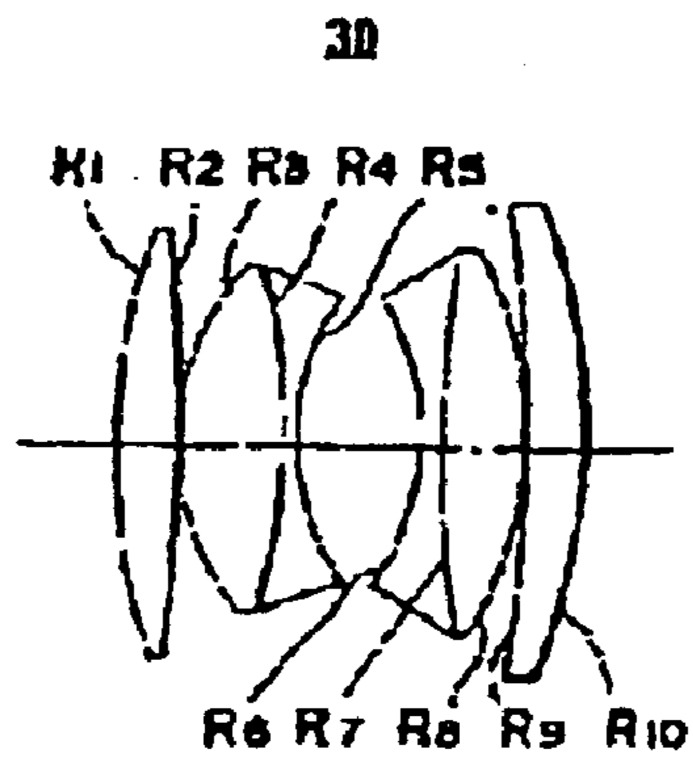
FIG. 32 (PRIOR ART)
