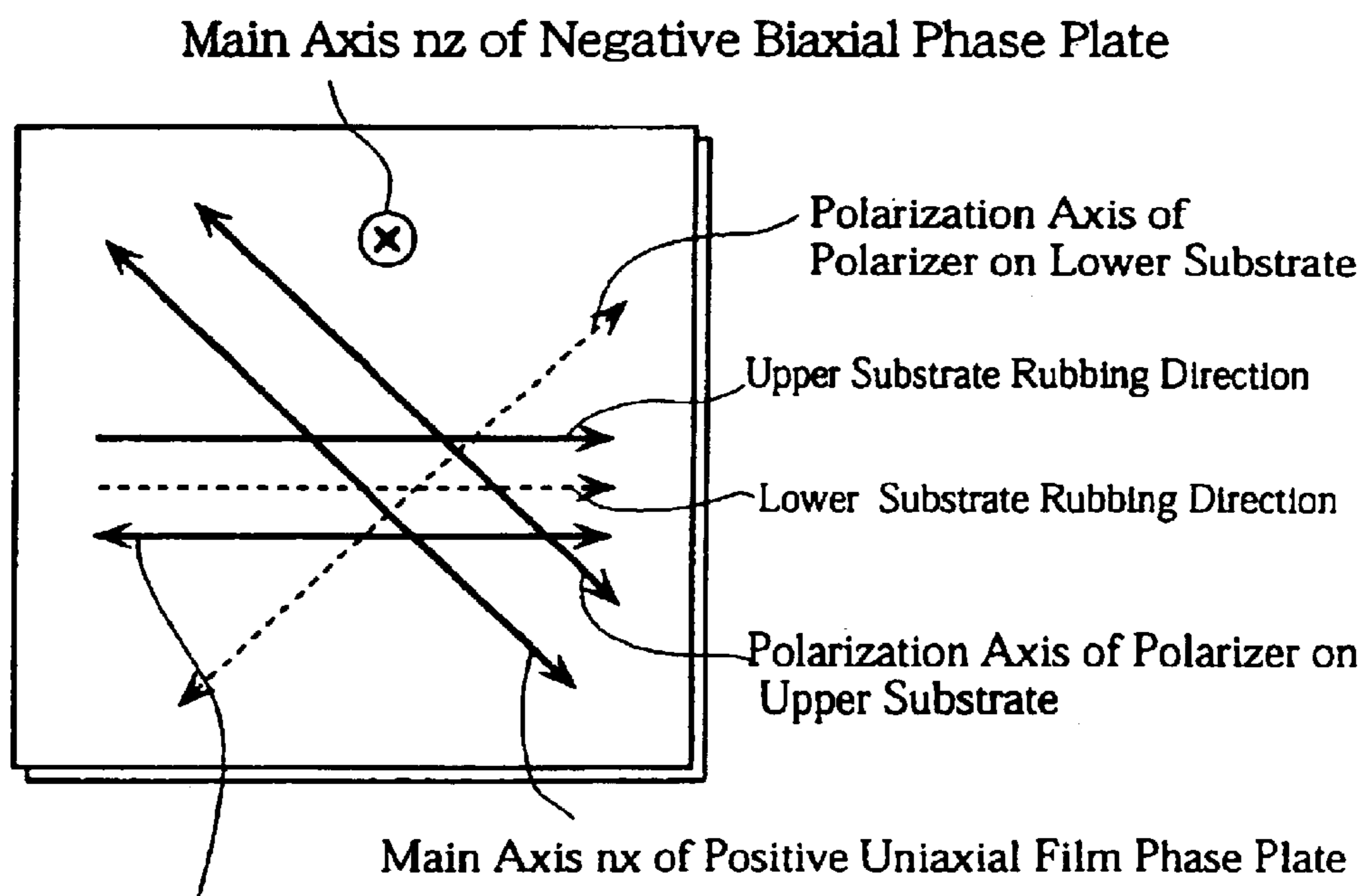
Orthographic Projection into the Substrate Plane of the Main Axis of Phase Difference Plate Made of an Optical Medium with Negative Reflective Index Anisotropy Whose Main Axes in Hybrid Arrangement
