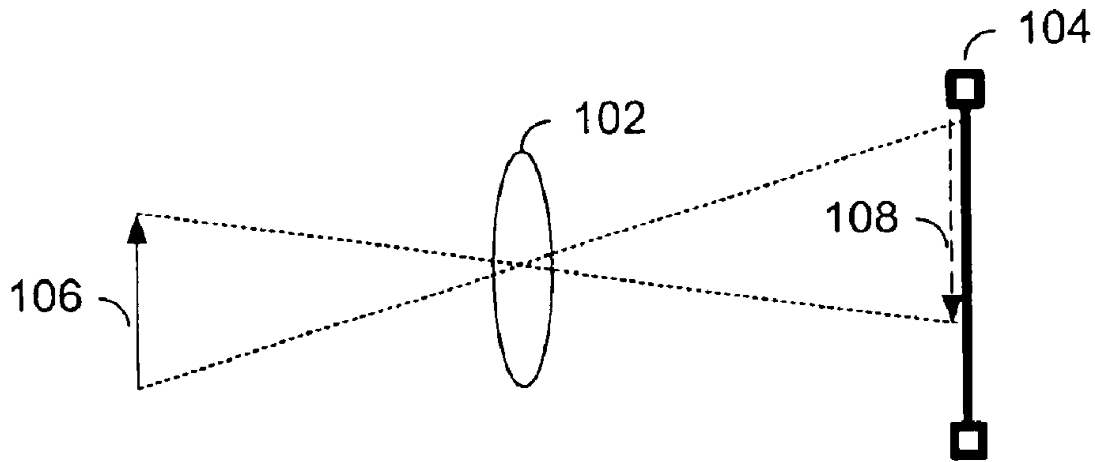
Fig. 1 (Prior Art)
